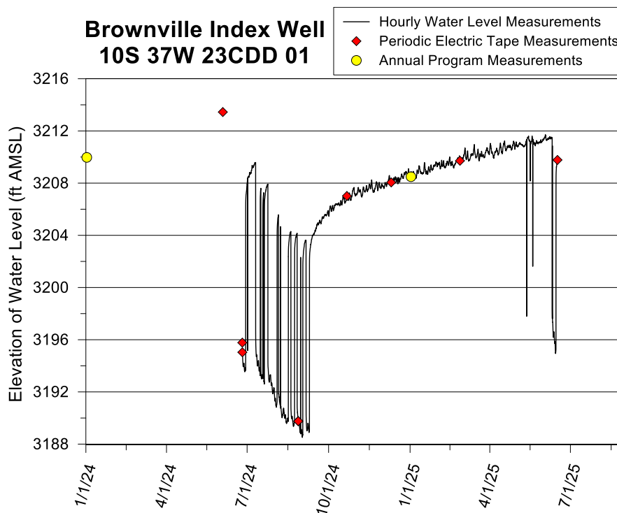
Figure 27—Brownville index well hydrograph—total data run to 6/16/25. A water-level elevation of 3,208 ft corresponds to a depth to water of 151 ft below lsf. The top of the 60 ft screen is 202 ft below lsf (elevation of 3,157 ft), and the bottom of the aquifer is 260 ft below lsf (elevation of 3,099 ft). There is a 2 ft sump below the bottom of the aquifer.
