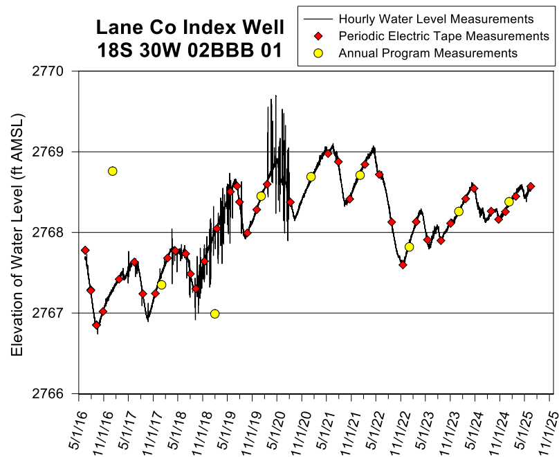
Figure 3—Lane County index well hydrograph—total data run to 6/16/25. A water-level elevation of 2,767 ft corresponds to a depth to water of 85 ft below land surface (lsf). The top of the screen is 105 ft below lsf (elevation of 2,747 ft), and the bottom of the aquifer is 118 ft below lsf (elevation of 2,734 ft). The screen terminates 3 ft above the bottom of the aquifer. The 2017 and 2019 annual water-level measurements appear to be in error. The in-field calibration approach described in Butler, Knobbe et al. (2021) has been applied to the transducer data to correct the drift noted in previous annual reports.
