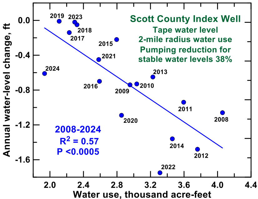
Figure 54—Correlation of annual water-level change based on manual measurements in the Scott County index well with annual water use within a 2 mi radius centered on the well during 2008–2024. The 2022 and 2024 water-level changes appear to have been affected by late-season pumping (recovery began on November 9, 2022, and October 24, 2024, respectively, while it typically begins in early to mid-September).
