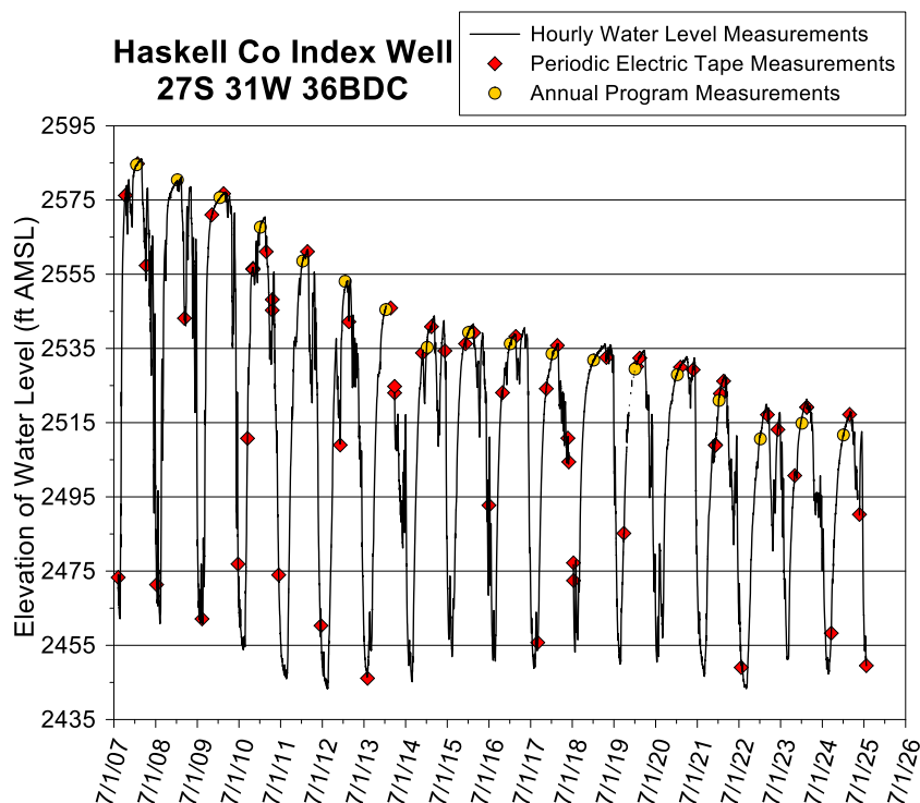
Figure 16—Haskell County index well hydrograph—total data run to 7/21/25. A water-level elevation of 2,455 ft corresponds to a depth to water of 382.8 ft below lsf. The top of the screen is 420 ft below lsf (elevation of 2,417.8 ft), and the bottom of the aquifer is 433 ft below lsf (elevation of 2,404.8 ft). The screen terminates 3 ft above the bottom of the aquifer. A sensor failure produced a break in monitoring from January to March 2014; a damaged cable produced a break in monitoring from early June to mid-July 2018; a malfunctioning sensor began producing many spurious values on 10/17/19 and was replaced on 1/16/20—only the sensor values deemed reasonable are plotted during that three-month period. A sensor failure produced a break in monitoring from 5/7/25 to 5/22/25.
