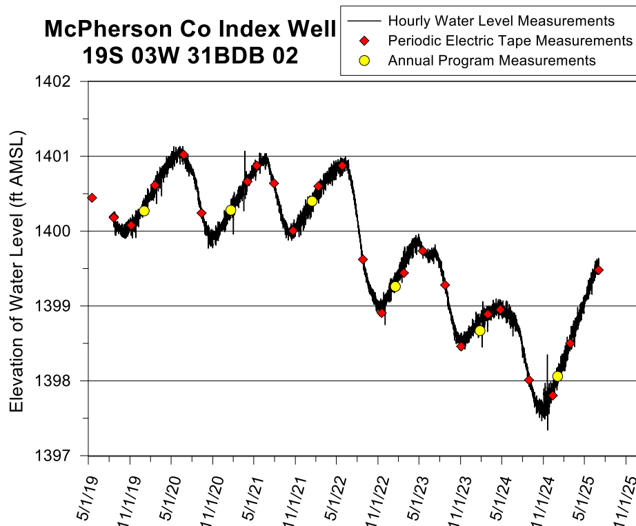
Figure 11—McPherson County index well hydrograph—total data run to 7/3/25. A water-level elevation of 1,400 ft corresponds to a depth to water of 94 ft below lsf. The top of the 44 ft screen is 139 ft below lsf (elevation of 1,355 ft), and the bottom of the screen is 183 ft below lsf (elevation of 1,311 ft). The bottom of the aquifer is 1 ft below the bottom of the screen (1,310 ft). We have yet to identify the mechanisms producing the infrequent anomalous spikes.
