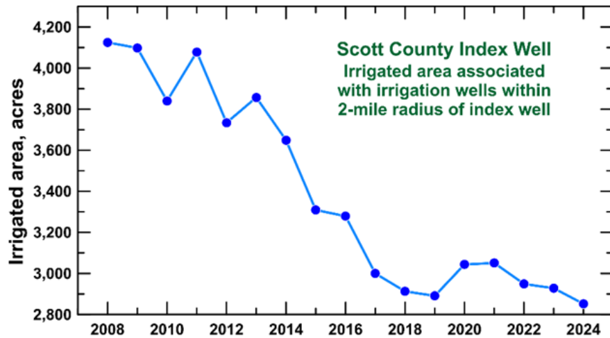
Figure 59—Change in irrigated area associated with the irrigation wells within the 2 mi radius of the Scott County index well for 2008–2024.
