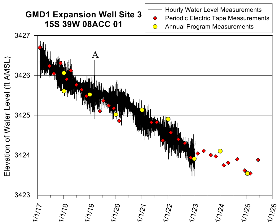
Figure 47—GMD1 Expansion Site 3 well hydrograph—total data run to 6/16/25. A water-level elevation of 3,424 ft corresponds to a depth to water of 199 ft below Isf. Bottom of well is 219.9 ft below Isf (elevation of 3,403.1 ft). A defined in text.
