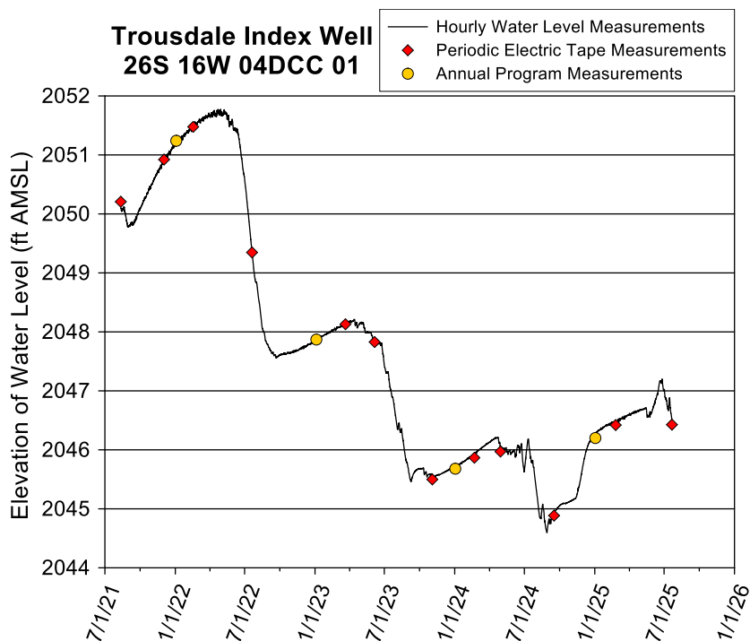
Figure 43—Trousdale index well hydrograph—total data run to 7/21/25. A water-level elevation of 2,046 ft corresponds to a depth to water of 38.8 ft below Isf. The top of the 10 ft screen is 47 ft below Isf (elevation of 2,037.8 ft). The bottom of the well is 57 ft below Isf (elevation of 2,027.8 ft); the base of the aquifer is at least 80 ft below the bottom of the well.
