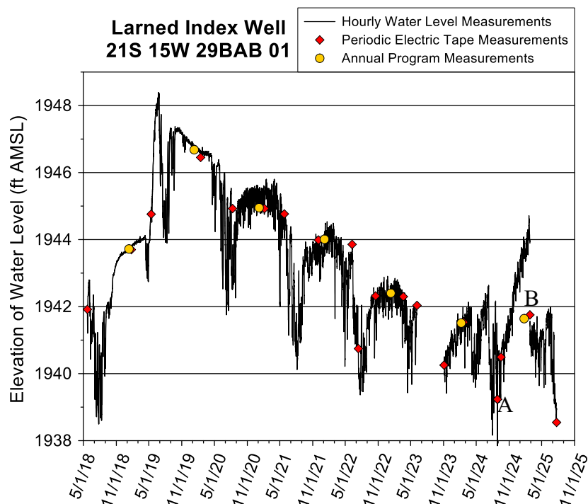
Figure 40—Larned index well hydrograph—total data run to 7/23/25. A water-level elevation of 1,942 ft corresponds to a depth to water of 13.3 ft below Isf. The top of the 5 ft screen is 66 ft below Isf (elevation of 1,889.3 ft), and the bottom of the screen, which is at the base of the aquifer, is 71 ft below Isf (elevation of 1,884.3 ft). Break in monitoring from 6/5/23 to 11/3/23 because of cable and transducer problems. A new transducer was installed on 8/27/24 (A) but malfunctioned and produced erroneous readings (e.g., 2.28 ft above 1/23/25 annual measurement). This transducer was replaced on 2/24/25 (B).
