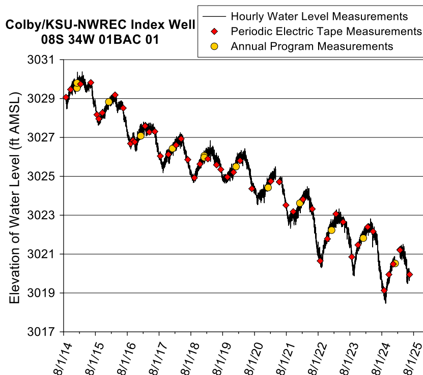
Figure 29—Colby index well hydrograph—total data run to 6/15/25. A water-level elevation of 3,021 ft corresponds to a depth to water of 156 ft below Isf. Total depth of the well is 175 ft below Isf (elevation of 3,002 ft). The screened interval extends from 156 to 175 ft below Isf. The base of the aquifer is estimated to be 250–300 ft below Isf (Butler, Whittemore et al., 2017). Sensor failed on 4/1/21 and was replaced on 5/12/21; sensor failed on 12/27/24 and was replaced on 2/25/25.
