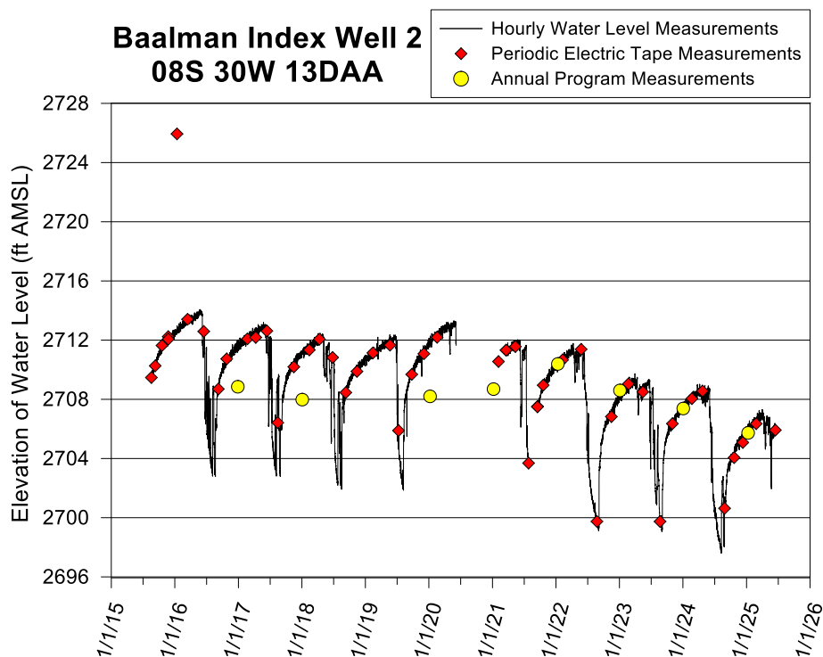
Figure 30—Baalman index well hydrograph—total data run to 6/15/25. A water-level elevation of 2,708 ft corresponds to a depth to water of 189 ft below lsf. The top of the 10 ft screen is 260 ft below lsf (elevation of 2,637 ft), and the bottom of the aquifer is 262 ft below lsf (elevation of 2,635 ft). The difference between the electric-tape and transducer measurements in January 2016 was caused by a malfunctioning electric tape.
