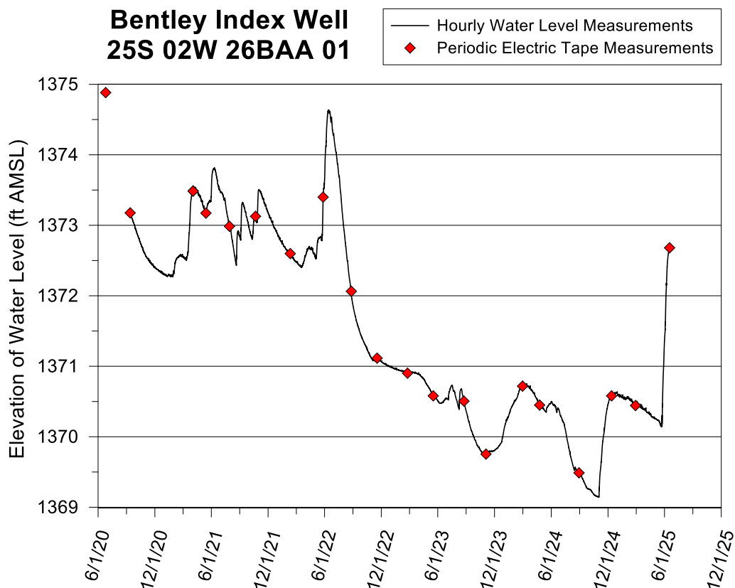
Figure 9—Bentley index well hydrograph—total data run to 6/17/25. A water-level elevation of 1,373 ft corresponds to a depth to water of 8 ft below lsf. The top of the 10 ft screen is 23 ft below lsf (elevation of 1,358 ft). The bottom of the aquifer is approximately 216 ft below lsf (elevation of 1,165 ft), and the bottom of the well is 33 ft below lsf (elevation of 1,348 ft).
