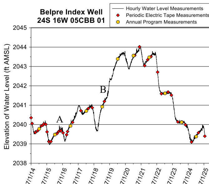
Figure 39—Belpre index well hydrograph—total data run to 7/21/25. A water-level elevation of 2,040 ft corresponds to a depth to water of 40 ft below Isf. The top of the 20 ft screen is 89 ft below Isf (elevation of 1,991 ft), and the bottom of the screen is 109 ft below Isf (elevation of 1,971 ft). The base of the aquifer is estimated to be 175–200 ft below Isf (elevation of 1,905–1,880 ft). A and B defined in text.
