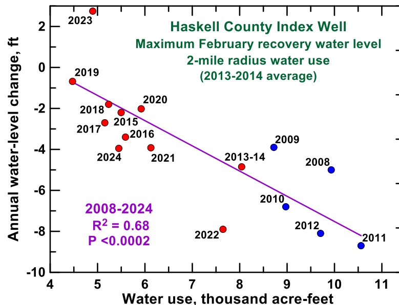
Figure 55—Correlation of change in maximum recovery water level during February based on transducer measurements in the Haskell County index well with annual water use within a 2 mi radius centered on the well during 2008–2024. Red points designate values after the court-ordered shutdowns (see section 3.3.2); 2013 and 2014 values are averaged because of equipment failure at the time of the 2013 maximum recovery. The 2022 value appears to have been affected by late-year (December) pumping; the result is that the 2022 value is more negative than would have been expected for the 2022 annual pumping and the 2023 value is more positive than would have been expected for the 2023 annual pumping.
