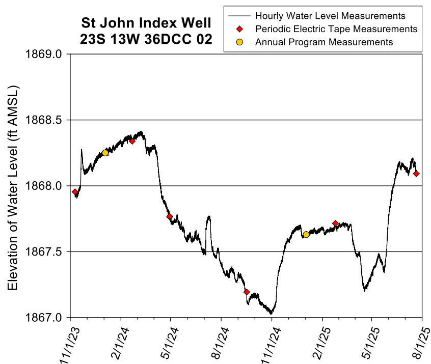
Figure 42—St. John index well hydrograph—total data run to 7/21/25. A water-level elevation of 1,868 ft corresponds to a depth to water of 30 ft below lsf. The top of the 10 ft screen is 65 ft below lsf (elevation of 1,833 ft). The bottom of the well is 75 ft below lsf (elevation of 1,823 ft); the base of the aquifer is 142 ft below lsf (elevation of 1,756 ft).
