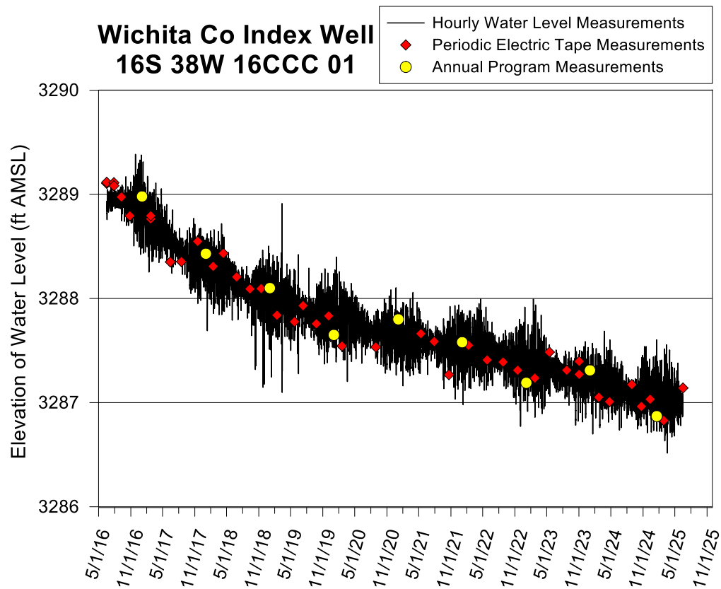
Figure 6—Wichita County index well hydrograph—total data run to 6/16/25. A water-level elevation of 3,287 ft corresponds to a depth to water of 161 ft below lsf. The top of the screen is 175 ft below lsf (elevation of 3,273 ft), and the bottom of the aquifer is 190 ft below lsf (elevation of 3,258 ft). The screen terminates 5 ft above the bottom of the aquifer. The in-field calibration approach described in Butler, Knobbe et al. (2021) has been applied to the transducer data to correct for sensor drift.
