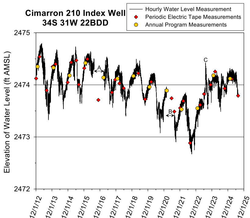
Figure 15—Cimarron 210 index well hydrograph—total data run to 7/23/25. A water-level elevation of 2,474 ft corresponds to a depth to water of 55 ft below Isf. The top of the 10 ft screen is 200 ft below Isf (elevation of 2,329 ft), and the bottom of the aquifer is 345 ft below Isf (elevation of 2,184 ft); A-C defined in text.
