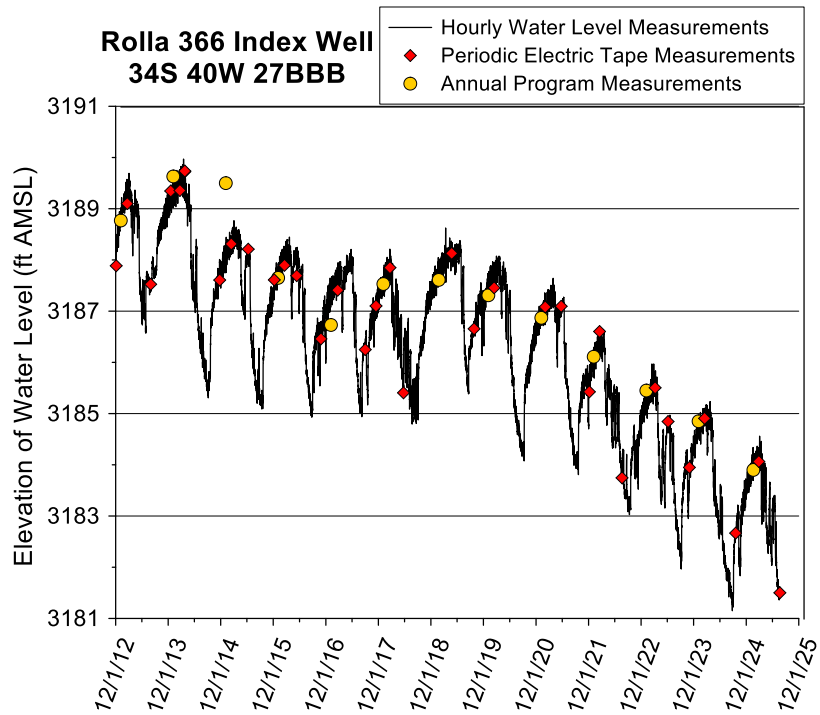
Figure 22—Rolla 366 index well hydrograph—total data run to 7/22/25. A water-level elevation of 3,185 ft corresponds to a depth to water of 190 ft below Isf. The top of the 10 ft screen is 356 ft below Isf (elevation of 3,019 ft), and the bottom of the aquifer is 399 ft below Isf (elevation of 2,976 ft). Note the suspect 2015 and 2017 annual program measurements.
