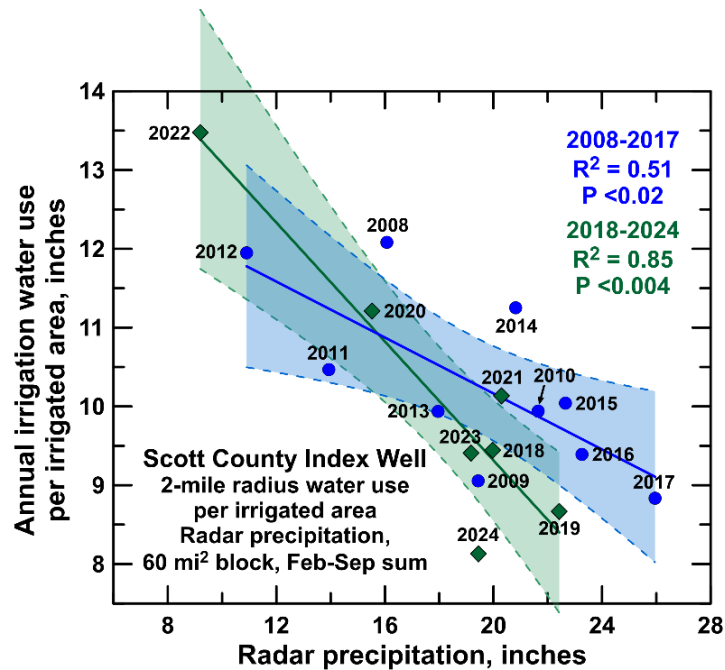
Figure 58—Correlation of annual irrigation groundwater use per irrigated area with radar precipitation at the Scott County index well for 2008–2024. The shaded intervals represent the 95% confidence interval for the linear regressions.
