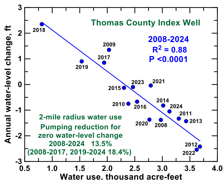
Figure 53—Correlation of annual water-level change based on manual measurements in the Thomas County index well with annual water use within a 2 mi radius centered on the well during 2008–2024.
