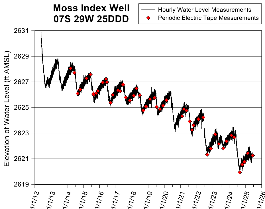
Figure 32—Moss index well hydrograph—total data run to 6/15/25. A water-level elevation of 2,621 ft corresponds to a depth to water of 195 ft below lsf. The top of the 40 ft screen is 205 ft below lsf (elevation of 2,611 ft), and the bottom of the aquifer is 243 ft below lsf (elevation of 2,573 ft). Measurements affected by datalogger overheating (mid-summer 2015 and earlier) are not displayed.
