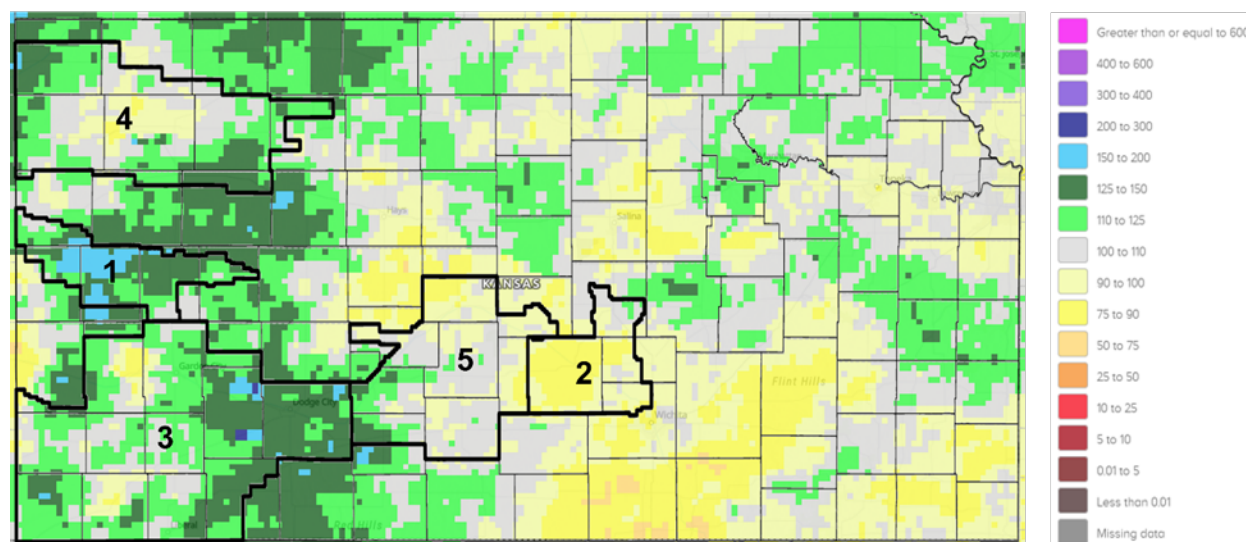
Figure 50—Percent of normal radar precipitation for Kansas in 2024. County lines are displayed and the GMD numbers and boundaries are bolded.
