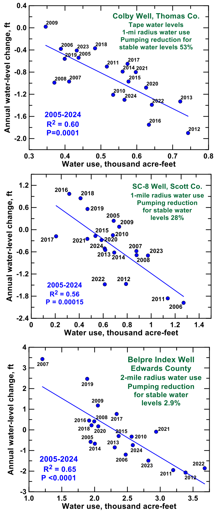
Figure 56—Correlation of annual water-level change in the Colby, SC-8, and Belpre wells with annual water use within a 1 or 2 mi radius centered on the wells during 2005–2024.
