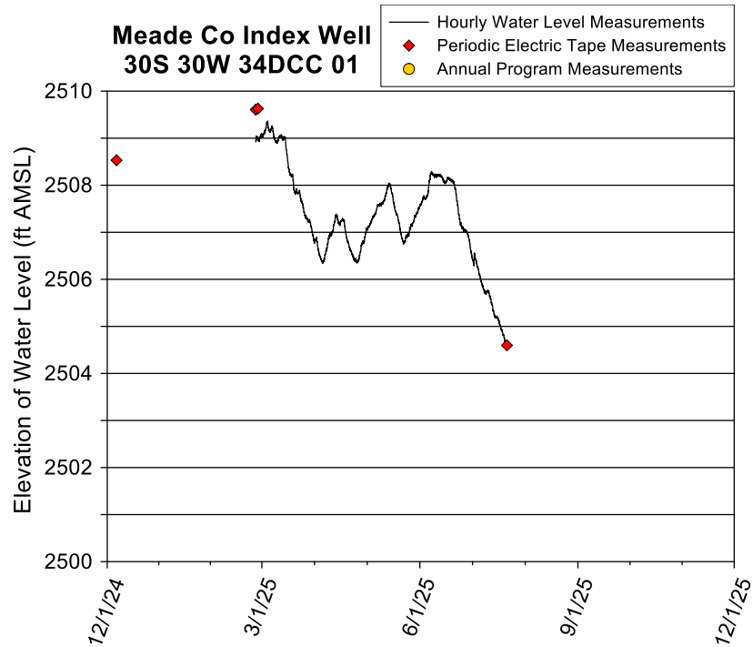
Figure 21 — Meade County index well hydrograph—total data run to 7/21/25. A water-level elevation of 2,508 ft corresponds to a depth to water of 249 ft below lsf. The top of the 40 ft screen is 420 ft below lsf (elevation of 2,337 ft). The bottom of the well is 457 ft below lsf (elevation of 2,300 ft); the base of the aquifer is 454 ft below lsf (elevation of 2,303 ft).
