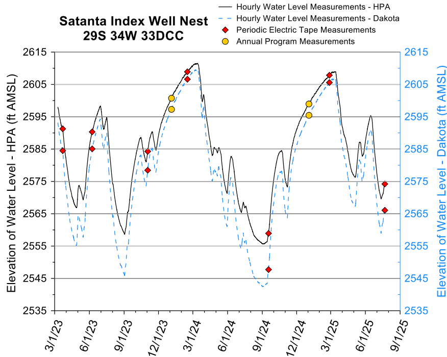
Figure 23—Satanta site hydrographs—total data run to 7/22/25. A water-level elevation of 2,575 ft corresponds to a depth to water of 405 ft below Isf. The top of the 20 ft screen in the HPA is 500 ft below Isf (elevation of 2,480 ft), and the top of the 20 ft screen in the Dakota is 600 ft below Isf (elevation of 2,380 ft). The bottom of the HPA is estimated to be at 520 ft below Isf (elevation of 2,460 ft); a 20-ft bentonite seal was placed in the annular space at 530–550 ft (just below the HPA-Dakota boundary). The well log indicates that the screened intervals in the HPA (sandy clay) and the Dakota (yellowish clay) are in lower permeability sediment.
