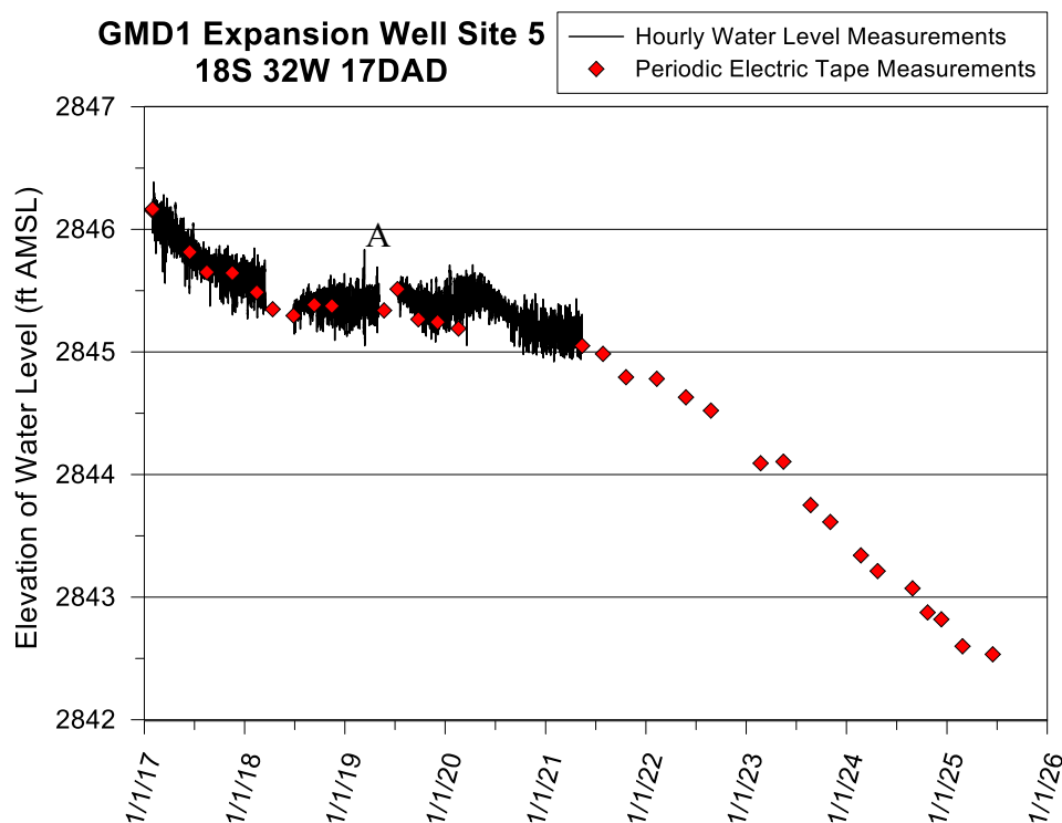
Figure 49—GMD1 Expansion Site 5 well hydrograph—total data run to 6/16/25. A water-level elevation of 2,845 ft corresponds to a depth to water of 131 ft below lsf. Elevation of well bottom is not known. A defined in text.
