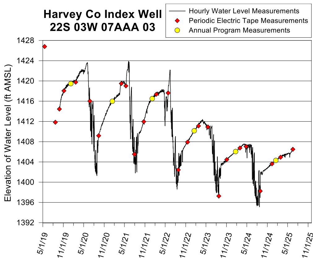
Figure 10—Harvey County index well hydrograph—total data run to 6/17/25. A water-level elevation of 1,408 ft corresponds to a depth to water of 47 ft below lsf. The top of the 10 ft screen is 198 ft below lsf (elevation of 1,257 ft), and the bottom of the aquifer is 206 ft below lsf (elevation of 1,249 ft). The in-field calibration approach described in Butler, Knobbe et al. (2021) has been applied to the transducer data to correct for sensor drift.
