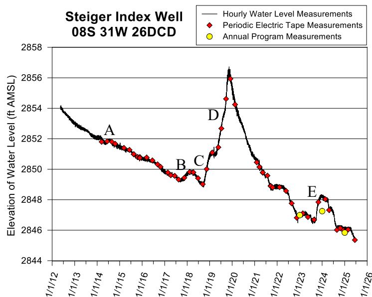
Figure 34—Steiger index well hydrograph—total data run to 6/15/25. A water-level elevation of 2,848 ft corresponds to a depth to water of 117 ft below Isf. The top of the 40 ft screen is 145 ft below Isf (elevation of 2,820 ft), and the bottom of the aquifer is 177 ft below Isf (elevation of 2,788 ft). A–E defined in text. Measurements affected by datalogger overheating (mid-summer 2015 and earlier) are not displayed.
