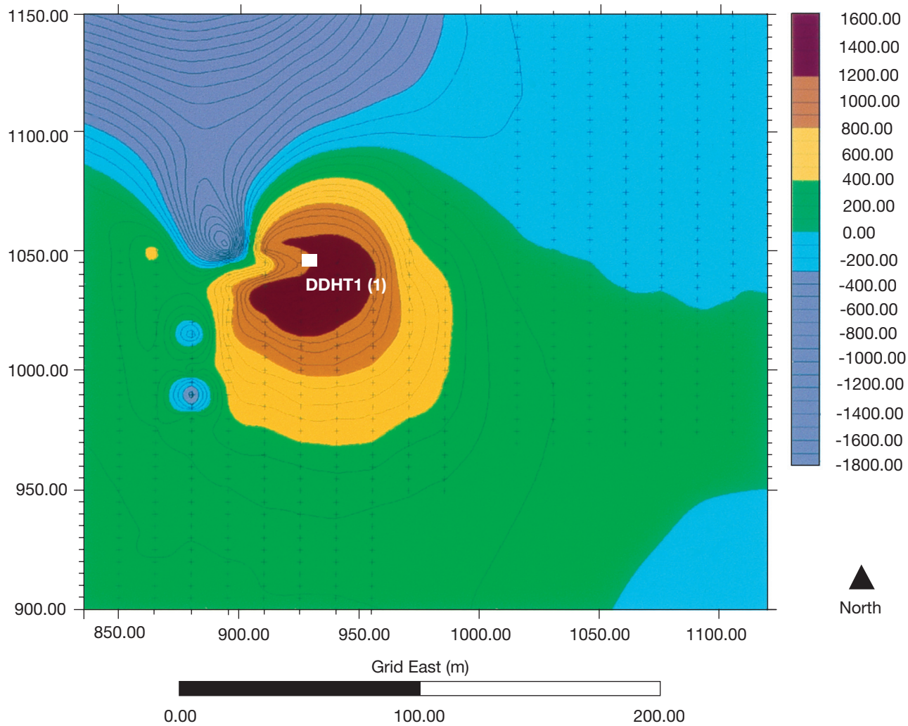
FIGURE 13—Tuttle ground magnetic anomaly, Riley County, Kansas.
