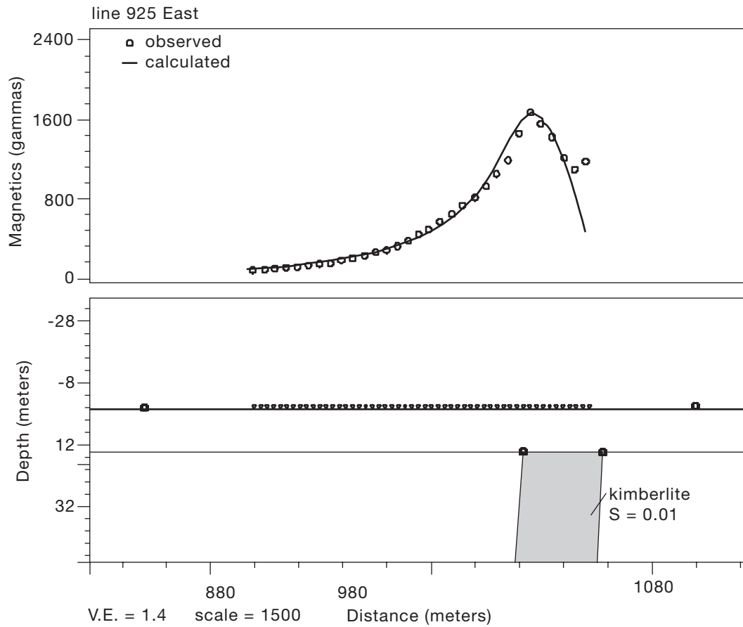
FIGURE 15—2.5-dimensional magnetic model of the Tuttle kimberlite.
