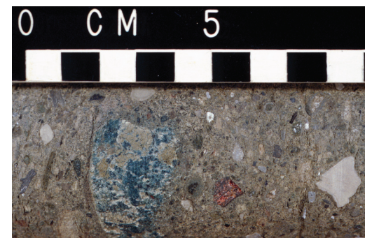
FIGURE 20—Baldwin Creek kimberlite at 230 ft. Many xenoliths, garnet, and chrome diopside.
