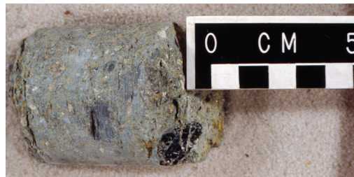
FIGURE 21—Tuttle kimberlite at 209 ft, showing phlogopite books.
