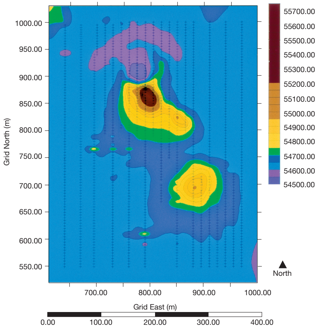
FIGURE 6—Antioch ground magnetic anomaly, Marshall County, Kansas.
