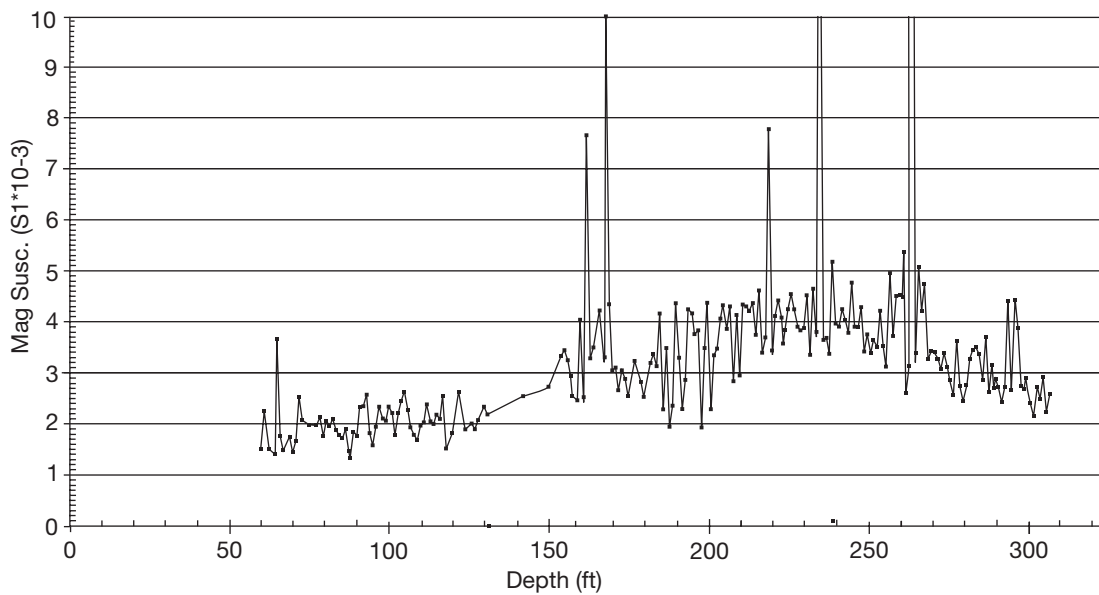
FIGURE 14—Tuttle Magnetic susceptibility plot.
