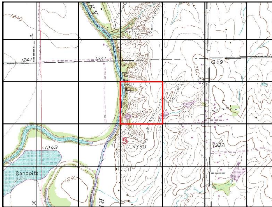
Figure 27. MODFLOW Model Cells. The cell outlined in red shows an example where the bedrock elevation was modified to be at least 10 feet below the streambed.
