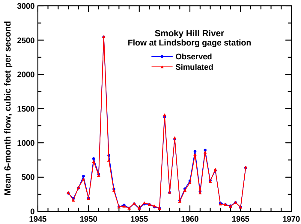
Figure 65. Calibrated Streamflow at Lindsborg
