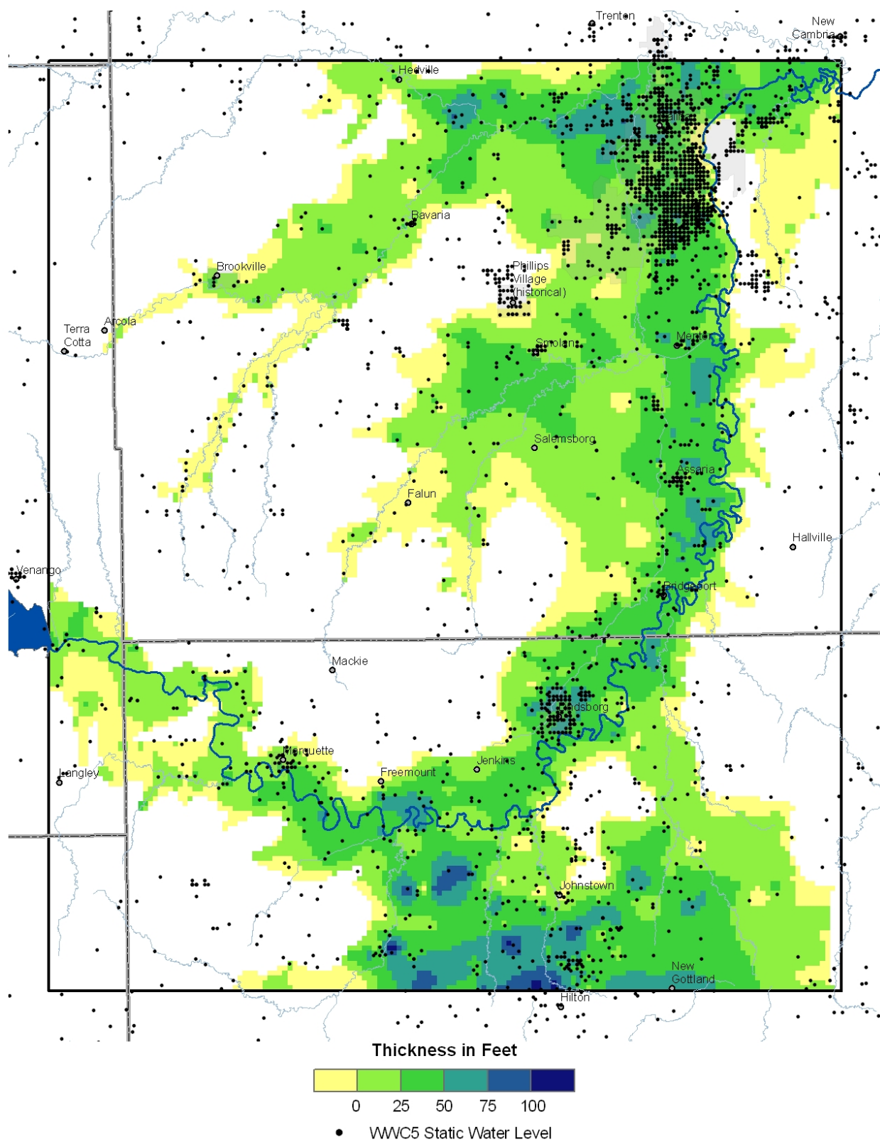
Figure 19. Interpolated WWC-5 static water level saturated thickness.
