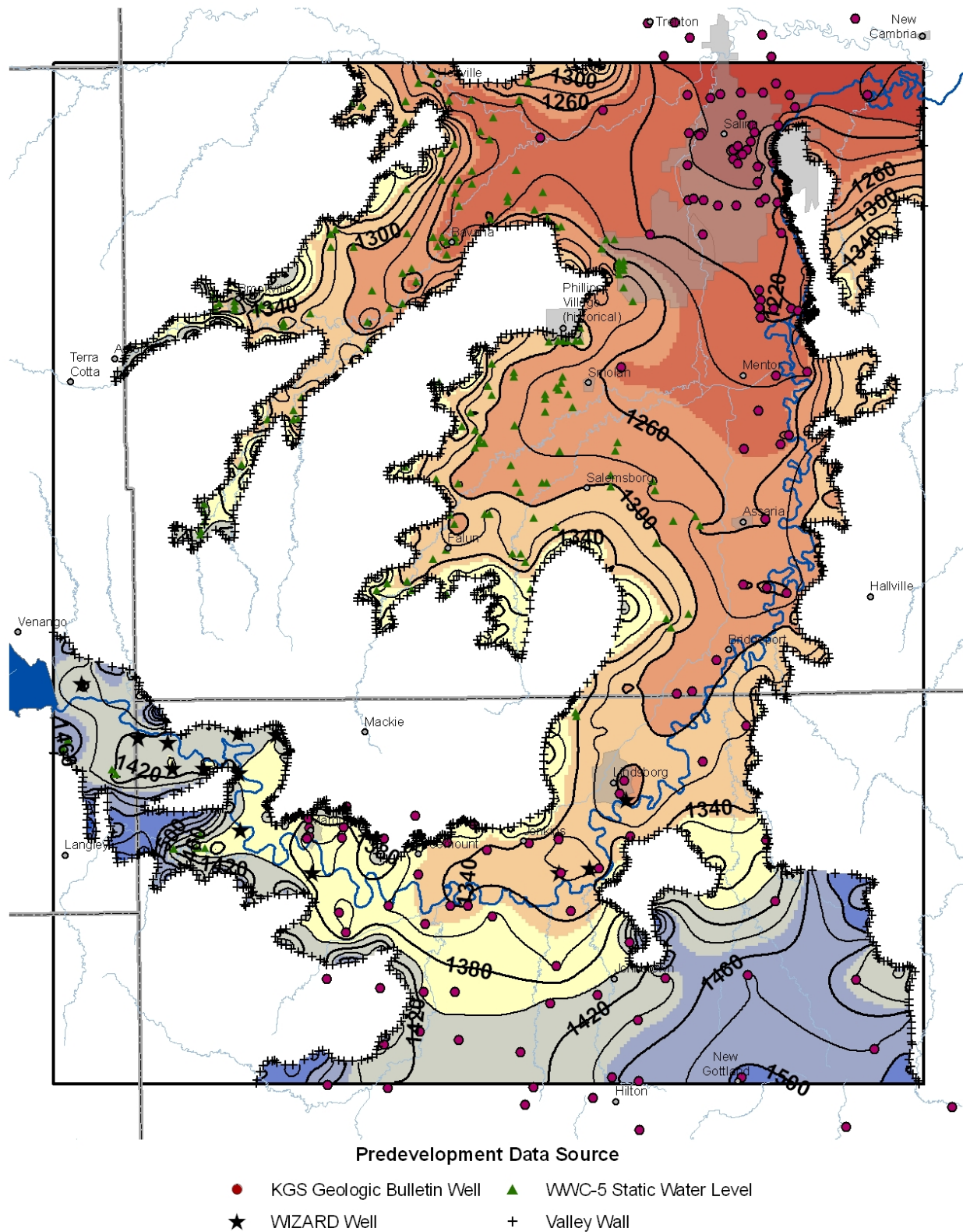
Figure 20. Interpolated predevelopment water table elevation.
