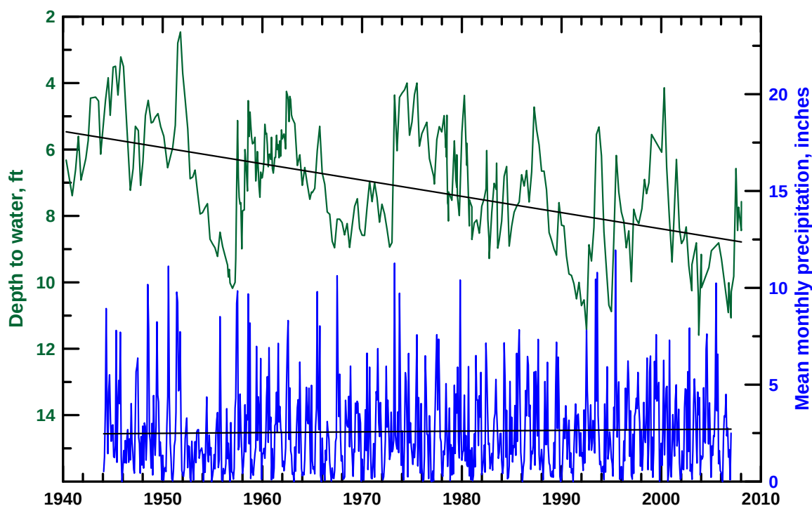
Figure 23. Water-level data for the Equus Beds monitoring well used a proxy for estimating the differences between winter and summer recharge.
