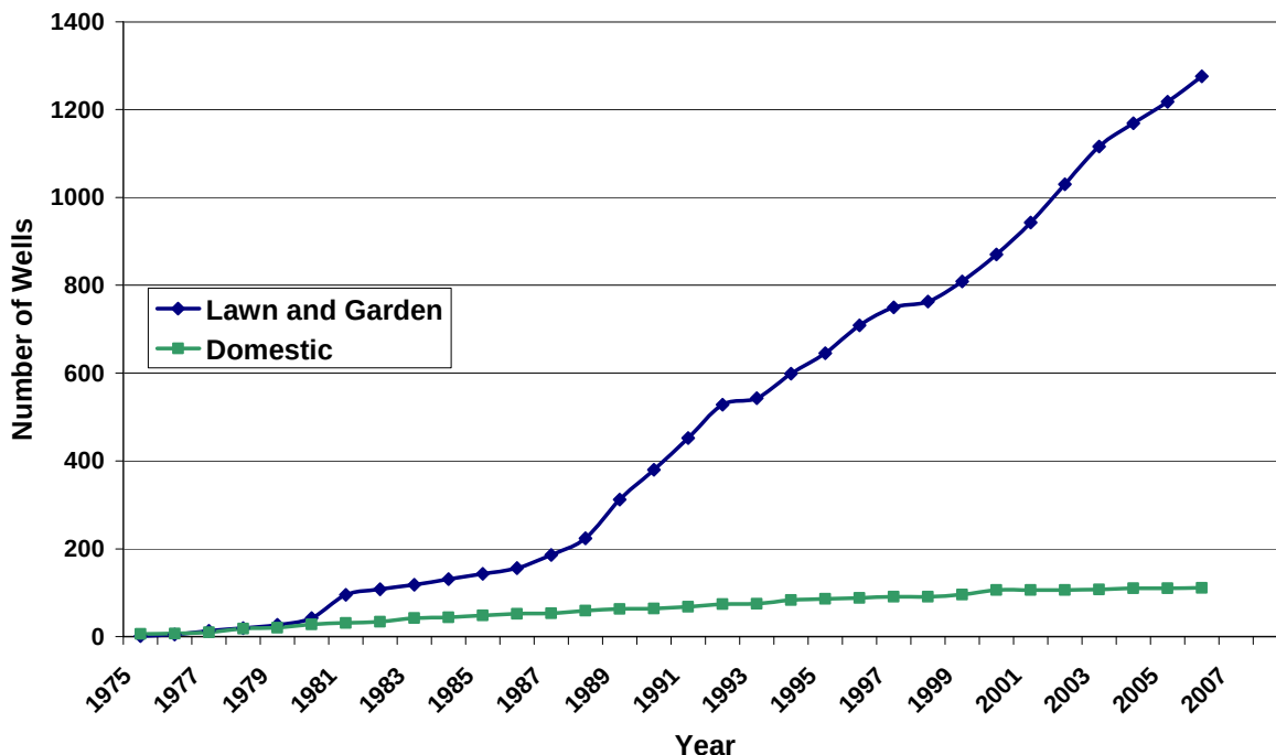
Figure 62. Private domestic and lawn/garden ground-water well development in and around Salina
