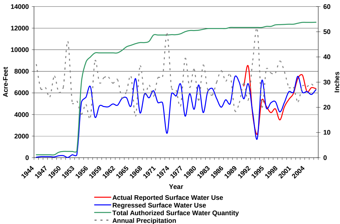
Figure 41. Regressed versus actual reported surface-water use.
