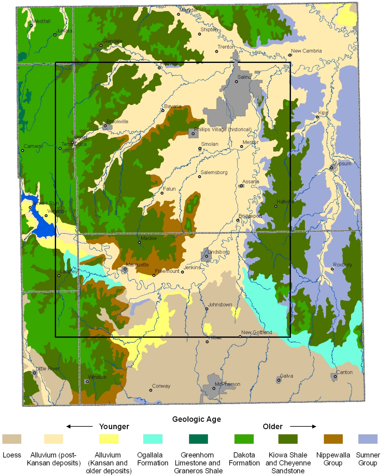
Figure 7. Surficial geology of the study area.
