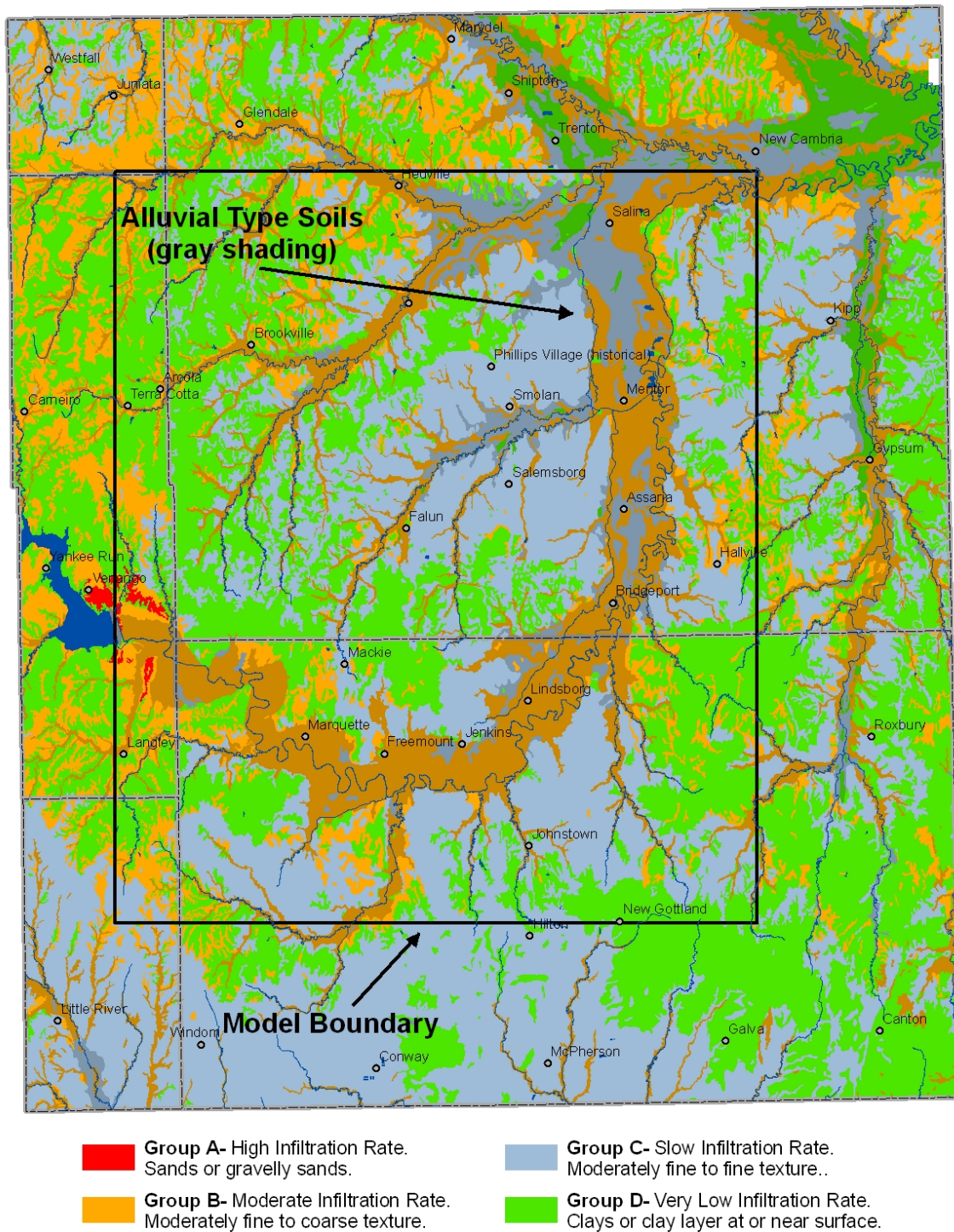
Figure 3. The four hydrologic soil groups and the alluvial type geomorphologic soils in the model region. The gray shading for the alluvial type soils is partially transparent and darkens the colors of the four soil groups where they overlap.
