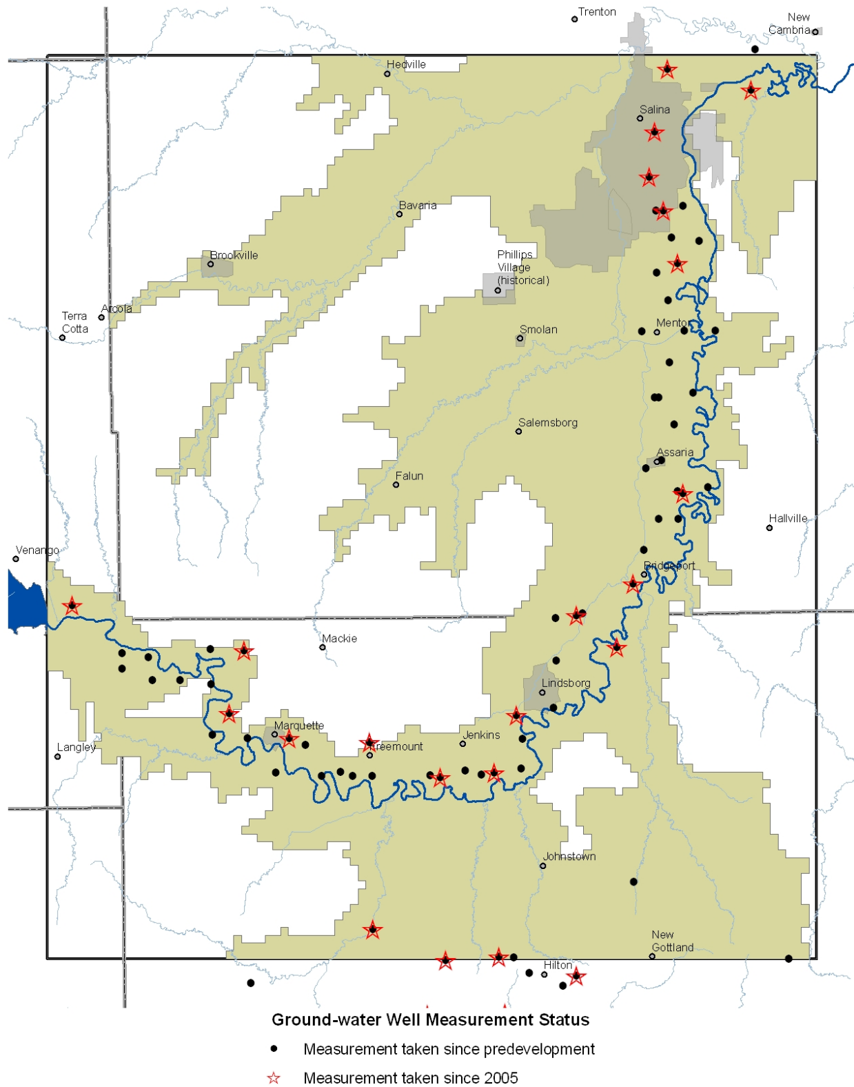
Figure 18. Spatial distribution of ground-water monitoring wells.
