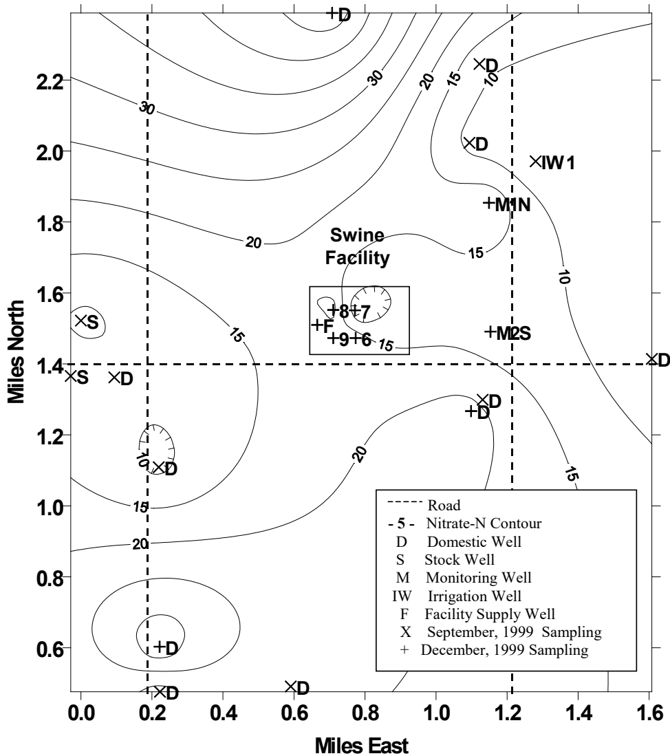
Figure 5. Contour map of nitrate-N concentration from KDHE sampling in September 1999 and KGS/KDHE sampling in December 1999. Note the general high nitrate-N throughout the area. Lower nitrate-N at monitoring well #7 (4.8 mg/L) indicated by hachure marks.
