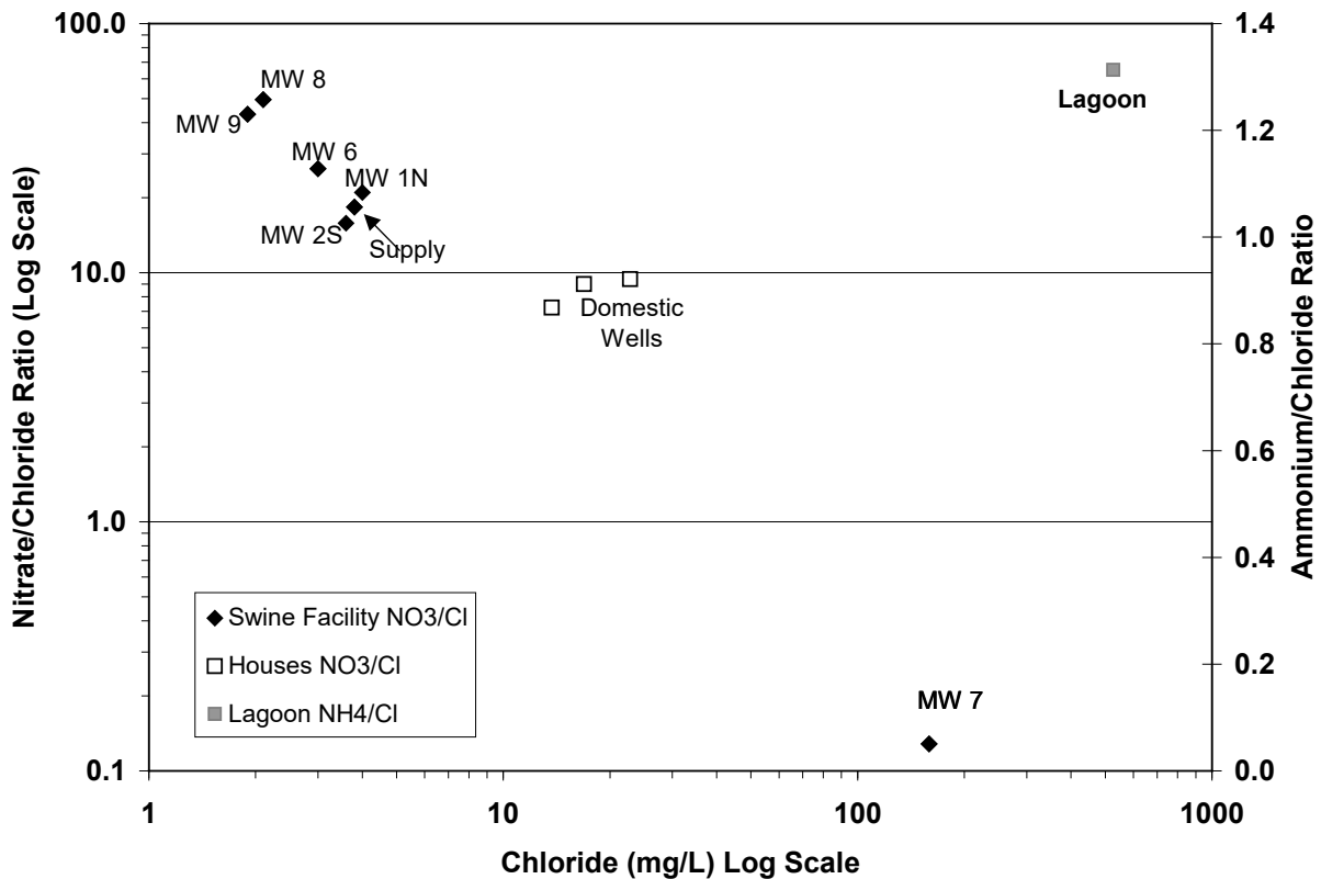
Figure 8. Nitrate/chloride and ammonium/chloride ratios for December 1999 sampling at swine facility. Monitoring well #7 and the domestic well samples show very different ratios than the other monitoring wells and the supply well.
