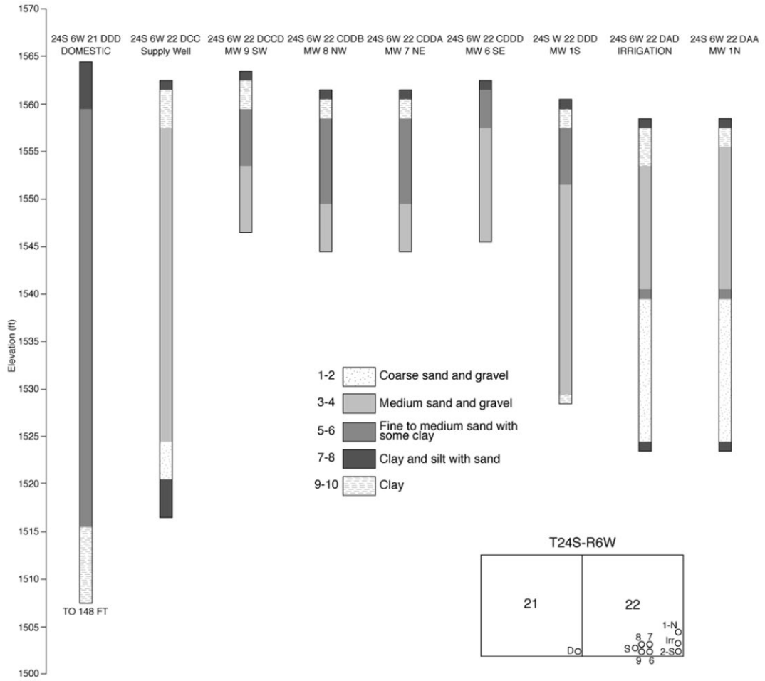
Figure 2. Cross section of wells in T24S-R6W-Sec 22. Note variation in thickness of clay and clay silt zones in upper portions of section. Circles represent locations of wells.
