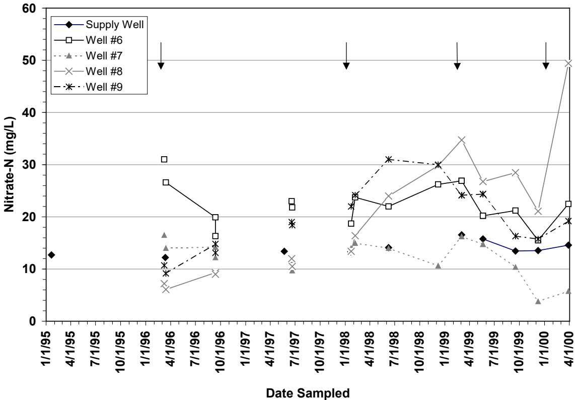
Figure 6. Graph of variation of nitrate-N concentration with time. Arrows indicate probable periods of fertilizer application. Note general increase in nitrate concentration during spring as indicated by arrows.
