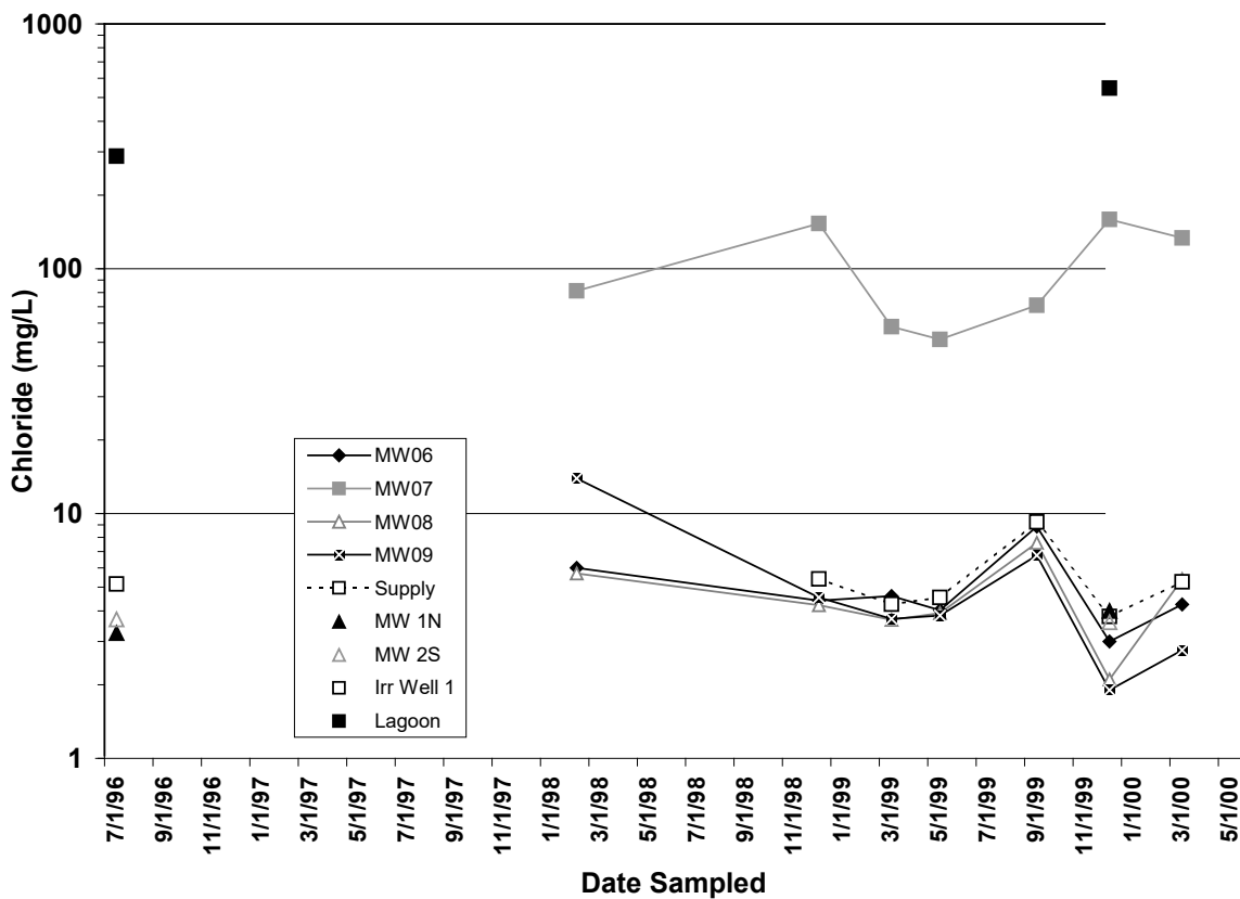
Figure 7. Chloride concentration for wells near swine facility plus waste lagoon. Note similarity of chloride concentration from all monitoring wells except well #7. Well #7 has concentrations between that of the lagoon and the regional water chemistry, indicating probable mixing of waters.
