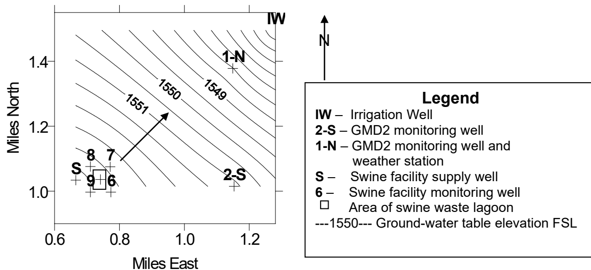
Figure 4. Ground-water elevation and flow direction (shown by arrow in figure) in the vicinity of swine facility in Reno County.
