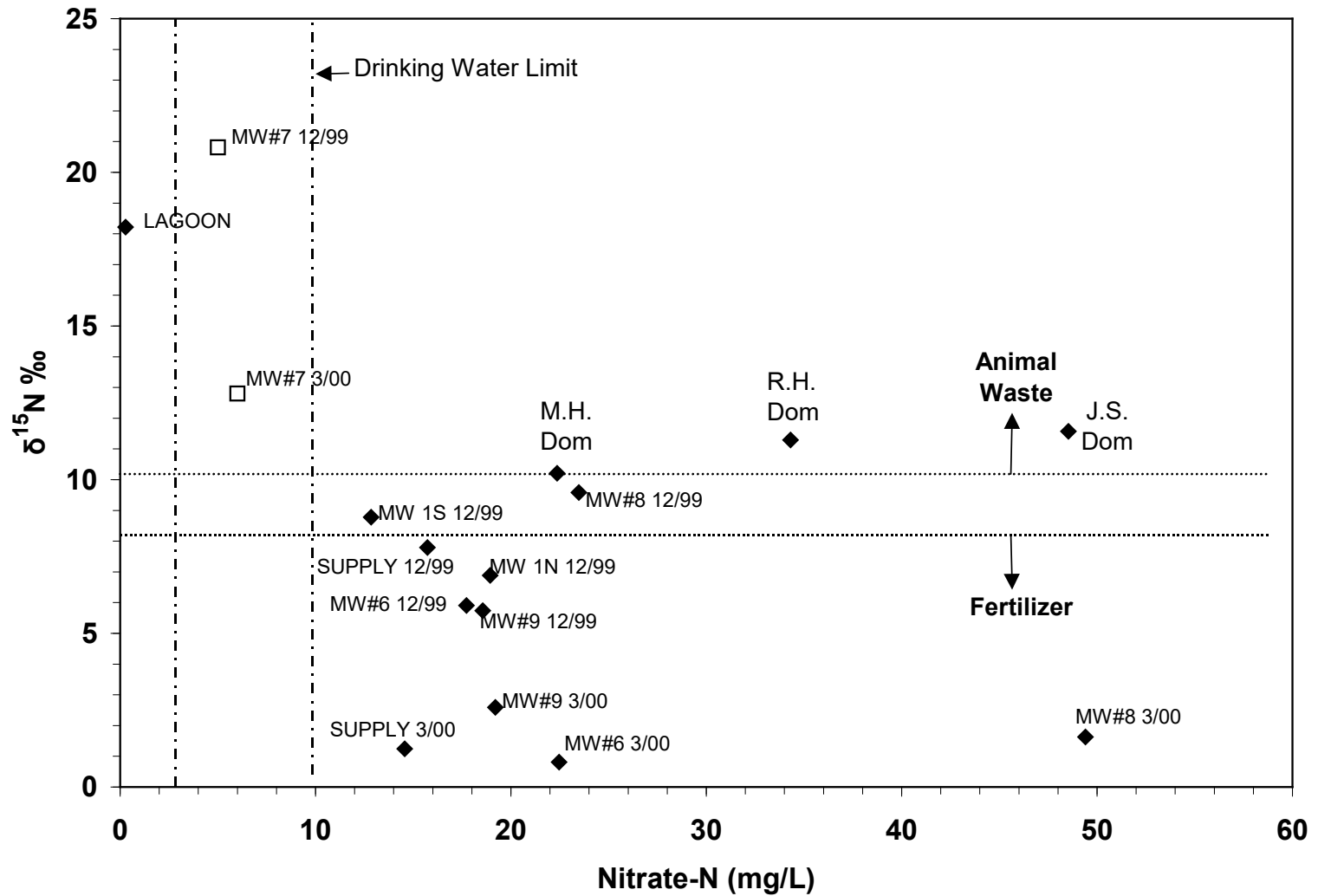
Figure 11. Nitrogen-15 and nitrate-N values for wells at swine facility and surrounding domestic wells. Samples collected in December, 1999 and March 2000.
