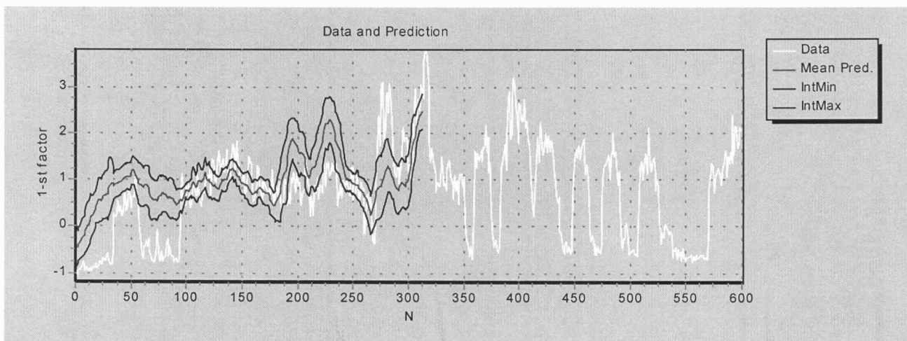
Fig. 8. Distribution of first principal component for the period 10-40 kyr BP and prediction for the period 10-25 kyr BP. Increments on horizontal axis are 50-years steps.
