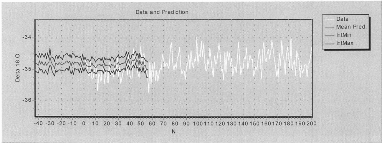
Fig. 9. Distribution of \delta^{18}\text{O} for the period 0-4 kyr BP and prediction for the period 1140 years BP to 2800 AD. Increments on horizontal axis are 20-years steps. 0 corresponds to the present time.
