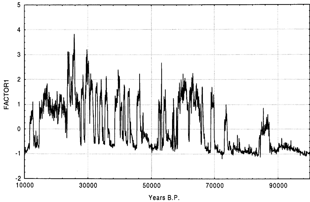
Fig. 3. Distribution of first principal component of chemical constituents from GISP2 ice core for the period of time 10-100 kyr B.P.
