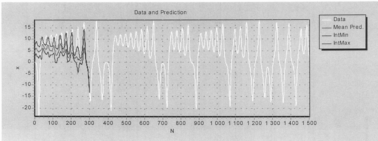
Fig. 7. Prediction for trace of Lorenz system: white curve – x -coordinate of the Lorenz system (discrete time is on horizontal axis, \delta t = 0.25 ), black curves represent average prediction and 99% confidence interval. M = 3 , L = 1 , k = 25 .
