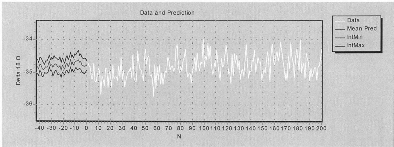
Fig. 10. Distribution of \delta^{18}\text{O} for the period 0-4 kyr BP and prediction for 800 years into the future. Increments on horizontal axis are 20-years steps. 0 corresponds to the present time.
