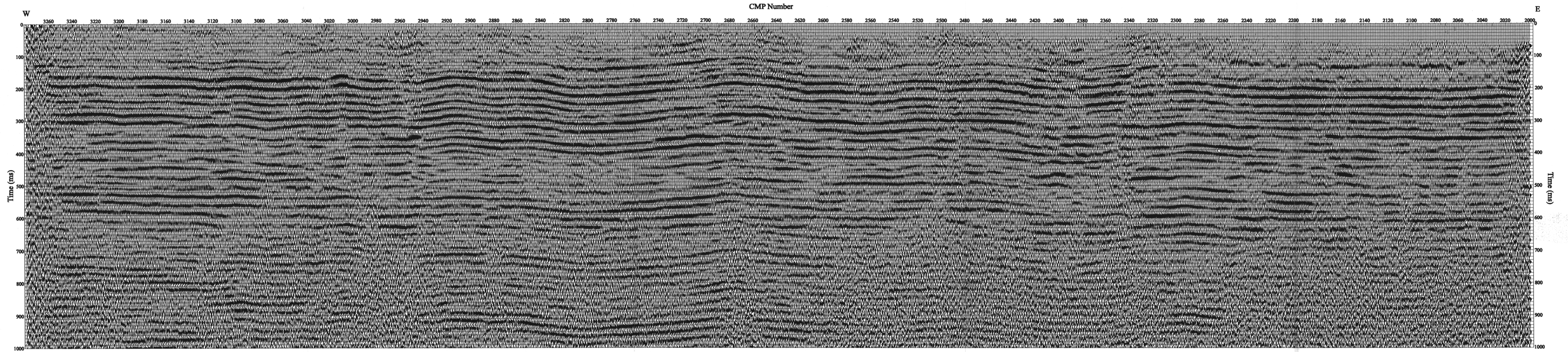
Plate A. Uninterpreted seismic data from Wabaunsee County, Kansas.
