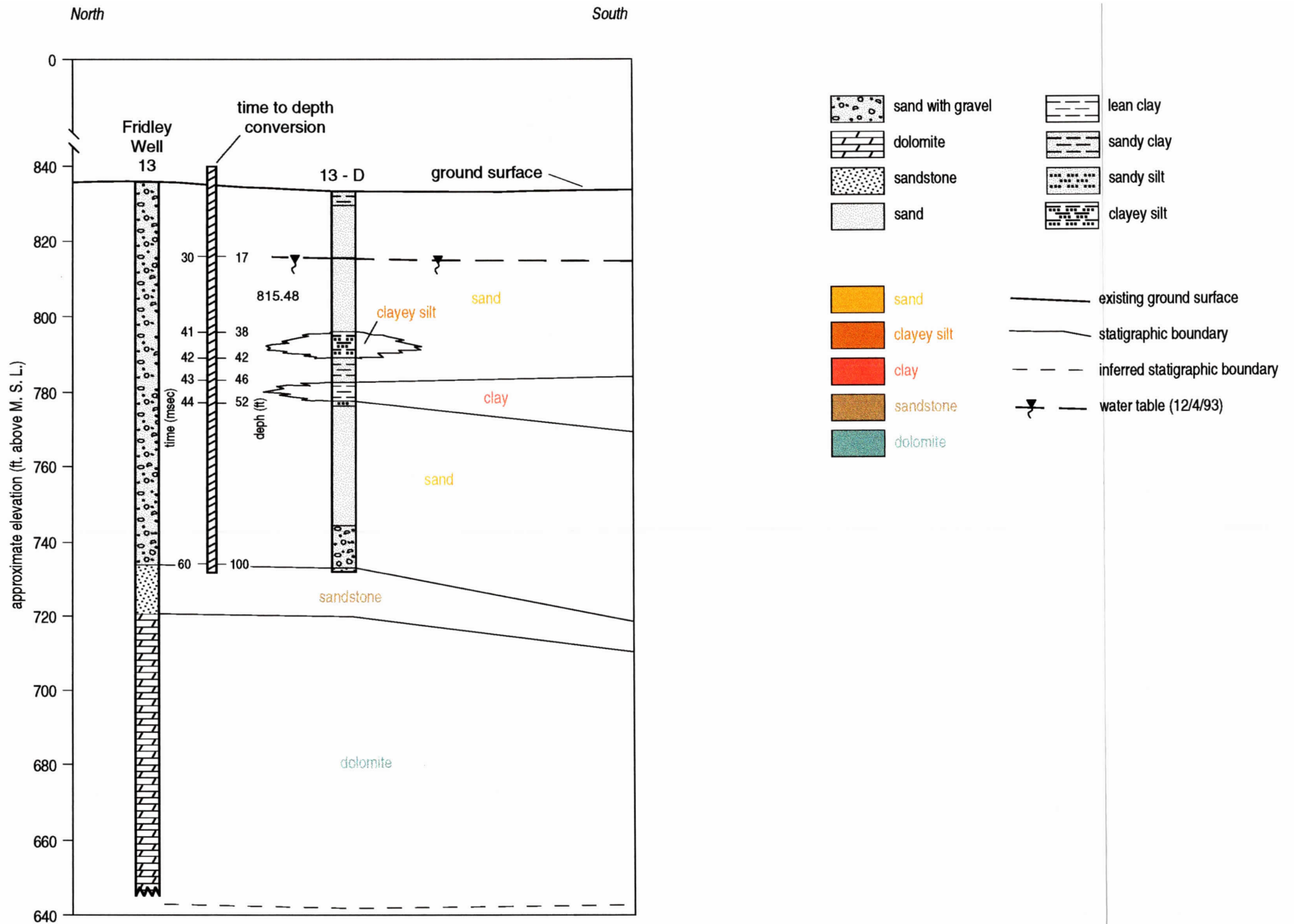
Figure 4. Two-way time-to-depth correlations from uphole survey and borehole-interpreted geology.
