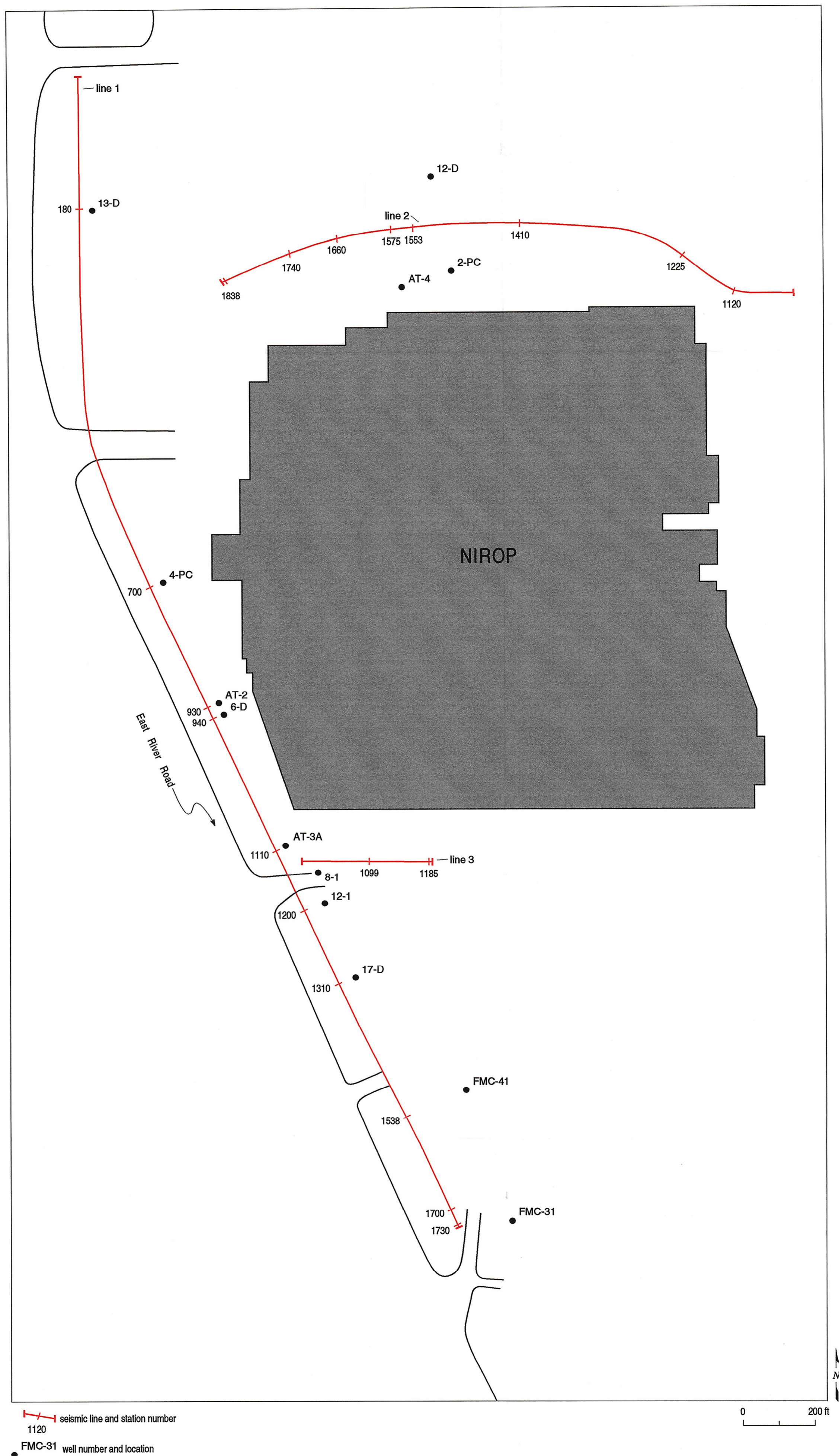
Figure 8. Detailed site map of U.S. Navy Northern Ordnance Plant, Fridley, Minnesota, showing approximate station numbers of CDP profiles relative to the facility and nearby wells.
