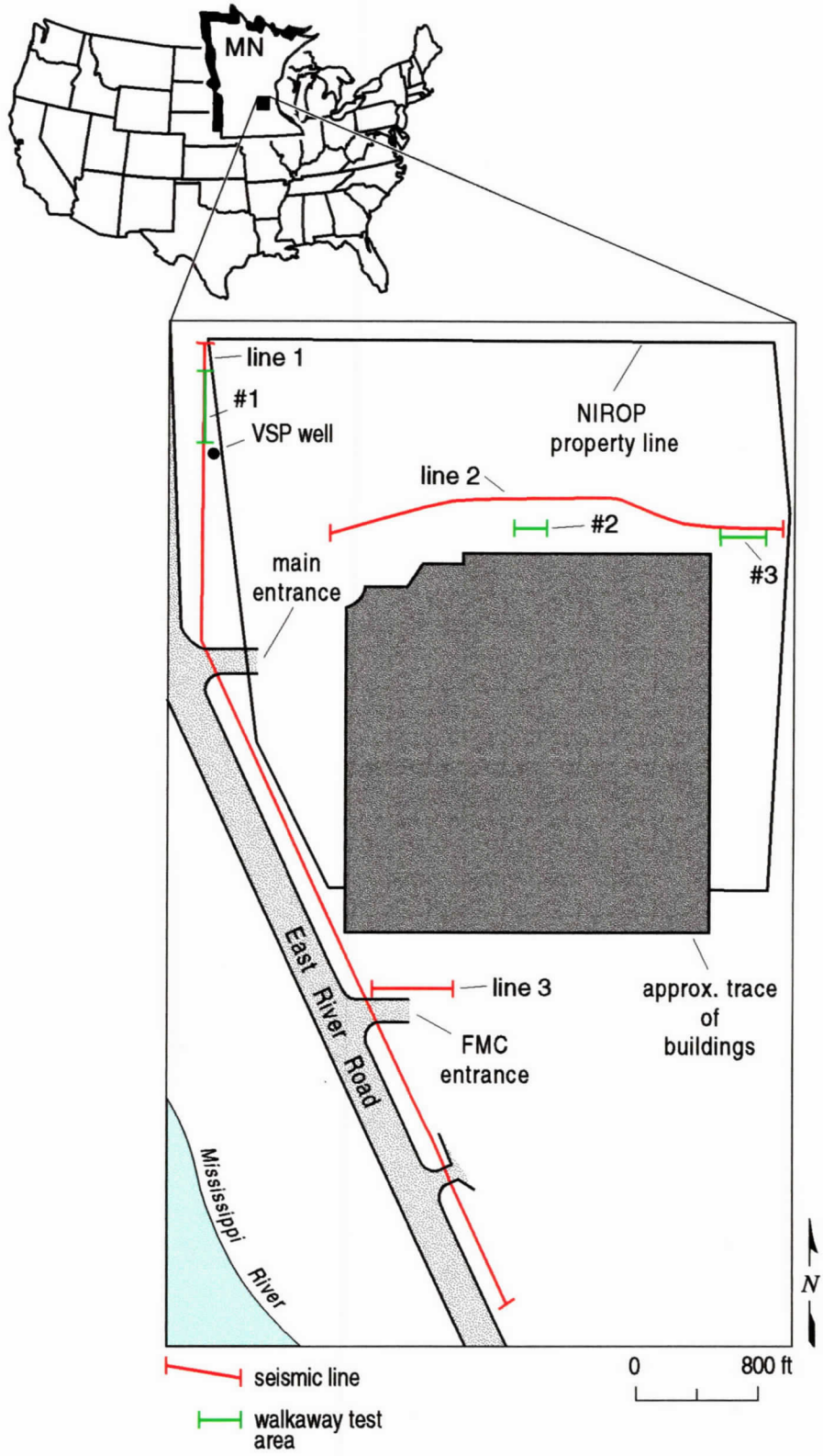
Figure 1. Generalized site map of U.S. Navy Northern Ordnance Plant, Fridley, Minnesota, showing seismic lines 1, 2, and 3, walkaway test lines, and VSP well.
