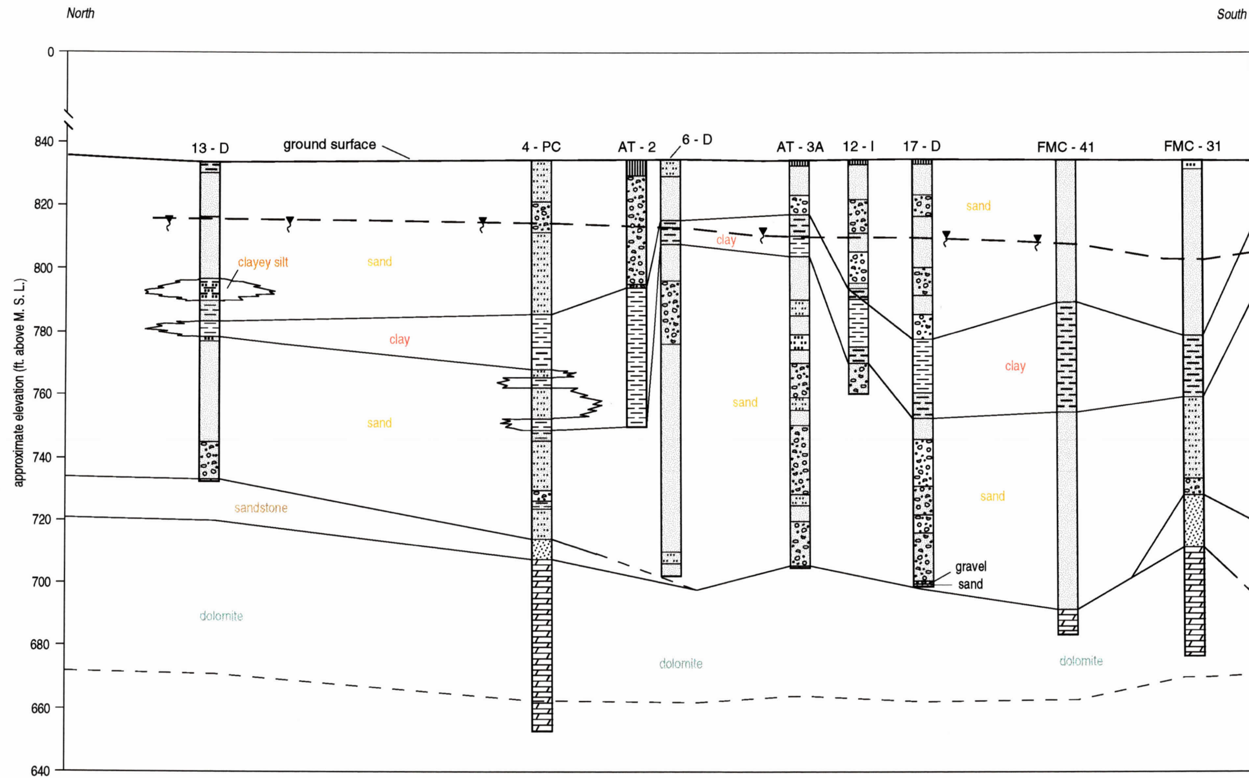
Figure 2. Geologic cross-section derived from drill data near the East River Road and approximately parallel to seismic line 1 (modified from cross-section generated by RMI Inc., 1995).
