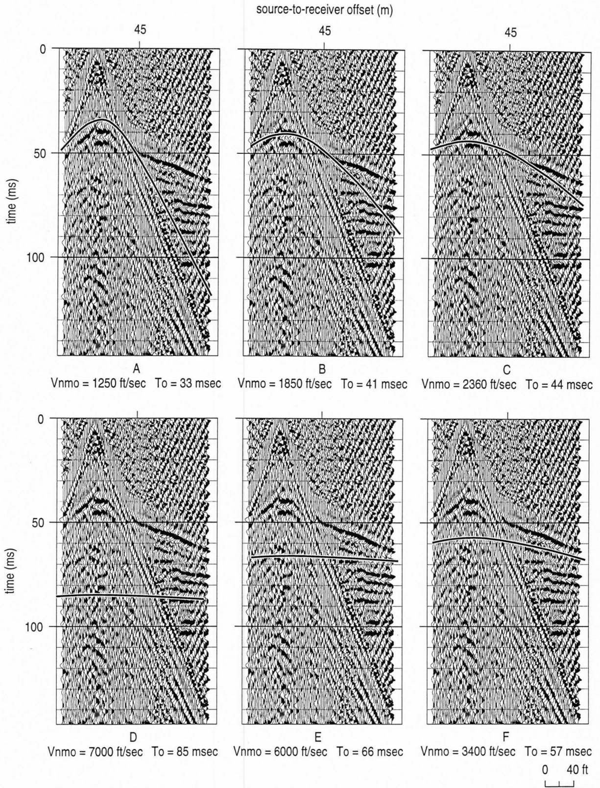
Figure 6. Selected shot gathers with six different normal moveout velocity curves overlaying the filtered data. Indicated velocities and curves selected based on uphole velocity survey.
