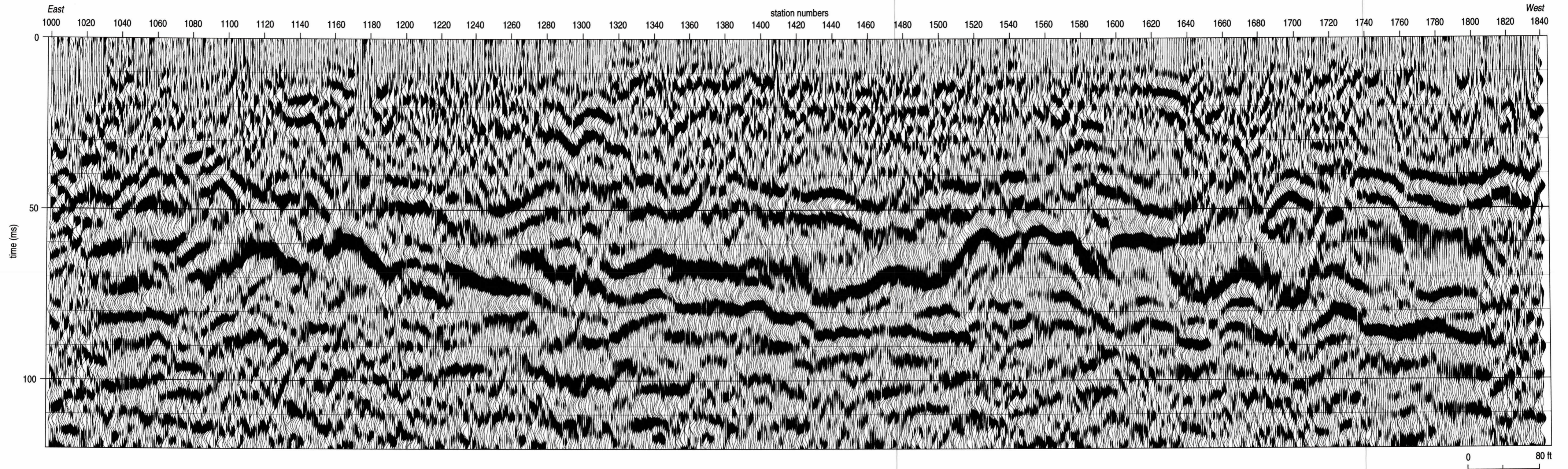
Figure 15. CDP stacked section of line 2, North 40 area. Stacked data quality is not as high on line 2 as line 1, likely due to the poorer near-surface conditions on line 2 in comparison to line 1.
