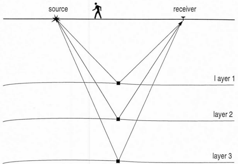
Figure B2. Reflection from three subsurface layers. The angle of incidence is different for each layer/ray but the reflecting points are vertically equivalent.
