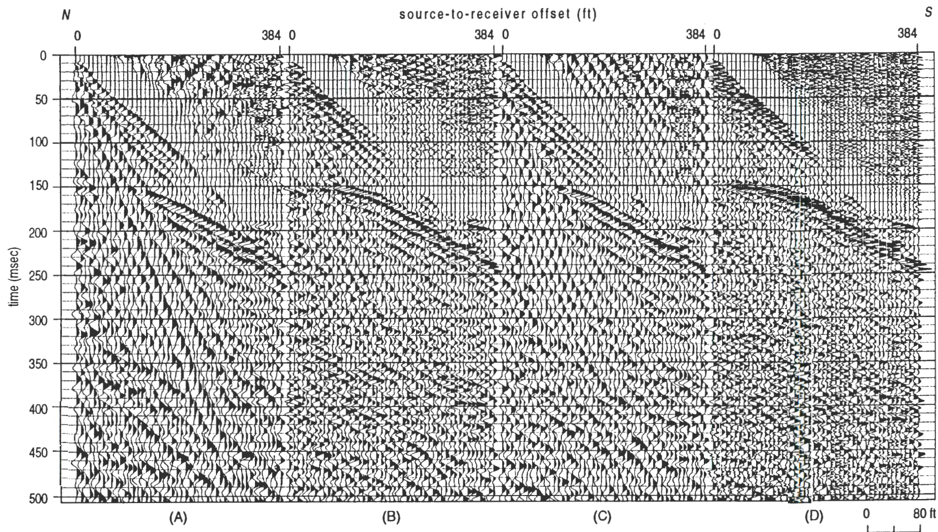
Figure 2. Walkaway noise tests conducted along the northeastern end of line 1. The four files were acquired with the same geophones and source location but different analog low-cut filters (a) out, (b) 100 Hz, (c) 50 Hz, and (d) 200 Hz. The prominent 145 msec reflection possesses textbook curvature and a dominant frequency of over 150 Hz on the 100 Hz low-cut file. Vertical resolution potential is less than 3 ft.
