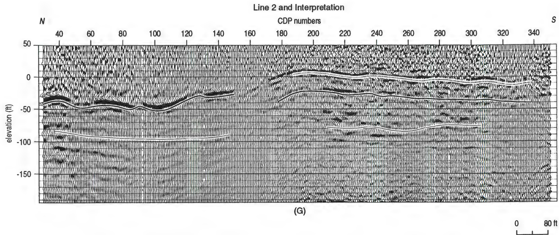
Figure 7A-G. Line 2, 24-fold, CDP stacked section. A) Elevation corrected to multiple sloping datums. B) Same CDP data as (A) elevation corrected to a single flat 48 ft sea level datum. C) Deconvolved (B). D) F-k migrated (C). E) Depth converted (D) using the stacking velocities. F) Interpreted (E) assuming the shallowest reflection is from the same reflector across the line. G) Interpretation of (E) if the shallowest reflection is discontinuous at the apparent offset.
