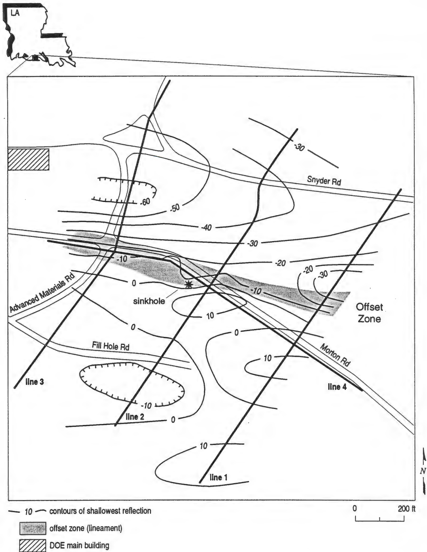
Figure 10. Linear projection of apparent offset and wavelet change on seismic lines 1, 2, 3, and 4. The lineament intersects the sinkhole and the steep sided ditch on line 1. Based on projections from mine maps, the lineament is consistent with the mine face of both the upper and lower cavities. Control points for the shallowest reflection contours are directly extracted from seismic sections 6F through 9F.
