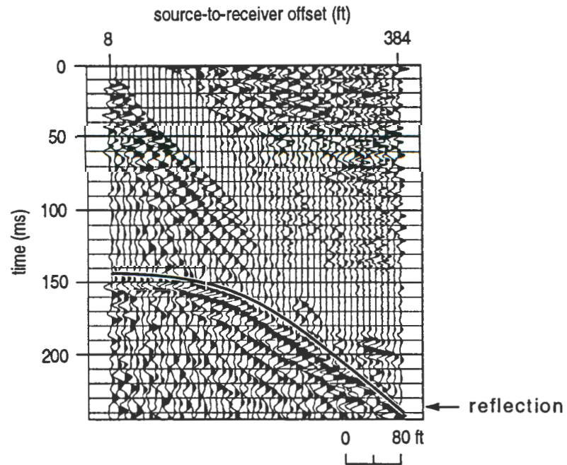
Figure 3. A computer simulated, 2100 ft/sec reflection hyperbola is displayed over field file (b) from the walkaway noise test (Figure 2). The theoretical curve is a perfect match. Depth conversion indicates the reflector is 150 ft deep.
