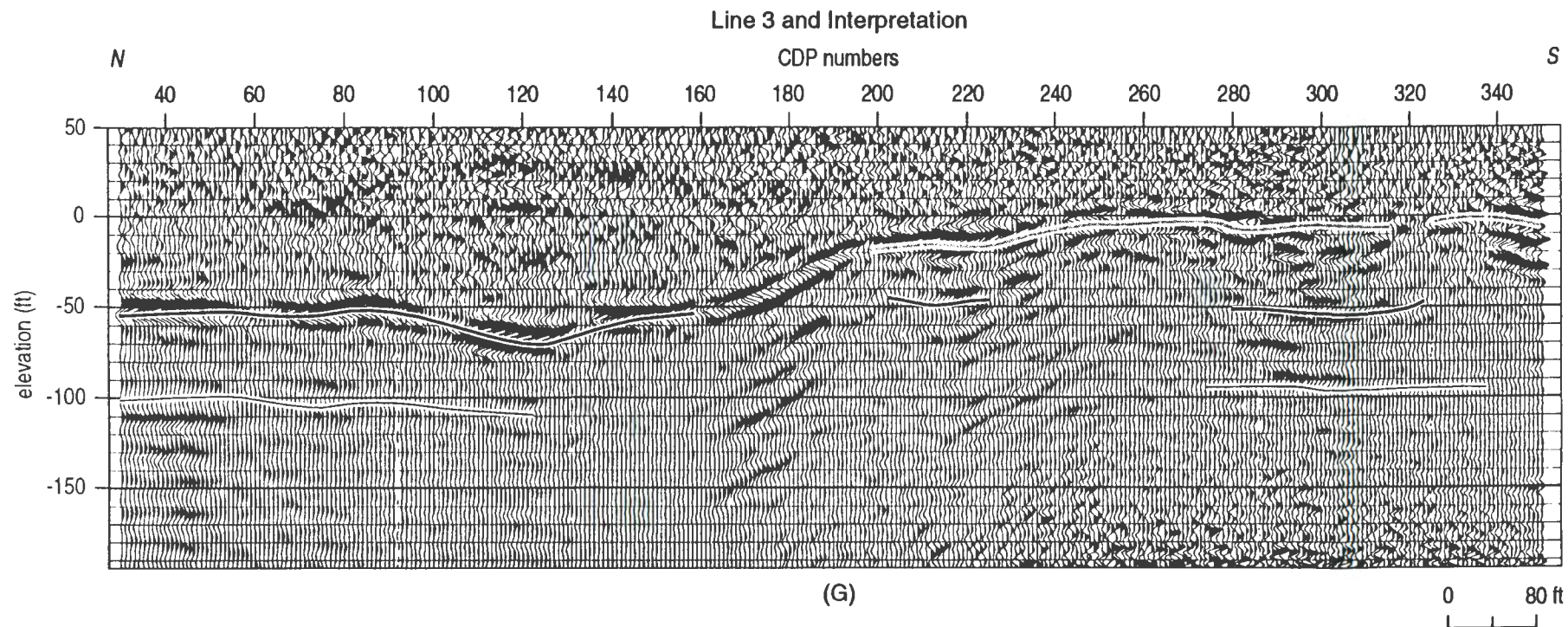
Figure 8A-G. Line 3, 24-fold, CDP stacked section. A) Elevation corrected to multiple sloping datums. B) Same CDP data as (A) elevation corrected to a single flat 48 ft sea level datum. C) Deconvolved (B). D) F-k migrated (C). E) Depth converted (D) using the stacking velocities. F) Interpreted (E) assuming the shallowest reflection is from the same reflector across the line. G) Interpretation of (E) if the shallowest reflection is discontinuous at the apparent offset.
