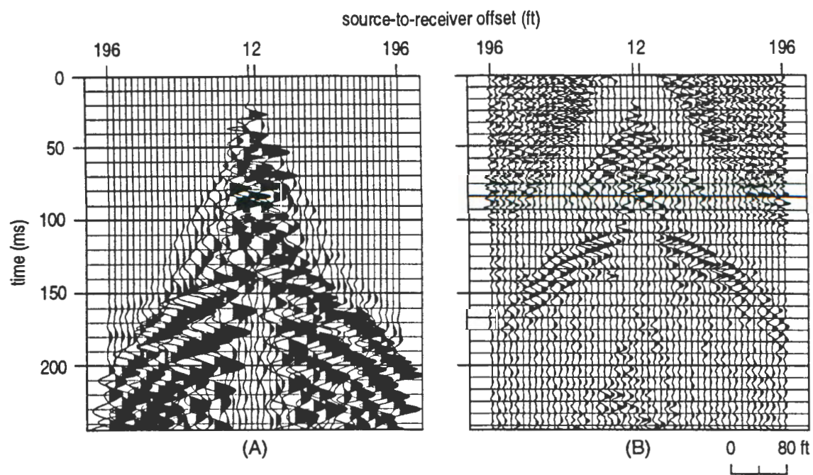
Figure 5. Raw field file (A) and normalized/filtered field file (B) from along line 4. In this split-spread source/receiver geometry the reflection traces a symmetric hyperbola near offset of 12 ft and far offset of 196 ft.
