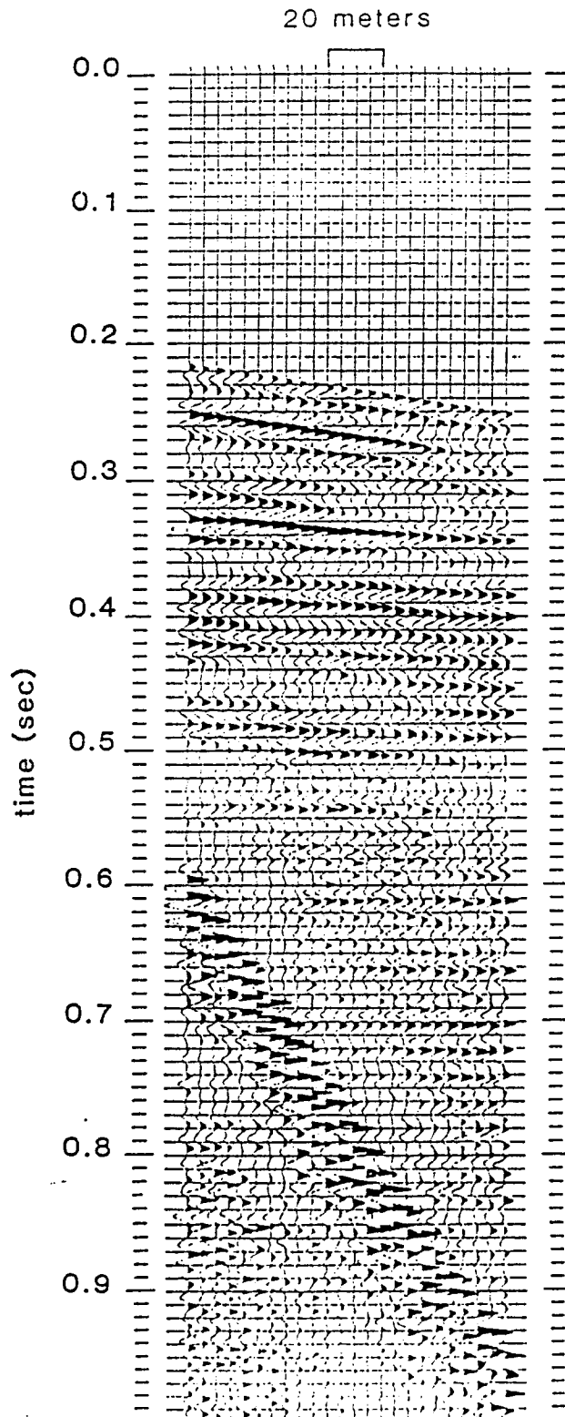
FIG. 4. This stacked field file has 100 Hz reflection energy as deep as 1100 meters.
