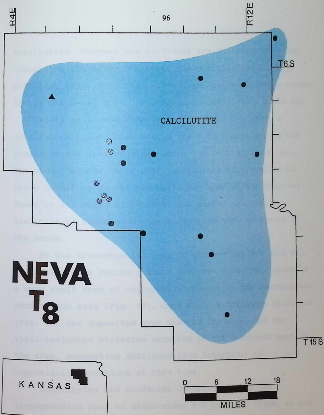
Figure 39. Paleogeographic map of lithofacies at the transgressive apex of NT 8 for the localities where NT 8 is present (for locality identification use overlay in pocket).
