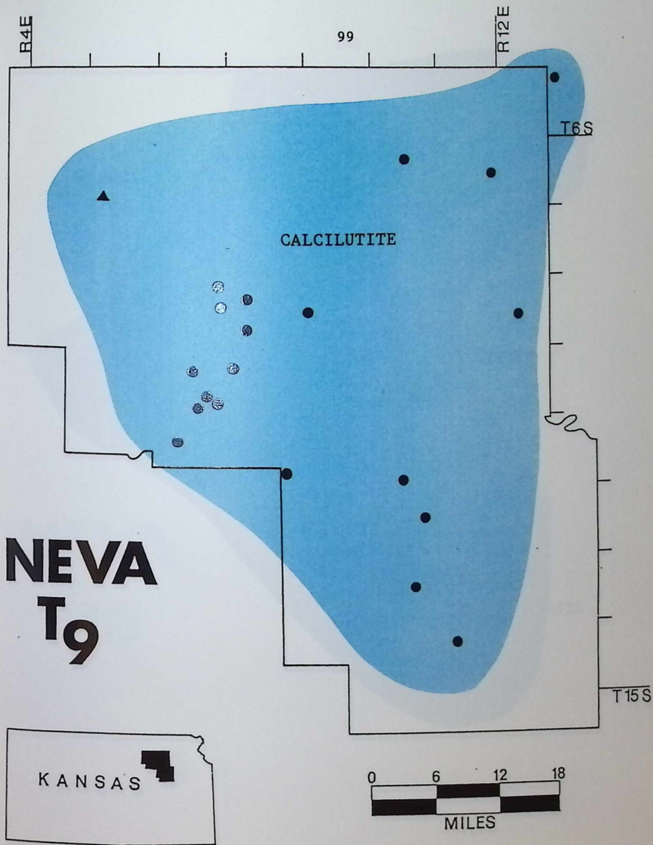
Figure 41. Paleogeographic map of lithofacies at the transgressive apex of NT, for the localities where NT, is present (for locality identification use overlay in pocket).
