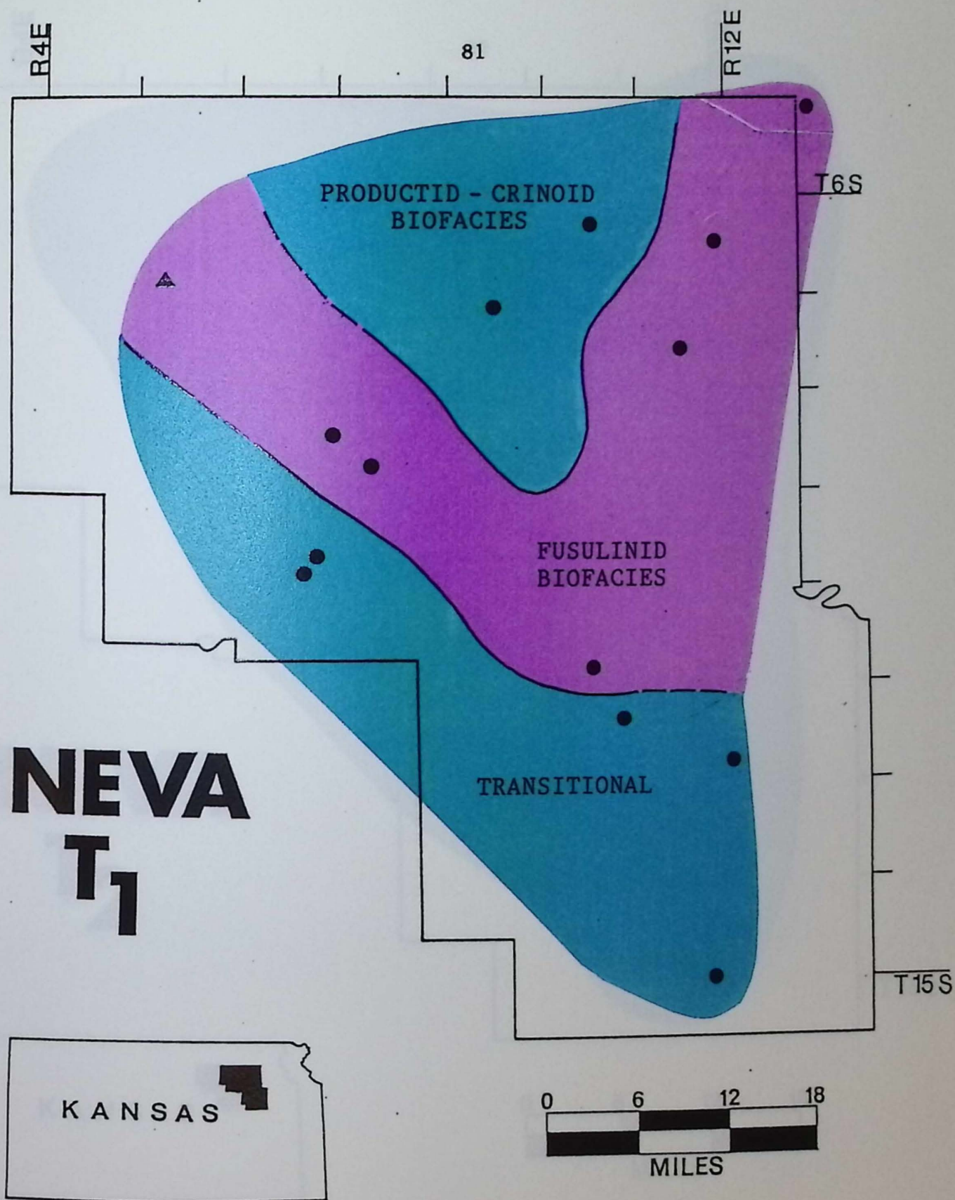
Figure 26. Paleogeographic map of biofacies at the transgressive apex of NT, for the localities where NT, is present (for locality identification use overlay in pocket).
