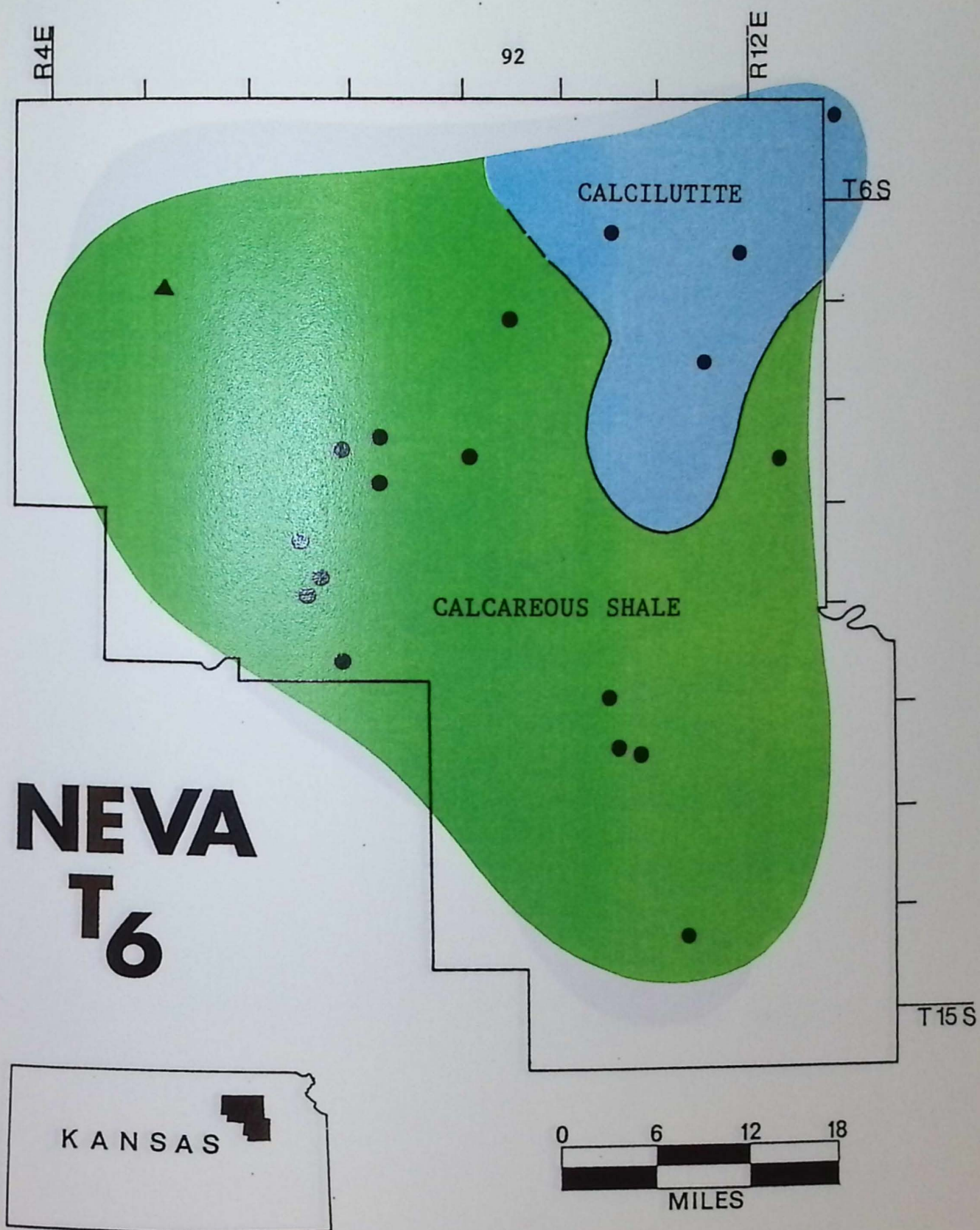
Figure 35. Paleogeographic map of lithofacies at the transgressive apex of NT_6 for the localities where NT_6 is present (for locality identification use overlay in pocket).
