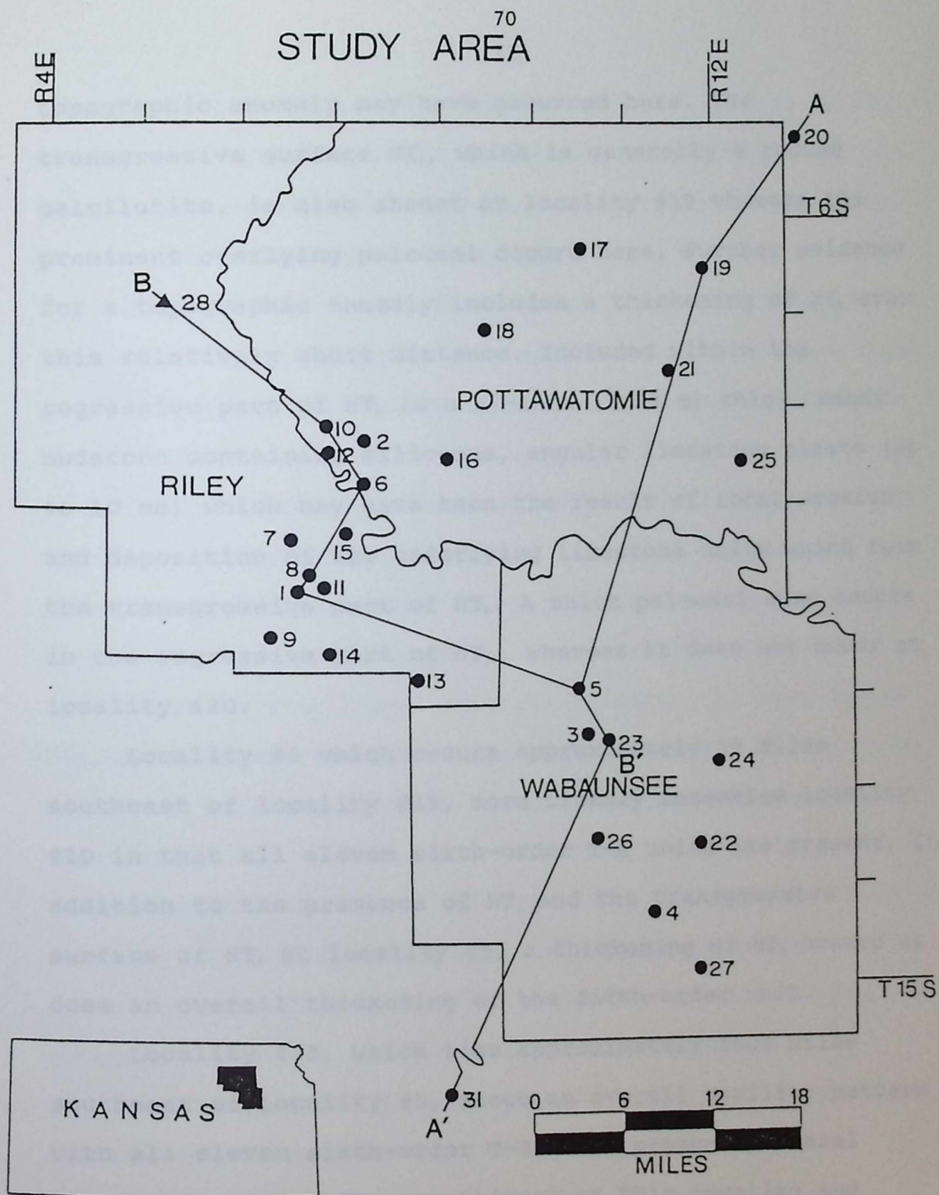
Figure 22. Location map for correlated cross-sections A-A' (localities # 20, 19, 5, 23, and 31), and B-B' (localities # 28, 10, 6, 8, 1, 5, and 23).
