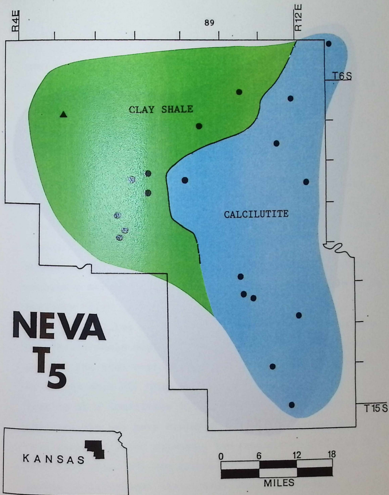
Figure 33. Paleogeographic map of lithofacies at the transgressive apex of NT, for the localities where NT, is present (for locality identification use overlay in pocket; for clay shale read mudstone).
