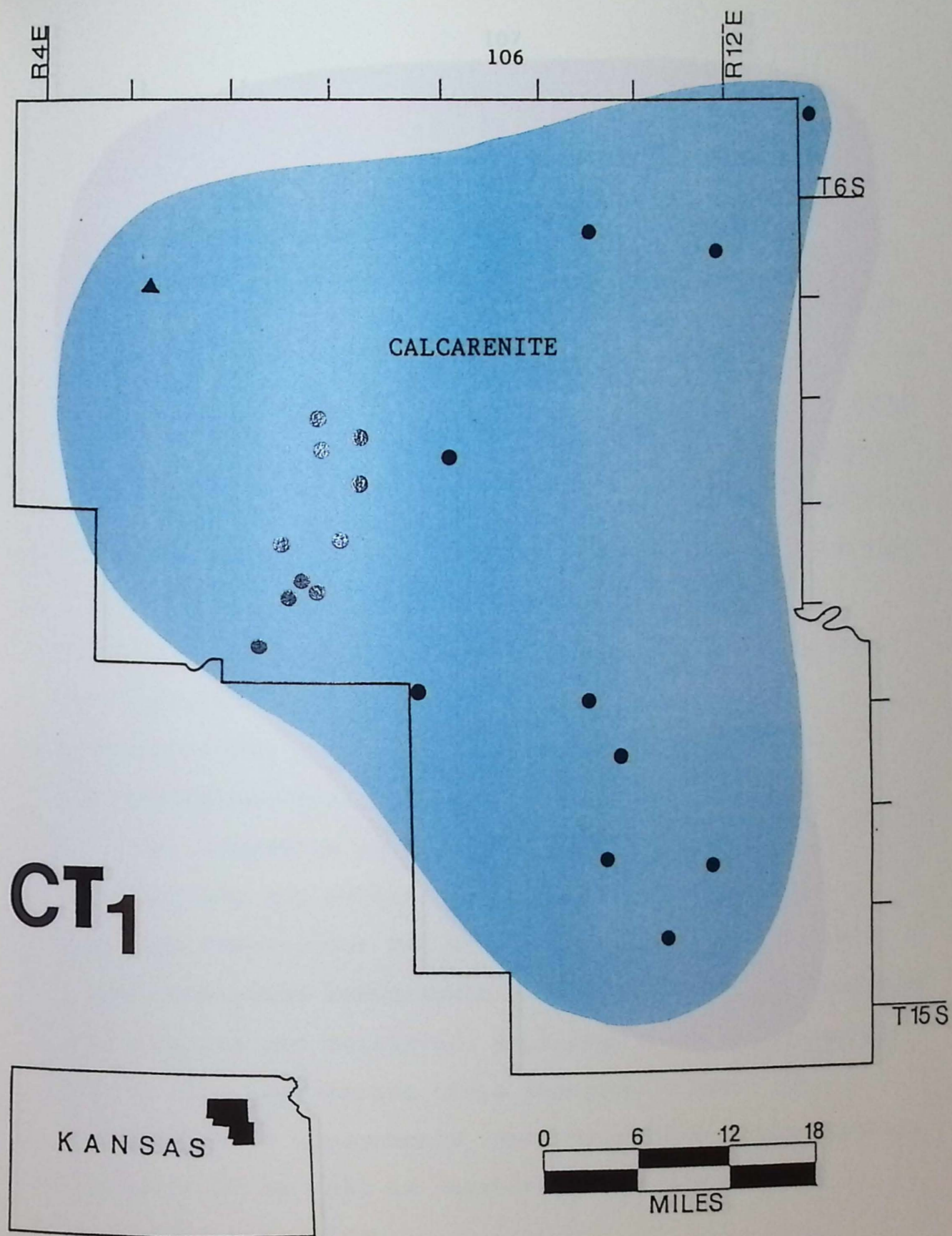
Figure 47. Paleogeographic map of lithofacies at the transgressive surface of CT 1 , for the localities where CT 1 is present (for locality identification use overlay in pocket).
