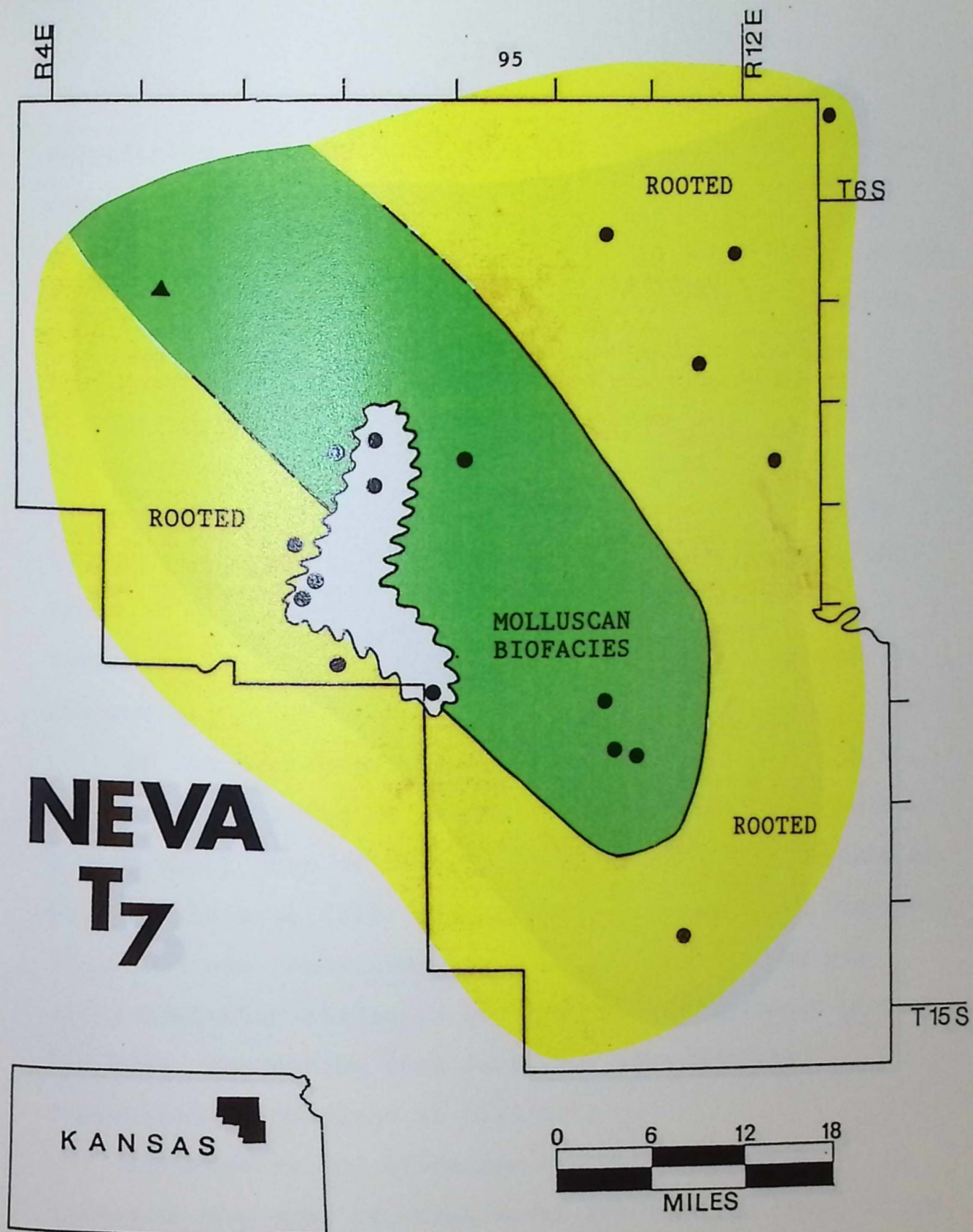
Figure 38. Paleogeographic map of biofacies at the transgressive apex of NT, for the localities where NT, is present (for locality identification use overlay in pocket).
