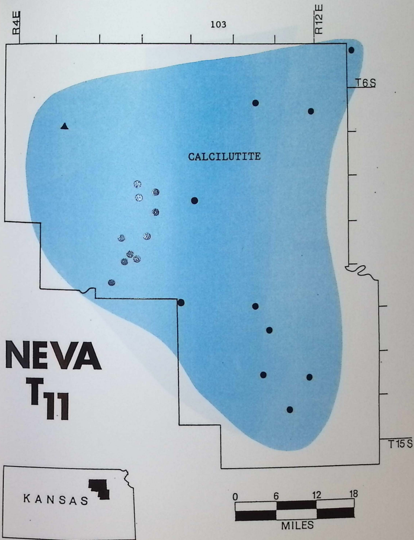
Figure 45. Paleogeographic map of lithofacies at the transgressive apex of NT 11 for the localities where NT 11 is present (for locality identification use overlay in pocket).
