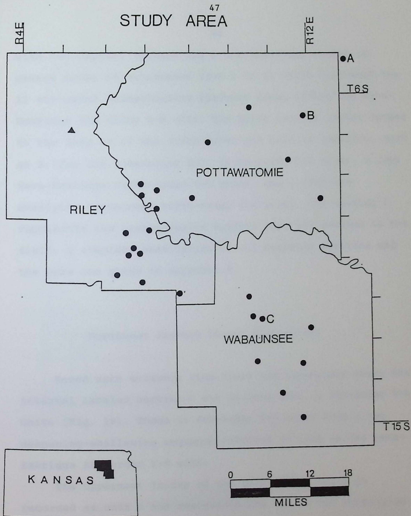
Figure 18. Location map of selected sections A (#20), B (#19), and C (#23).
