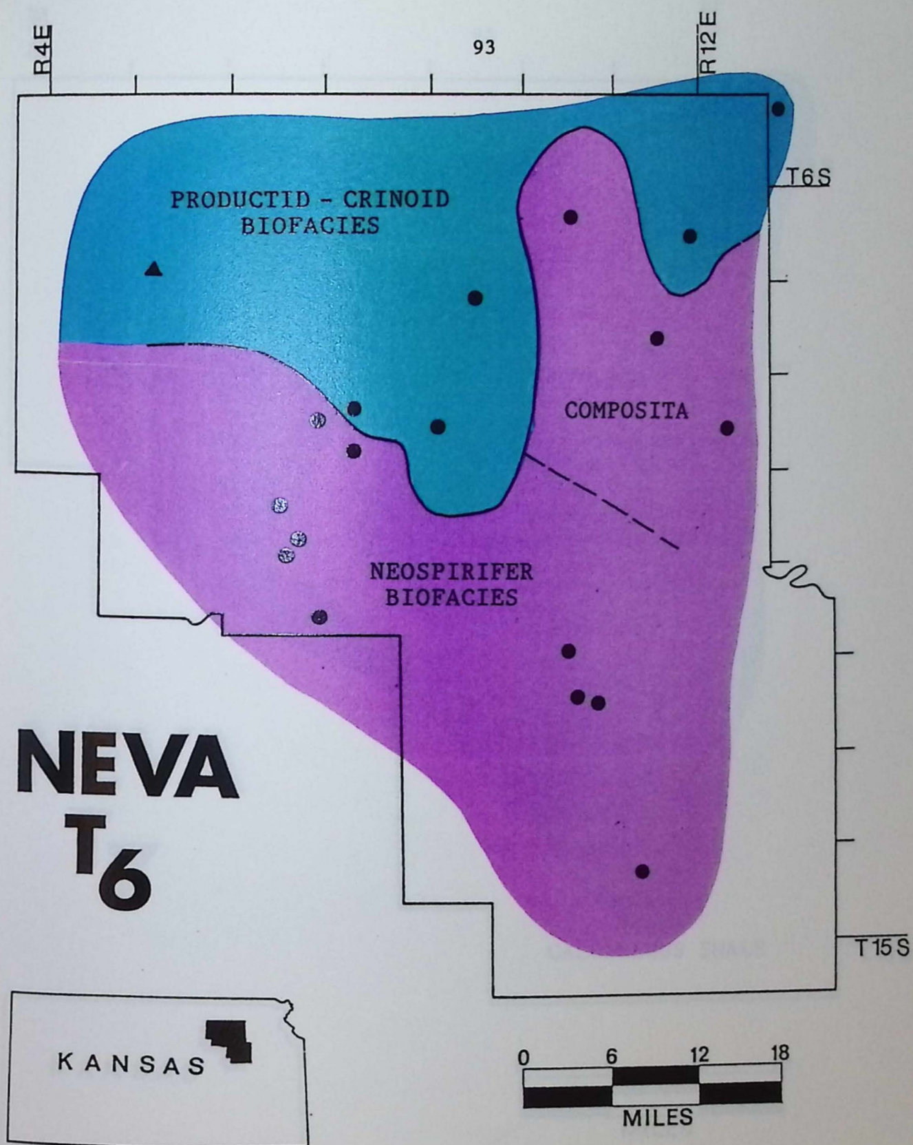
Figure 36. Paleogeographic map of biofacies at the transgressive apex of NT 6 for the localities where NT 6 is present (for locality identification use overlay in pocket).
