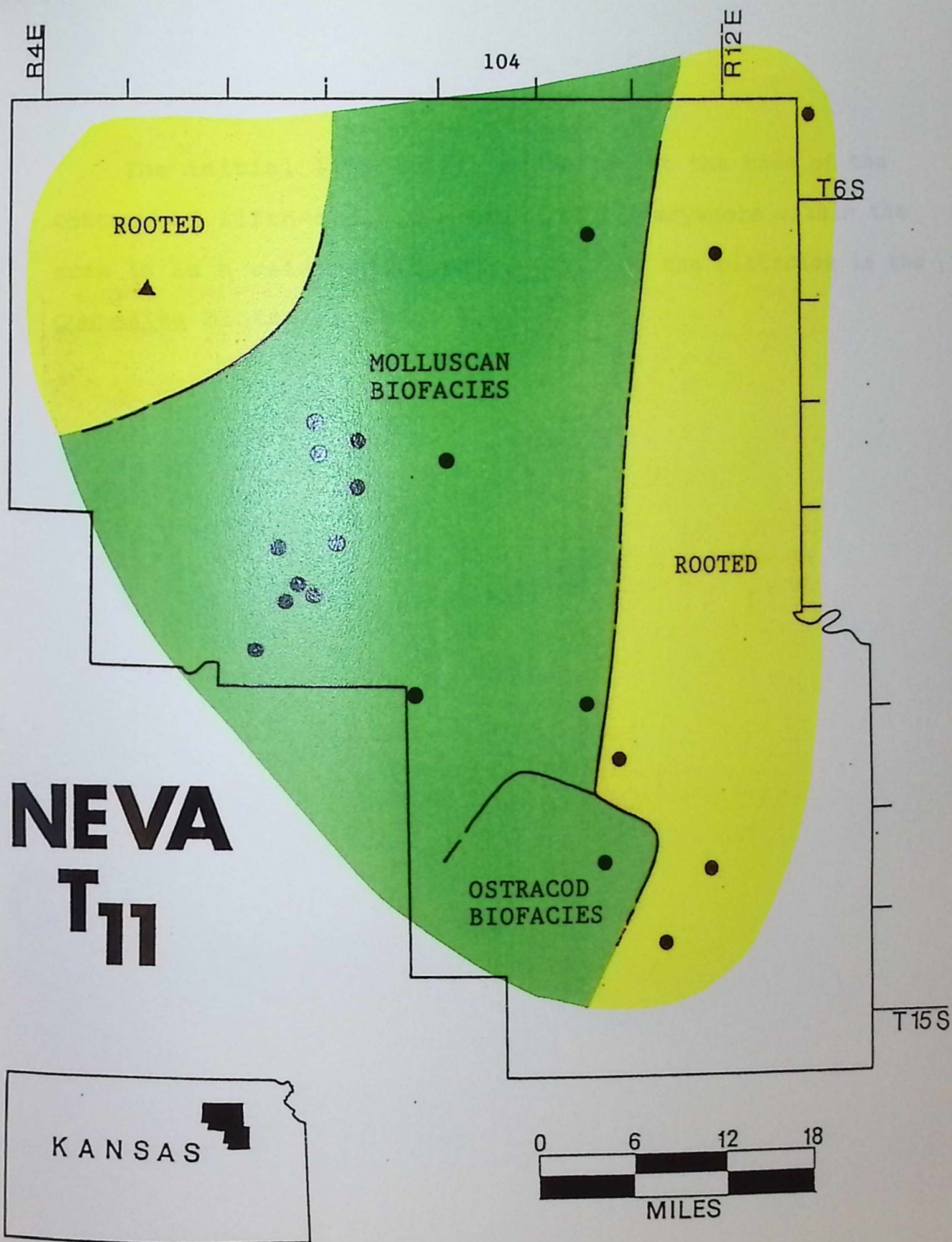
Figure 46. Paleogeographic map of biofacies at the transgressive apex of NT 11 for the localities where NT 11 is present (for locality identification use overlay in pocket).
