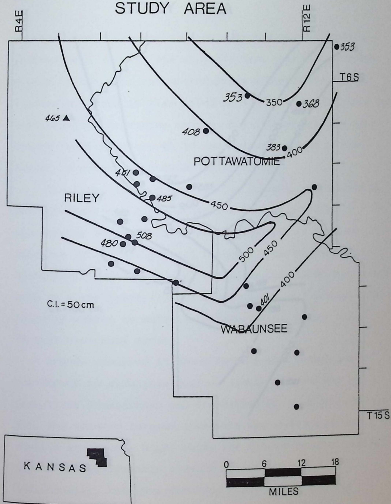
Figure 52. Isopach map of the Neva-Eskridge transgressive hemicycle using the localities where complete intervals are present (for locality identification use overlay in pocket).
