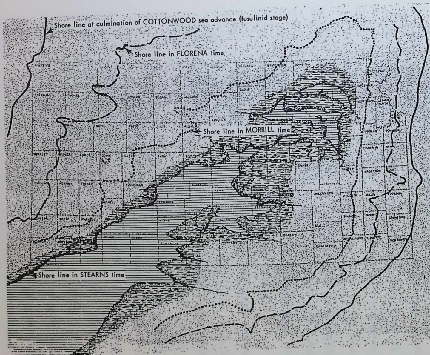
Figure 7. Shoreline development of the members of the Beattie cyclothem (from Moore, 1964).
