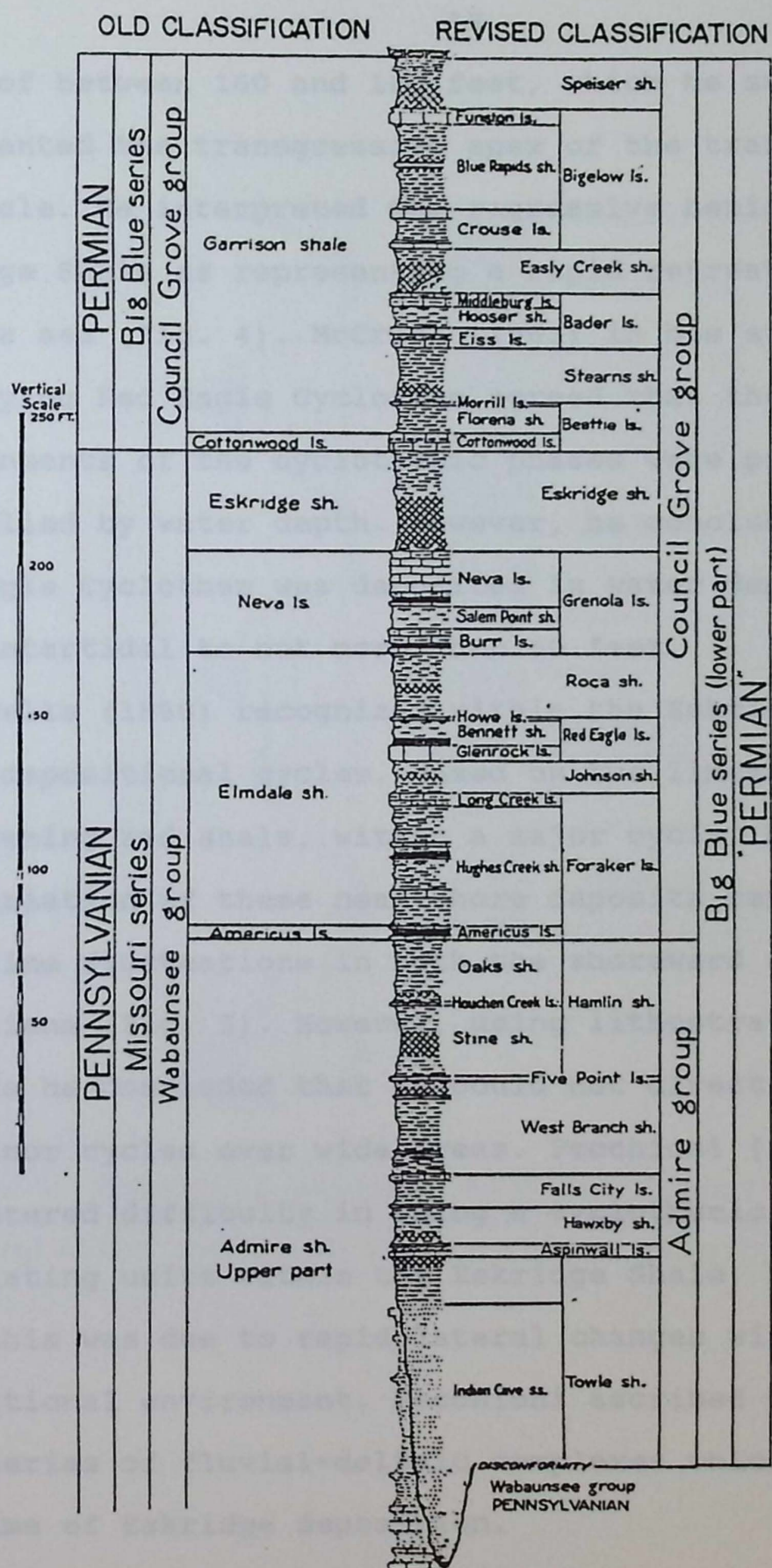
Figure 3. Old and revised classifications for Permo-Carboniferous rocks of Kansas (from Moore, 1936).
