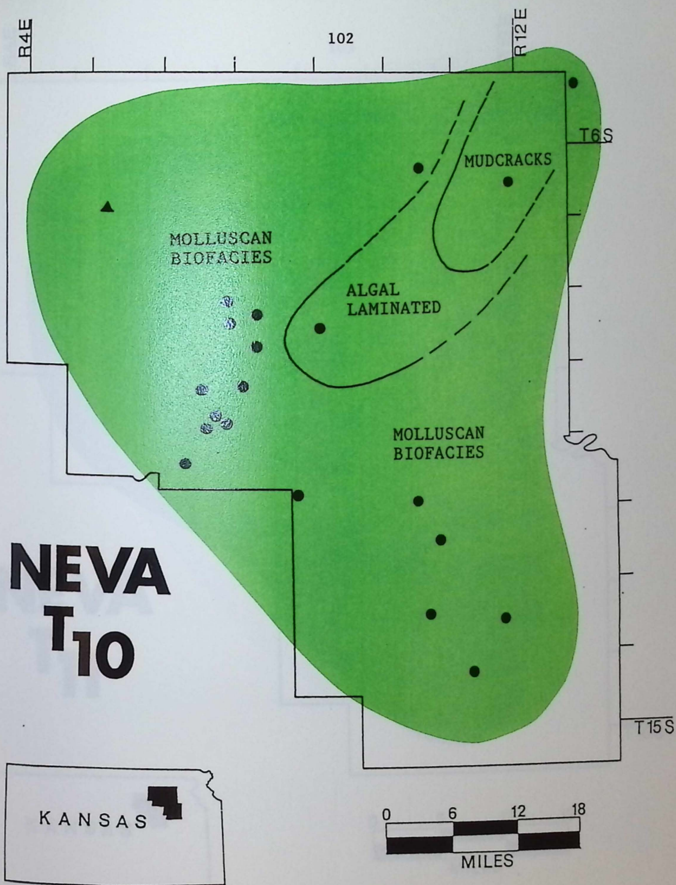
Figure 44. Paleogeographic map of biofacies at the transgressive apex of NT 10 for the localities where NT 10 is present (for locality identification use overlay in pocket).
