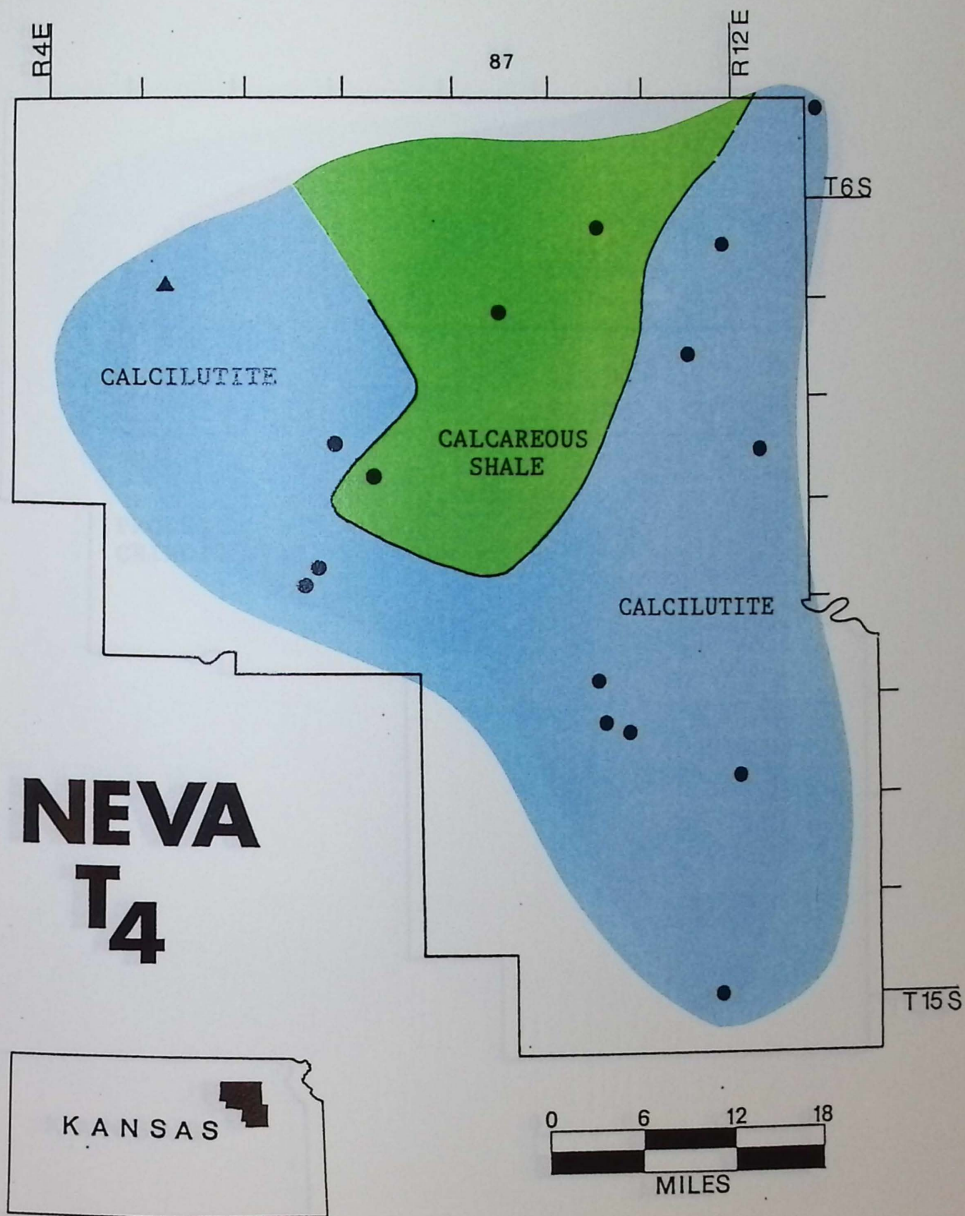
Figure 31. Paleogeographic map of lithofacies at the transgressive apex of NT 4 for the localities where NT 4 is present (for locality identification use overlay in pocket).
