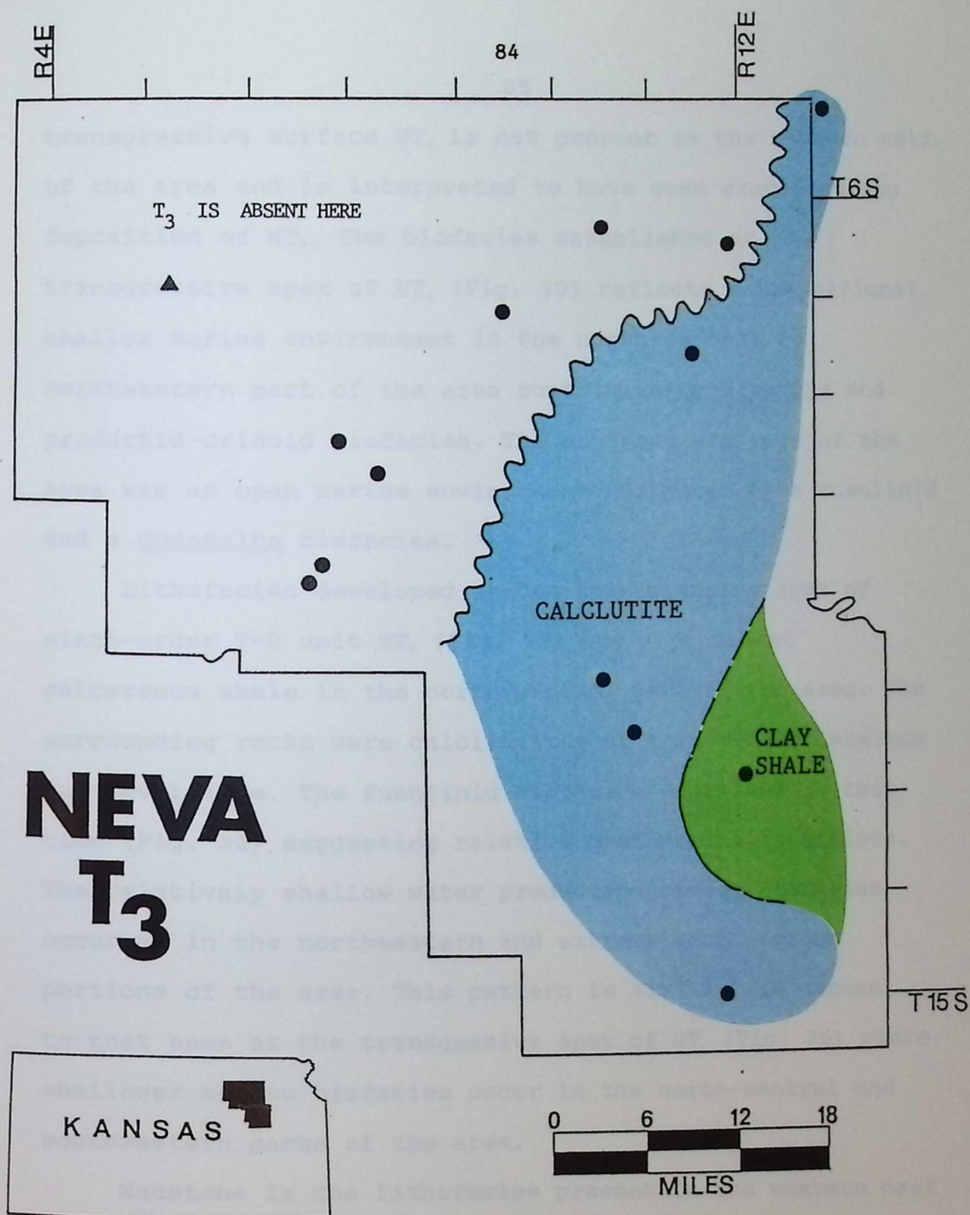
Figure 29. Paleogeographic map of lithofacies at the transgressive apex of NT, for the localities where NT, is present (for locality identification use overlay in pocket).
