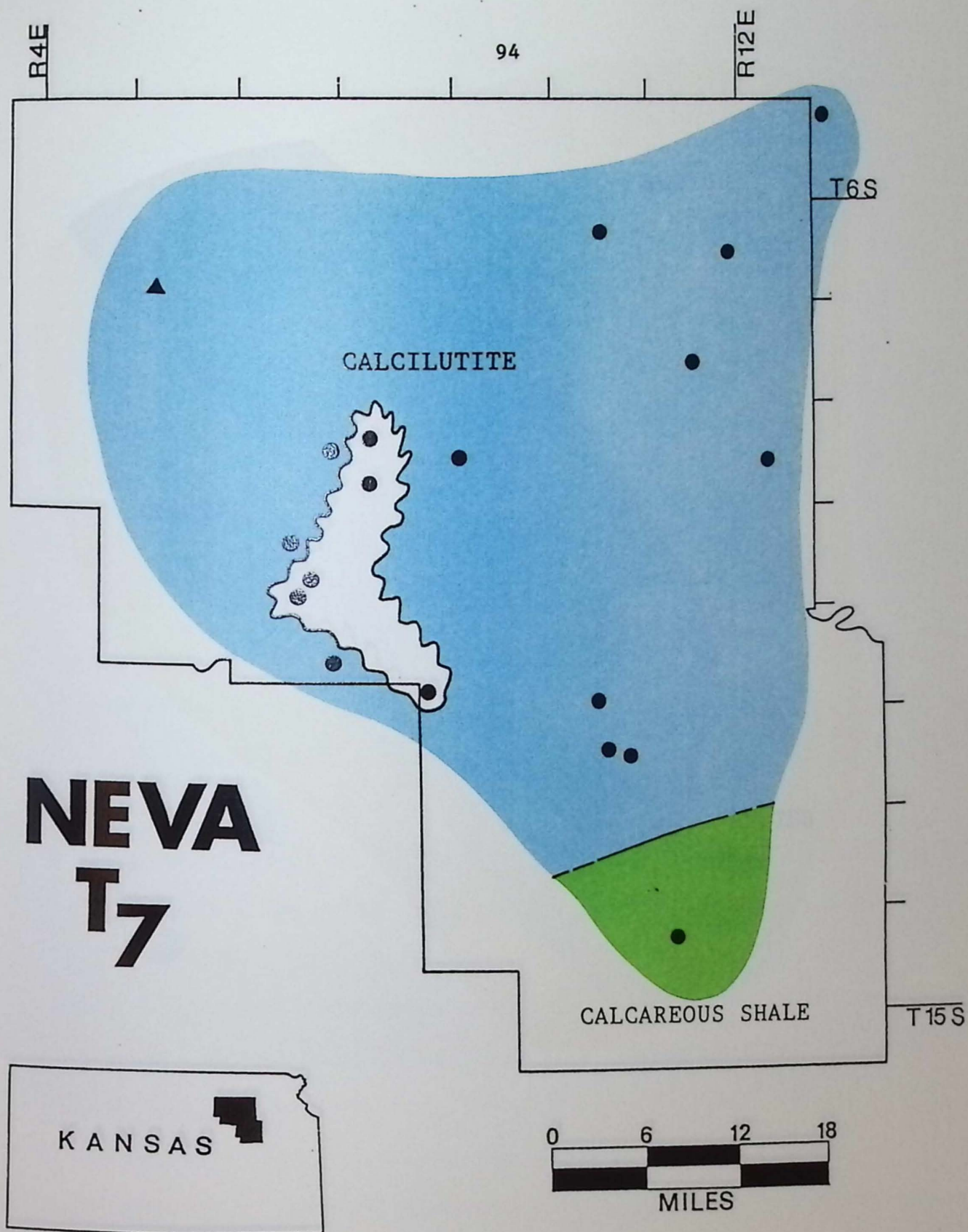
Figure 37. Paleogeographic map of lithofacies at the transgressive apex of NT, for the localities where NT, is present (for locality identification use overlay in pocket).
