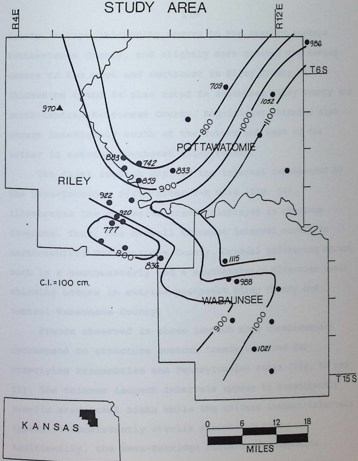
Figure 53. Isopach map of the Neva-Eskridge regressive hemicycle using the localities where complete intervals are present (for locality identification use overlay in pocket).
