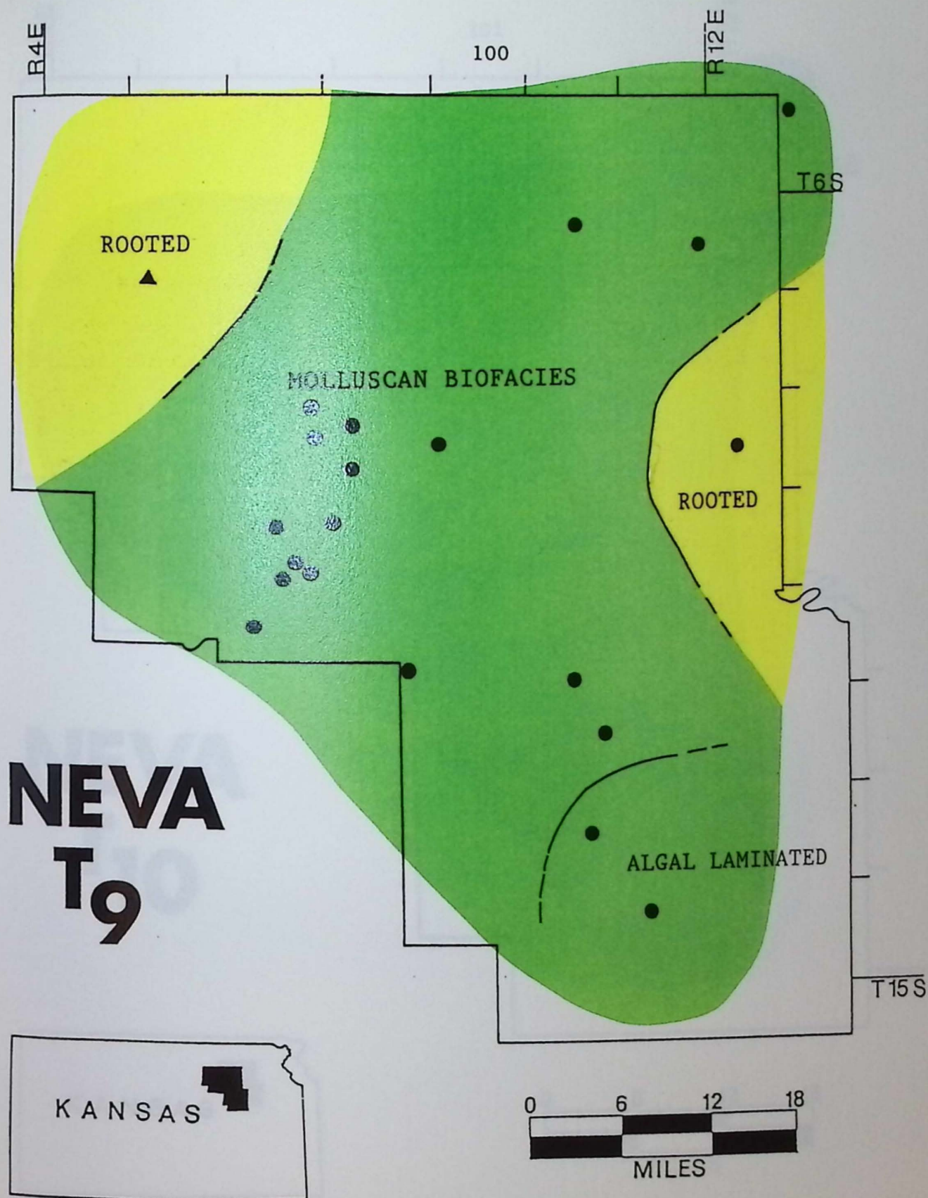
Figure 42. Paleogeographic map of biofacies at the transgressive apex of NT, for the localities where NT, is present (for locality identification use overlay in pocket).
