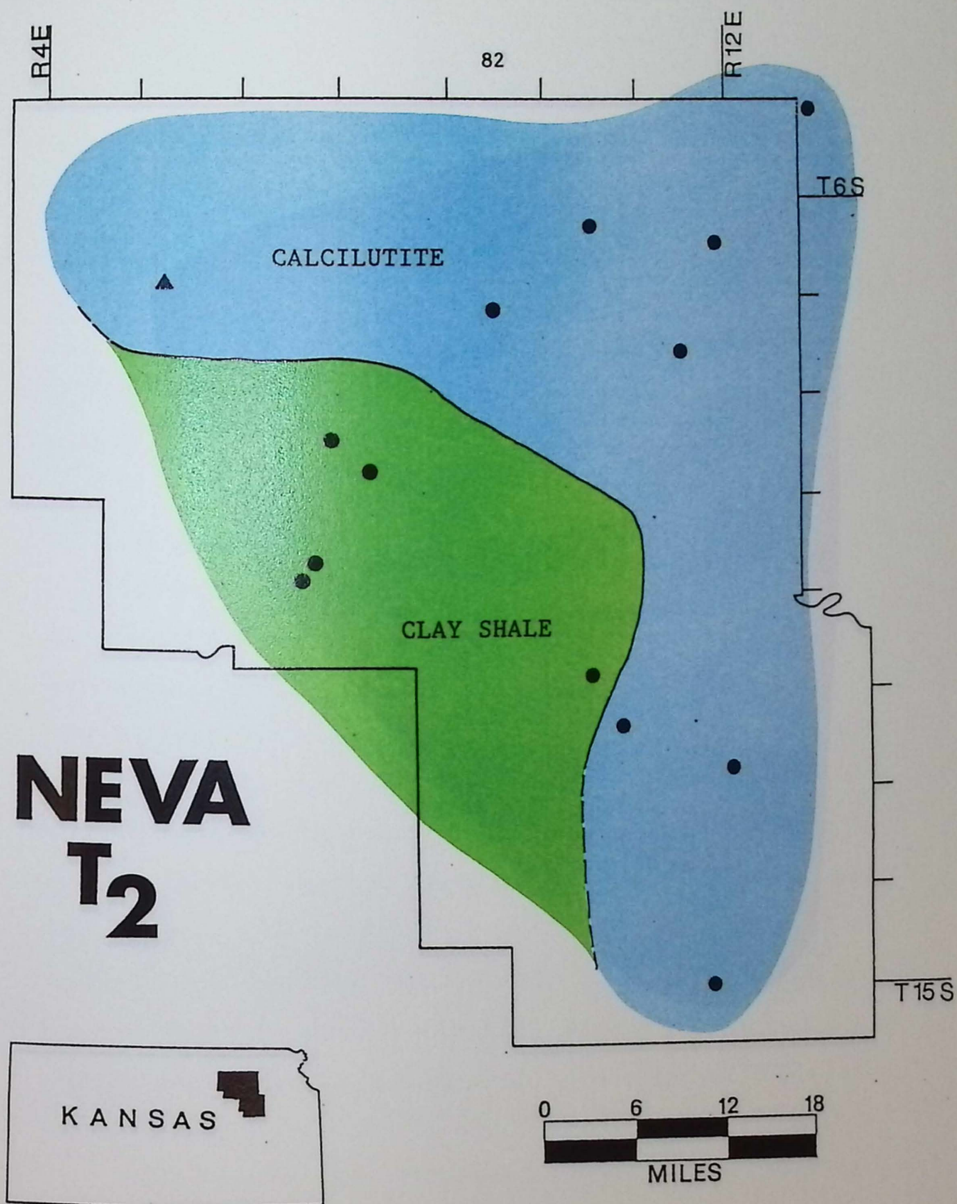
Figure 27. Paleogeographic map of lithofacies at the transgressive apex of NT 2 for the localities where NT 2 is present (for locality identification use overlay in pocket; for clay shale read mudstone).
