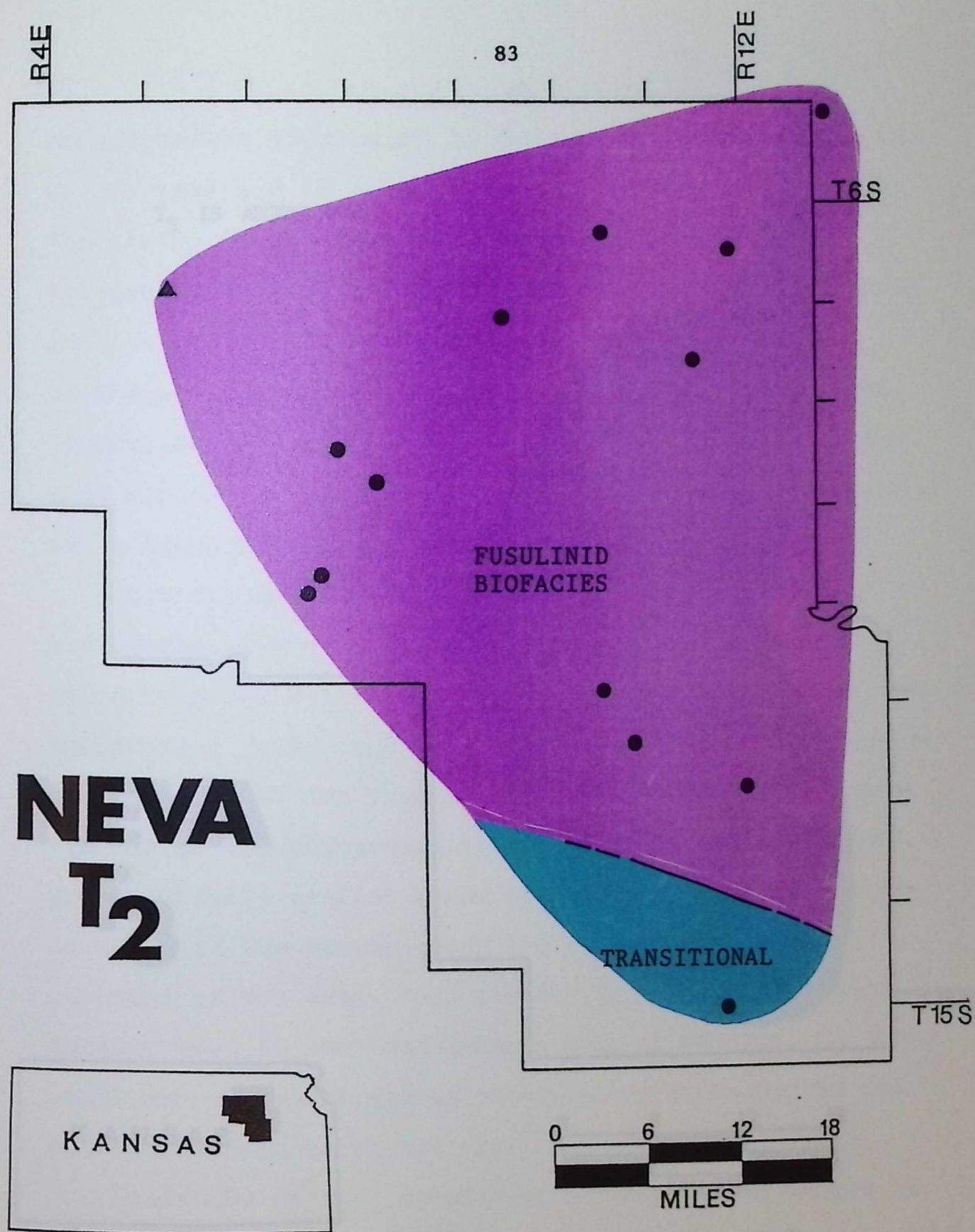
Figure 28. Paleogeographic map of biofacies at the transgressive apex of NT 2 for the localities where NT 2 is present (for locality identification use overlay in pocket).
