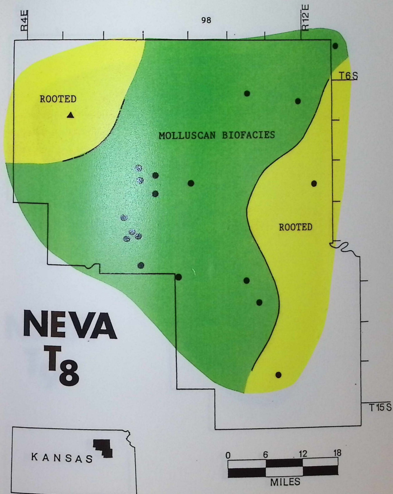
Figure 40. Paleogeographic map of biofacies at the transgressive apex of NT 8 for the localities where NT 8 is present (for locality identification use overlay in pocket).
