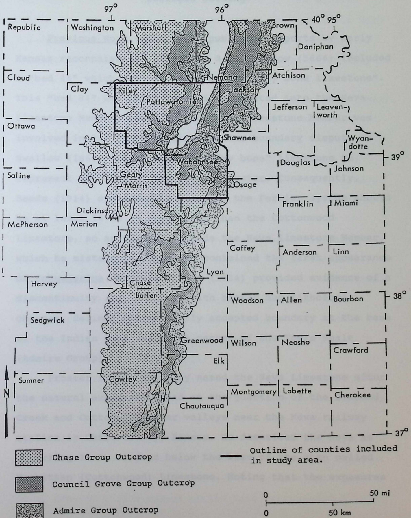
Figure 2. Map view of outcropping Lower Permian aged rocks in eastern Kansas (modified from Aber and Grisafe, 1982).
