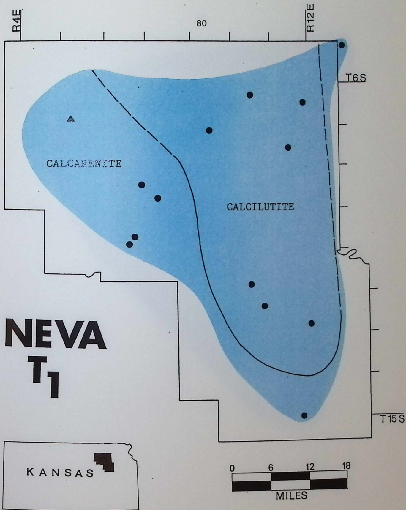
Figure 25. Paleogeographic map of lithofacies at the transgressive apex of NT 1 for the localities where NT 1 is present (for locality identification use overlay in pocket).
