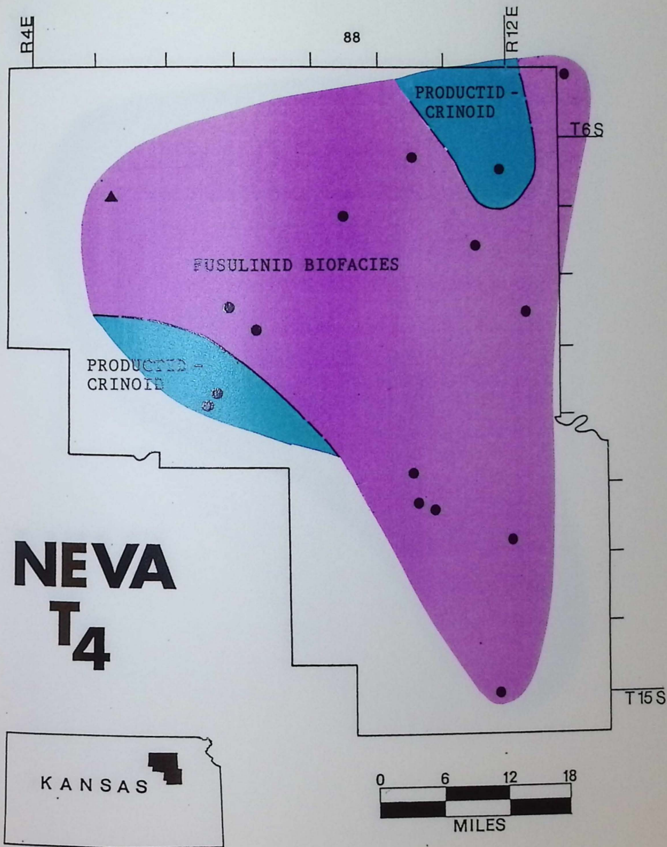
Figure 32. Paleogeographic map of biofacies at the transgressive apex of NT 4 , for the localities where NT 4 is present (for locality identification use overlay in pocket).
