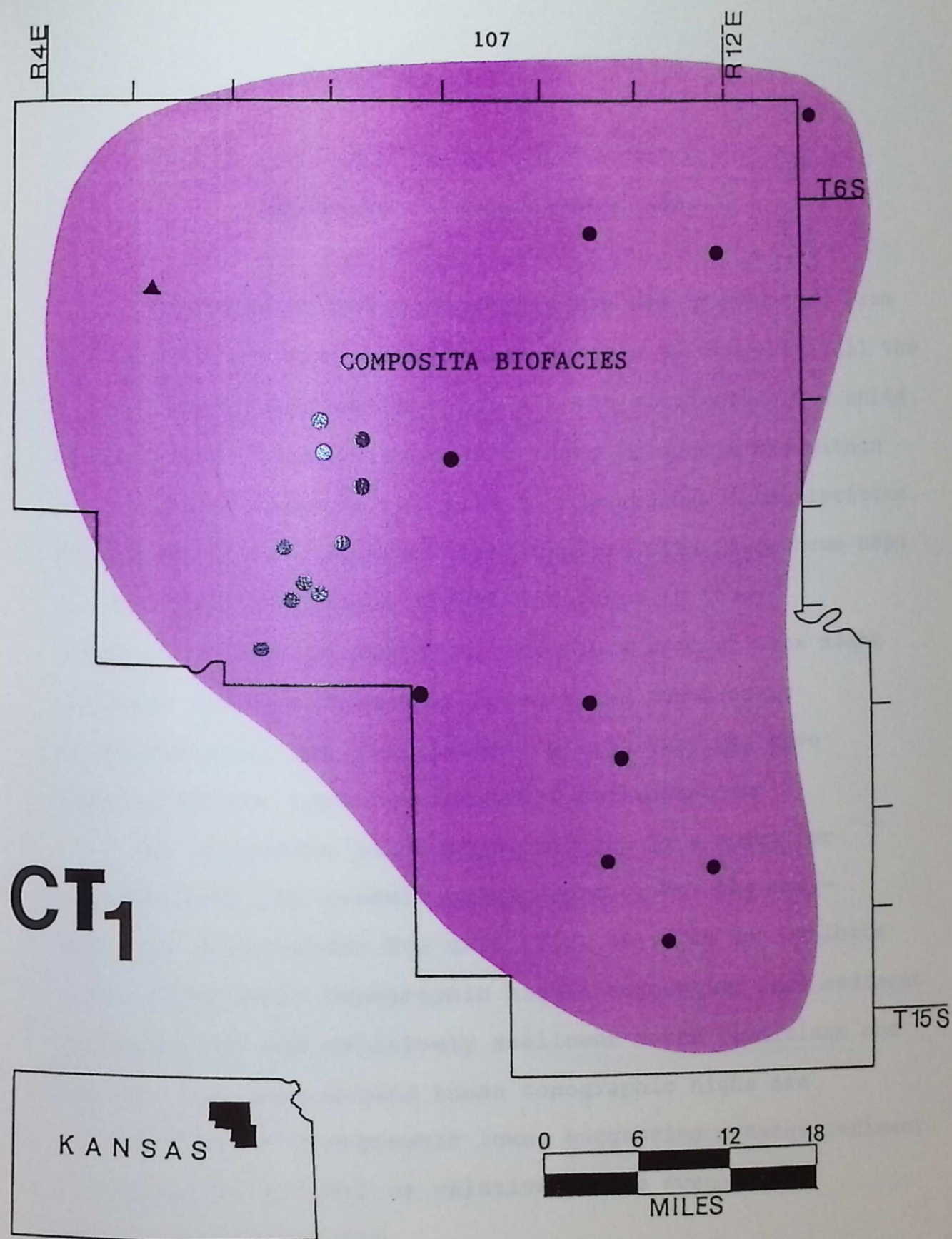
Figure 48. Paleogeographic map of biofacies at the transgressive surface of CT 1 , for the localities where CT 1 is present (for locality identification use overlay in pocket).
