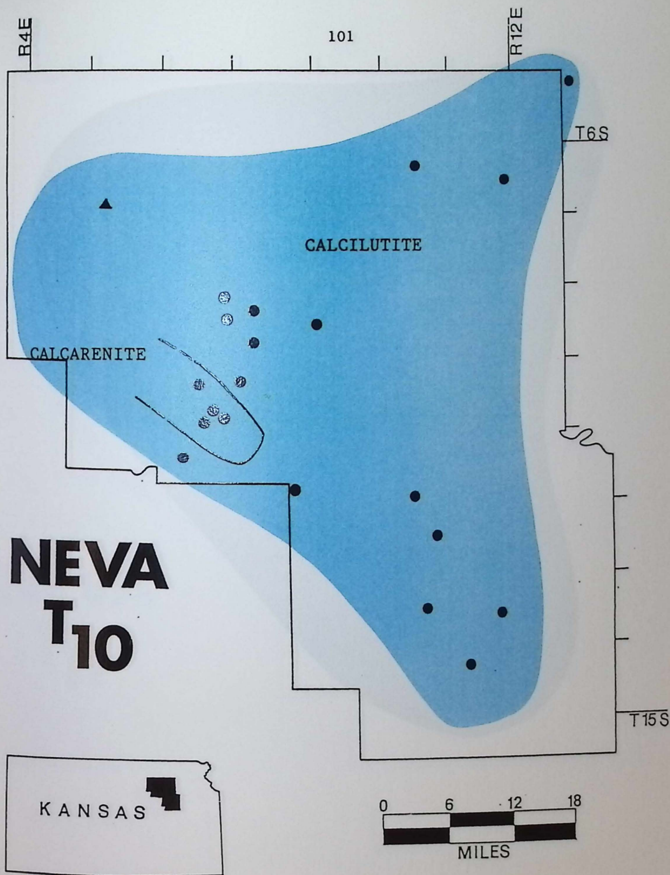
Figure 43. Paleogeographic map of lithofacies at the transgressive apex of NT_{10} for the localities where NT_{10} is present (for locality identification use overlay in pocket).
