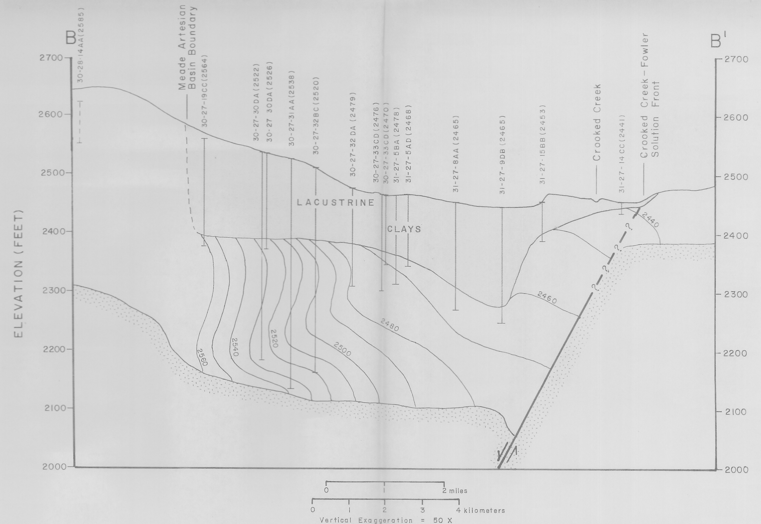
B-B' - CROSS SECTION OF MEADE ARTESIAN BASIN (SEE LOCATION MAP)
