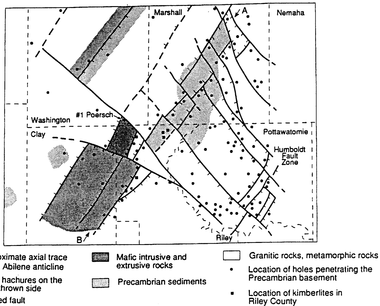
Figure 4. Tectonic map of the Midcontinent rift in Kansas (after Berendsen, et al. , 1988, Fig. 18).
