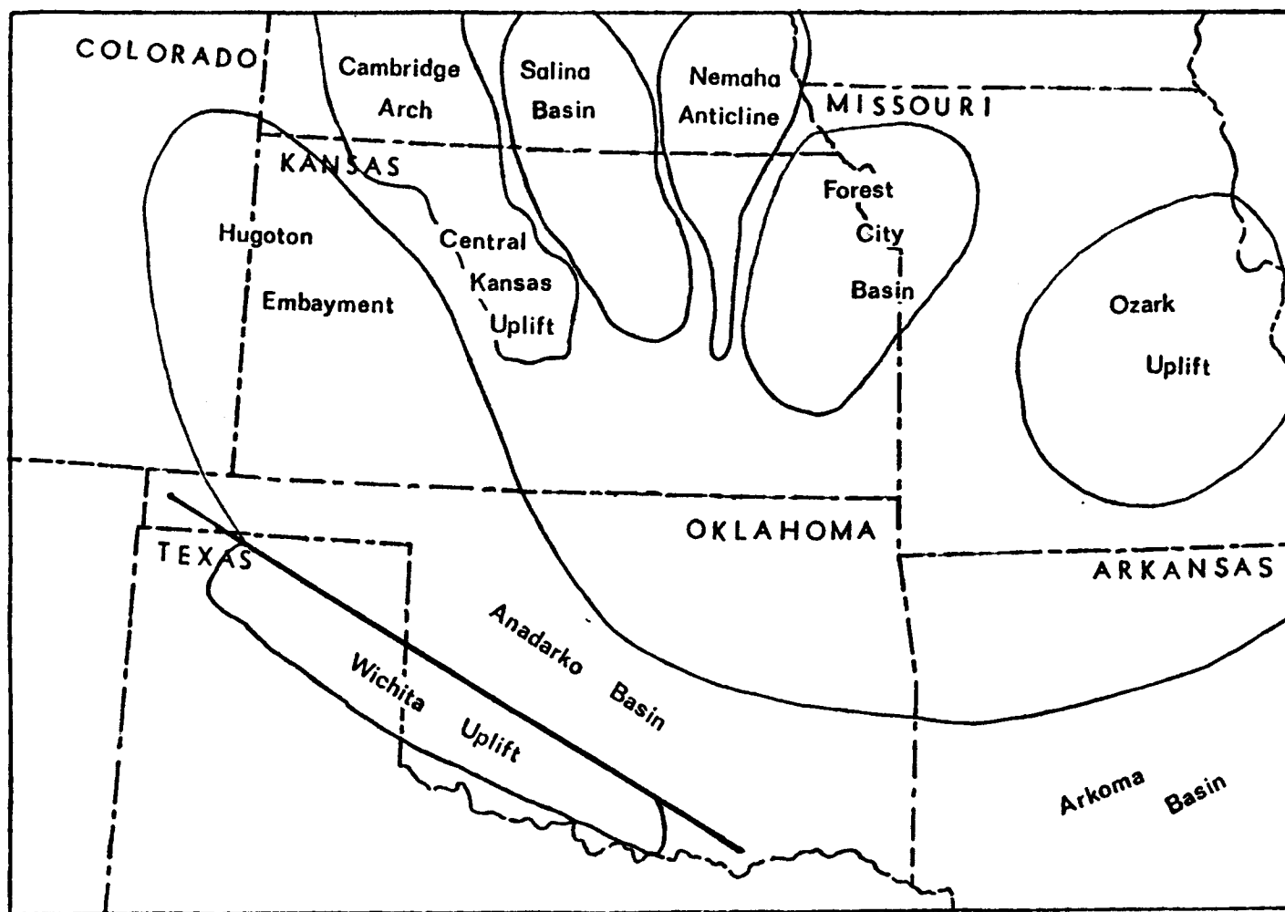
Figure 6. Map of post-Late Mississippian regional structures (after Roehl, 1985, Fig. 20).
