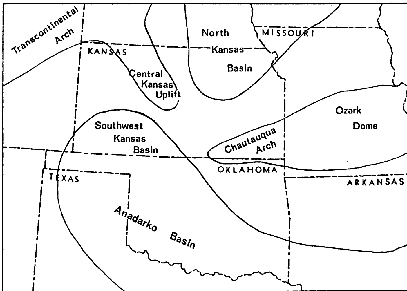
Figure 5. Map of pre-Late Mississippian regional structures (after Roehl, 1985, Fig. 19).
