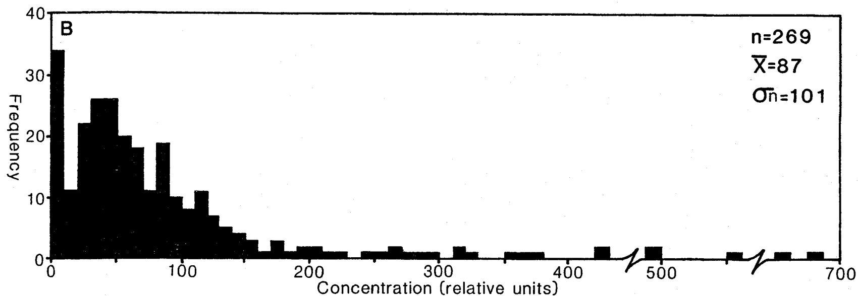
Figure 13. Histograms of A) "absolute", and B) "relative" hydrogen soil gas measurements.
