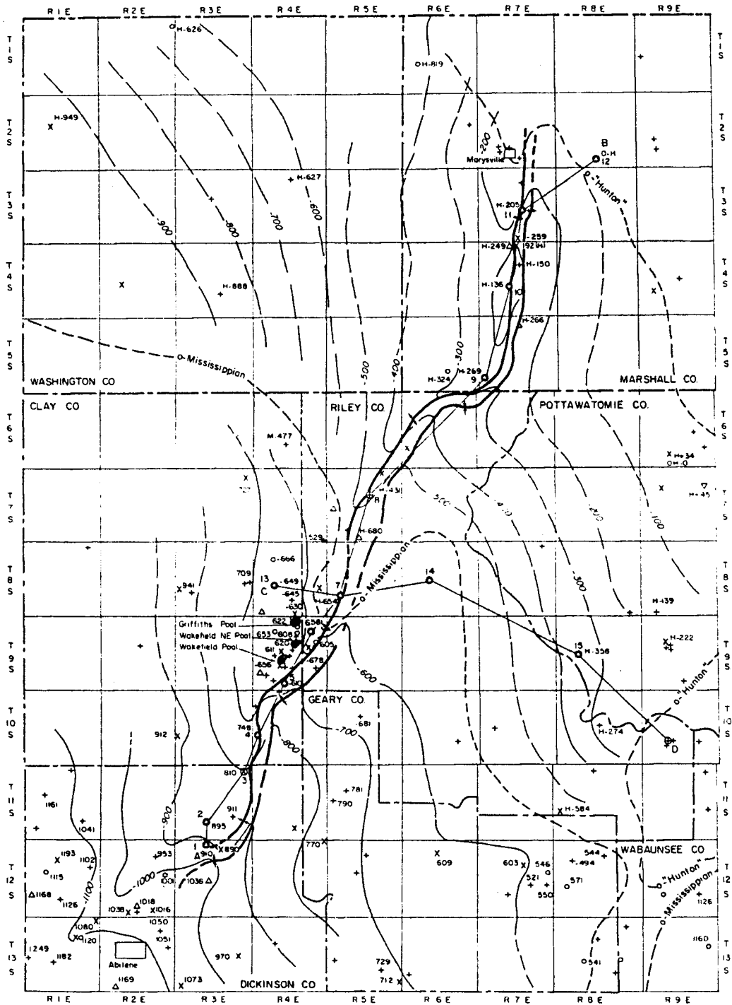
Figure 7. Map showing location of Abilene anticline (after Shenkel, 1959, Fig. 2).
