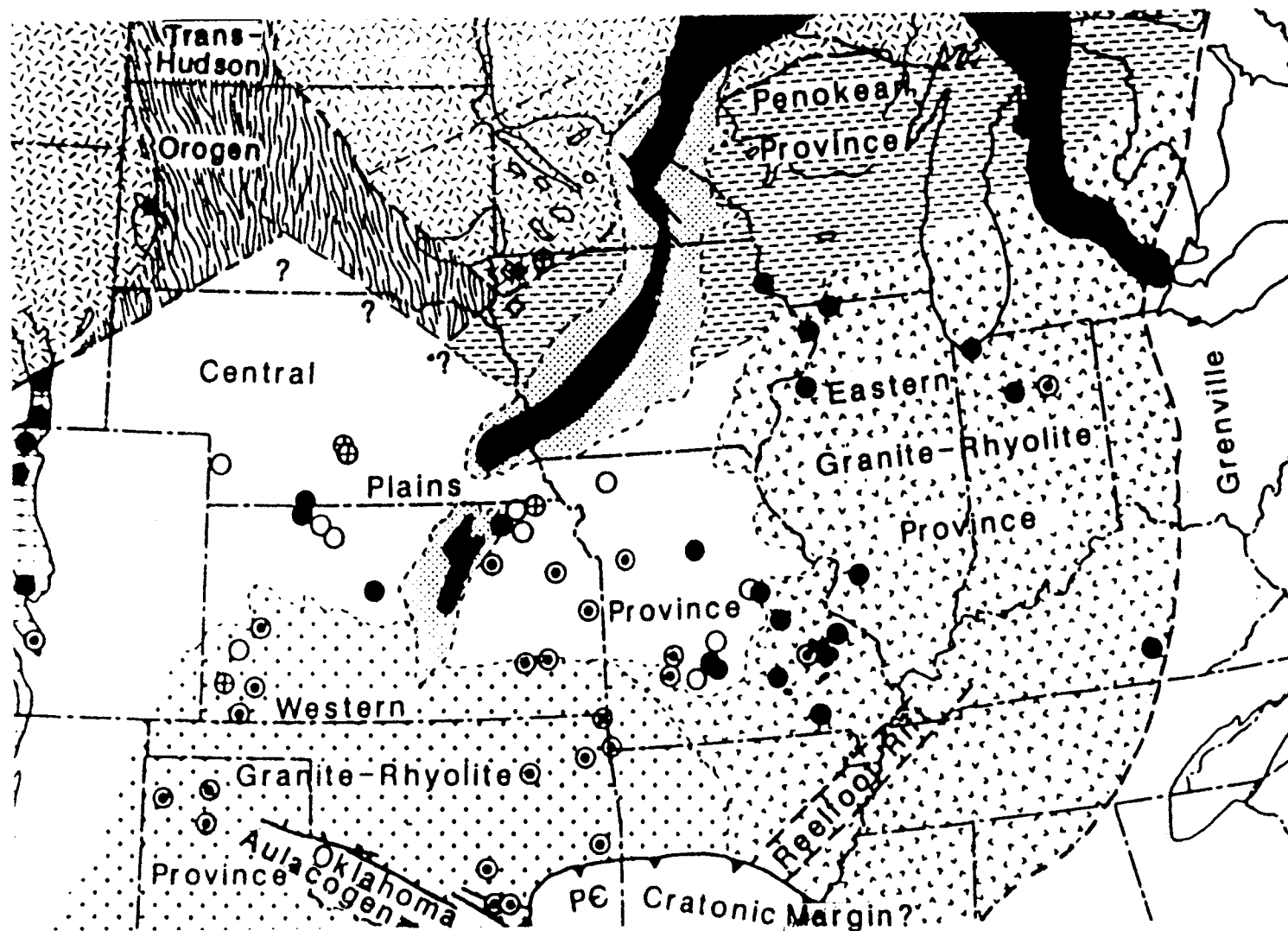
Figure 2. Map of regional Precambrian radiometric-age provinces (after Bickford, et al. , 1986, Fig. 1).
