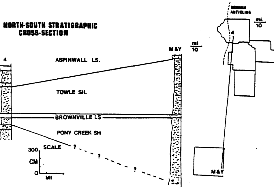
Figure 5. North-south stratigraphic cross-section from central Pottawatomie County to eastern Cowley County.
