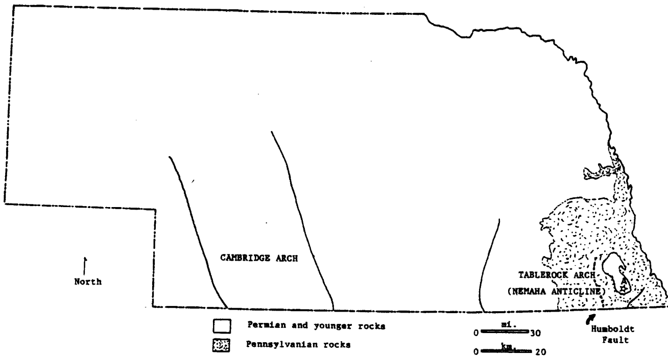
Figure 2. Major structural features of southern Nebraska, Permian-Pennsylvanian outcrop belt, and location of Section A
