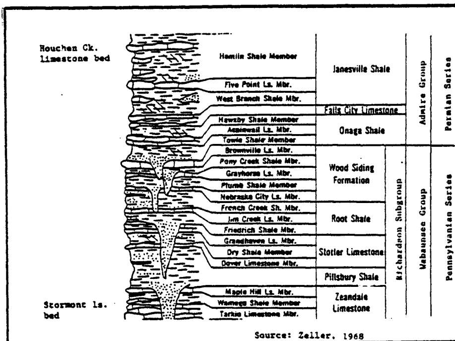
Figure 1. Stratigraphic position of the Onaga Shale and Wood Siding Formation
