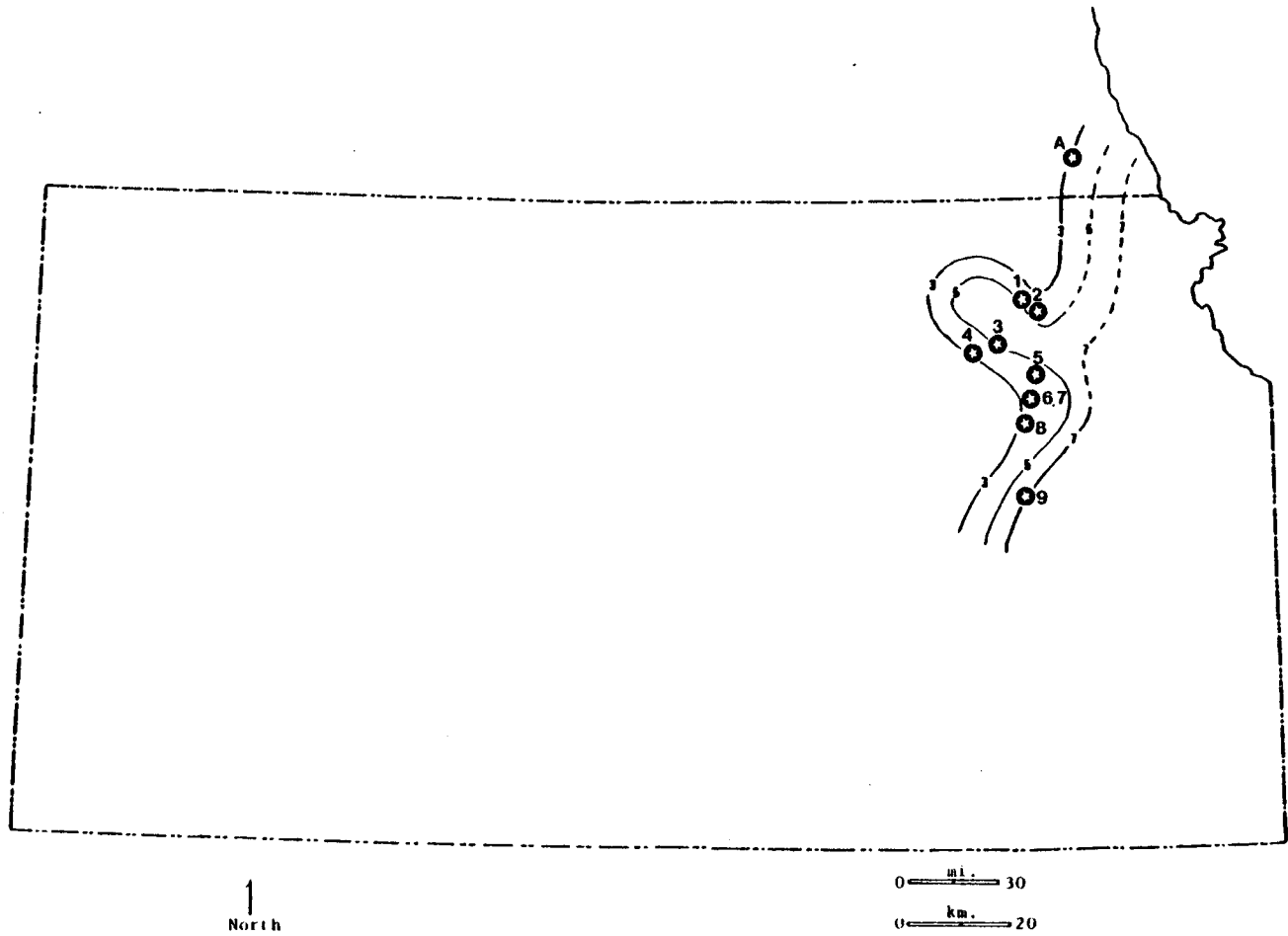
Figure 6. Relative diversity of taxa in the Brownville Limestone Member. Contours based on number of major taxa (refer to allochems section, Appendix III) present at each locality.
