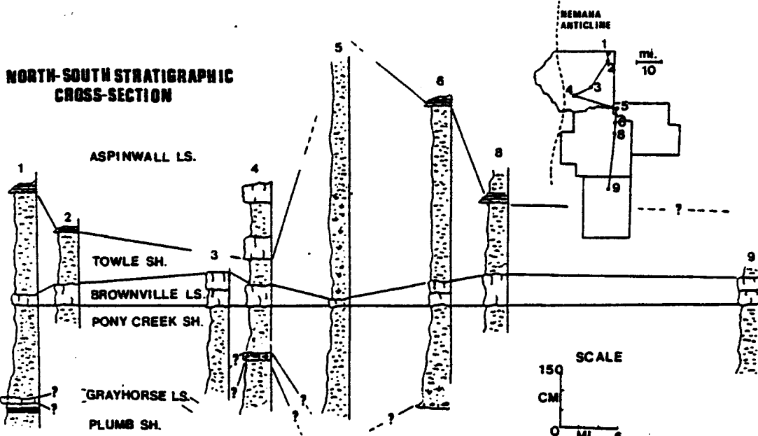
Figure 4. North-south stratigraphic cross-section from northern Pottawatomie County to north-central Lyon County.
