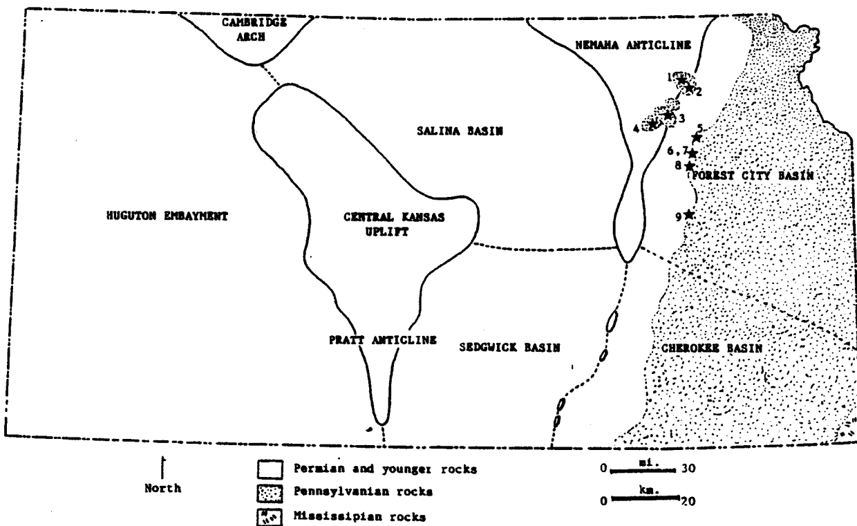
Figure 3. Major structural features of Kansas, Permian-Pennsylvanian outcrop belt, and location of measured sections.
