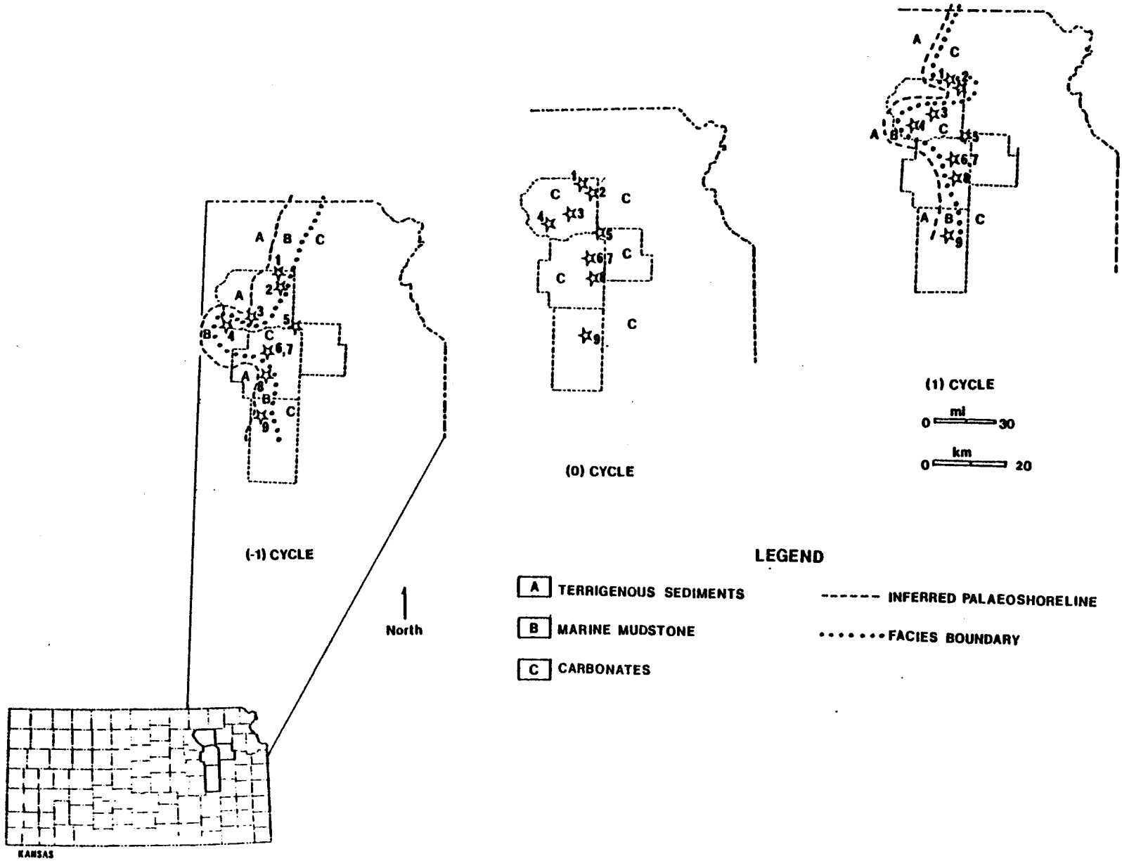
Figure 10. Probable facies deposition and location of palaeoshoreline during (-1), (0), and (1) cycles.
