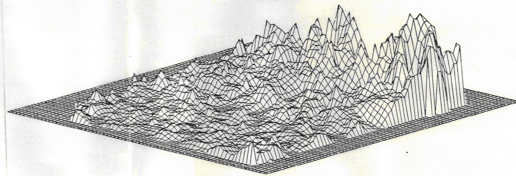
K. G. Society Short Course Prospective Diagram Thickness of Porous Carbonate J-Zone 15' above horizon, looking southeast W. Lynn Watney Kansas Geological Survey 4/15/86
