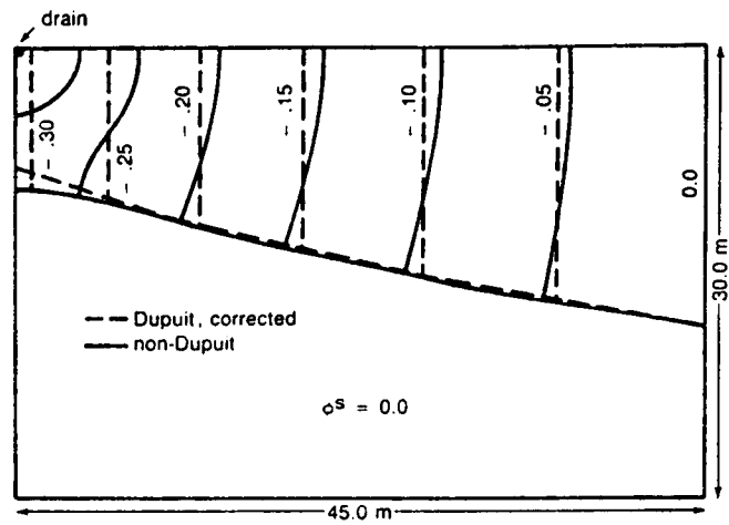
Figure 9.6 Interface location and freshwater flow net, \phi_D = -.564 m.
