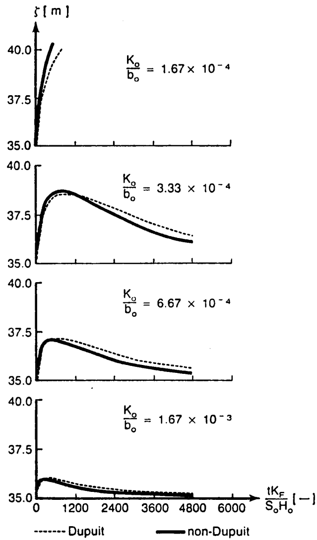
Figure 9.10 Rise of interface under a river.
