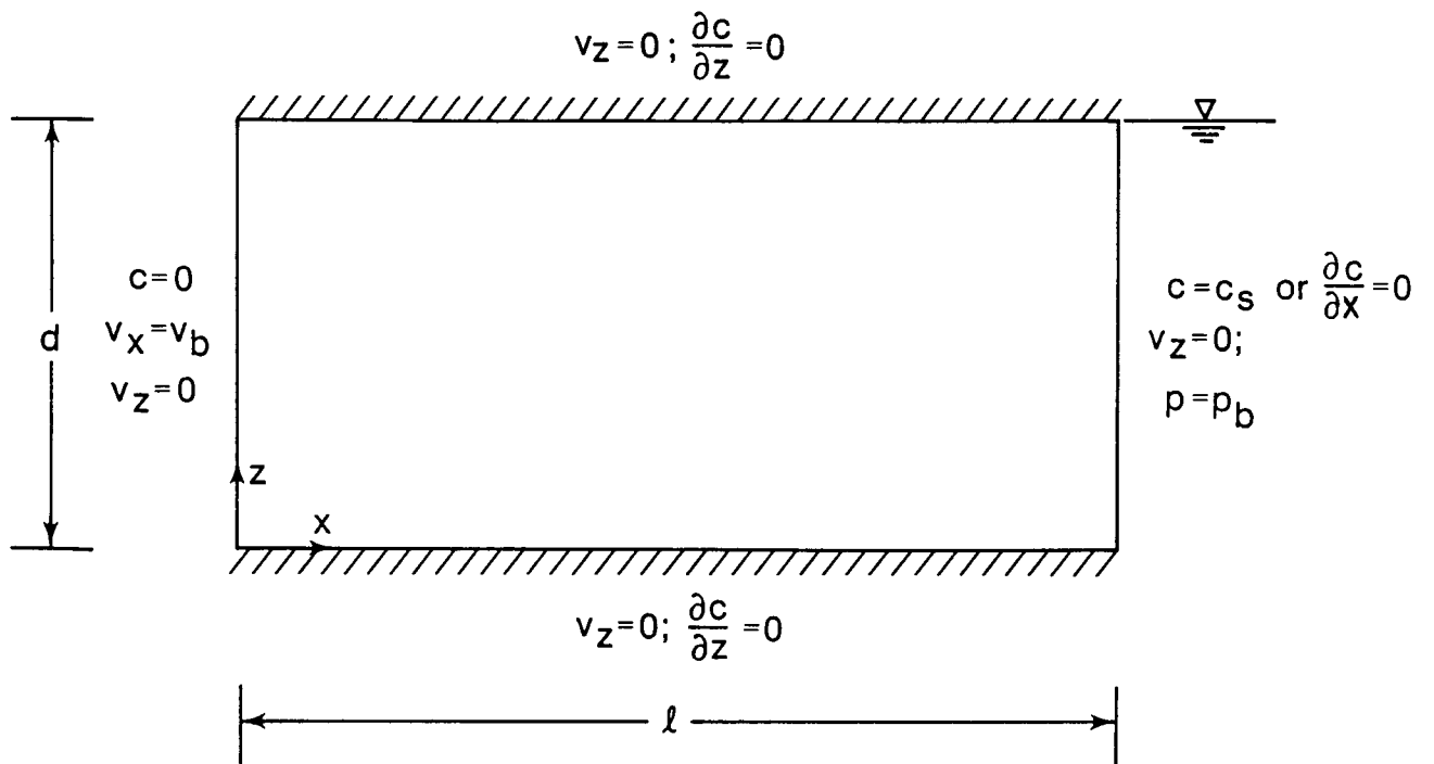
Figure 11.1 Schematic representation of the Henry's example.
