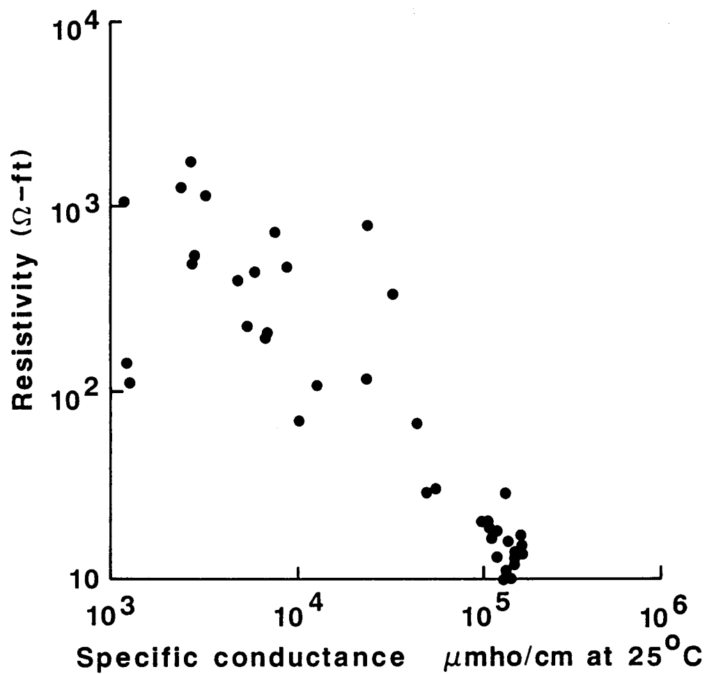
Figure 5.2 Scatter diagram of borehole fluid resistivities vs. specific conductance of the water samples.
