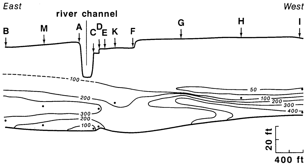
Figure 6.3 Variation of the hydraulic conductivity (ft/day) in the field cross-section.
