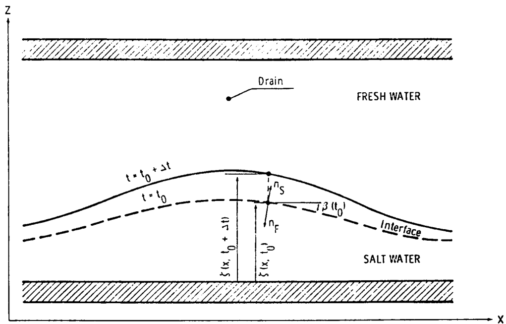
Figure 8.1 Saltwater/freshwater interface-motion scheme.
