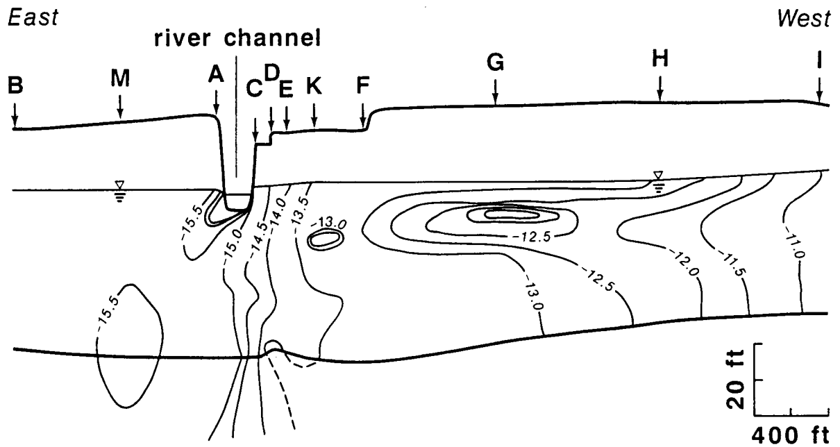
Figure 6.7 Hydraulic head distribution along the field cross-section on October 16, 1985.
