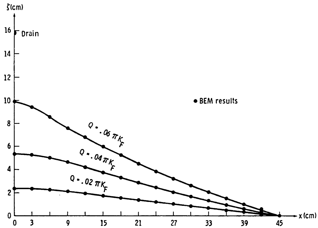
Figure 8.10 The shapes of the steady-state interfaces.
