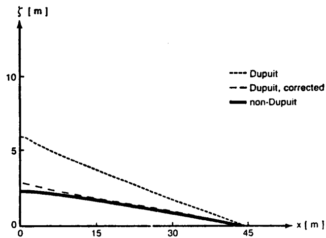
Figure 9.4 Location of steady-state interface, \phi_D = -.175 m.
