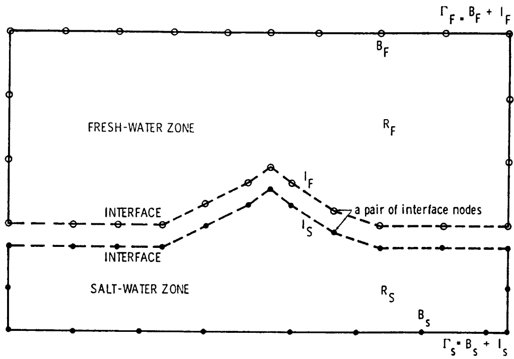
Figure 8.2 Discretized region for the numerical solution.
