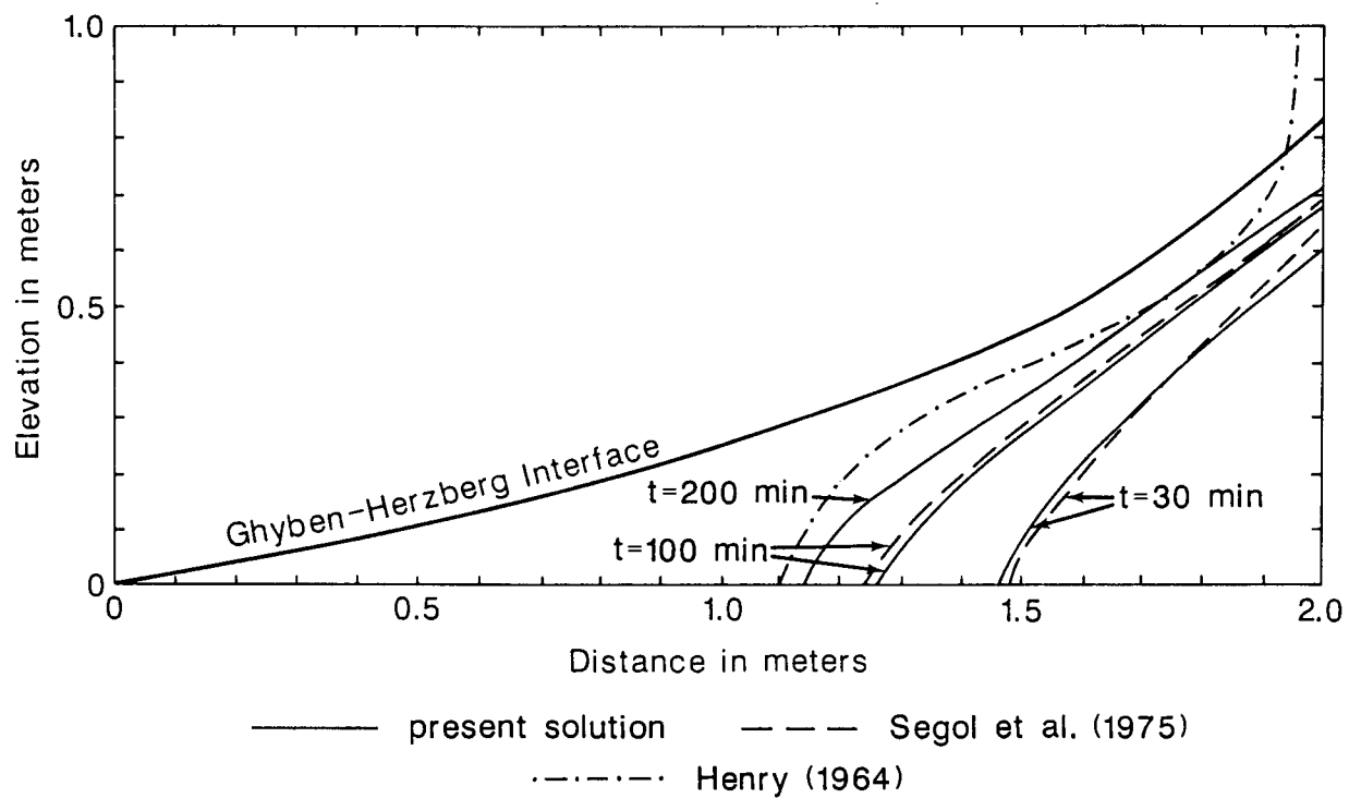
Figure 11.3 The comparison of 0.5 isochlors computed by the present model using mixed interpolations with several available solutions.
