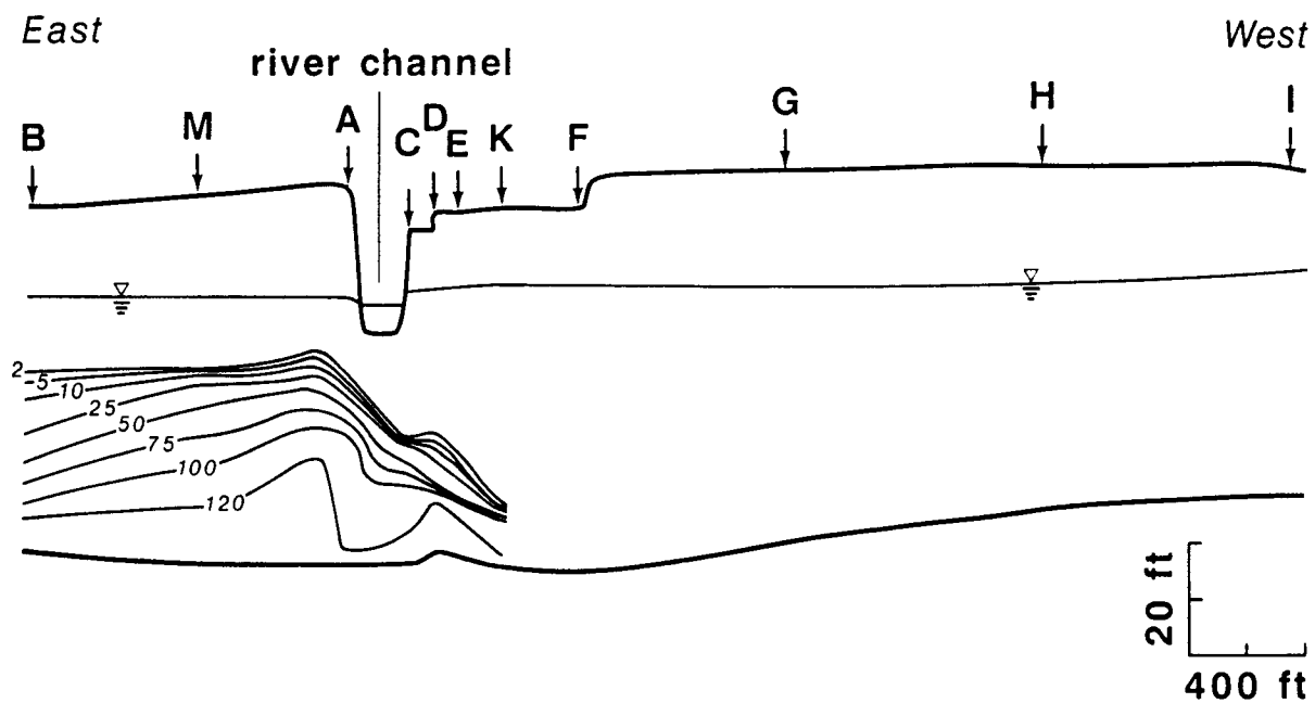
Figure 6.17 Distribution of total dissolved solids of ground-water at the field cross-section on October 16, 1985.
