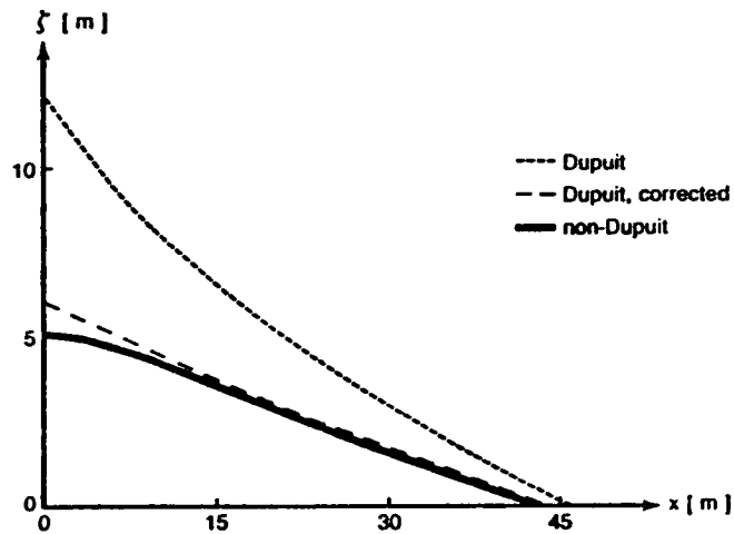
Figure 9.5 Location of steady-state interface, \phi_D = -.36 m.
