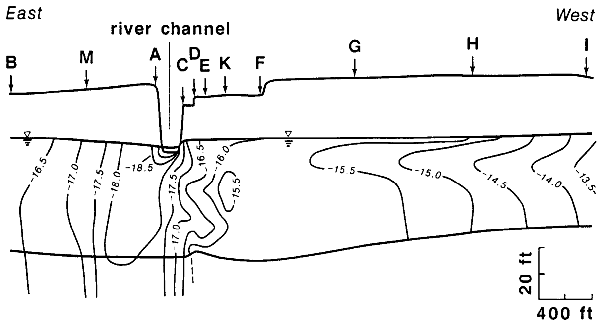
Figure 6.9 Hydraulic head distribution along the field cross-section on November 27, 1985.
