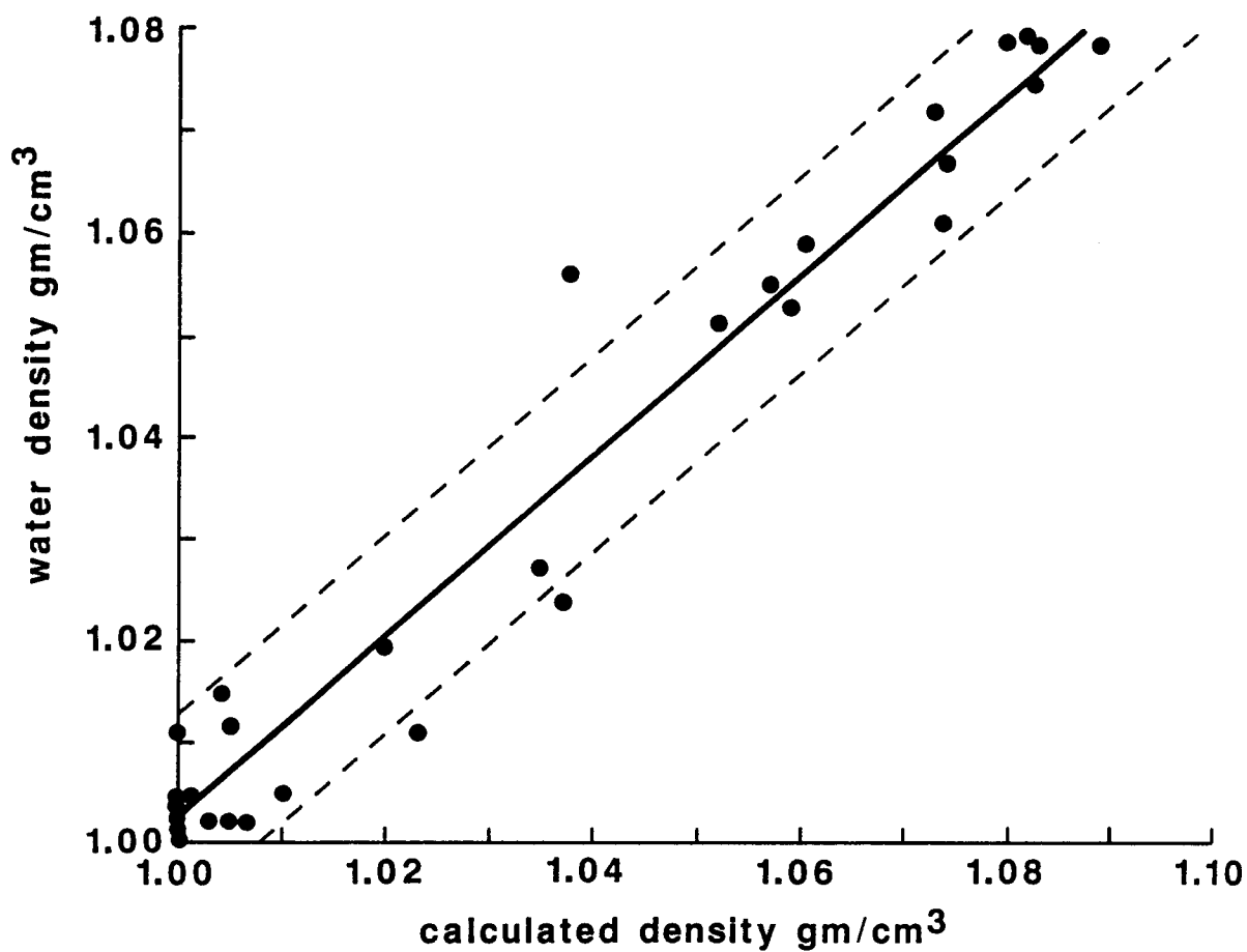
Figure 5.6 Linear regression of groundwater sample densities and ground-water densities calculated from the differential pressure method, showing also the 95% prediction limits.
