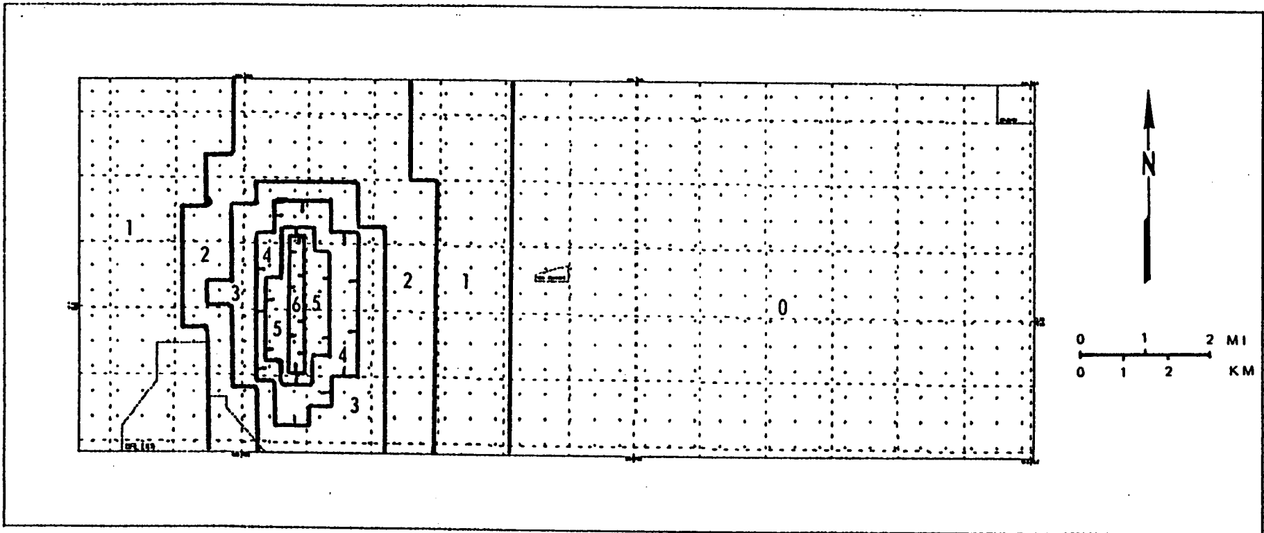
Figure II-12. Drawdown Case I, Test 5 for the mathematically calibrated model.
