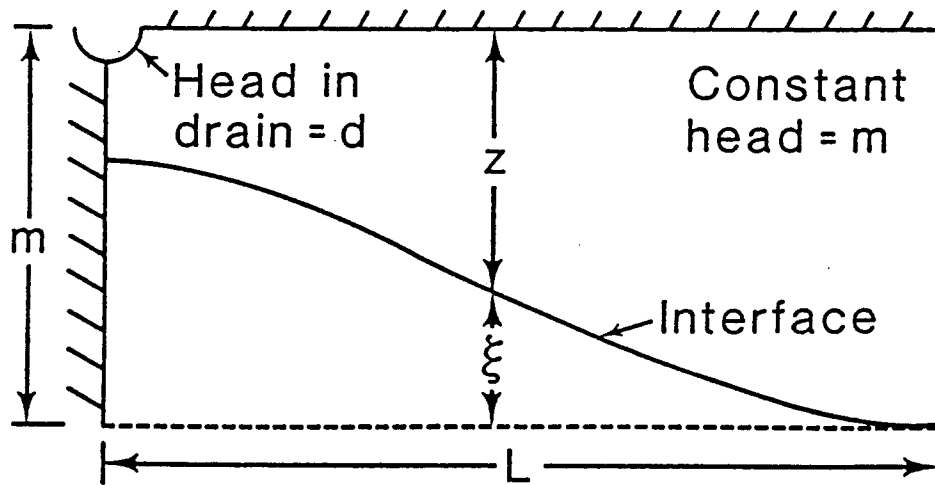
b. Idealized flow toward a drain
