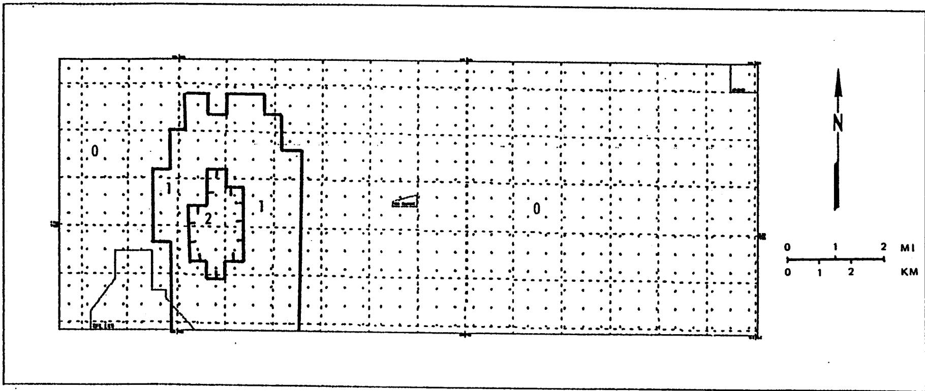
Figure II-11. Drawdown Case I, Test 2 for the mathematically calibrated model.
