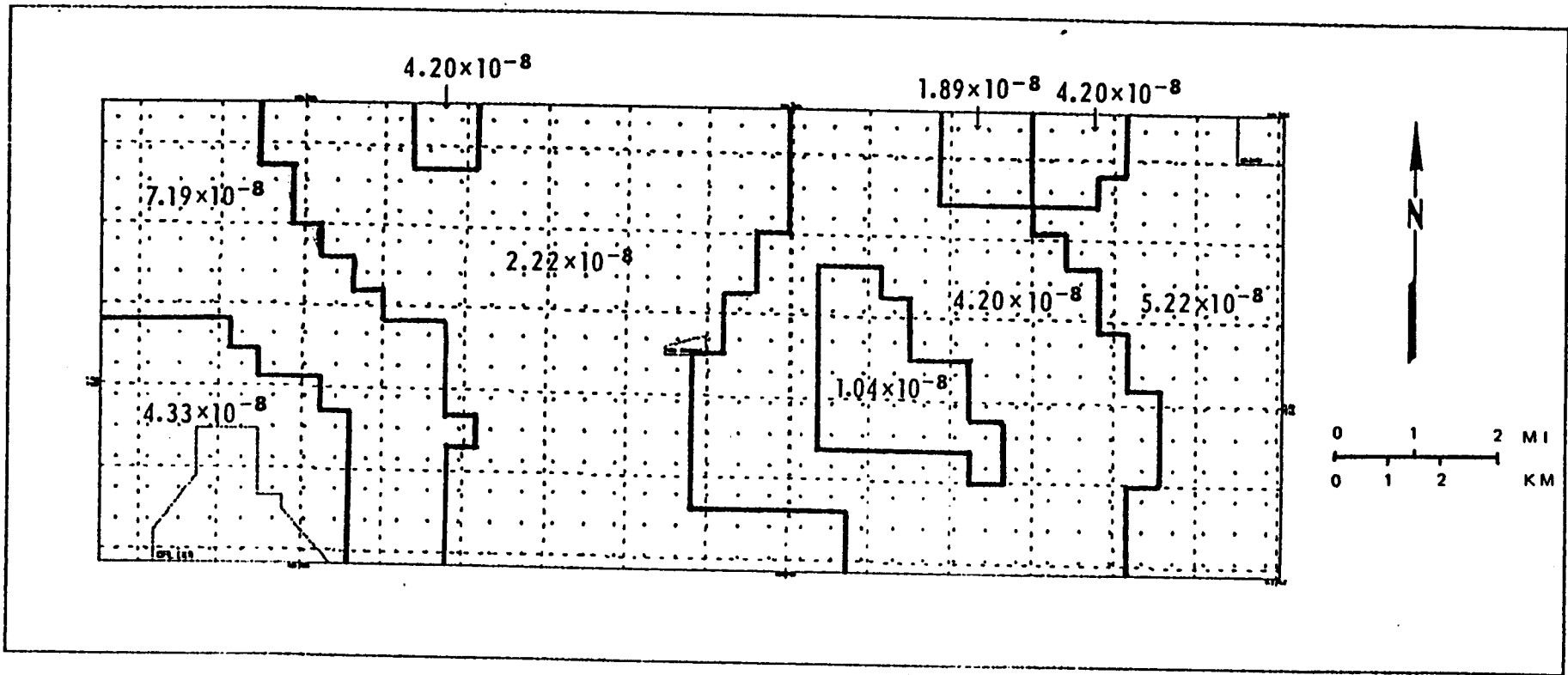
Figure II-8. Confining bed hydraulic conductivity (ft/sec) for the mathematically calibrated model.
