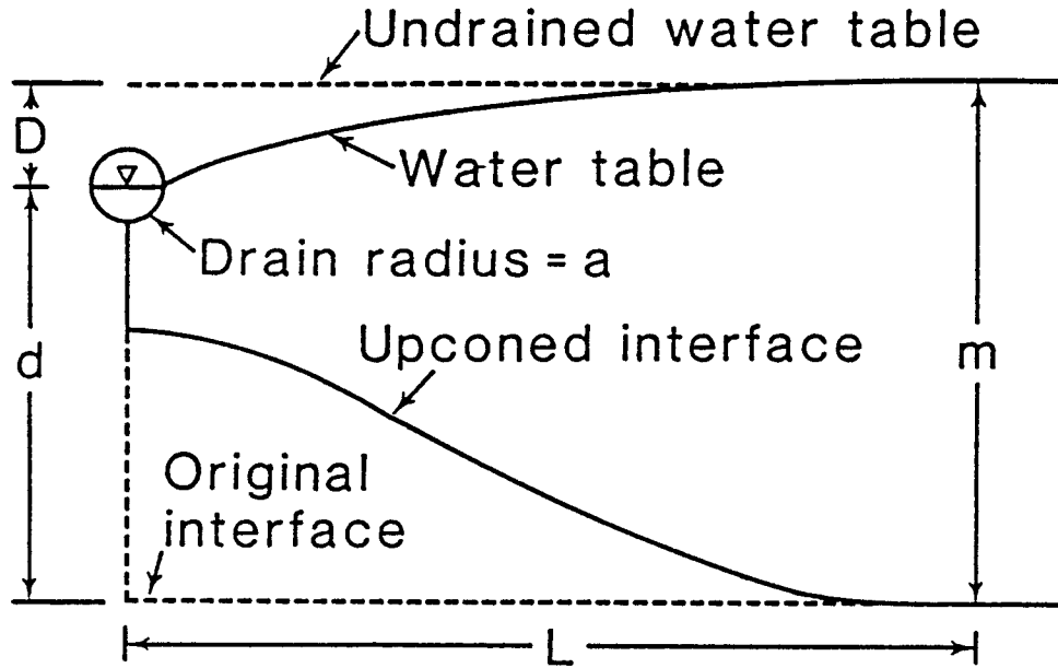
a. Flow toward a drain
