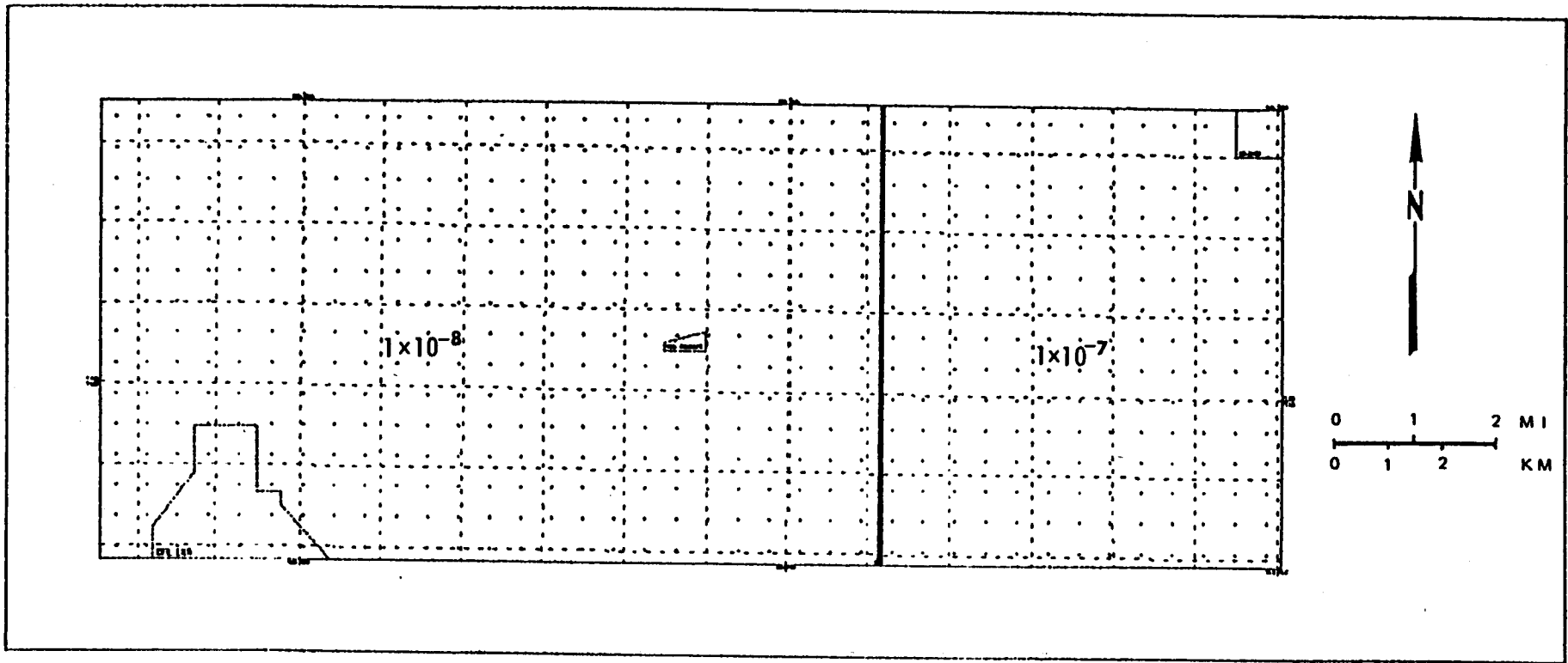
Figure II-9. Confining bed hydraulic conductivity (ft/sec) for the intuitively calibrated model.
