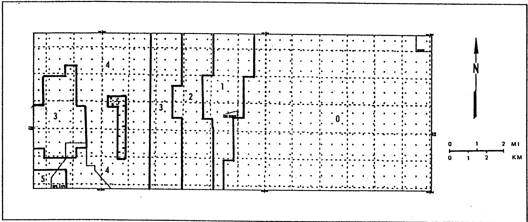
Figure II-13. Drawdown Case I, Test 2 for the intuitively calibrated model.
