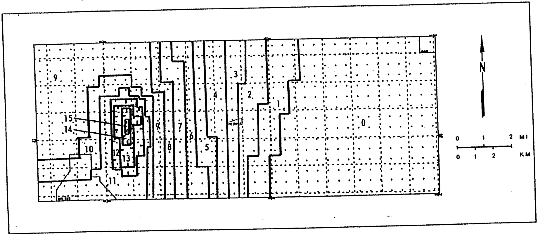
Figure II-14. Drawdown Case I, Test 5 for the intuitively calibrated model.
