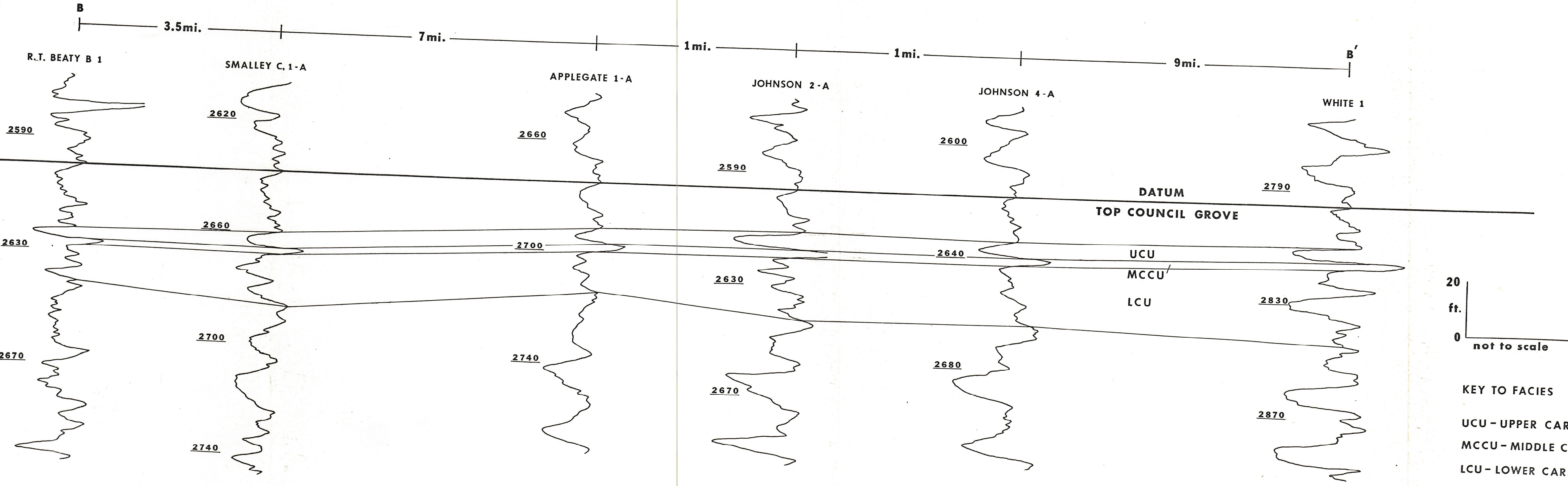
FIGURE 7 - STRATIGRAPHIC CROSS SECTION B - B' ALL LOGS GAMMA RAY
