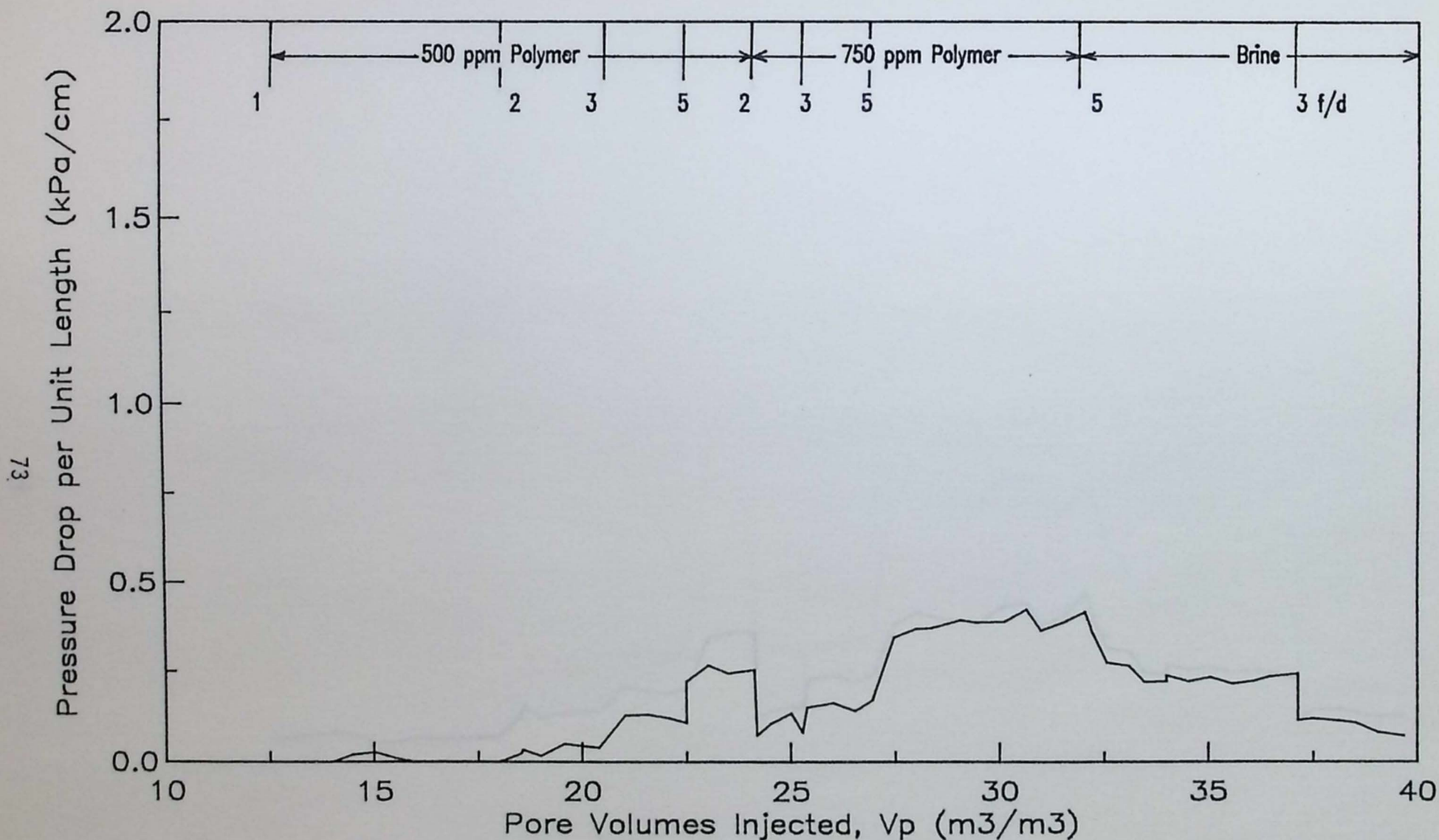
FIGURE 4.2 A PRESSURE GRADIENT ACROSS FRONT FACE OF BAKER DOLOMITE CORE FOR FLOOD BAK5 DURING POLYMER AND BRINE FLOW (BETZ 1160 IN BROOKS SYNTHETIC BRINE)
