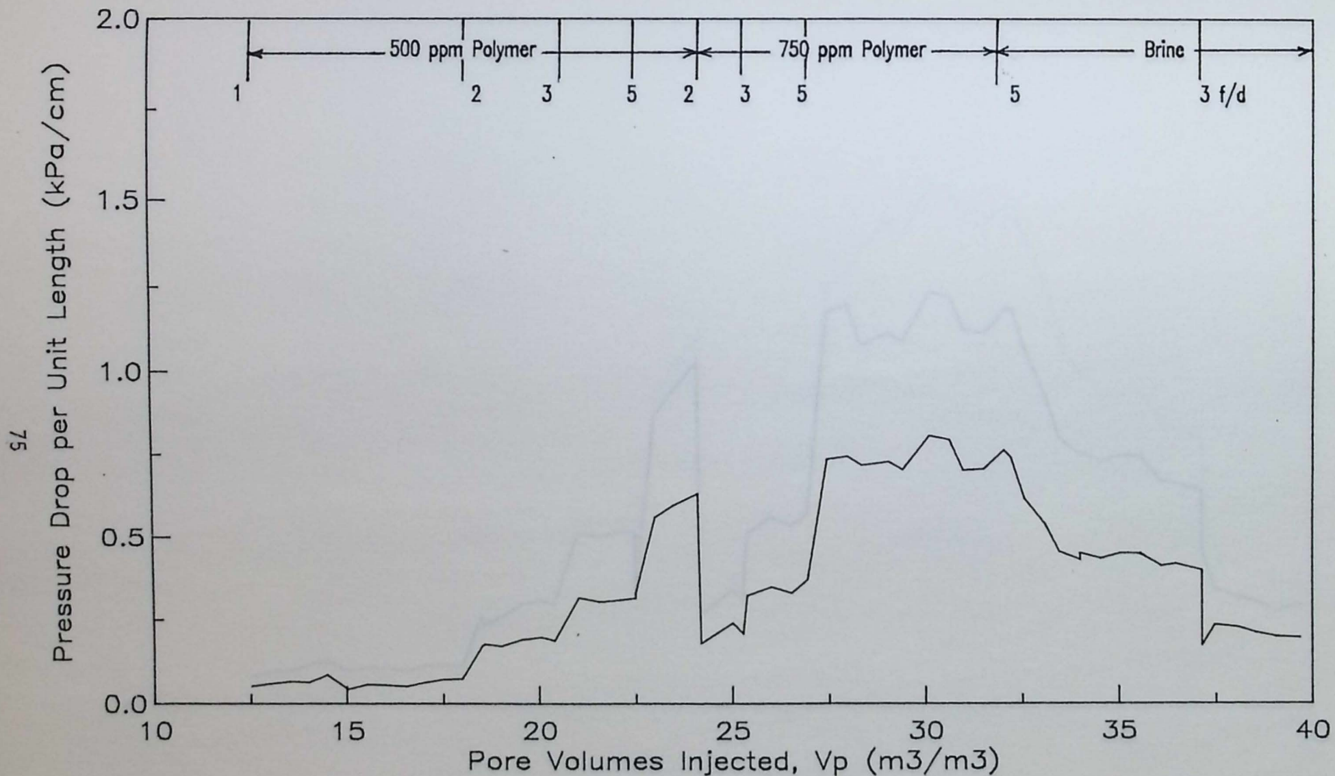
FIGURE 4.2c PRESSURE GRADIENT ACROSS SECTION 2 OF BAKER DOLOMITE CORE FOR FLOOD BAK5 DURING POLYMER AND BRINE FLOW (BETZ 1160 IN BROOKS SYNTHETIC BRINE)
