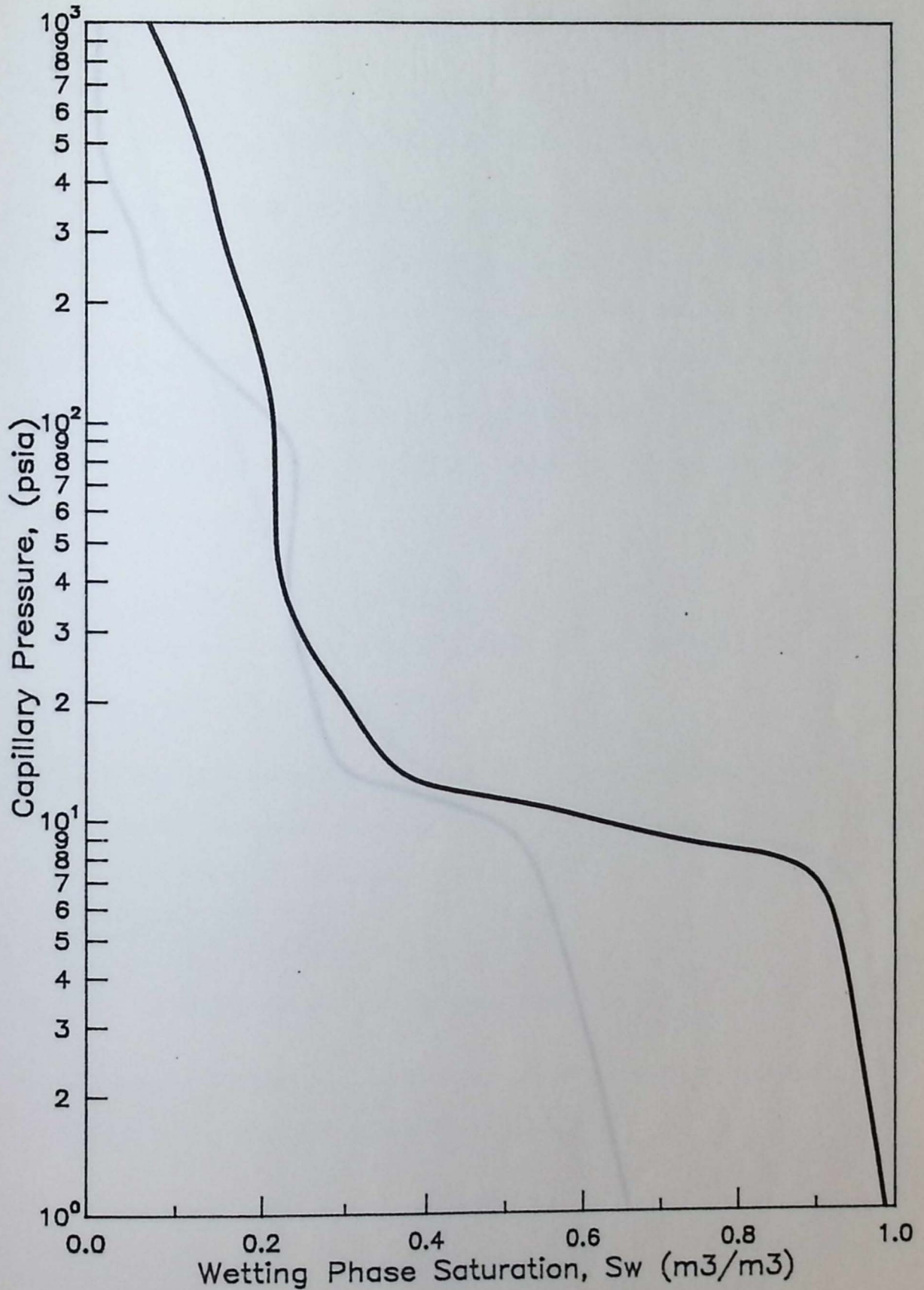
FIGURE 4.12 CAPILLARY PRESSURE CURVE FOR SOU1 CORE
