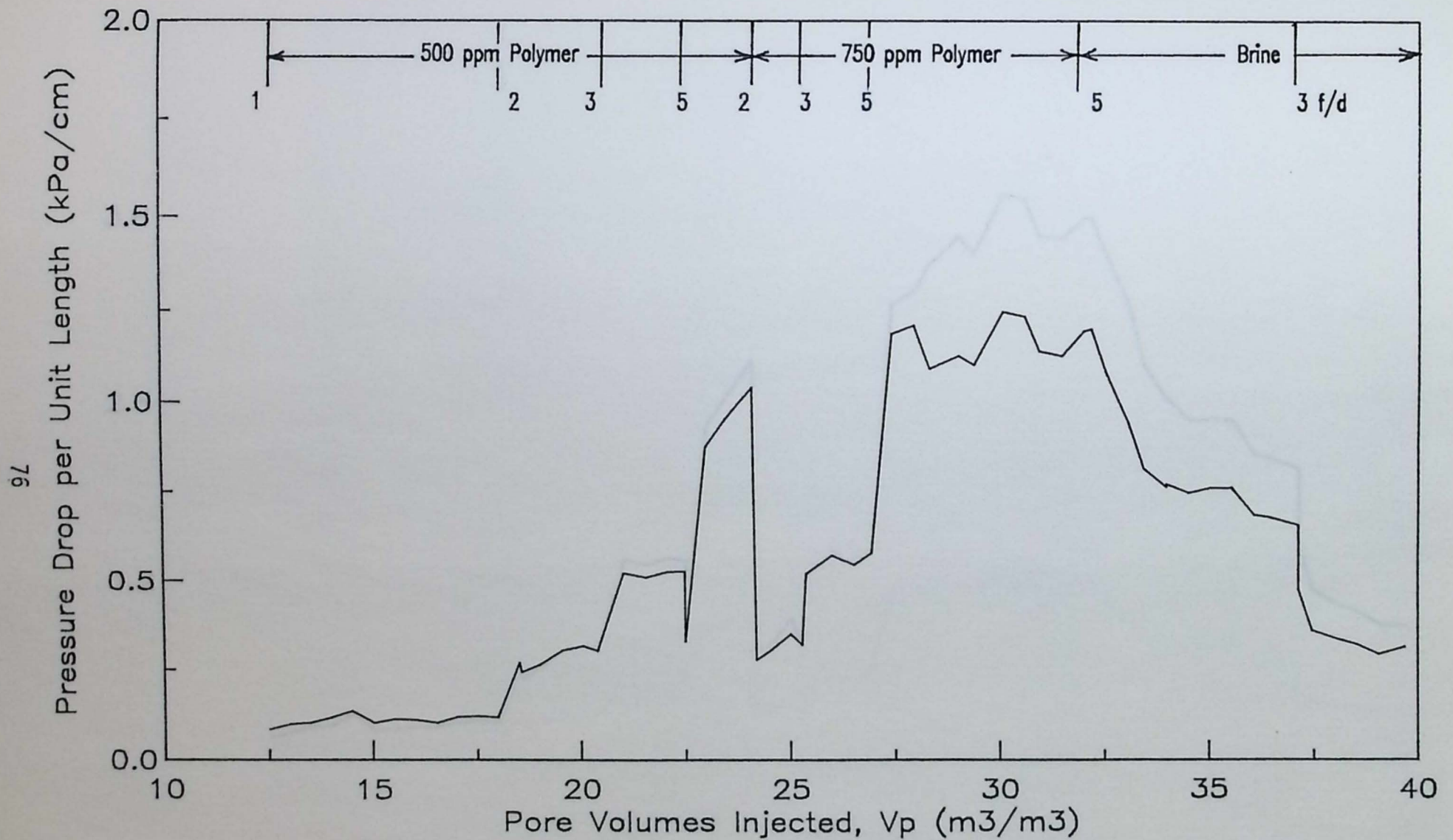
FIGURE 4.2D PRESSURE GRADIENT ACROSS SECTION 3 OF BAKER DOLOMITE CORE FOR FLOOD BAK5 DURING POLYMER AND BRINE FLOW (BETZ 1160 IN BROOKS SYNTHETIC BRINE)
