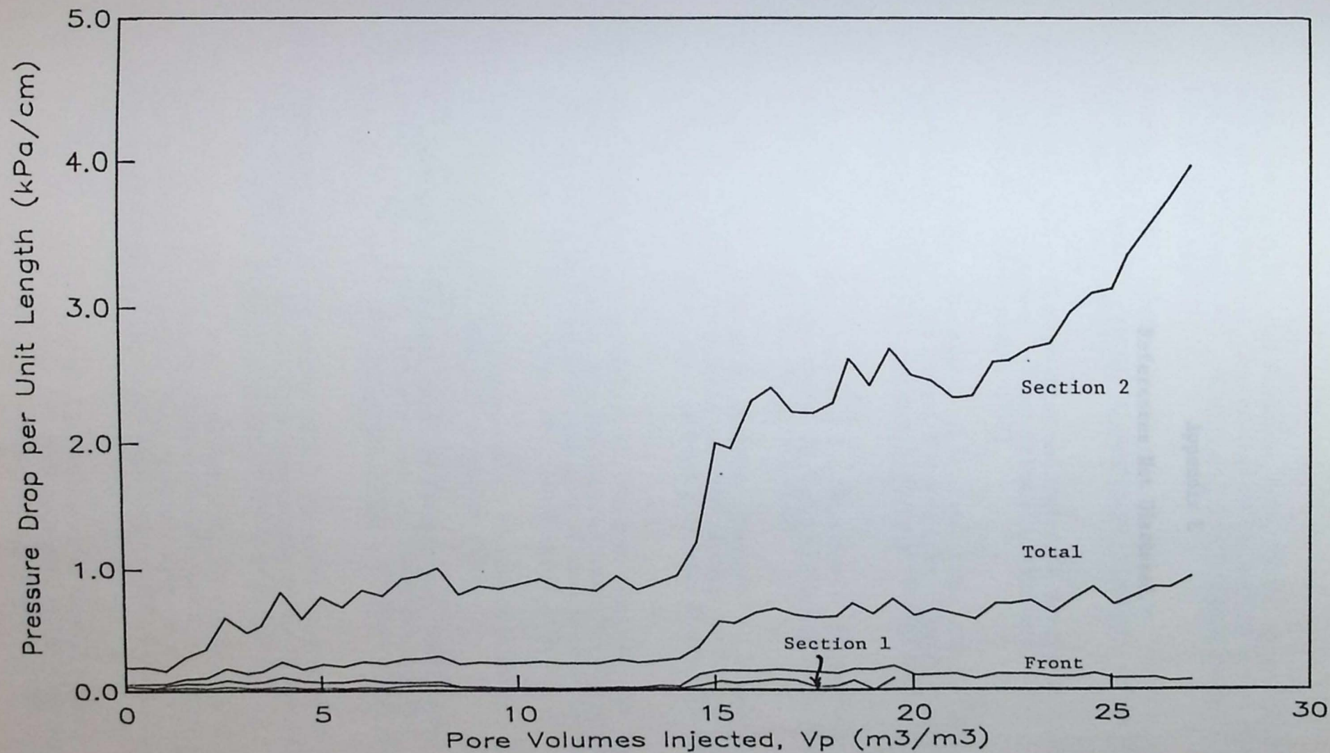
FIGURE D-1 PRESSURE GRADIENT ACROSS SECTIONS AND TOTAL CORE LENGTH FOR DENK1 FLOOD (BETZ 1160 IN BROOKS SYNTHETIC BRINE)
