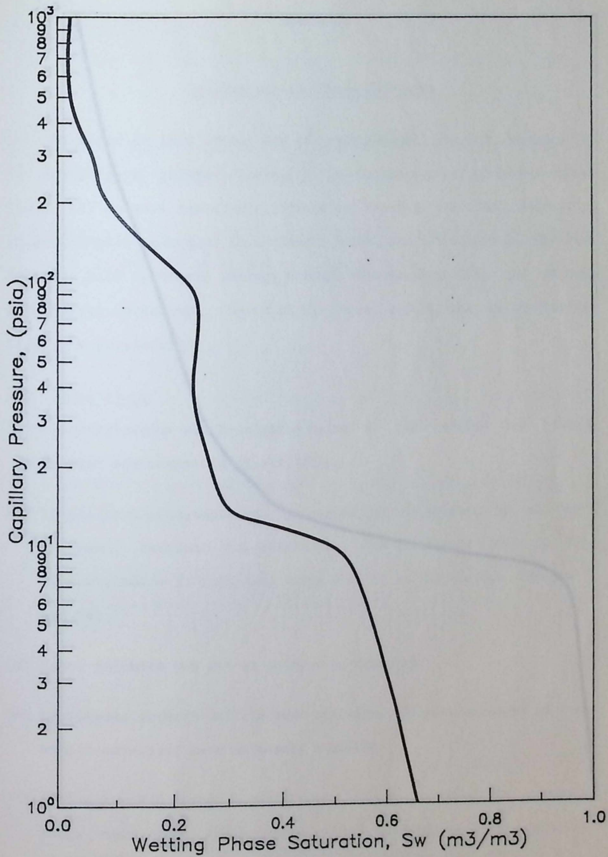
FIGURE 4.13 CAPILLARY PRESSURE CURVE FOR BAK7 CORE
