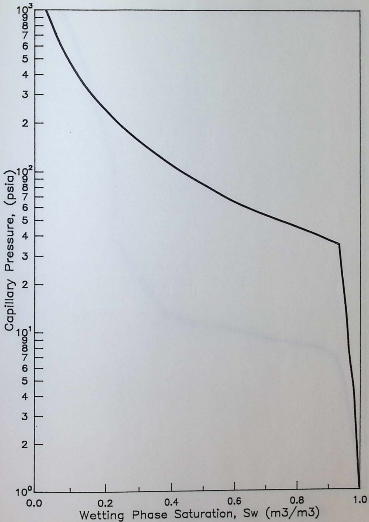
FIGURE 4.11 CAPILLARY PRESSURE CURVE FOR HUSK1 CORE
