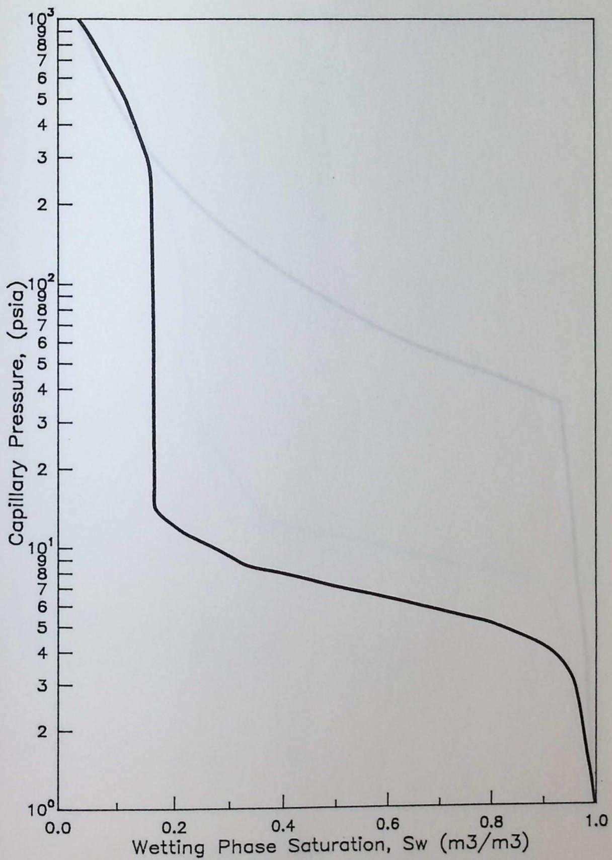
FIGURE 4.10 CAPILLARY PRESSURE CURVE FOR DENK2 CORE
