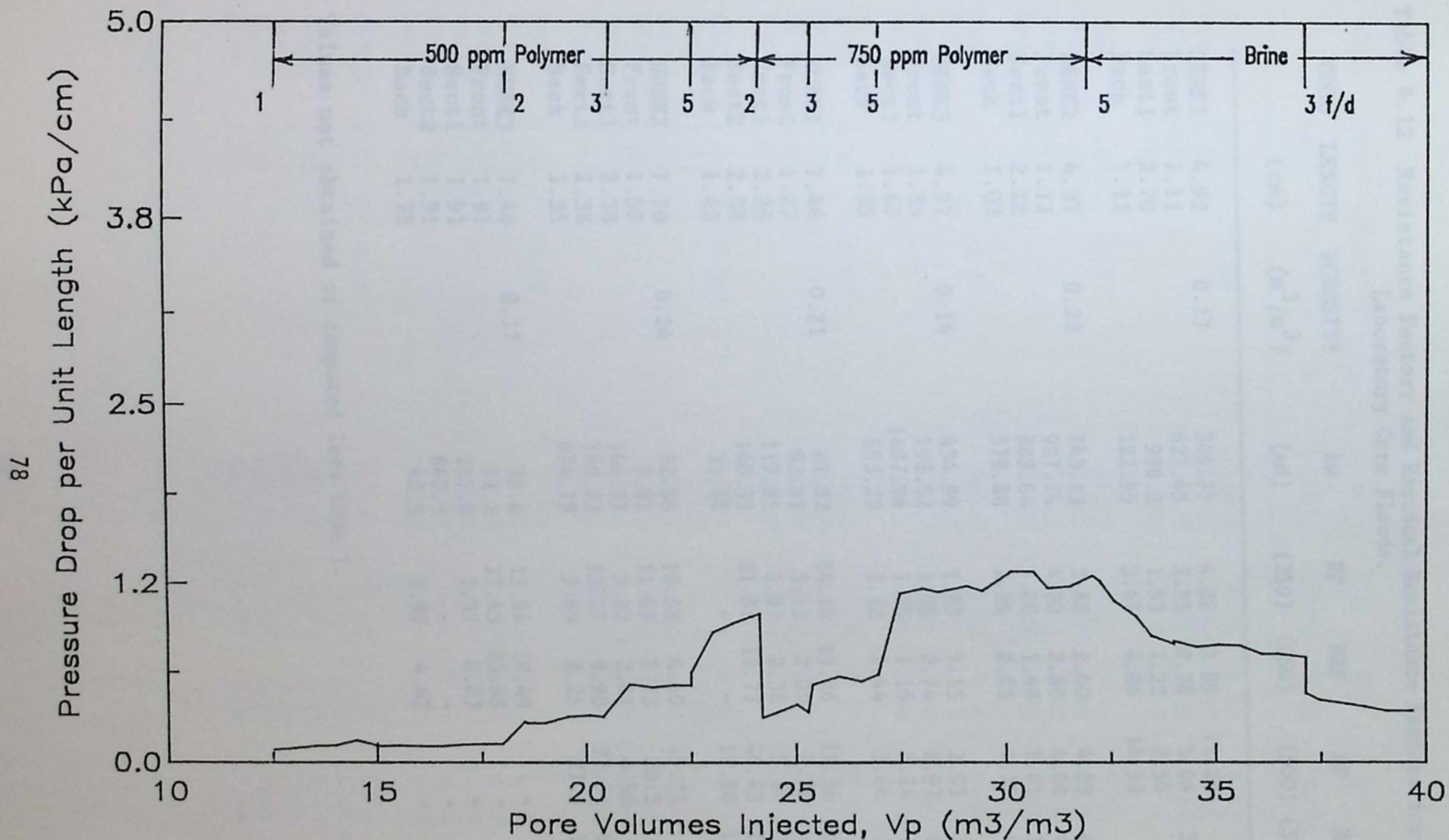
FIGURE 4.2 F PRESSURE GRADIENT ACROSS TOTAL BAKER DOLOMITE CORE FOR FLOOD BAK5 DURING POLYMER AND BRINE FLOW (BETZ 1160 IN BROOKS SYNTHETIC BRINE)
