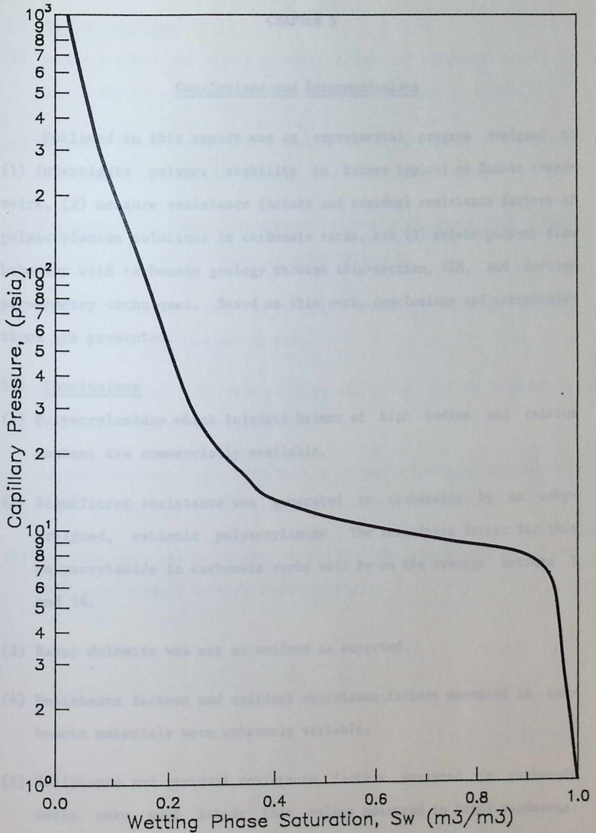
FIGURE 4.14 CAPILLARY PRESSURE CURVE FOR BEREA SANDSTONE
