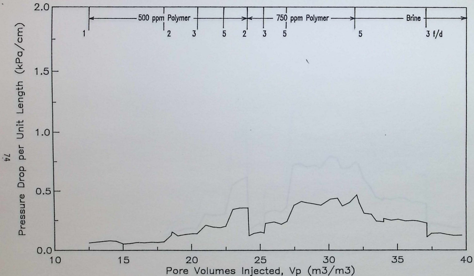
FIGURE 4.2 B PRESSURE GRADIENT ACROSS SECTION 1 OF BAKER DOLOMITE CORE FOR FLOOD BAK5 DURING POLYMER AND BRINE FLOW (BETZ 1160 IN BROOKS SYNTHETIC BRINE)
