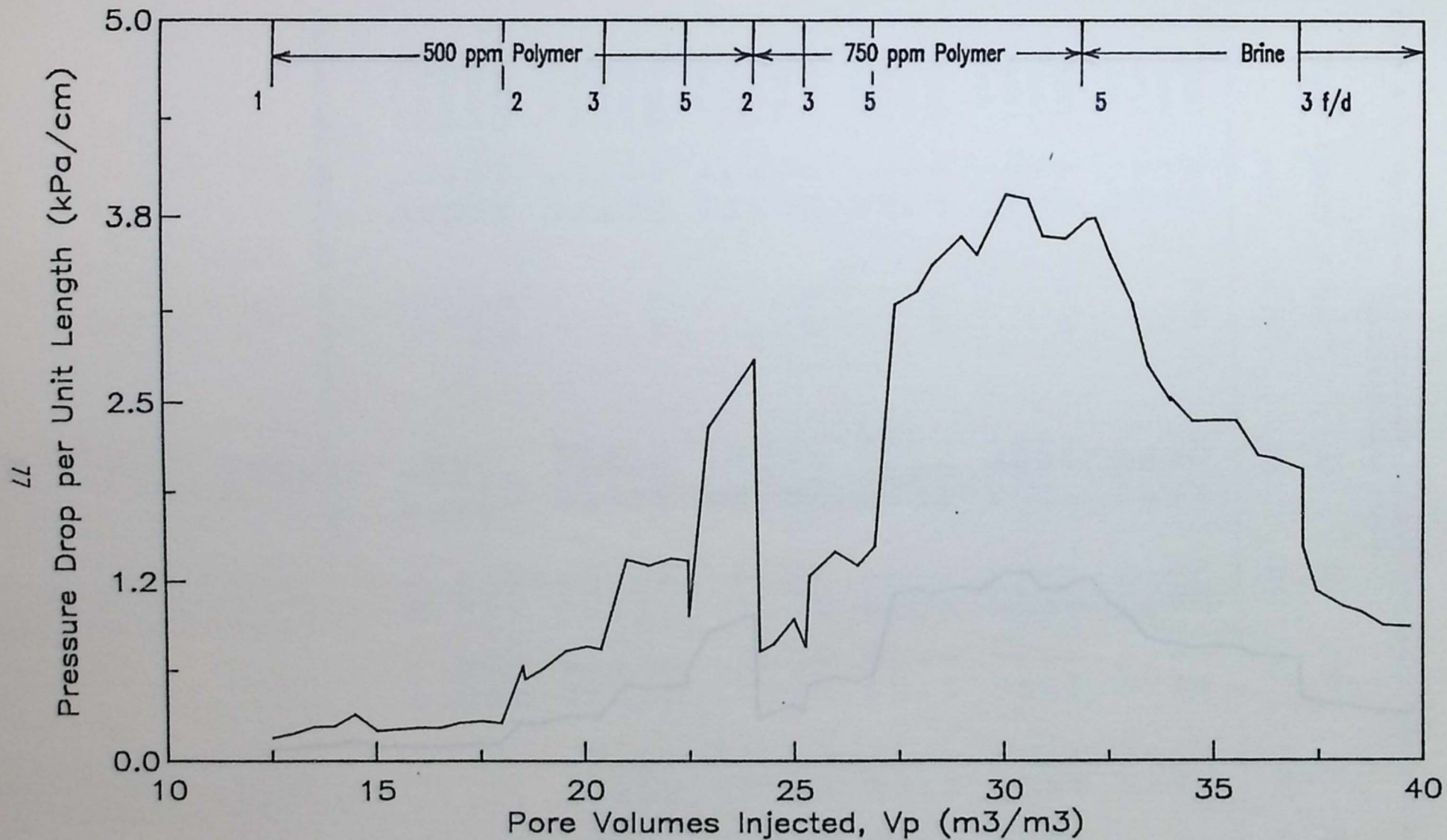
FIGURE 4.2 E PRESSURE GRADIENT ACROSS BACK FACE OF BAKER DOLOMITE CORE FOR FLOOD BAK5 DURING POLYMER AND BRINE FLOW (BETZ 1160 IN BROOKS SYNTHETIC BRINE)
