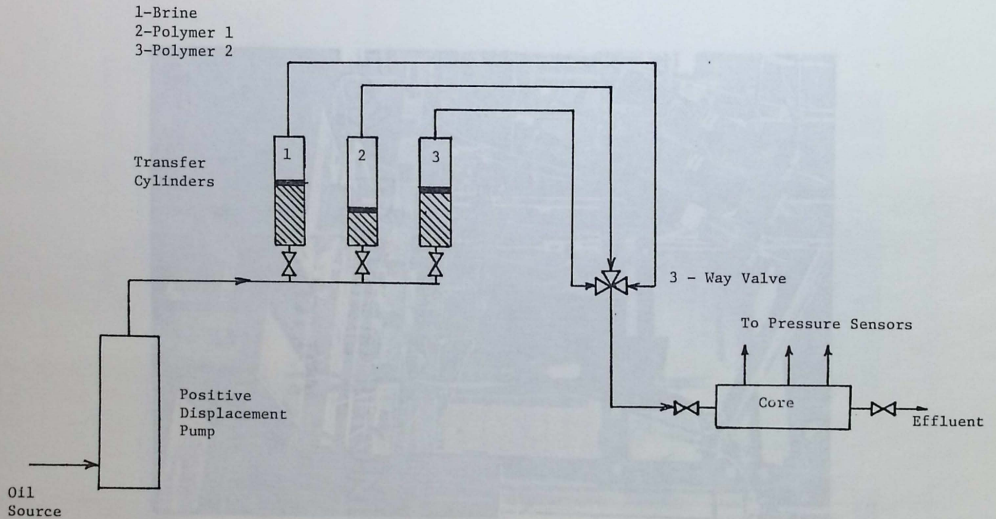
Figure 3.2 Schematic Diagram of Laboratory Core Flood Apparatus.
