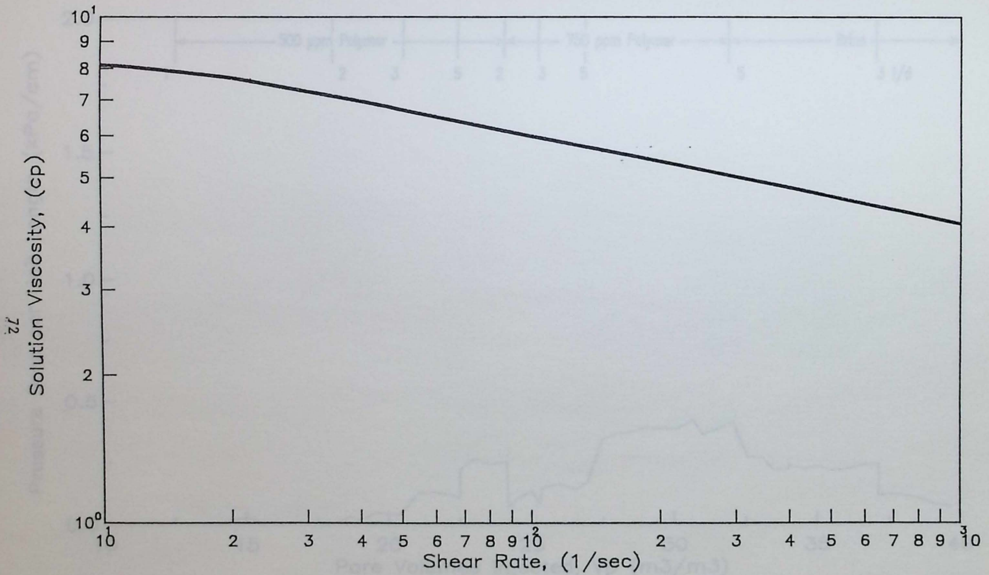
FIGURE 4.1 SHEAR RATE DEPENDENCY OF 2000 BETZ POLYMER 1160 IN BROOKS SYNTHETIC BRINE
