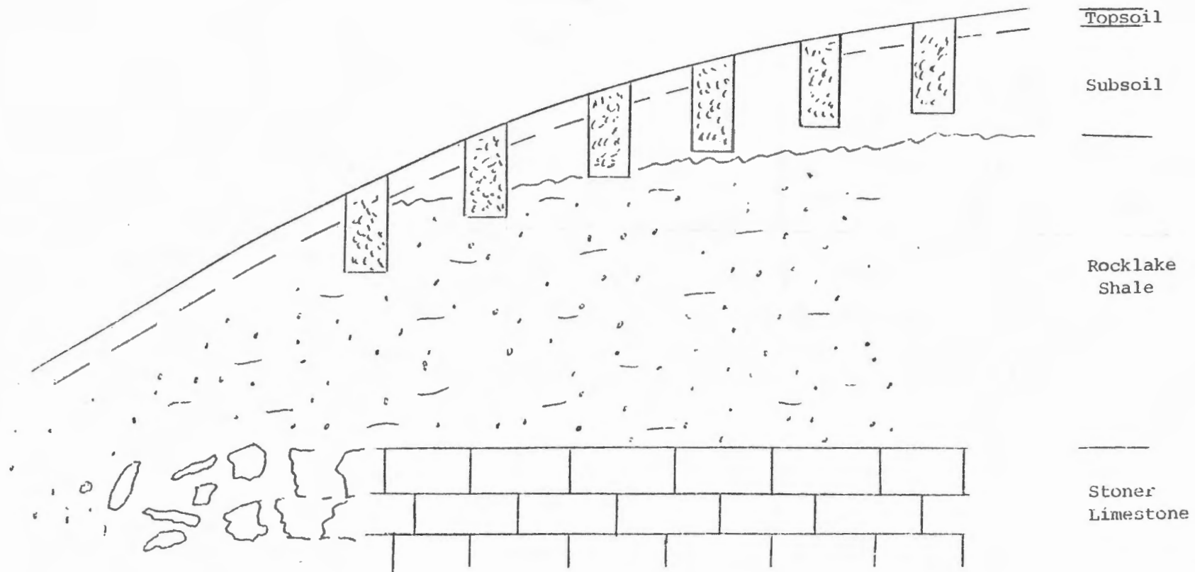
FIGURE 3 Cross-Section of the Waste Disposal Site (Diagram not to scale)
