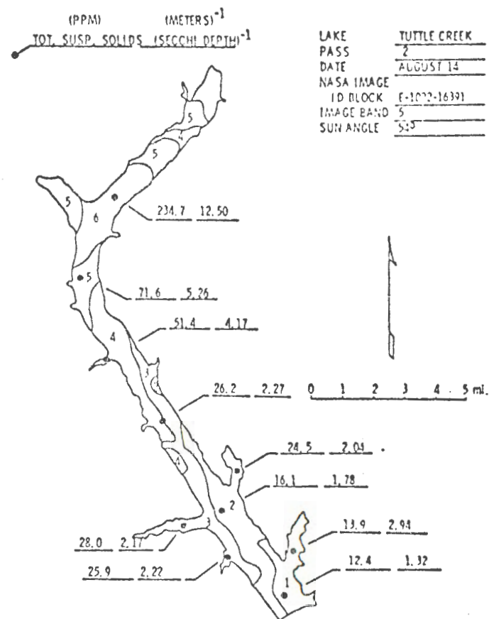
Figure 47. Tuttle Creek Reservoir Gray Levels, 14 August 1972, MSS 5 (IDECs Analysis of NASA Image: ERTS E-1022-16391-5 01)
