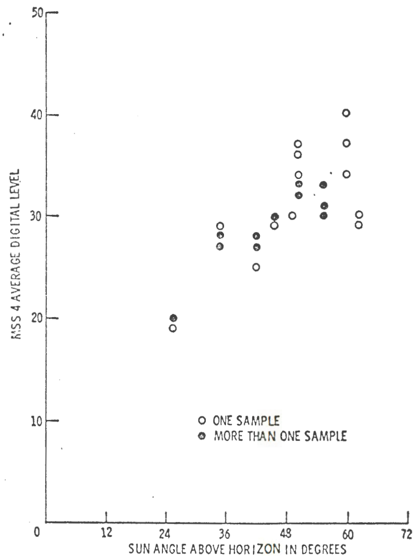
FIGURE 16. MSS 4 CCT DIGITAL LEVEL VS. SUN ANGLE FOR SAMPLES BETWEEN 25 AND 45 PPM IN FIG. 9.
