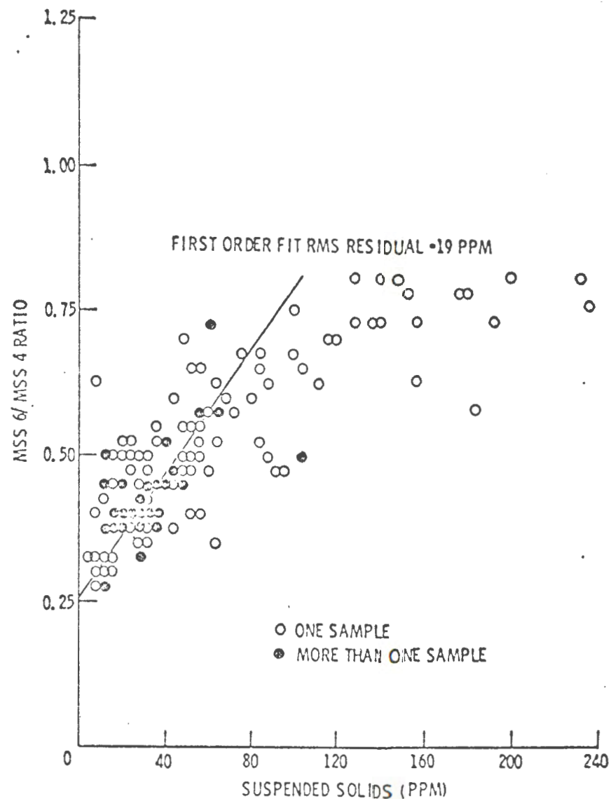
FIGURE 14. MSS 6/MSS 4 CCT RATIO VS. SUSPENDED SOLIDS FOR 166 WATER SAMPLES TAKEN FROM 3 KANSAS RESERVOIRS DURING 13 DIFFERENT ERTS-1 CYCLES.
