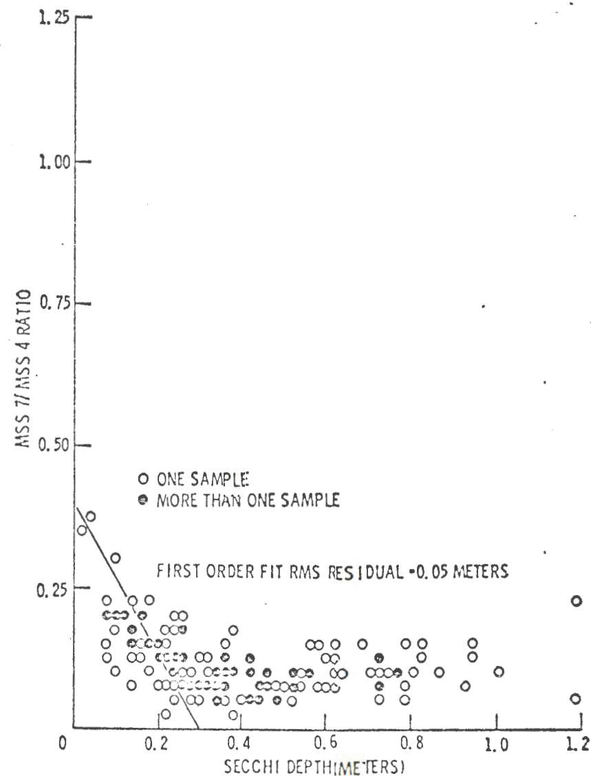
FIGURE 28. MSS 7/MSS 4 CCT RATIO VS. SECCHI DEPTH FOR 171 WATER SAMPLES TAKEN FROM 3 KANSAS RESERVOIRS DURING 13 DIFFERENT ERTS-1 CYCLES.
