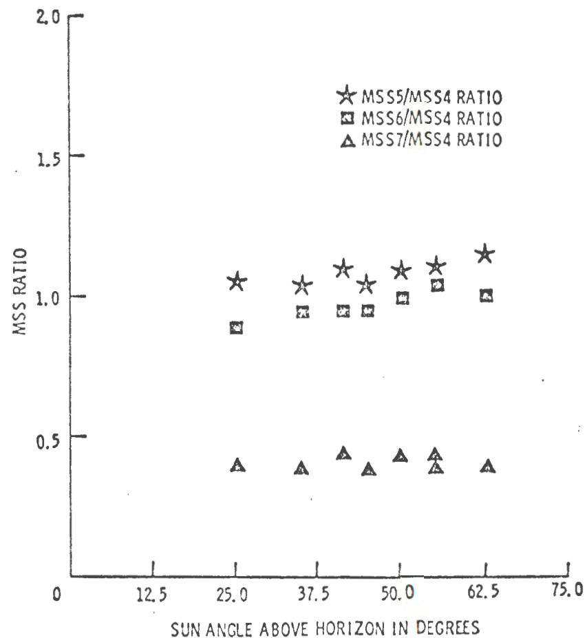
FIGURE 6. MSS BAND RATIOS FROM CCT VS. SUN ANGLE FOR TUTTLE CREEK CONCRETE DAM.
