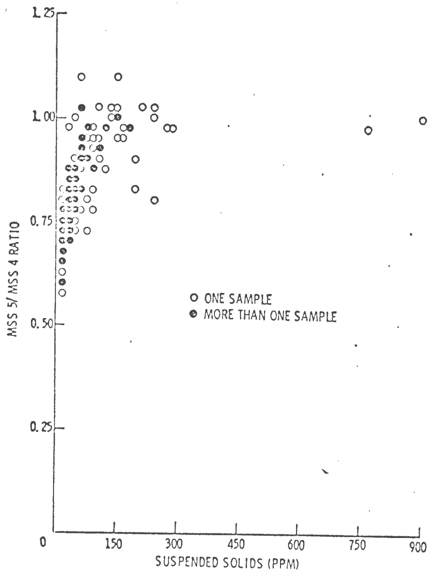
FIGURE 19. MSS 5/MSS 4 CCT RATIO VS. SUSPENDED SOLIDS FOR 171 WATER SAMPLES TAKEN FROM 3 KANSAS RESERVOIRS DURING 13 DIFFERENT ERTS-1 CYCLES.
