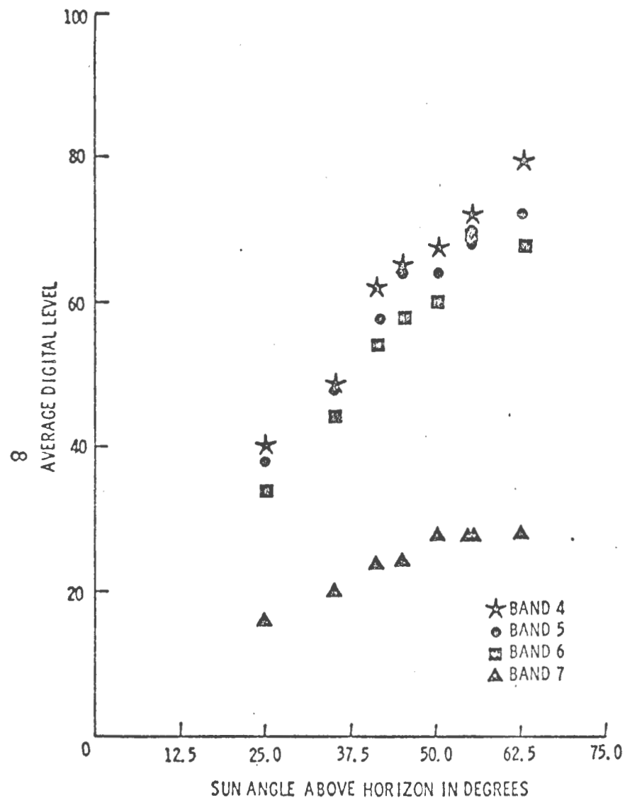
FIGURE 5. MSS DIGITAL LEVELS FROM CCT VS. SUN ANGLE FOR TUTTLE CREEK CONCRETE DAM.
