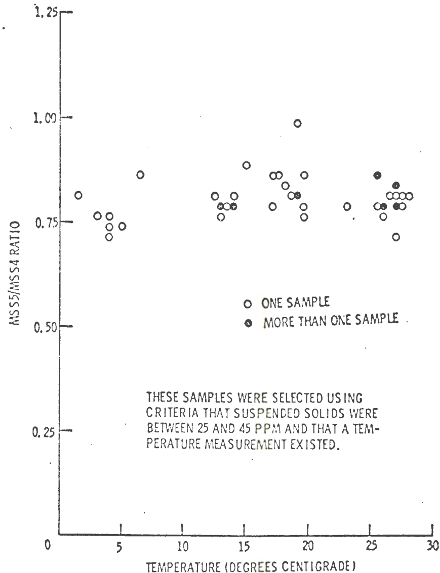
FIGURE 31. MSS 5/MSS 4 CCT RATIO VS. TEMPERATURE FOR 44 SAMPLES TAKEN FROM 2 KANSAS RESERVOIRS OVER A 13 MONTH PERIOD.
