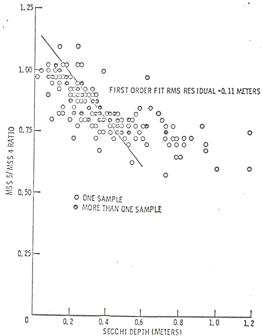
FIGURE 26. MSS 5/MSS 4 CCT RATIO VS. SECCHI DEPTH FOR 171 WATER SAMPLES TAKEN FROM 3 KANSAS RESERVOIRS DURING 13 DIFFERENT ERTS-1 CYCLES.
