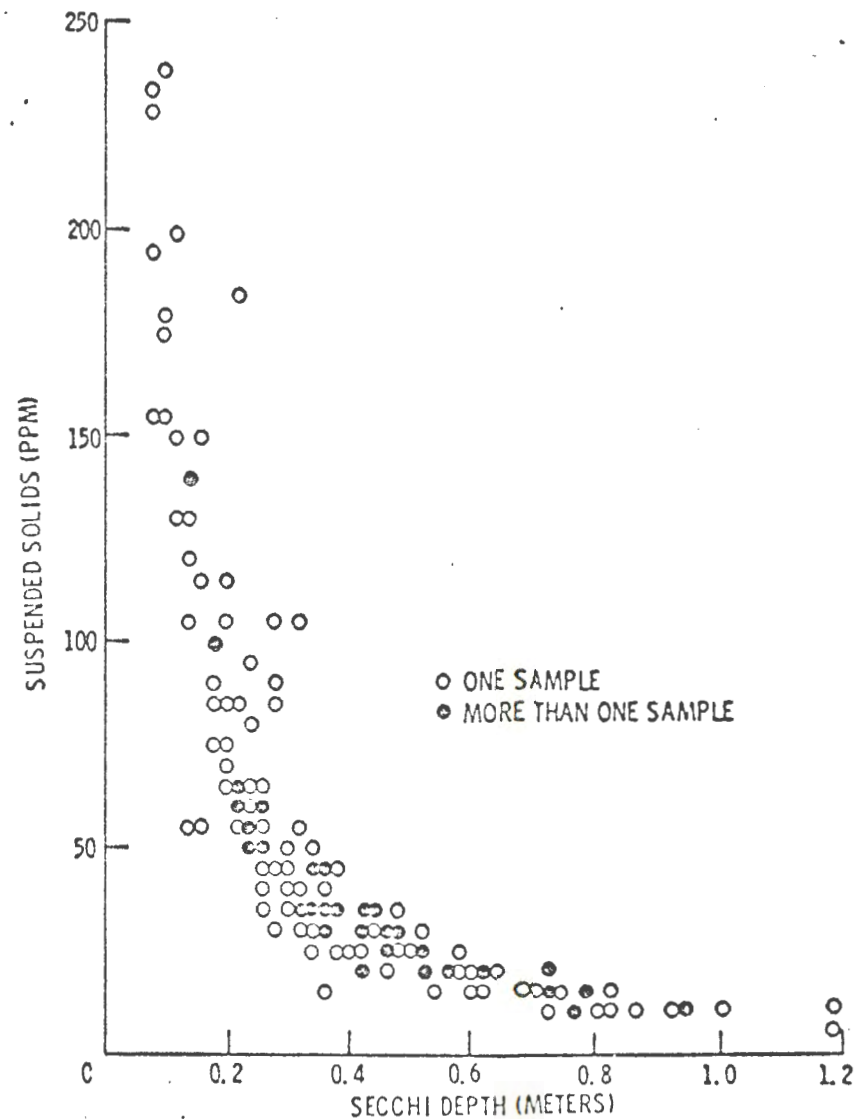
FIGURE 24. SUSPENDED SOLIDS VS. SECCHI DEPTH FOR 168 WATER SAMPLES TAKEN FROM 3 KANSAS RESERVOIRS DURING 13 DIFFERENT ERTS-1 CYCLES.
