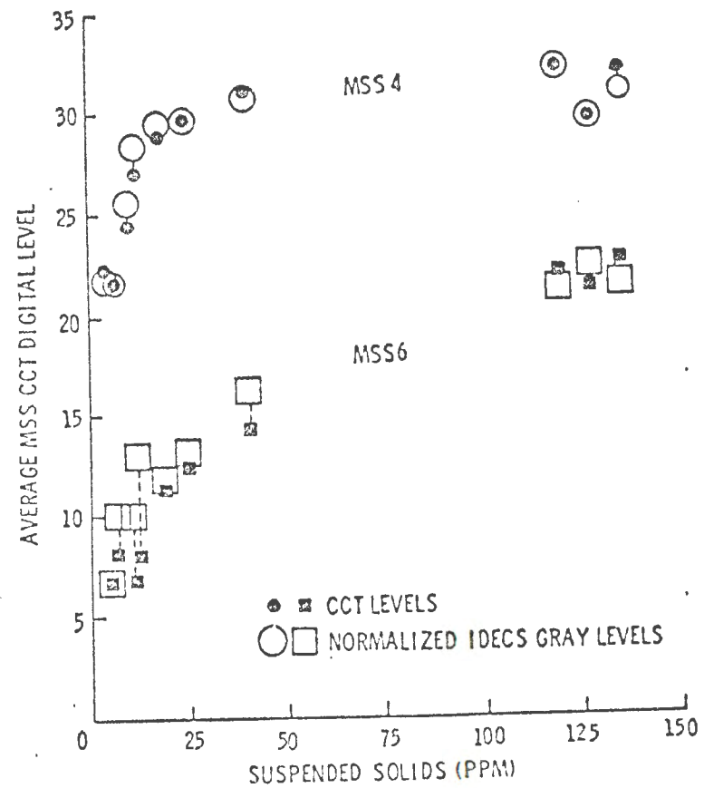
FIGURE 49. COMPARISON OF CCT LEVELS WITH IDECS LEVELS FOR PERRY, ERTS CYCLE 2.
