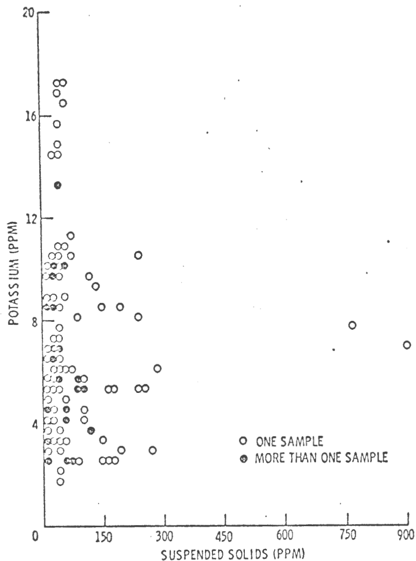
FIGURE 44. POTASSIUM [K] VS. SUSPENDED SOLIDS FOR 140 SAMPLES TAKEN FROM 2 KANSAS RESERVOIRS OVER A 13 MONTH PERIOD.
