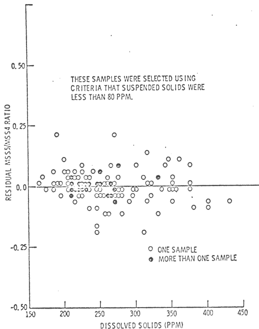
FIGURE 36. RESIDUAL MSS 5/MSS 4 CCT RATIO VS. DISSOLVED SOLIDS FOR 133 SAMPLES TAKEN FROM 3 RESERVOIRS OVER A 13 MONTH PERIOD. RESIDUAL WAS OBTAINED BY SUBTRACTING LINEAR DEPENDENCE ON SUSPENDED SOLIDS.
