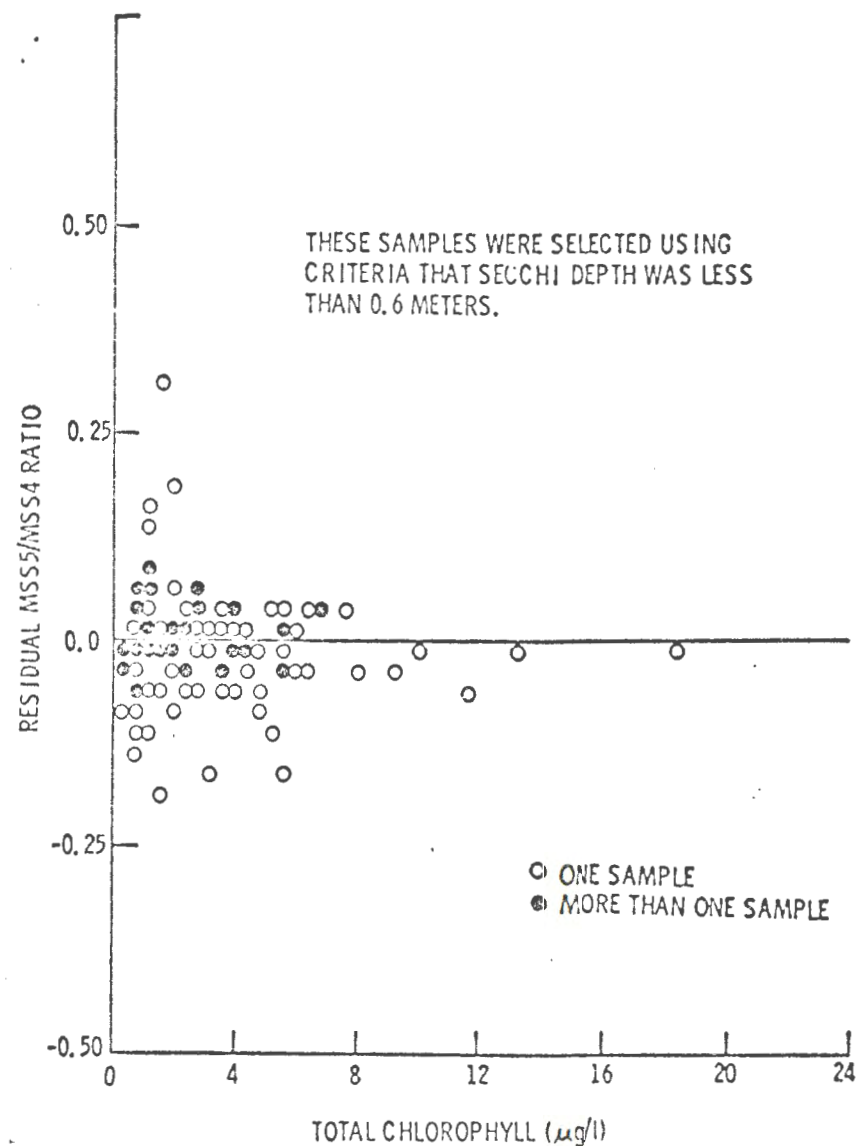
FIGURE 43. RESIDUAL MSS 5/MSS 4 CCT RATIO VS. TOTAL CHLOROPHYLL FOR 114 SAMPLES TAKEN FROM 2 KANSAS RESERVOIRS OVER A 13 MONTH PERIOD. RESIDUAL WAS OBTAINED BY SUBTRACTING LINEAR DEPENDENCE ON SECCHI DEPTH.
