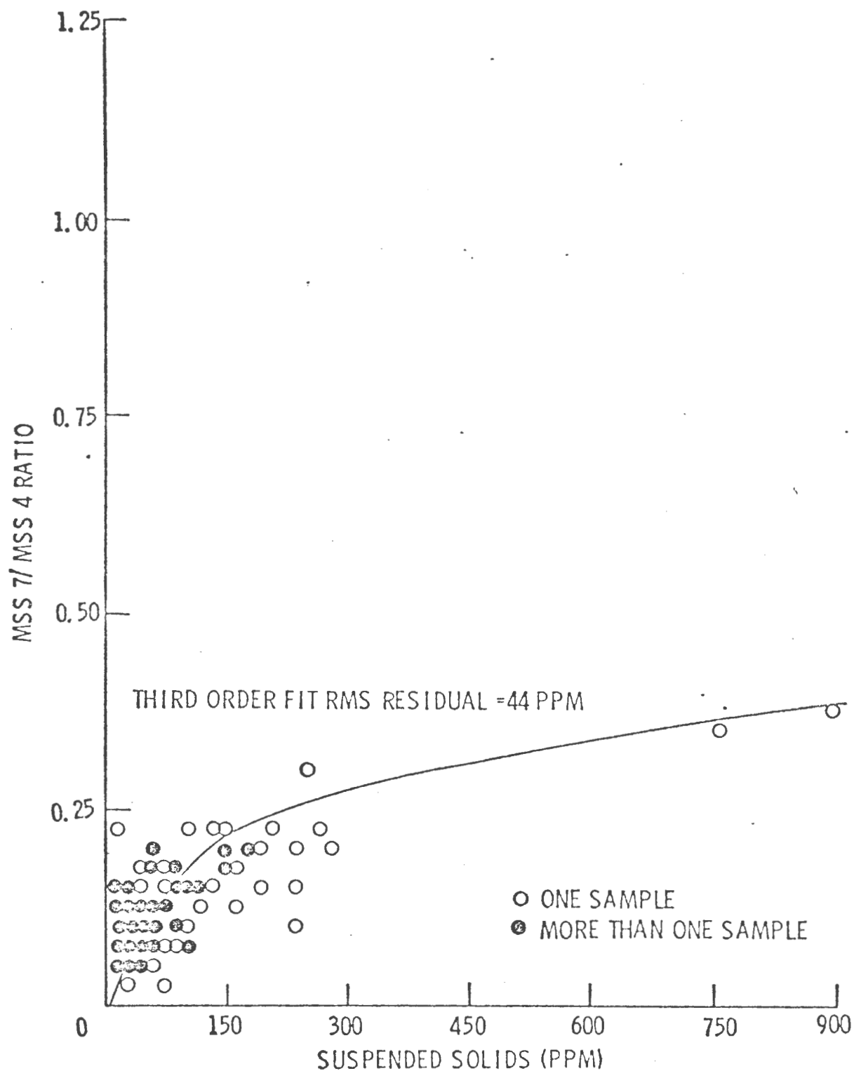
FIGURE 21. MSS 7/MSS 4 CCT RATIO VS. SUSPENDED SOLIDS FOR 171 WATER SAMPLES TAKEN FROM 3 KANSAS RESERVOIRS DURING 13 DIFFERENT ERTS-1 CYCLES.
