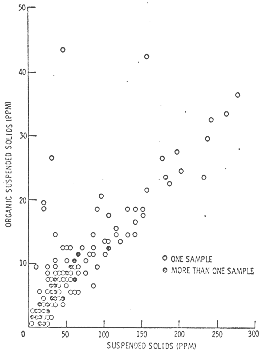
FIGURE 32. ORGANIC SUSPENDED SOLIDS VS. SUSPENDED SOLIDS FOR 120 WATER SAMPLES TAKEN FROM 3 KANSAS RESERVOIRS OVER A 13 MONTH PERIOD.
