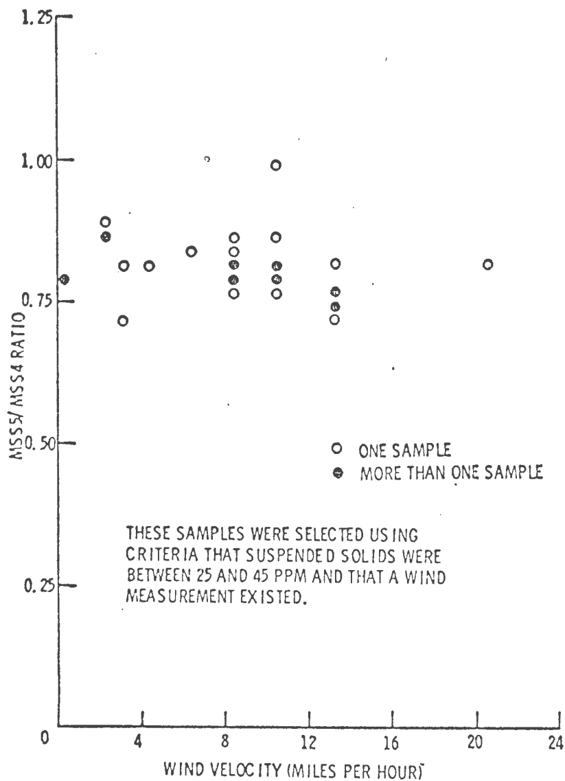
FIGURE 30. MSS 5/MSS 4 CCT RATIO VS. WIND VELOCITY FOR 35 SAMPLES TAKEN FROM 2 KANSAS RESERVOIRS OVER A 13 MONTH PERIOD.
