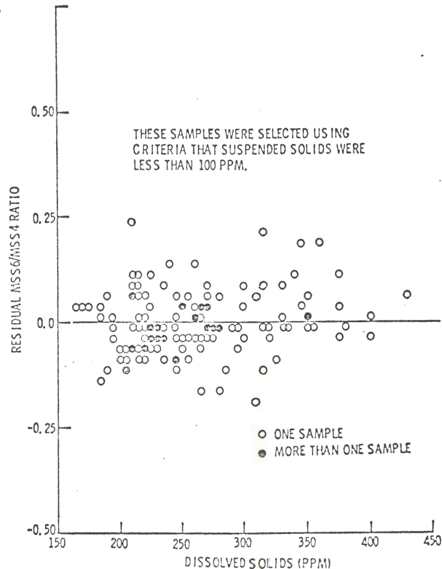
FIGURE 37. RESIDUAL MSS 6/MSS 4 CCT RATIO VS. DISSOLVED SOLIDS FOR 141 SAMPLES TAKEN FROM 3 KANSAS RESERVOIRS OVER A 13 MONTH PERIOD. RESIDUAL WAS OBTAINED BY SUBTRACTING LINEAR DEPENDENCE ON SUSPENDED SOLIDS.
