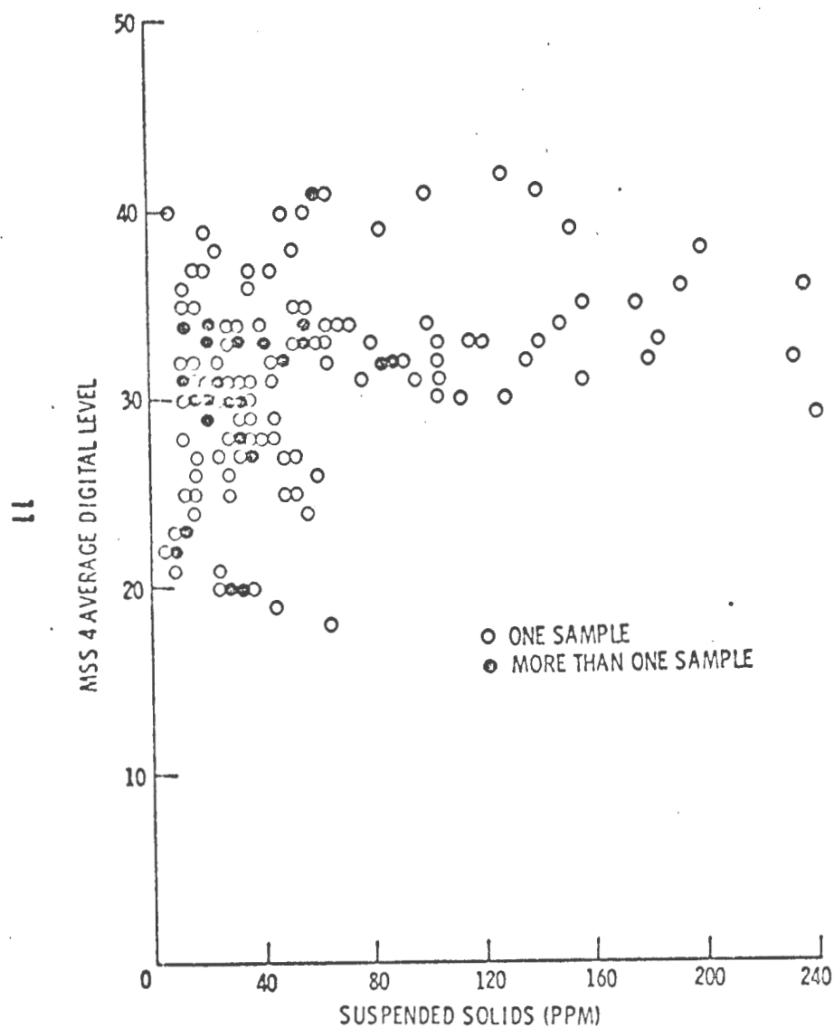
FIGURE 9. MSS 4 CCT DIGITAL LEVEL VS. SUSPENDED SOLIDS FOR 166 WATER SAMPLES TAKEN FROM 3 KANSAS RESERVOIRS DURING 13 DIFFERENT ERTS-1 CYCLES.
