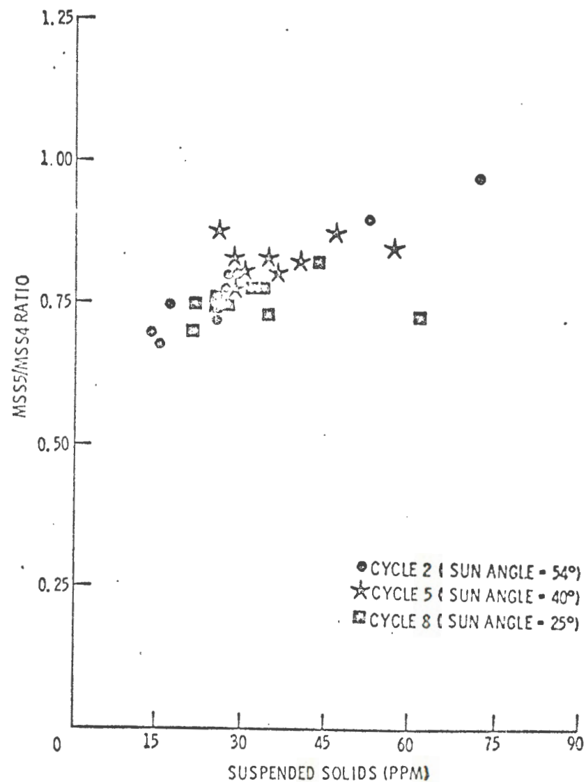
FIGURE 8. MSS5/MSS4 RATIO FROM CCT VS. SUSPENDED SOLIDS FOR 28 WATER SAMPLES FROM 3 ERTS-1 CYCLES.
