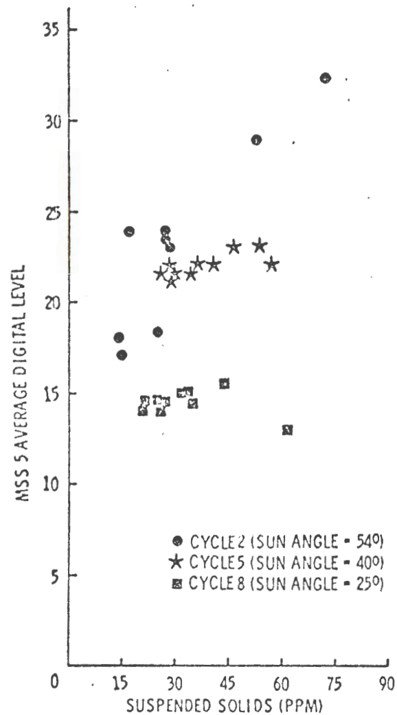
FIGURE 7. MSS5 DIGITAL LEVELS FROM CCT VS. SUSPENDED SOLIDS FOR 28 WATER SAMPLES FROM 3 ERTS-1 CYCLES.
