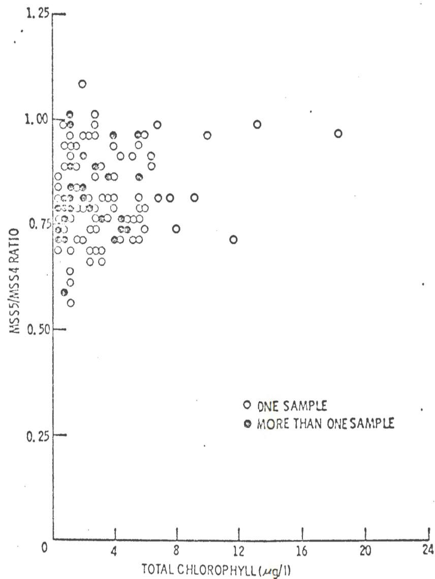
FIGURE 39. MSS 5/MSS 4 CCT RATIO VS. TOTAL CHLOROPHYLL FOR 140 SAMPLES TAKEN FROM 2 KANSAS RESERVOIRS OVER A 13 MONTH PERIOD.
