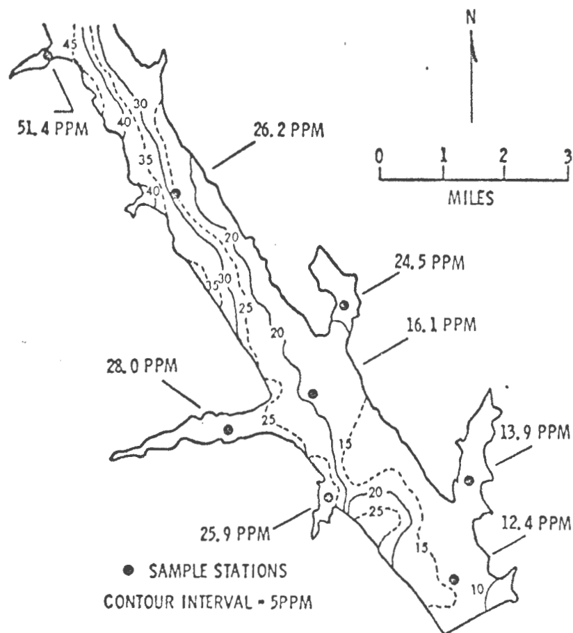
FIGURE 23. SUSPENDED SOLIDS CONTOUR MAP OF TUTTLE CREEK RESERVOIR (AUGUST 14, 1972 ERTS-1 ID NO. 1022-16391-5) DERIVED FROM CCTS (MSS 5) FOR 4 ERTS-1 PASSES.
