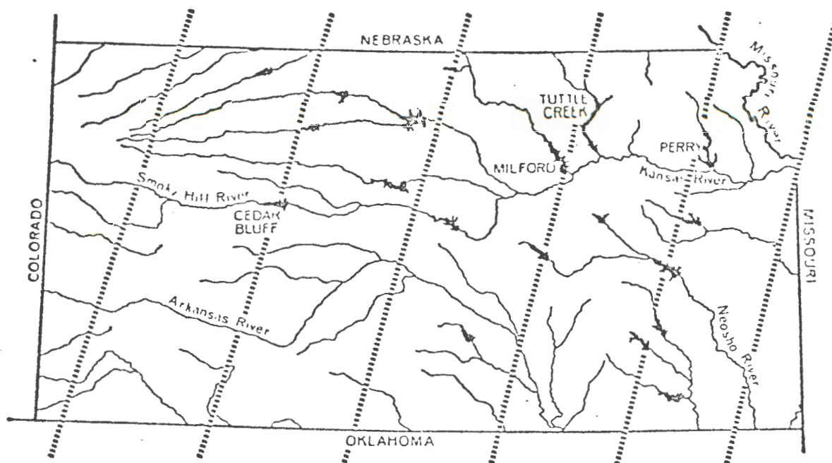
FIGURE 1. RESERVOIRS AND ERTS TRACKS IN KANSAS
