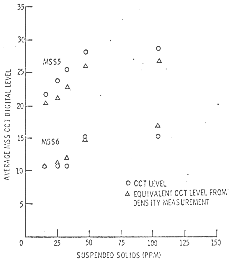
FIGURE 48. COMPARISON OF CCT DIGITAL LEVELS WITH IMAGE DENSITY MEASUREMENTS FOR TUTTLE CREEK RESERVOIR, ERTS CYCLE 4. DENSITY MEASUREMENTS WERE CONVERTED TO EQUIVALENT CCT LEVELS BY USING STEP WEDGE AT BOTTOM OF IMAGE.
