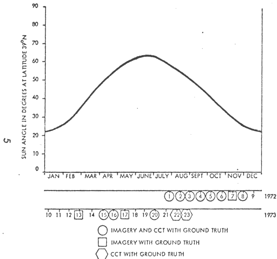
FIGURE 3. DATA ACQUISITION AS A FUNCTION OF TIME OF YEAR, SUN ANGLE, AND ERTS CYCLE NUMBER.
