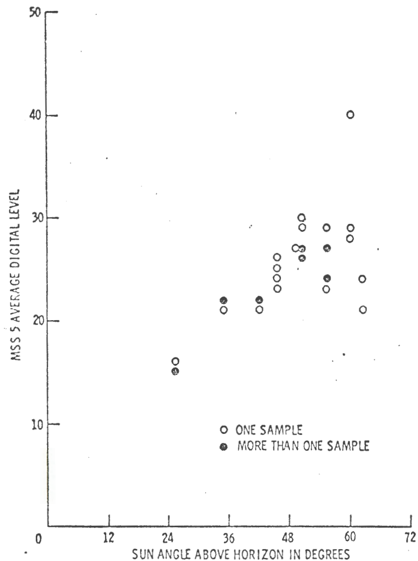
FIGURE 17. MSS 5 CCT DIGITAL LEVEL VS. SUN ANGLE FOR SAMPLES BETWEEN 25 AND 45 PPM IN FIG. 10.
