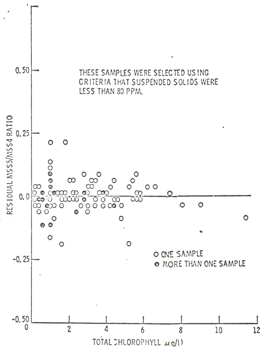
FIGURE 41. RESIDUAL MSS 5/MSS 4 CCT RATIO VS. TOTAL CHLOROPHYLL FOR 106 SAMPLES TAKEN FROM 2 KANSAS RESERVOIRS OVER A 13 MONTH PERIOD. RESIDUAL WAS OBTAINED BY SUBTRACTING LINEAR DEPENDENCE ON SUSPENDED SOLIDS.
