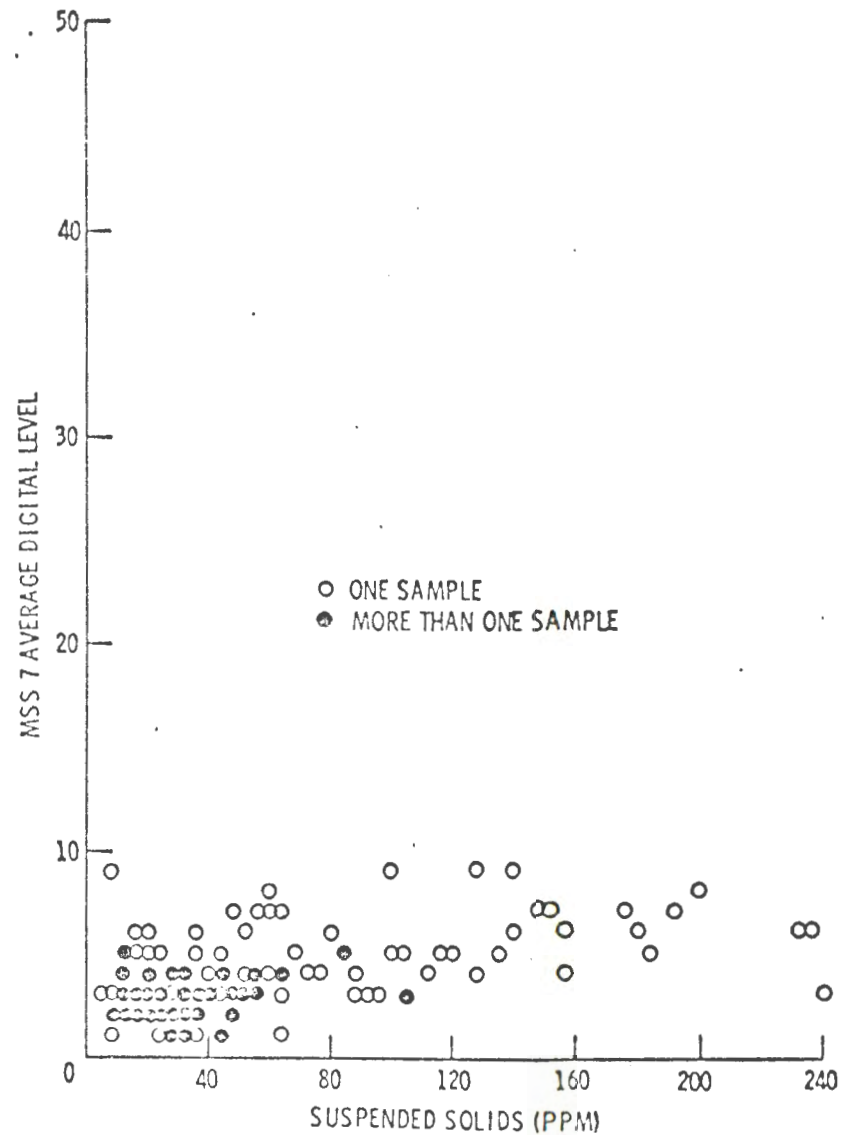
FIGURE 12. MSS 7 CCT DIGITAL LEVEL VS. SUSPENDED SOLIDS FOR 165 WATER SAMPLES TAKEN FROM 3 KANSAS RESERVOIRS DURING 13 DIFFERENT ERTS-1 CYCLES.
