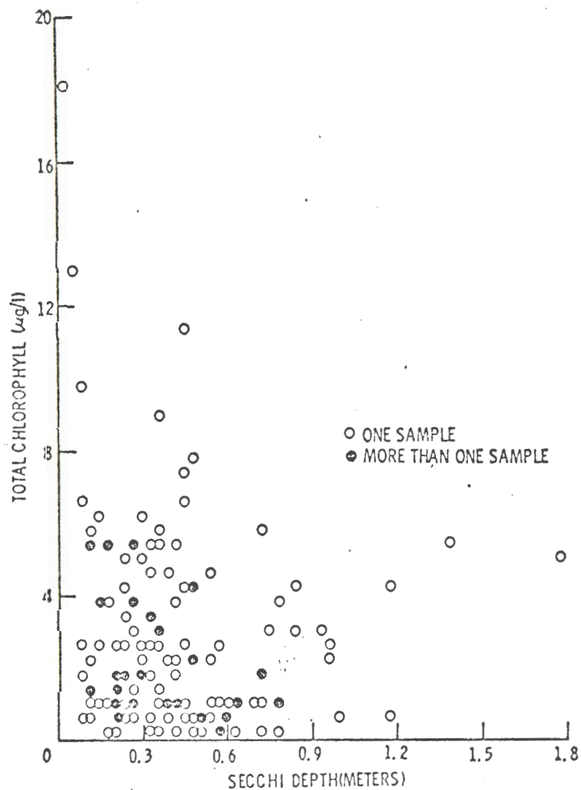
FIGURE 42. TOTAL CHLOROPHYLL VS. SECCHI DEPTH FOR 143 SAMPLES TAKEN FROM 2 KANSAS RESERVOIRS OVER A 13 MONTH PERIOD.
