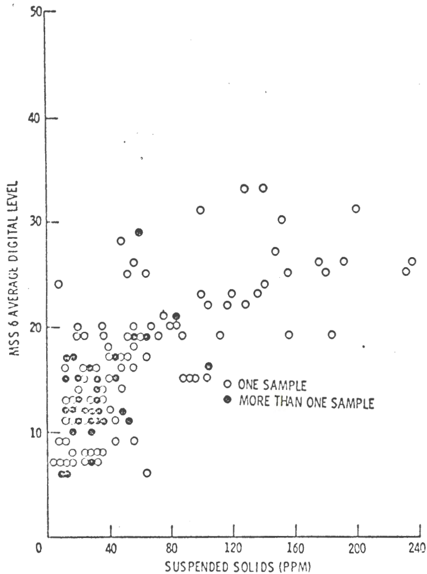
FIGURE 11. MSS 6 CCT DIGITAL LEVEL VS. SUSPENDED SOLIDS FOR 164 WATER SAMPLES TAKEN FROM 3 KANSAS RESERVOIRS DURING 13 DIFFERENT ERTS-1 CYCLES.
