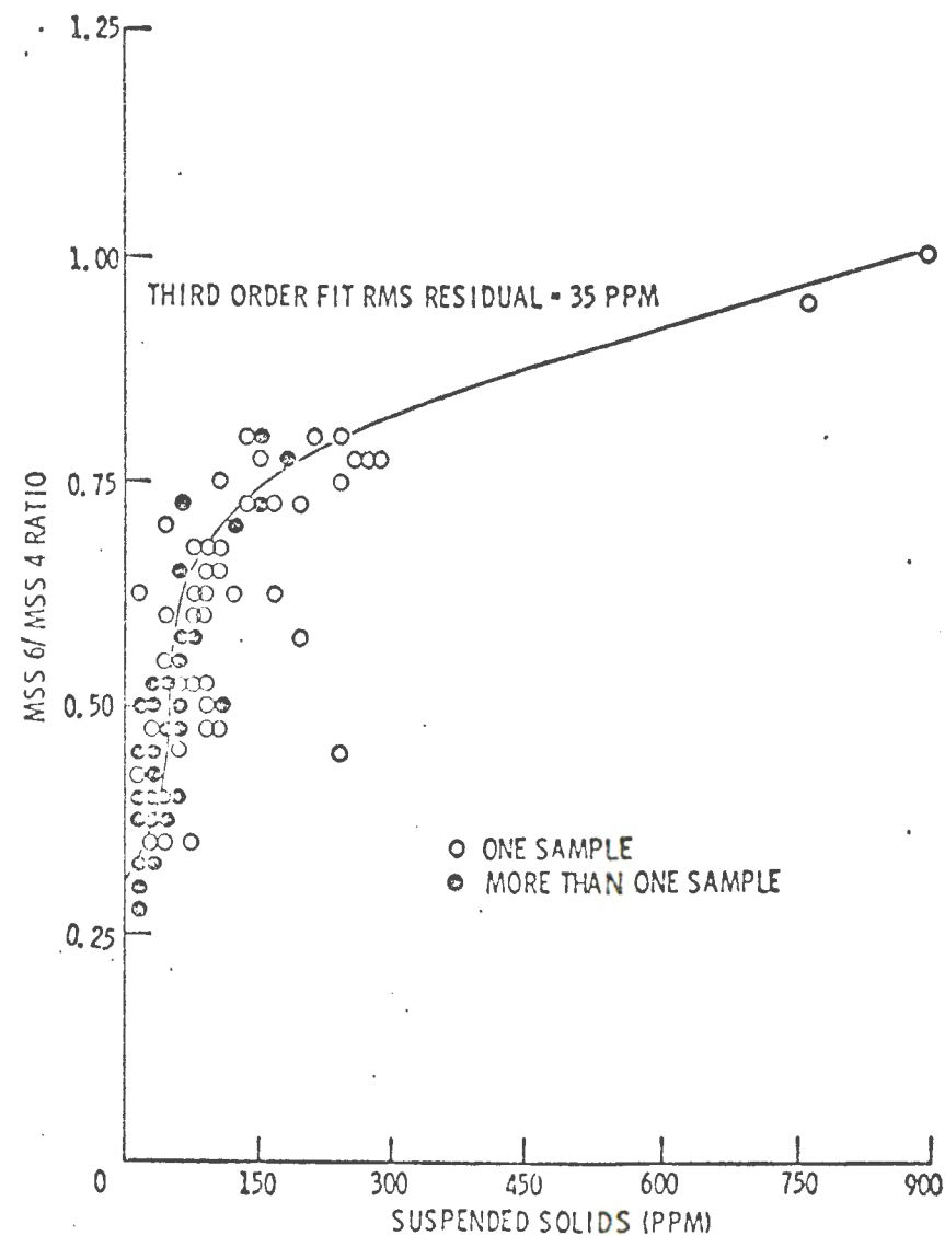
FIGURE 20. MSS 6/MSS 4 CCT RATIO VS. SUSPENDED SOLIDS FOR 170 WATER SAMPLES TAKEN FROM 3 KANSAS RESERVOIRS DURING 13 DIFFERENT ERTS-1 CYCLES.
