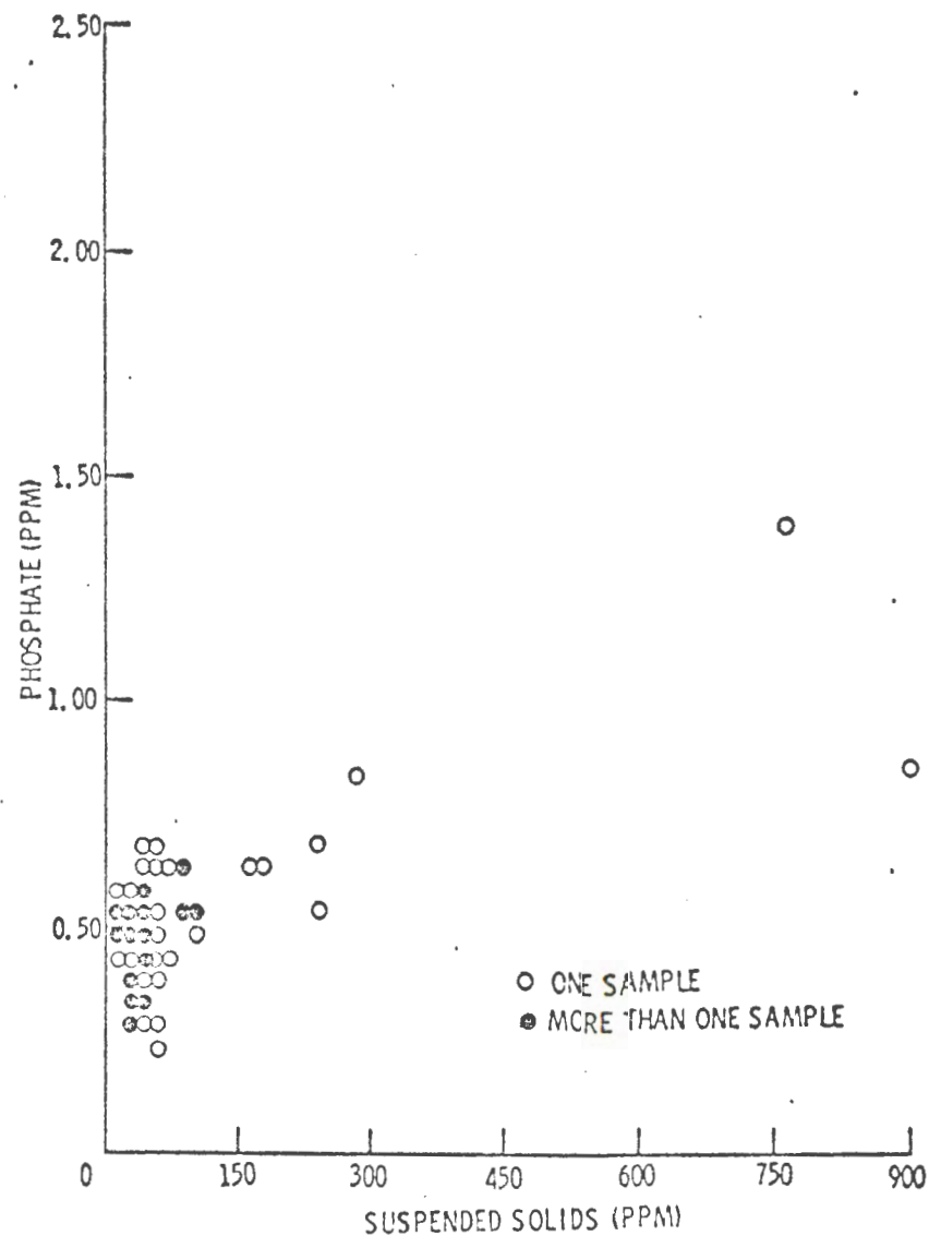
FIGURE 45. PHOSPHATE [ PO_4 ] VS. SUSPENDED SOLIDS FOR 70 SAMPLES TAKEN FROM 2 KANSAS RESERVOIRS OVER A 13 MONTH PERIOD.
