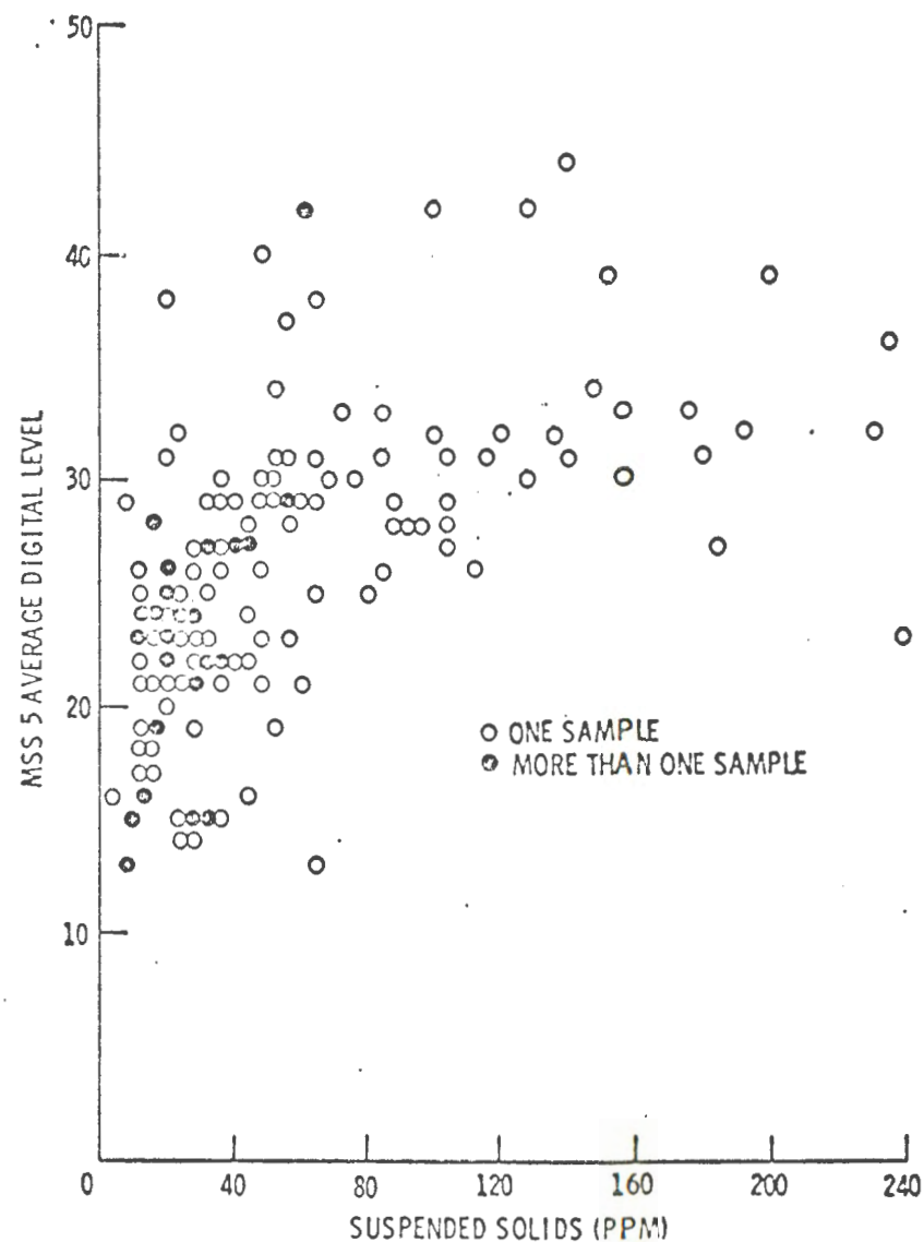
FIGURE 10. MSS 5 CCT DIGITAL LEVEL VS. SUSPENDED SOLIDS FOR 166 WATER SAMPLES TAKEN FROM 3 KANSAS RESERVOIRS DURING 13 DIFFERENT ERTS-1 CYCLES.
