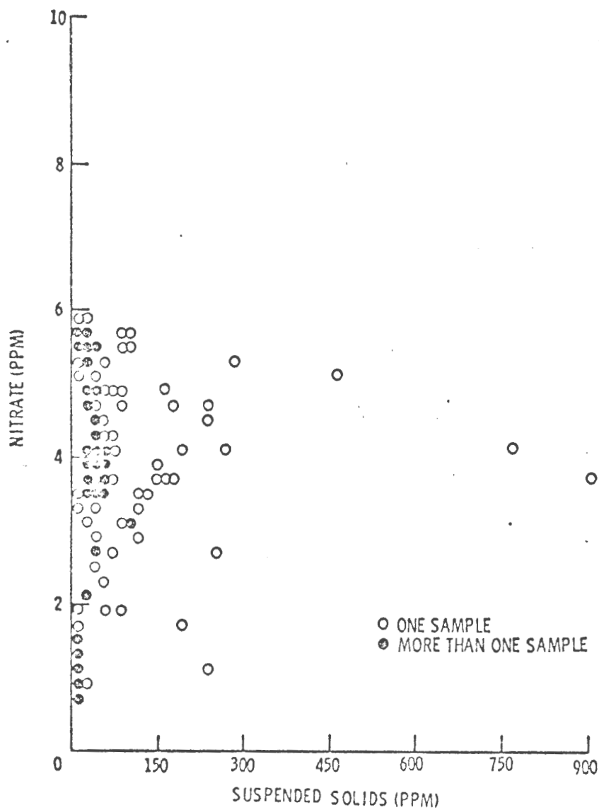
FIGURE 46. NITRATE [NO_3] VS. SUSPENDED SOLIDS FOR 140 SAMPLES TAKEN FROM 2 KANSAS RESERVOIRS OVER A 13 MONTH PERIOD.
