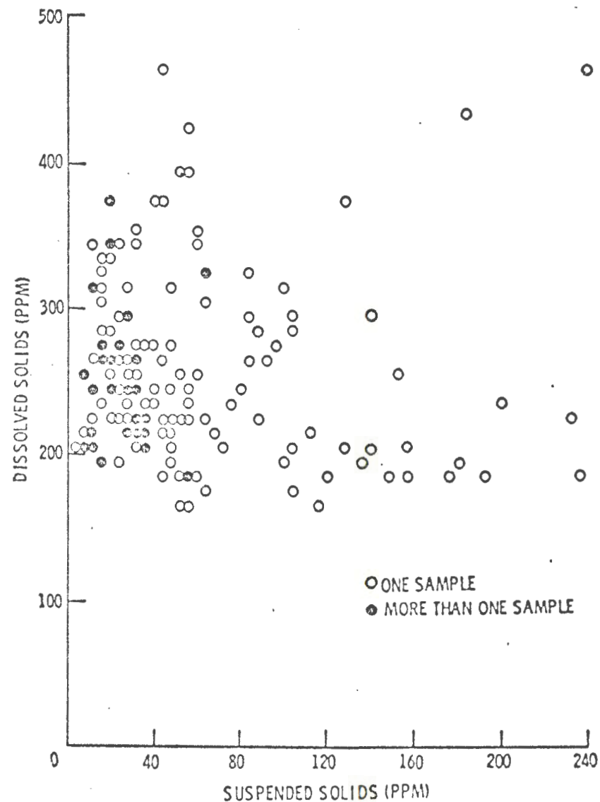
FIGURE 33. DISSOLVED SOLIDS VS. SUSPENDED SOLIDS FOR 120 WATER SAMPLES TAKEN FROM 3 KANSAS RESERVOIRS OVER A 13 MONTH PERIOD.
