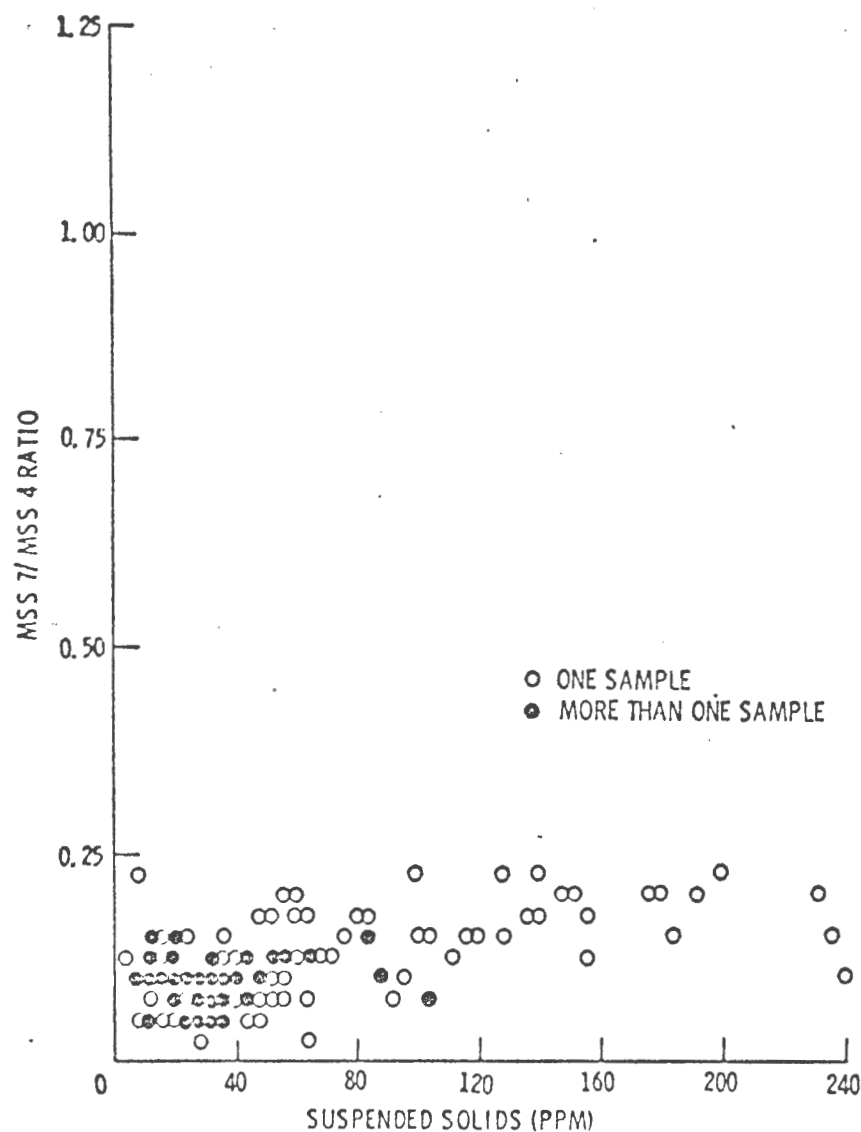
FIGURE 15. MSS 7/MSS 4 CCT RATIO VS. SUSPENDED SOLIDS FOR 167 WATER SAMPLES TAKEN FROM 3 KANSAS RESERVOIRS DURING 13 DIFFERENT ERTS-1 CYCLES.
