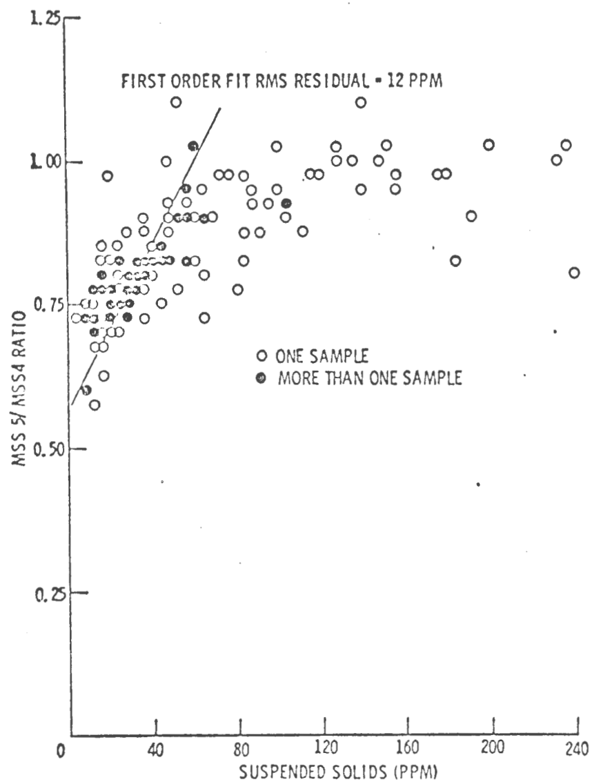
FIGURE 13. MSS 5/MSS 4 CCT RATIO VS. SUSPENDED SOLIDS FOR 167 WATER SAMPLES TAKEN FROM 3 KANSAS RESERVOIRS DURING 13 DIFFERENT ERTS-1 CYCLES.
