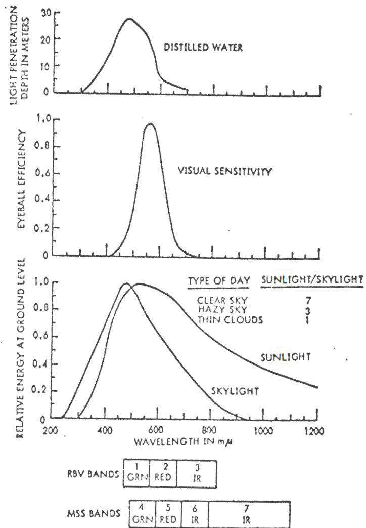
FIGURE 4. RADIANCE vs WAVELENGTH.
