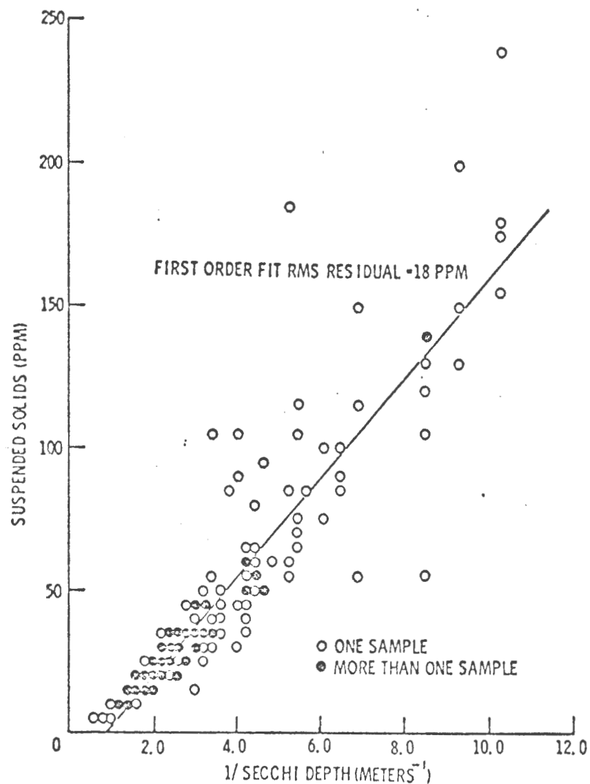
FIGURE 25. SUSPENDED SOLIDS VS. INVERSE SECCHI DEPTH FOR 164 WATER SAMPLES TAKEN FROM 3 KANSAS RESERVOIRS DURING 13 DIFFERENT ERTS-1 CYCLES.
