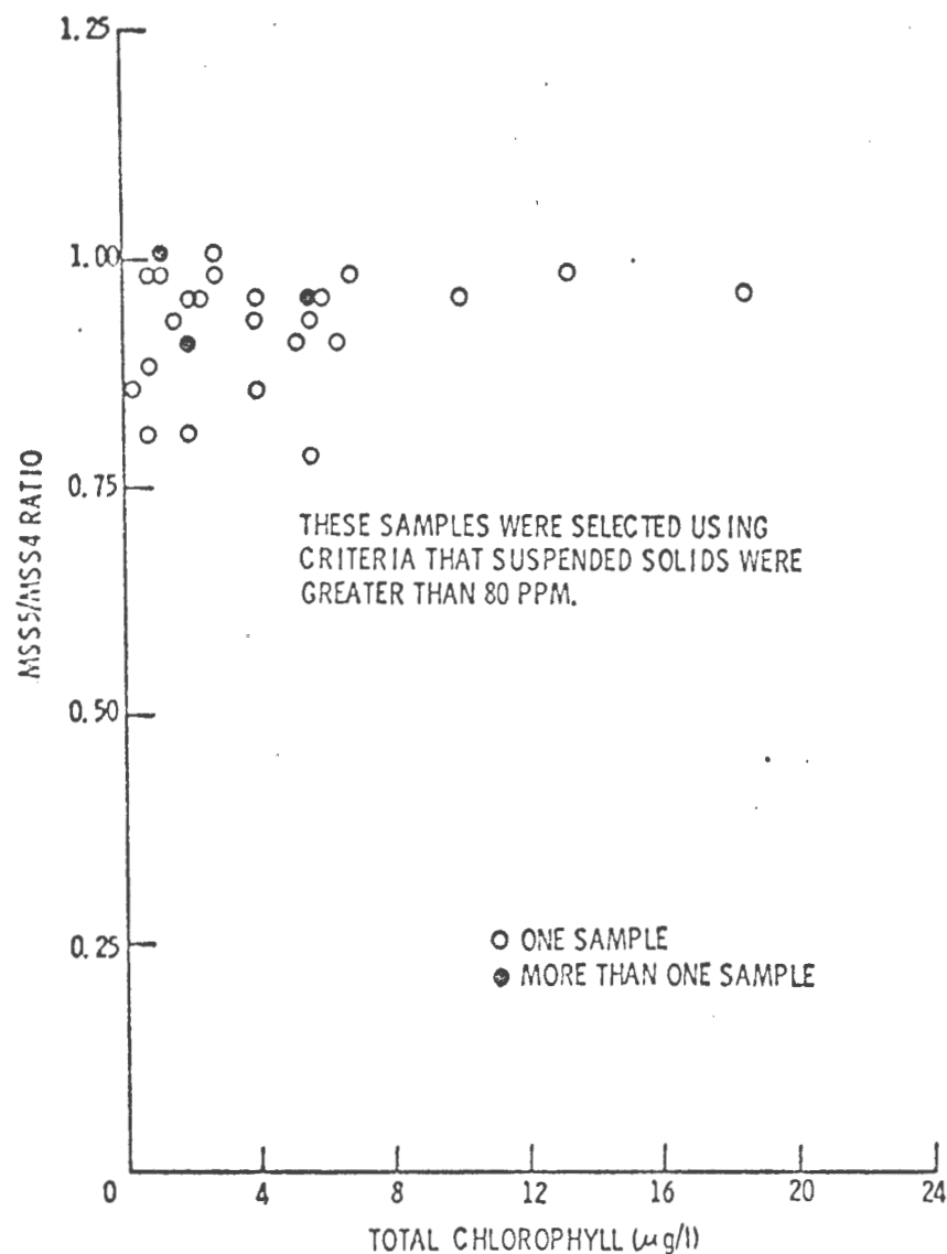
FIGURE 40. MSS 5/ MSS 4 CCT RATIO VS. TOTAL CHLOROPHYLL FOR 30 SAMPLES TAKEN FROM 2 KANSAS RESERVOIRS OVER A 13 MONTH PERIOD.
