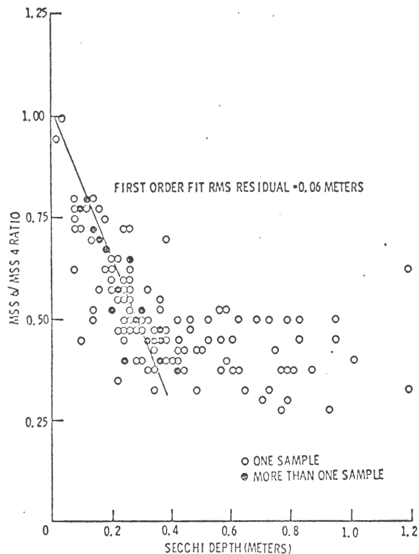
FIGURE 27. MSS 6/MSS 4 CCT RATIO VS. SECCHI DEPTH FOR 170 WATER SAMPLES TAKEN FROM 3 KANSAS RESERVOIRS DURING 13 DIFFERENT ERTS-1 CYCLES.
