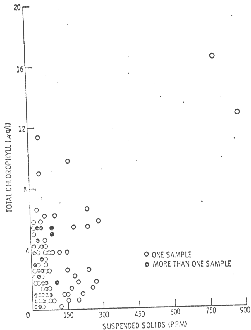
FIGURE 38. TOTAL CHLOROPHYLL VS. SUSPENDED SOLIDS FOR 140 SAMPLES TAKEN FROM 2 KANSAS RESERVOIRS OVER A 13 MONTH PERIOD.
