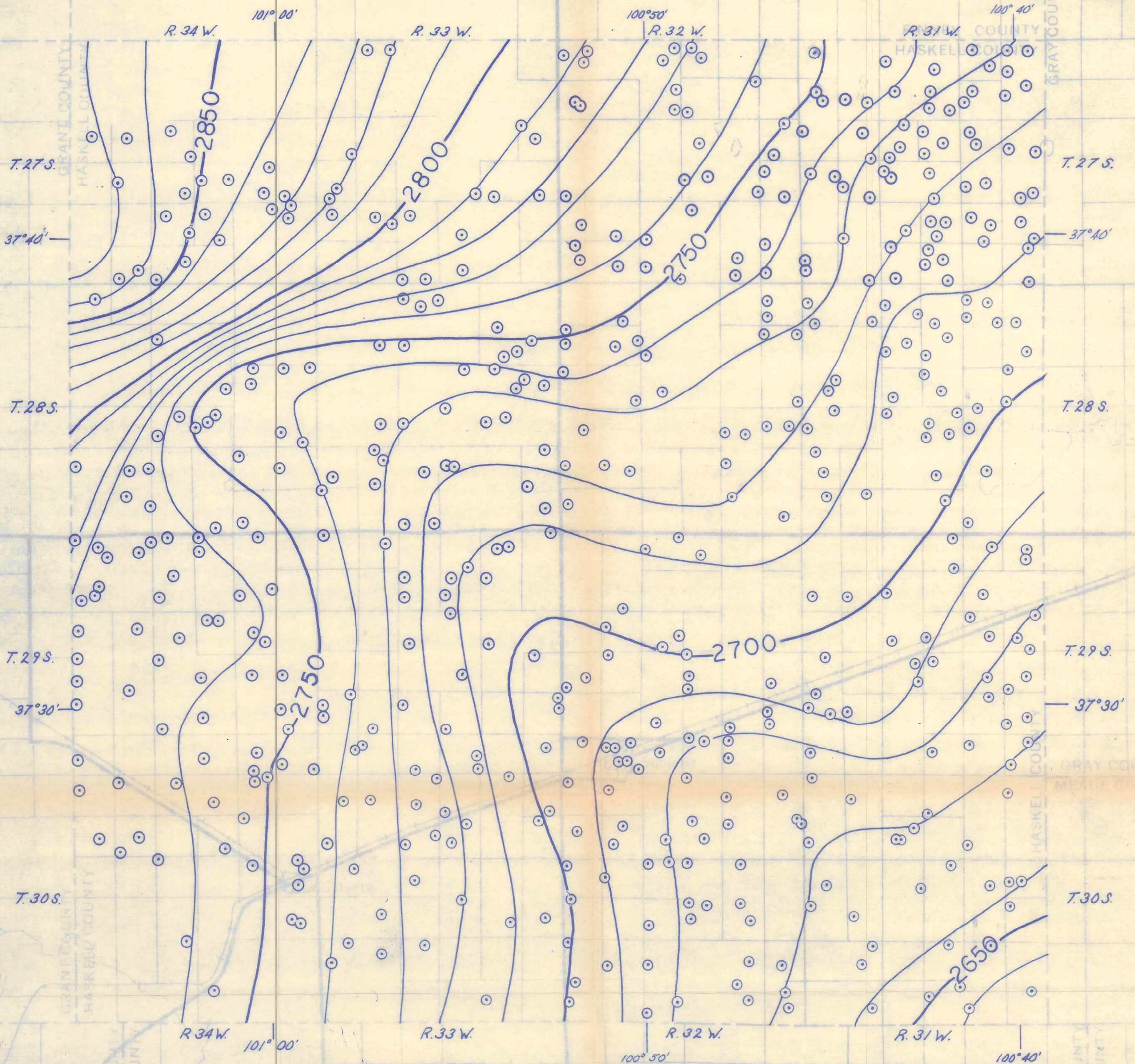
FIGURE 6A. Hydrologic map showing water-level contours and location of large-capacity wells (January 1970)
