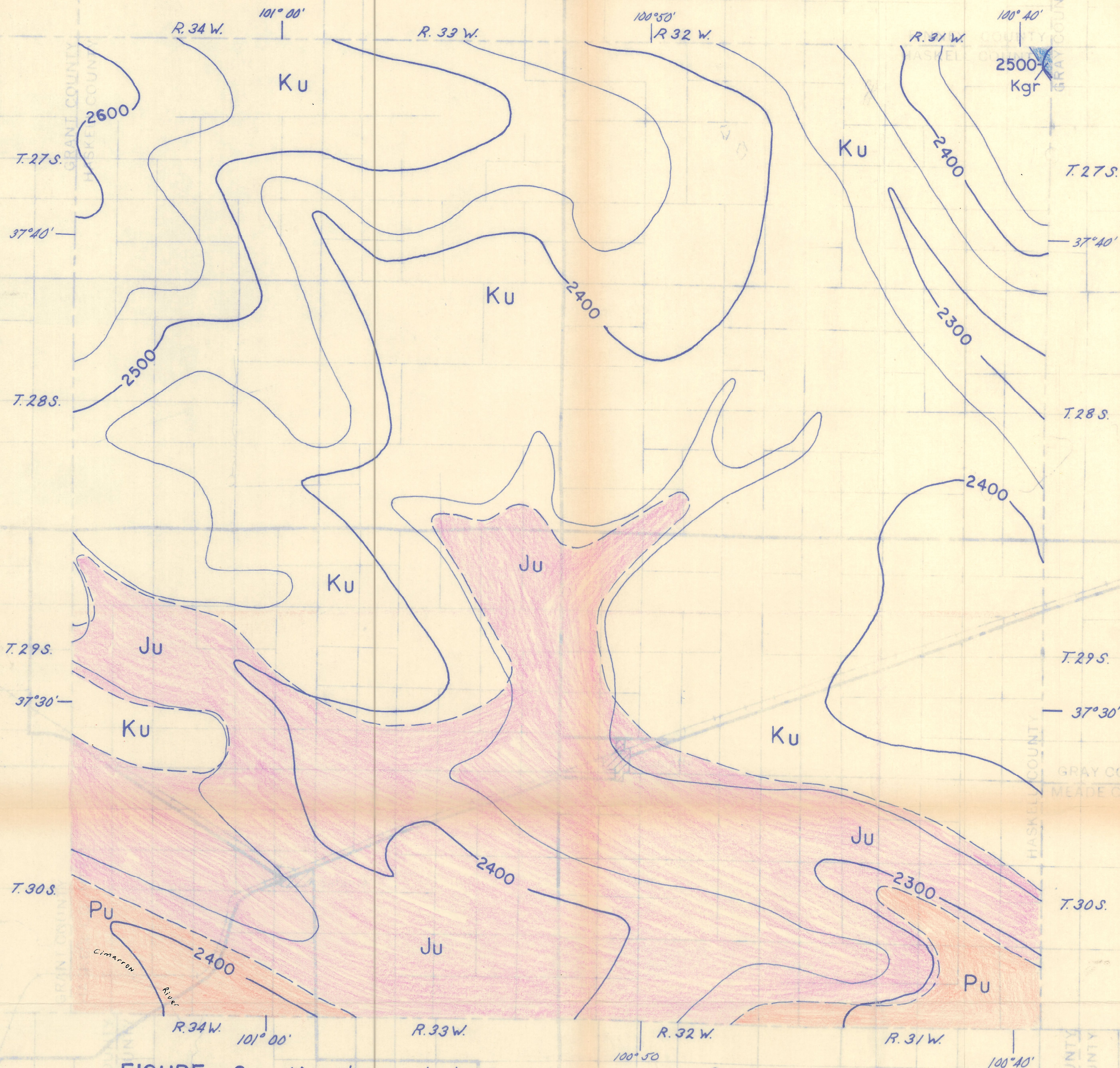
FIGURE 2. Map showing bedrock geology and configuration of bedrock surface
