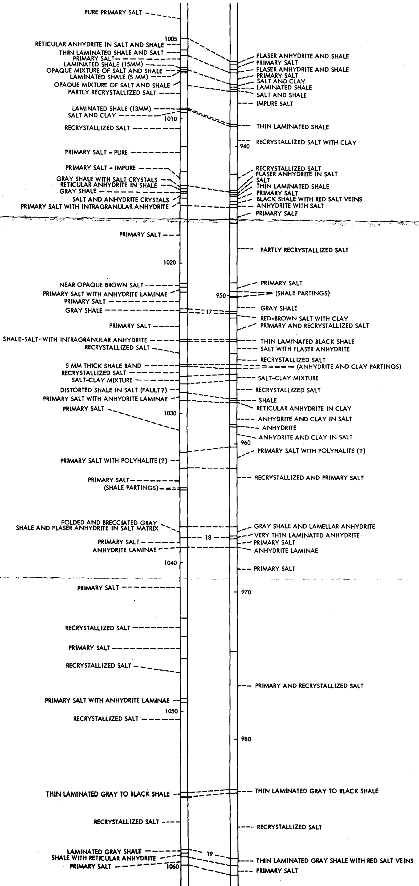
Fig. 53--Lithologic correlation of "key" beds in proposed disposal zone between AEC Core Hole No. 1 and No. 2.
