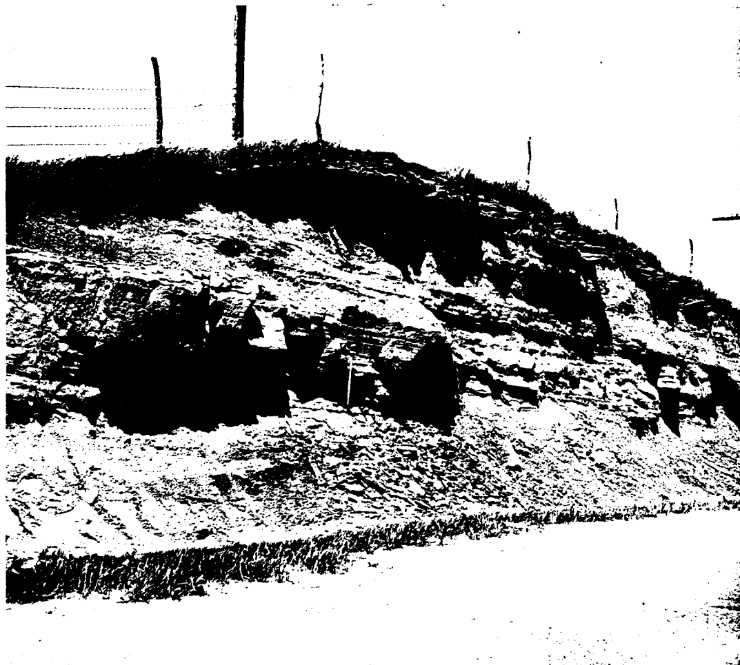
Fig. 4.--- Thin-bedded siltstone marking top of Longford Member, Kiowa Formation, about 0.15 mile (0.24 km) north SE cor. sec. 8, T. 10 S., R. 1 E., Clay County, Kansas. Upper parts contain numerous discoidal concretionary masses of calcite cement. Handle of pick is about 2.5 feet (0.8 m) long.
