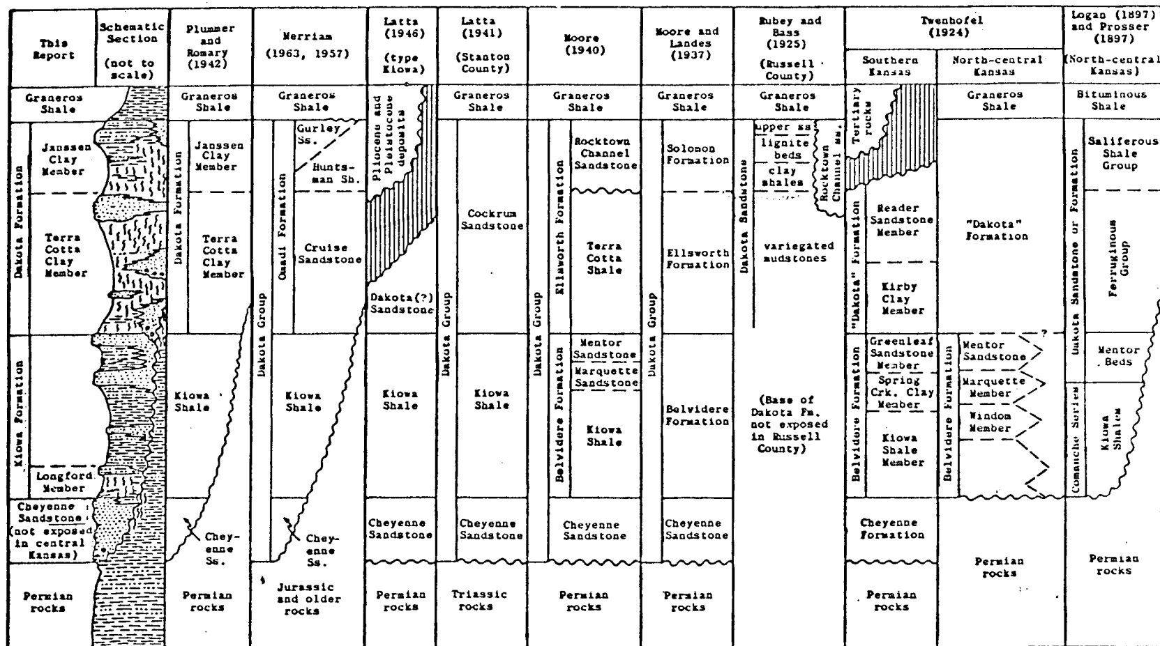
Fig. 2. --- Chart showing generalized section of basal Cretaceous rocks in Kansas and some of the variations in nomenclature and interpretations of stratigraphic relationships.
