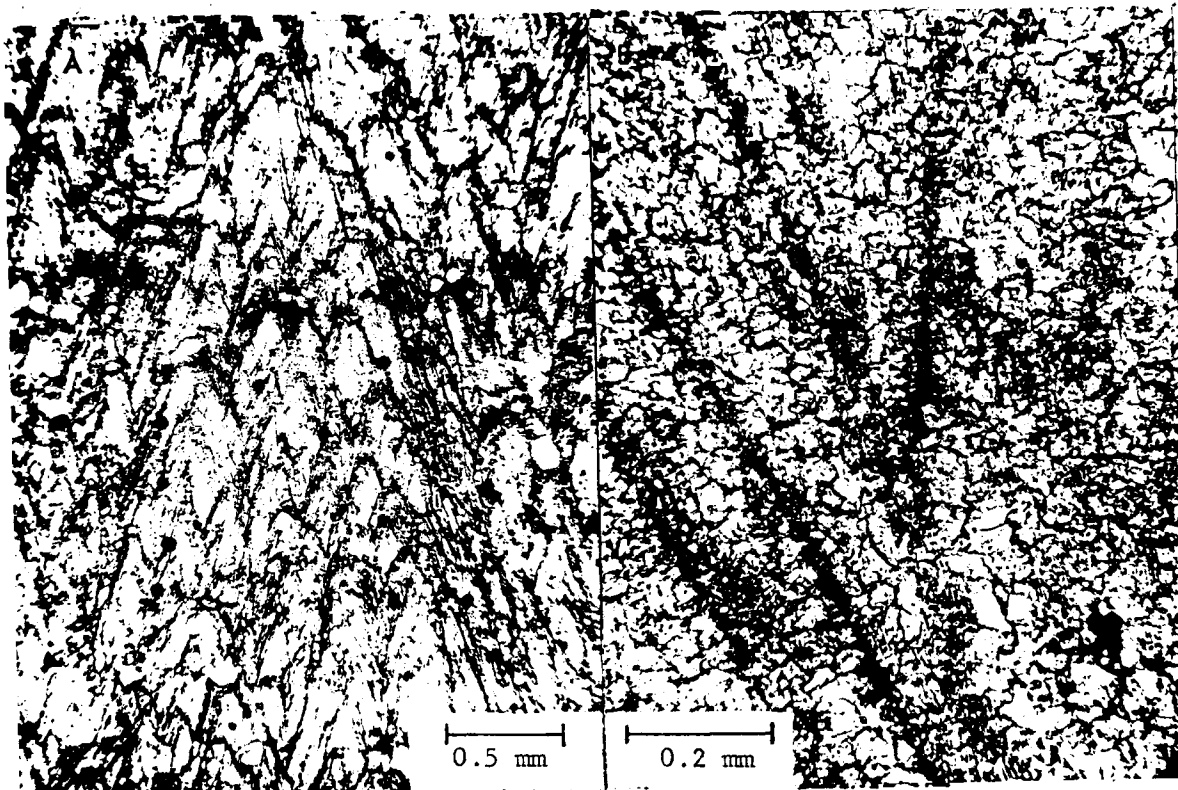
Fig. 14.--- Photomicrographs of calcareous cone-in-cone structure, north-central Kansas. Plane-polarized light.
