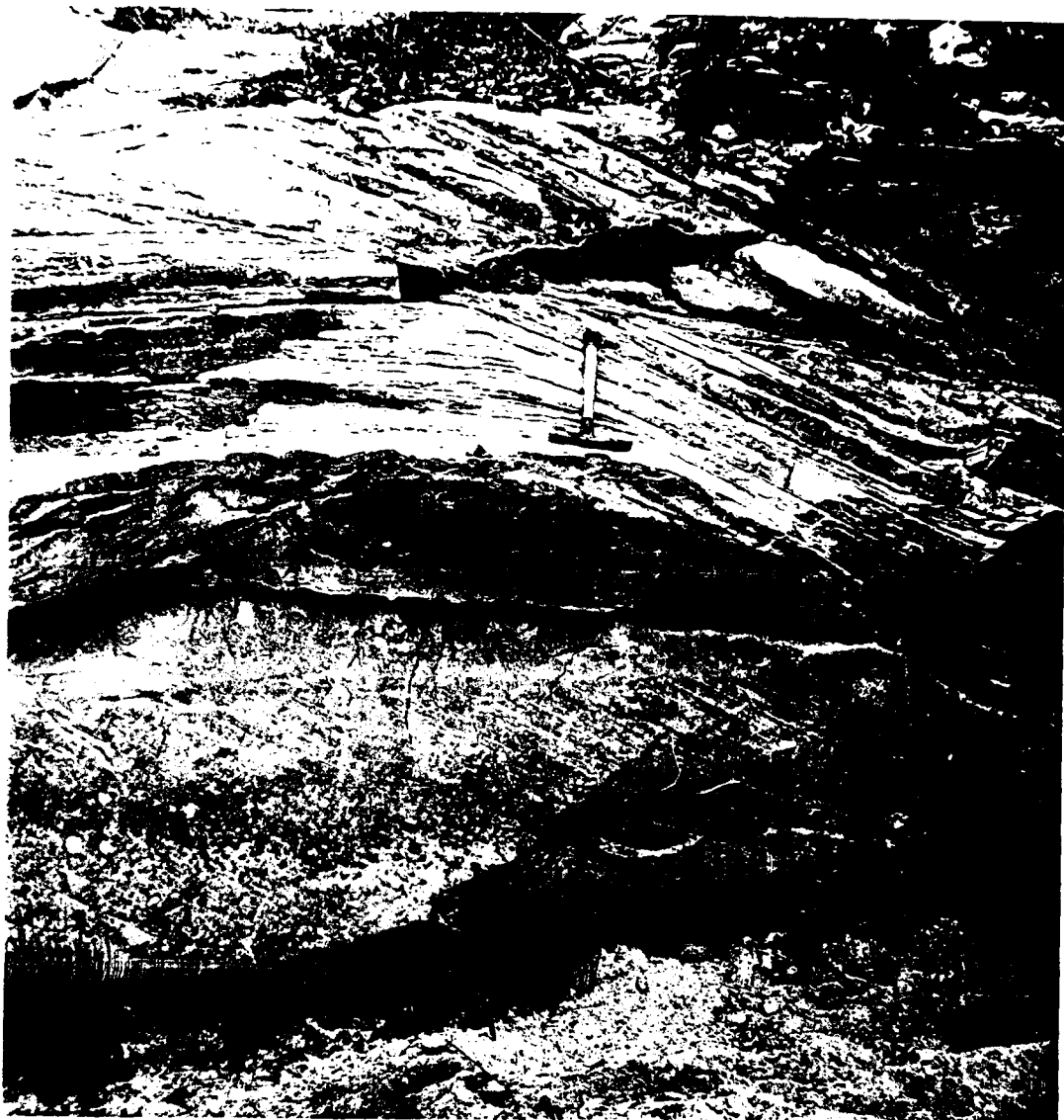
Fig. 21.--- Simple cross-stratification in thick lenticular deposit of Kiowa sandstone in W 1 SW 1 sec. 31, T. 15 S., R. 6 W., Ellsworth County, Kansas. The set of simple cross-strata shows steep dip to the west-southwest and a reverse dip of a few degrees to the east-northeast. An inclined planar surface separates the set from wedge-planar set above. The set of simple cross-strata also is separated from a set of trough-shaped cross-strata below by a zone of seemingly structureless sandstone in the center part of the photograph, but to the right the simple cross-stratification occupies a scour cut into the set of trough-shaped strata. The sandstone is part of the same thick deposit pictured in Figures 19-A and 20.
