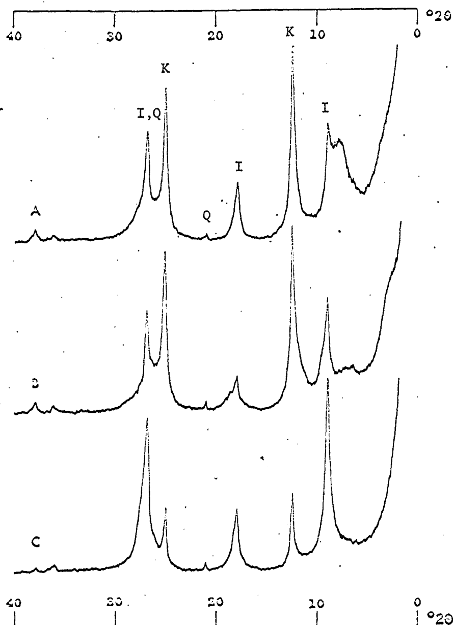
Fig. 34.--- Diffractometer patterns of fraction finer than 2 microns from red-mottled Dakota mudstone in lower part of Terra Cotta Clay Member, S\frac{1}{2} SW \frac{1}{4} sec. 28, T. 15 S., R. 7 W., Ellsworth County, Kansas (unit 18, Measured Section 5, Appendix and Plate 4). The patterns illustrate the absence of chlorite and vermiculite and the abundance of kaolinite (K) in most Dakota rocks, and the presence of appreciable illite (I) and mixed-layer illite-montmorillonite in the basal part of the formation. A) air-dried, B) glycerated, C) heated to 450°C. Some quartz (Q) is present. In Pattern A, the illite 001 peak at 8.8^{\circ}2\theta (10A) is strongly skewed and a hump appears near 7.7^{\circ}2\theta . The shape of Pattern A indicates weak mixed-layer "superlattice" diffractions between 3^{\circ} and 4^{\circ}2\theta . Pattern B shows shift of the mixed-layer hump and "superlattice" reflections. Pattern C only shows skewing that can be attributed to Lorentz polarization and angular effects. See Figure 33-B.
