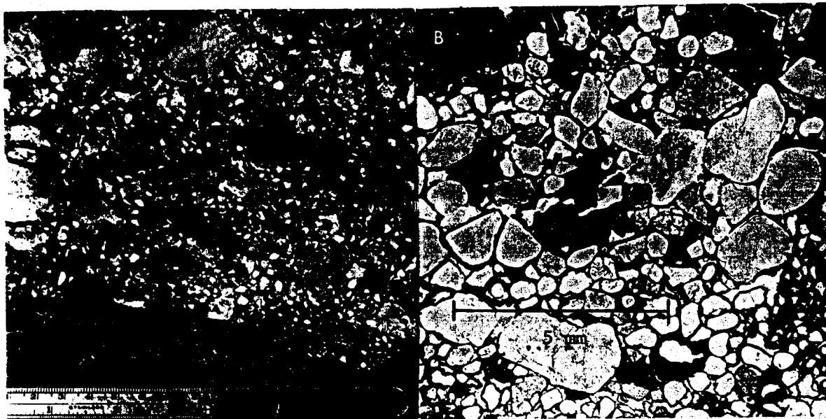
Fig. 17.--- Conglomeratic Kiowa sandstone, Ottawa County, Kansas. A) Close-up of bedding surface of dominantly fine-grained sandstone near cen. sec. 8, T1 11 S., R. 2 W.. The irregular surface is paved with well-rounded coarse grains and granules of quartz, quartzite, and chert as well as with molds of rounded shale pebbles.
