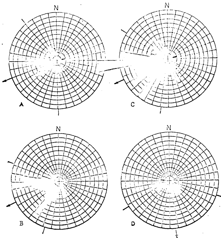
Fig. 25.--- Circular histograms of vector resultants of cross-strata dip bearings calculated for localities in north-central Kansas. Vector resultants are plotted in 10-degree sectors; each segment represents one vector resultant. Sample density is one locality per township. Arrows show grand vector resultants; arc between lines is one standard deviation plotted on each side of grand vector resultant.
