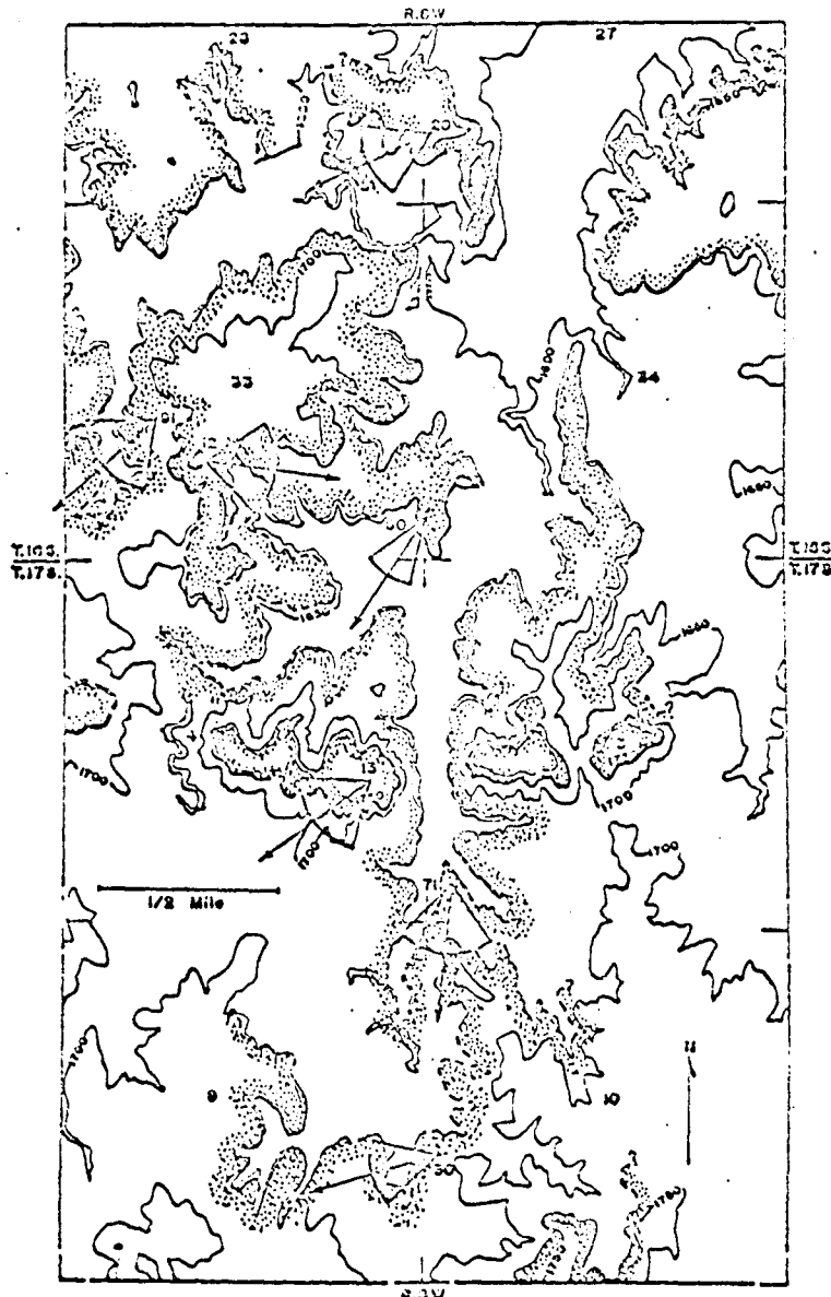
Fig. 38. --- Map showing lenticular nature of sandstone and local variability of cross-stratification trends in Dakota Formation in parts of T. 16 and 17 S., R. 8 W., Ellsworth County, Kansas. Bases of prominent sandstone lenses mapped from aerial photographs and shown by dark lines, long dash where approximately located, short dash where inferred. Stipples are on uphill side of contacts; queries mark areas where sandstone lenses pinch out within or grade laterally into sequences composed largely of mudstone and claystone. Light lines are contours; contour interval 50 feet (15 m). Arrows show vector resultants of dip bearings of cross-stratification. Arc delimited on each side of vector resultants is one standard deviation; numerals show number of measurements at each locality. The writer estimates that as many as 5 or 6 lenses of sandstone are shown in the seven square-mile area.
