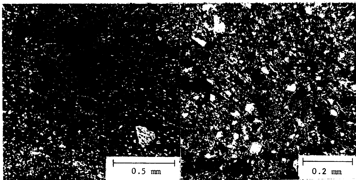
Fig. 26.--- Photomicrographs of thin sections of siltstone and mudstone, Longford Member, Kiowa Formation, north-central Kansas.
