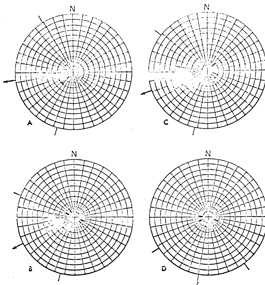
Fig. 24.--- Circular histograms of vector resultants of cross-strata dip bearings calculated for localities in Ellsworth County, Kansas. Vector resultants are plotted in 10-degree sectors; each segment represents one vector resultant. Stipples designate vector resultants used to simulate one-locality-per-township sampling grid. Arrows show grand vector resultants; arc between lines is one standard deviation plotted on each side of grand vector resultant.
