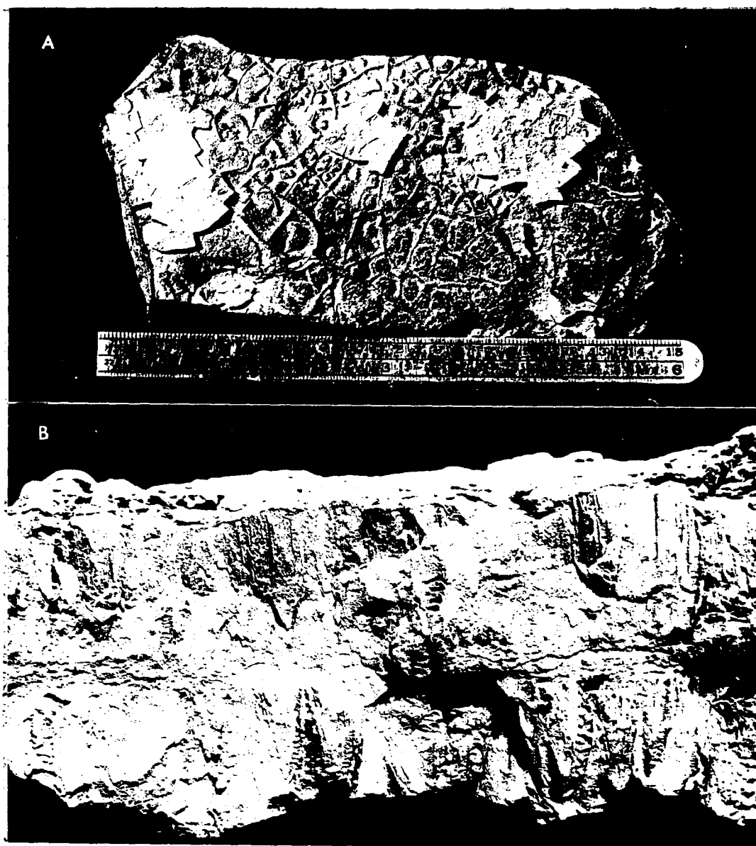
Fig. 12.--- Concretionary structures in Kiowa shale. A) Fragment of impure siderite (clay-ironstone) concretion from SE \frac{1}{4} SW \frac{1}{4} sec. 1, T. 16 S., R. 7 W., Ellsworth County, Kansas. Unusual surface markings and polygonal cracks probably are colloidal phenomena allied to synaeresis during lithification.
