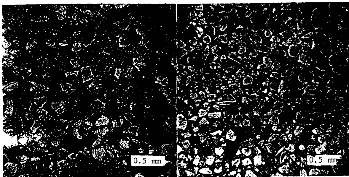
Fig. 16.--- Photomicrographs of thin sections of Kiowa sandstone, Ellsworth County, Kansas. Plane-polarized light. A) Fine-grained quartz-rich sandstone from thick lenticular deposit in SE \frac{1}{4} sec. 1, T. 16 S., R. 7 W.. Note generally subangular character of the quartz grains. The rock contains less than one percent interstitial clay and is from the same lenticular deposit as the calcite-cemented sandstone shown in Figure 18.
