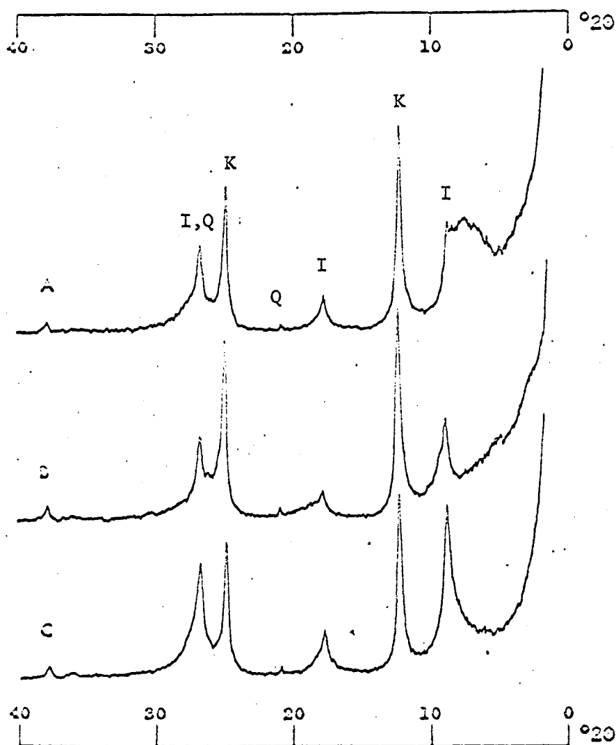
Fig. 47 --- Diffractometer patterns of fraction finer than 2 microns of a sample of kaolinitic and illitic shale from the Graneros Shale near cen. N\frac{1}{2} sec. 6, T. 15 S., R. 10 W., Ellsworth County, Kansas (unit 15, Measured Section 3, Appendix and Plate 8). A) air-dried, B) glycerated, C) heated to 450°C. Pattern A shows strong kaolinite peaks (K) and weaker reflections from illite (I). Small amounts of quartz (Q) are present. The illite 001 reflection at 8.8^{\circ}2\theta is strongly skewed and shows a prominent hump near 7.6^{\circ}2\theta . On glyceration, the skewed mixed-layer reflection is displaced to about 5.1^{\circ}2\theta (about 17A) and a "superlattice" diffraction maximum appears near 3^{\circ}2\theta . Swelling of the mixed-layer material to about 17A indicates the presence of montmorillonite. Collapse to 10A (Pattern C) on heating and little or no sign of skewing except for that which can be attributed to Lorentz polarization and angular effects verifies the presence of montmorillonite in the mixed-layer structure and demonstrates the absence of detectable chlorite or vermiculite.
