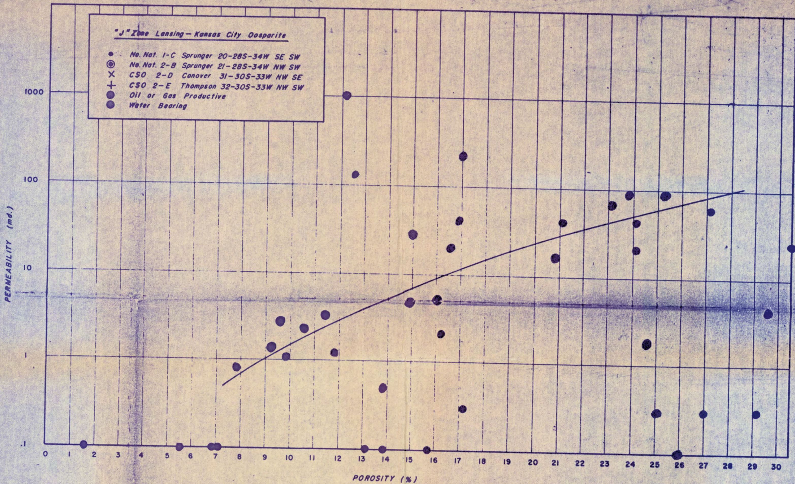
EXHIBIT 5-C of 14 GRAPH - POROSITY VERSUS PERMEABILITY "J" ZONE EXAMINATION OF PENNSYLVANIAN CARBONATE BANKS IN SOUTHWESTERN KANSAS BY HAROLD A. BROWN GEOLOGICAL REPORT NO. 13-A PAN AMERICAN PETROLEUM CORPORATION CENTRAL DIVISION GEOLOGICAL CONSULTING GROUP APRIL 1963
