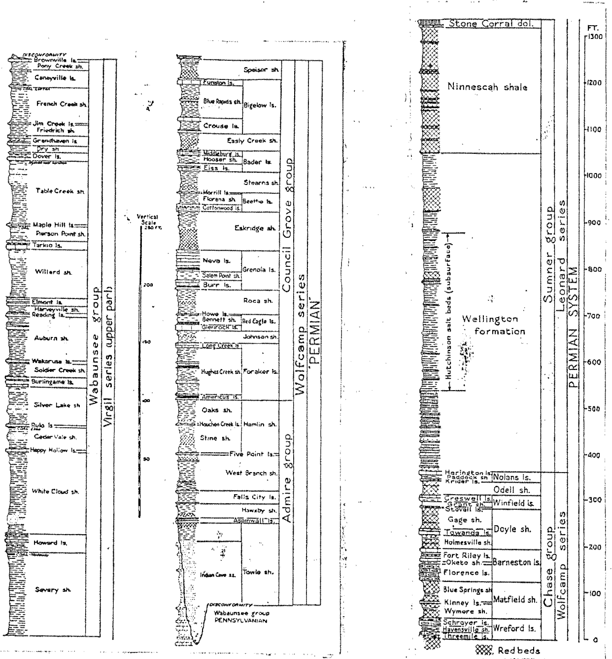
Figure 2. -- Generalized section of Middle and Lower Permian and Upper Pennsylvanian rocks for the state of Kansas. The stratigraphic position of outcropping formations in Cowley County is shown by these sections.
