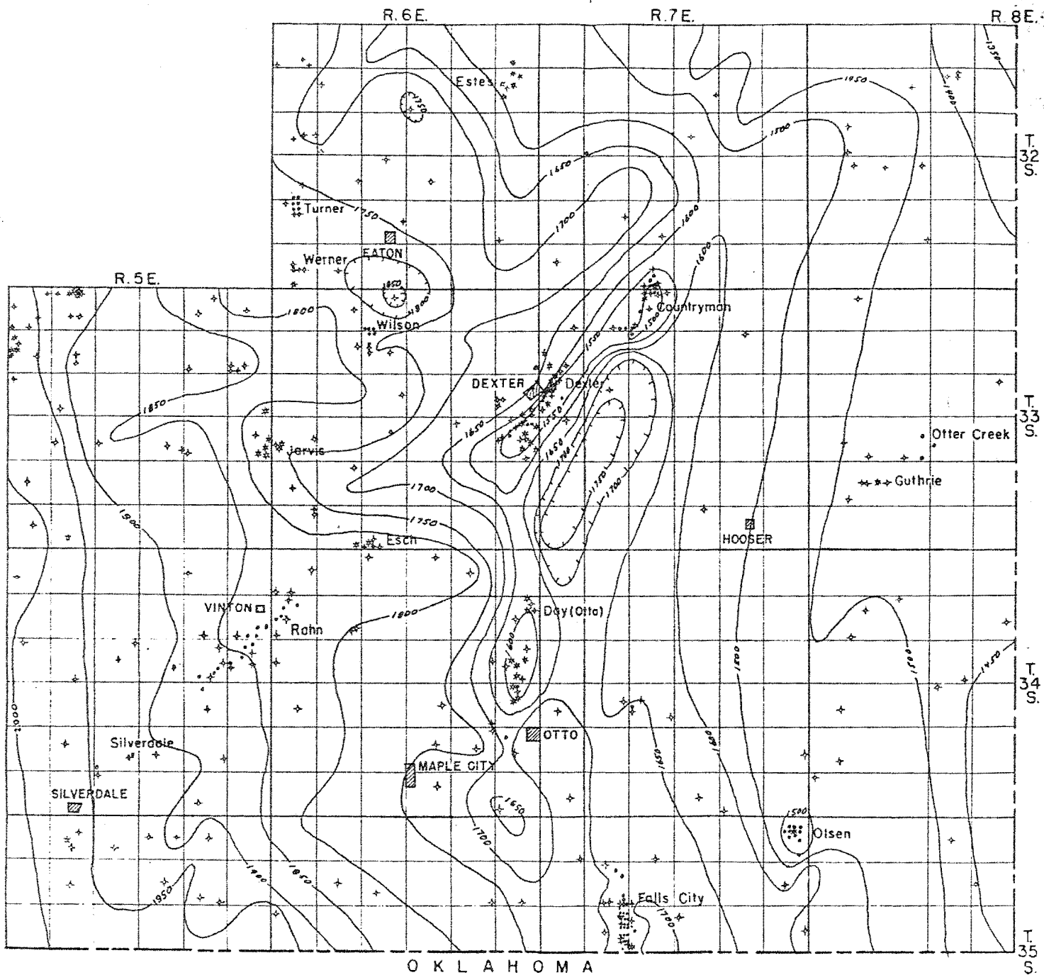
Figure 6. -- Generalized structural geologic map showing the structure of the top of the Mississippian limestone.
