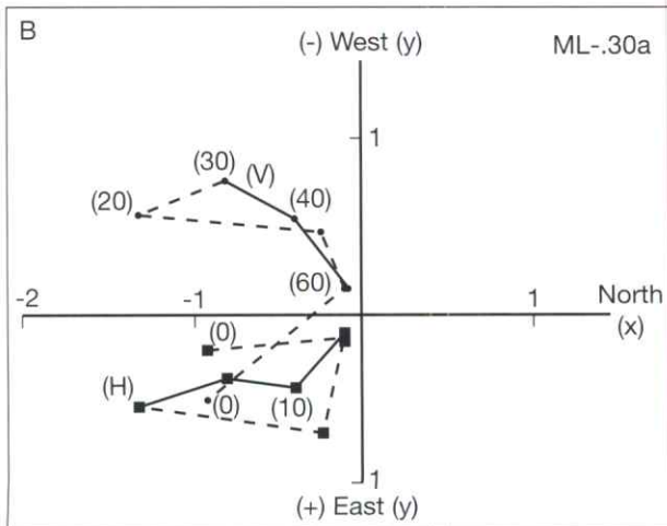
FIGURE 3-B-5. Vector intensity diagrams, Whipoorwill formation. Units are those of intensity ( A/m \times 10^{-3} ).
