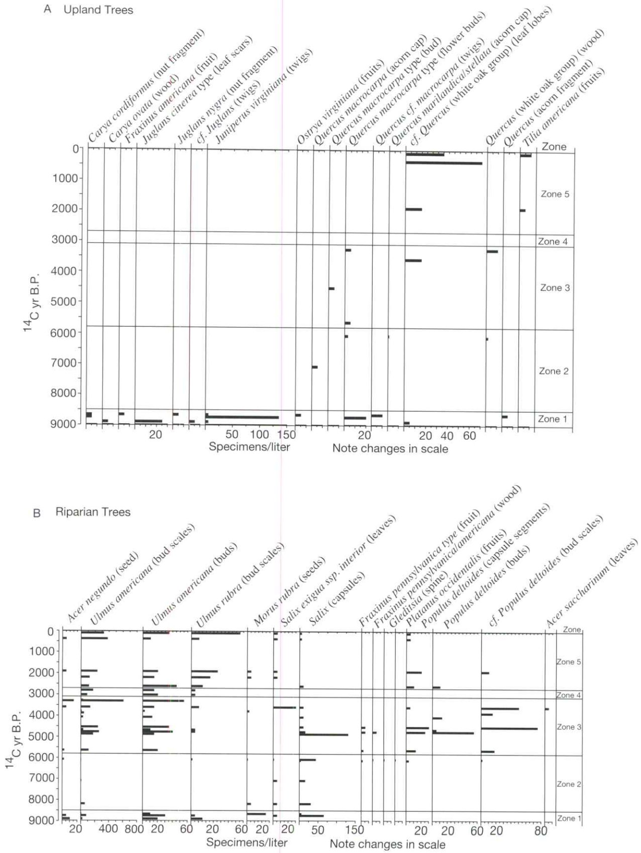
FIGURE 2-10. Summary of plant macrofossils derived from trees. The macrofossils were recovered from Holocene sediments exposed in cutbanks along the South Fork of the Big Nemaha River near Du Bois, Nebraska.
