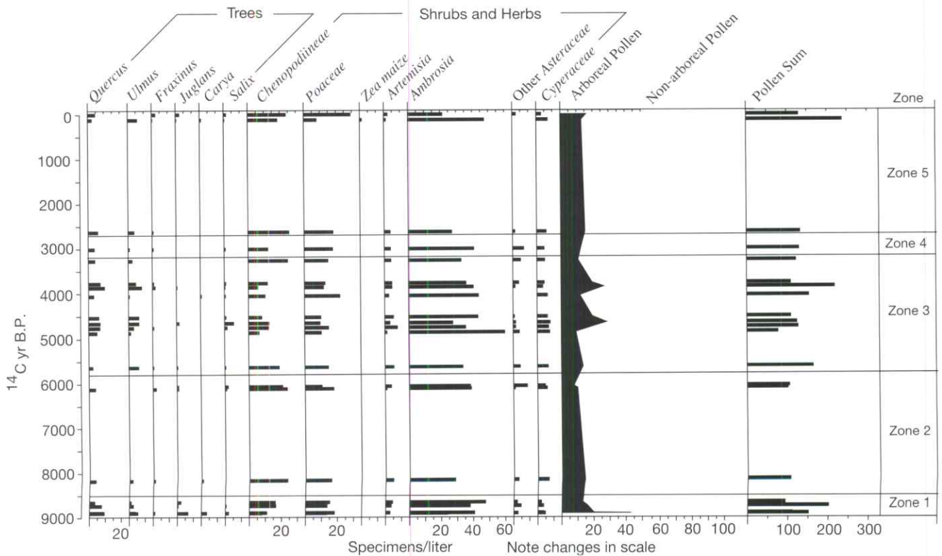
FIGURE 2-9. Pollen spectra for sediment samples collected from cutbanks along the South Fork of the Big Nemaha River near Du Bois, Nebraska. The pollen analysis was conducted by Glen Fredlund.
