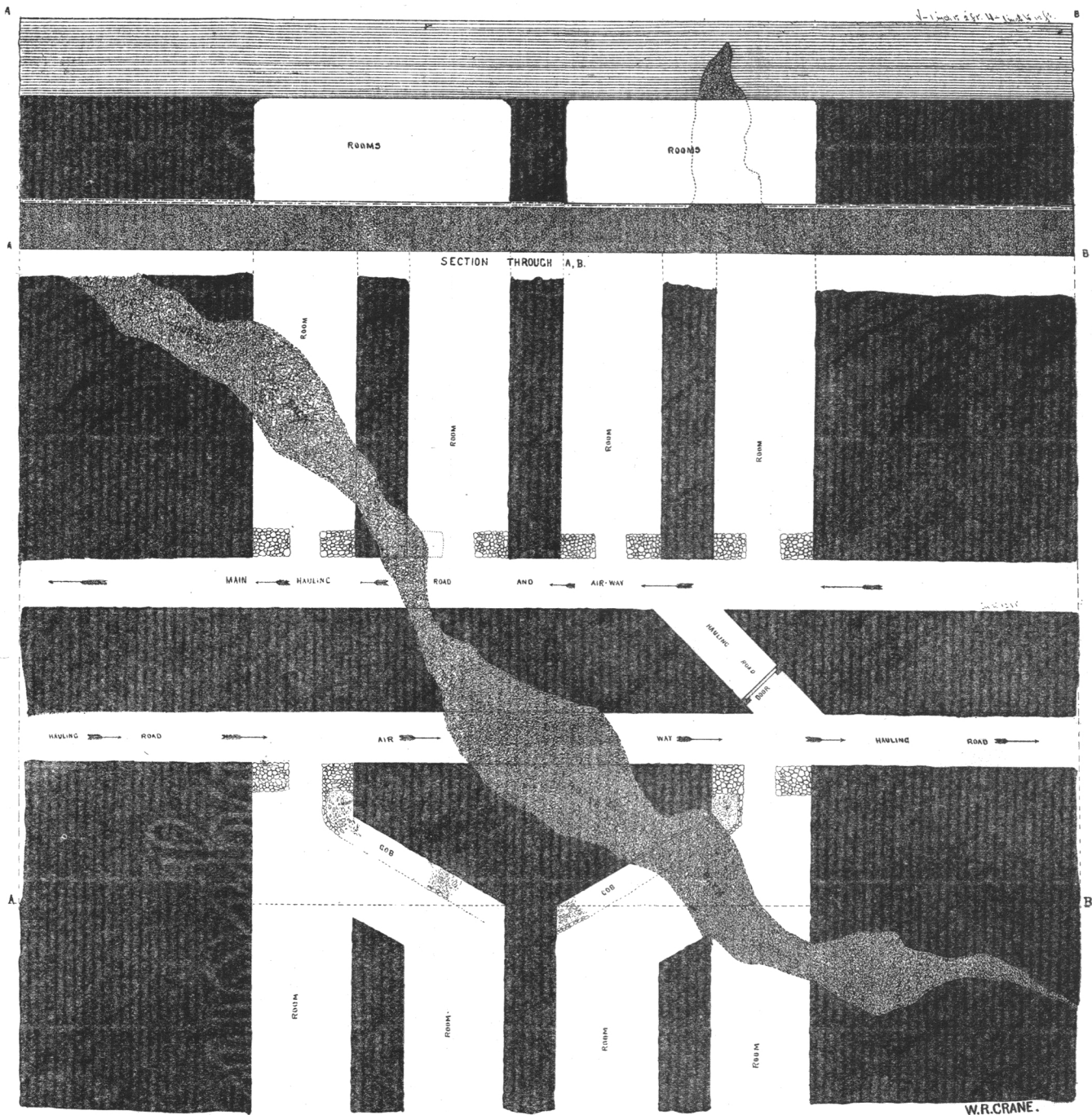
VERTICAL SECTION AND HORIZONTAL PLAN OF A SMALL PORTION OF A ROOM AND PILLAR WORKING, SHOWING A HORSEBACK INTERSECTING THE COAL AND ACCOMPANYING STRATA.
