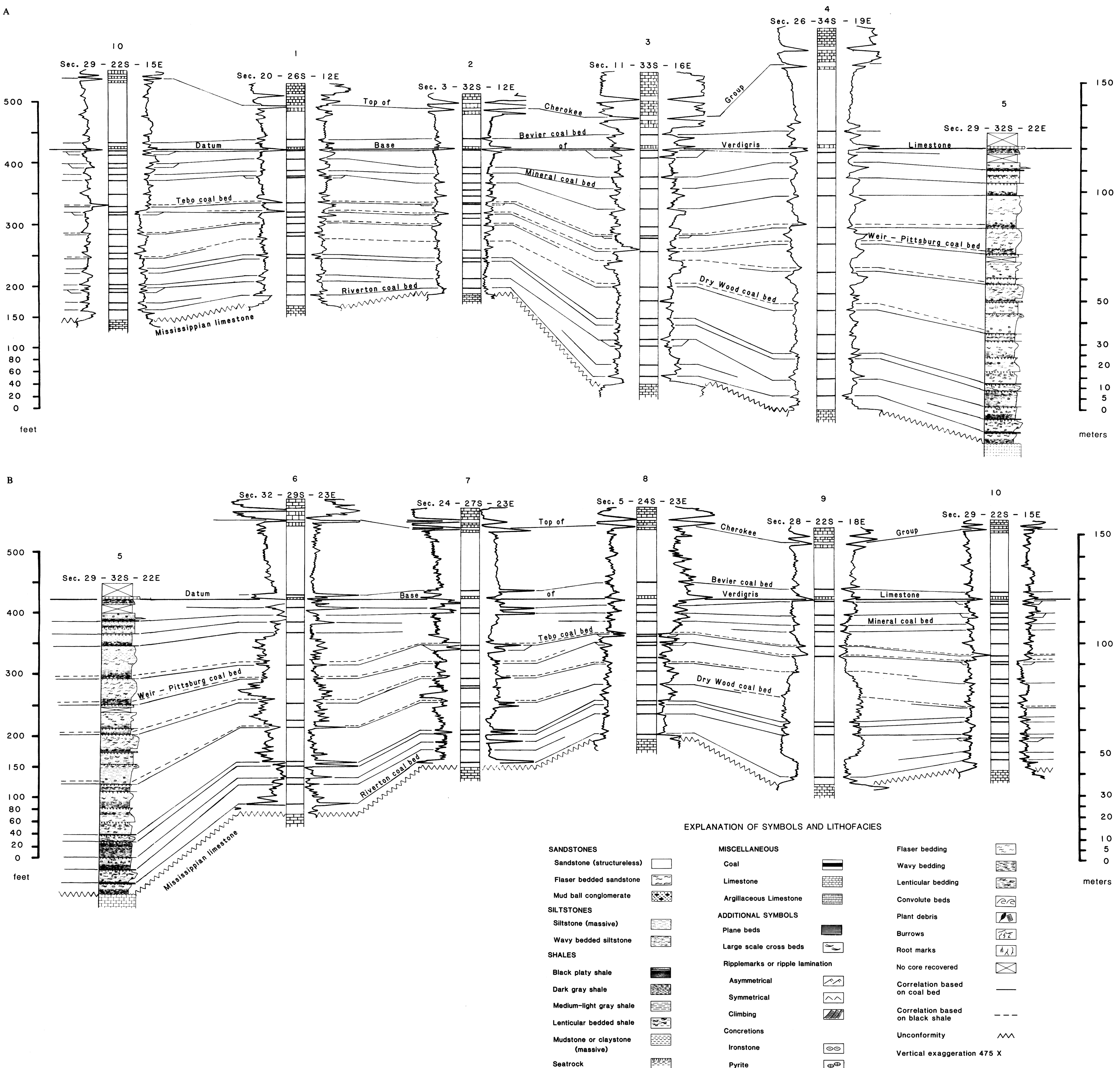
FIGURE 4—(A and B) Stratigraphic cross section of the Cherokee Group, southeastern Kansas (Harris, 1983).
