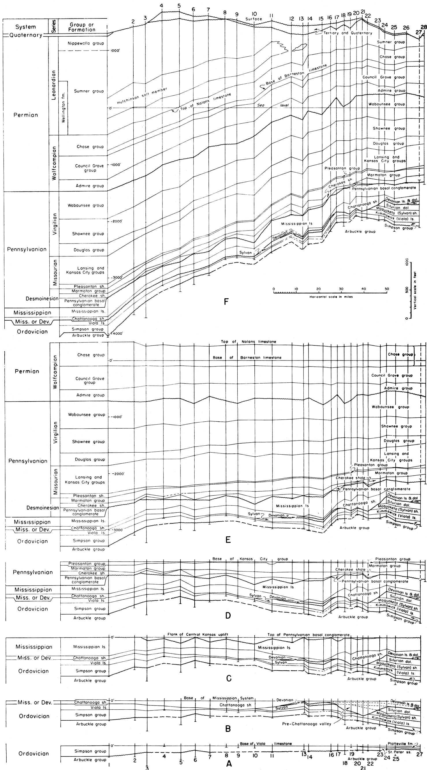
FIG. 3.—Skeletonized cross sections on the line of the large cross section showing the development of structure by correlation of logs on successive beveled or depositional surfaces. A shows the attitude of the older rocks at the end of Simpson time. B shows the attitude of the Chattanooga shale and older rocks before the deposition of the Mississippian limestones; the dashed lines show the relation of Devonian and Silurian rocks before the erosion of the pre-Chattanooga valley. C shows the attitude of the pre-Pennsylvanian rocks after post-Mississippian beveling. D shows the attitude of the older rocks at the beginning of Kansas City time. E shows the attitude of the rocks at the beginning of Barneston time. F shows the present attitude of the rocks.
