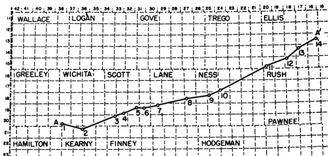
Map of Western Kansas area, showing location of cross section A-A'
