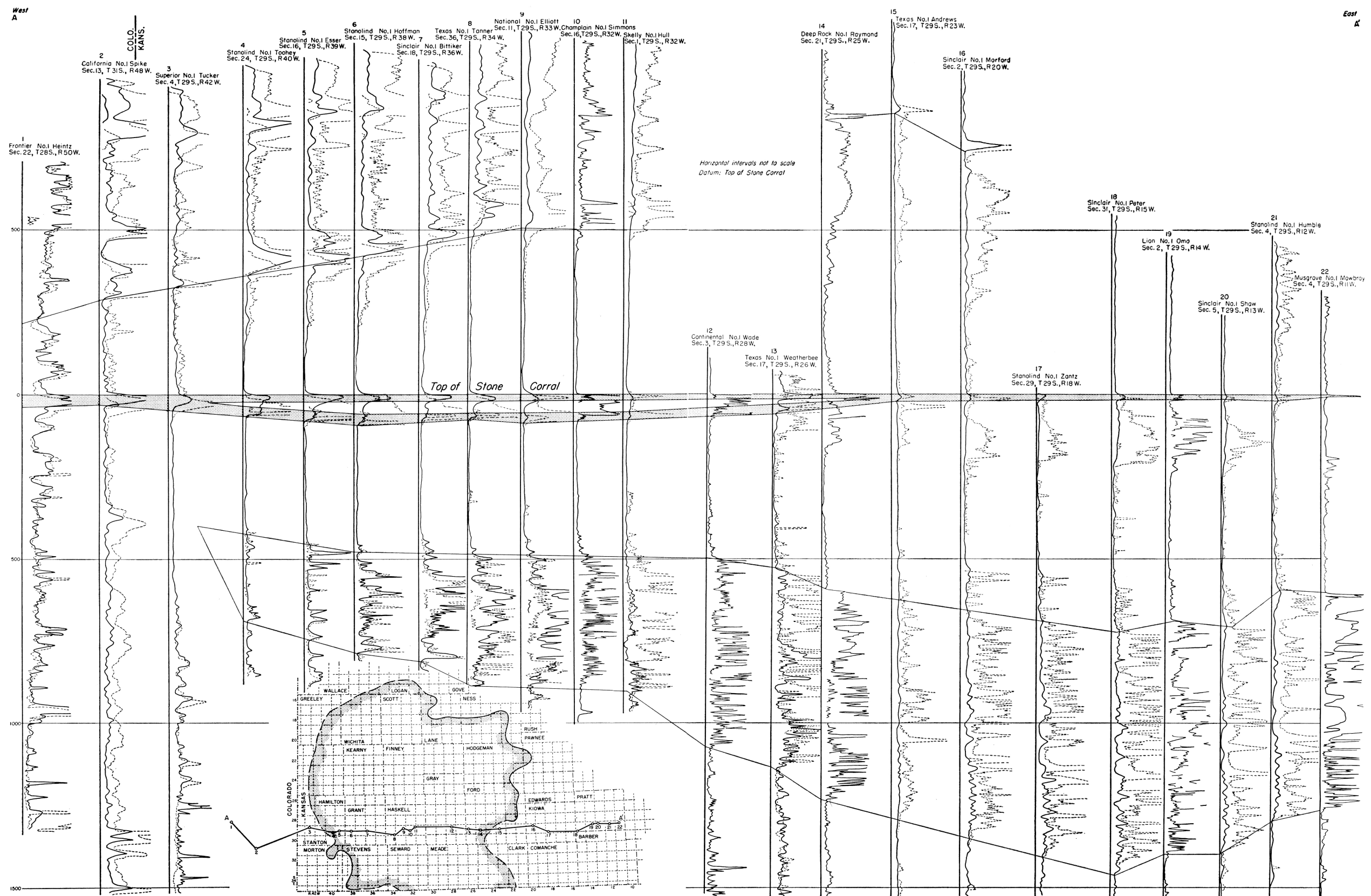
FIG. 2.—Cross section showing separation of Stone Corral formation into two anhydrite member on line A-A' and inset outlining area in which separation occurs.
