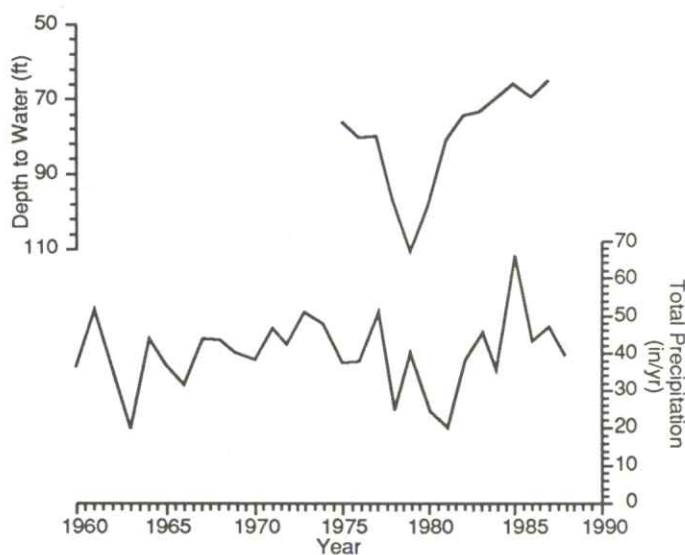
FIGURE 3—HYDROGRAPH FOR WELL 34S, 25E, 13BAC [1150 FT (351 M)], CHEROKEE COUNTY, ROUBIDOUX AQUIFER.
