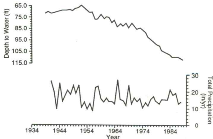
FIGURE 5—HYDROGRAPH FOR WELL 24S, 32W, 03DAC [185 FT (56.4 M)], FINNEY COUNTY, PLEISTOCENE WELL.
