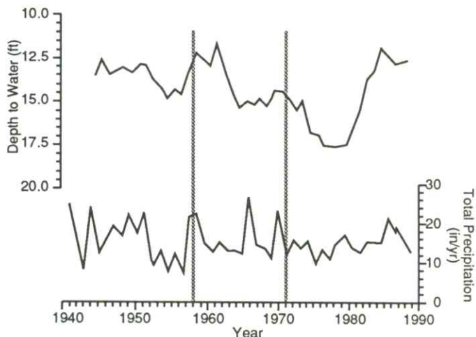
FIGURE 6—HYDROGRAPH FOR WELL 23S, 43W, 21ABA [29 FT (8.8 M)], HAMILTON COUNTY, ALLUVIAL WELL.
