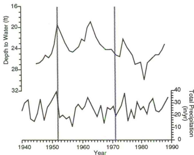
FIGURE 8—HYDROGRAPH FOR WELL 20S, 33W, 09BBB [128 FT (39.0 M)], SCOTT COUNTY, OGALLALA FORMATION.
