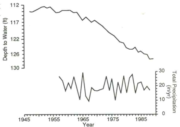
FIGURE 10—HYDROGRAPH FOR WELL 08S, 34W, 01BAC [160 FT (48.8 M); THOMAS COUNTY, OGALLALA WELL] SHOWING EFFECT OF PRECIPITATION RECHARGE ON WATER LEVELS.
