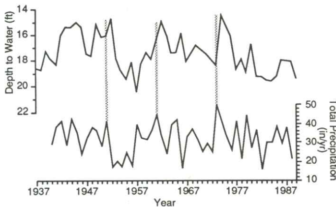
FIGURE 9—HYDROGRAPH FOR WELL 25S, 01W, 26DAD [54 FT (16 M); SEDGWICK COUNTY, PLEISTOCENE WELL] SHOWING EFFECT OF PRECIPITATION RECHARGE ON WATER LEVELS.
