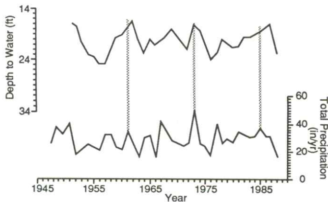
FIGURE 4—HYDROGRAPH FOR WELL 12S, 20E, 17CCB [50 FT (15 M); DOUGLAS COUNTY, PLEISTOCENE WELL] SHOWING EFFECT OF PRECIPITATION RECHARGE ON WATER LEVELS.
