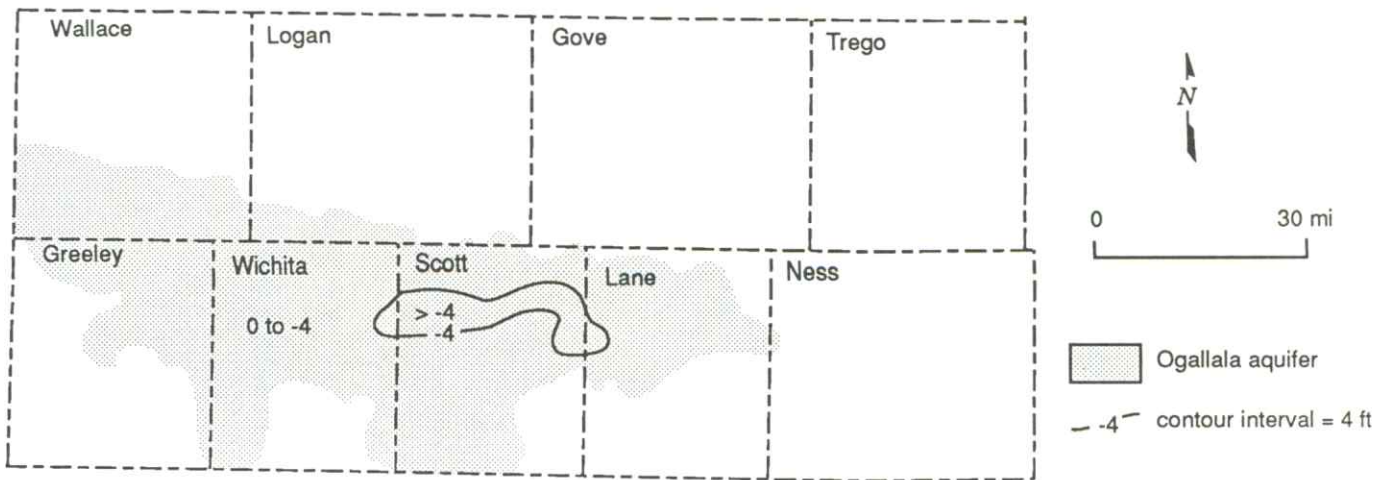
FIGURE 12—MAP OF GENERALIZED WATER-LEVEL DECLINE FOR REGION II, WEST-CENTRAL KANSAS, 1988-89.
