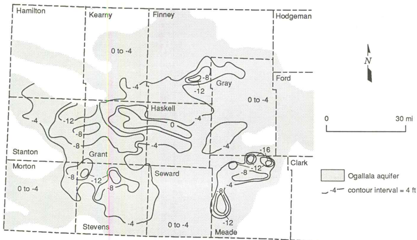
FIGURE 11—MAP OF GENERALIZED WATER-LEVEL DECLINE FOR REGION I, SOUTHWEST KANSAS, 1988–89.
