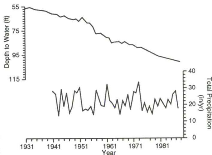
FIGURE 8—HYDROGRAPH FOR WELL 20S, 33W, 09BBB [128 FT (39.0 M)], SCOTT COUNTY, OGALLALA FORMATION.
