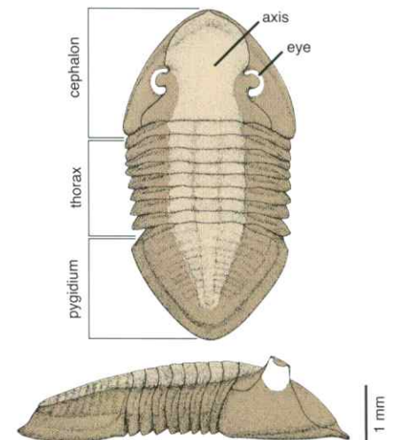
FIGURE 61—Two views of the Ordovician trilobite Isotelus , showing the basic divisions of the carapace, or external skeleton (adapted from Whittington, 1997, fig. 157).
