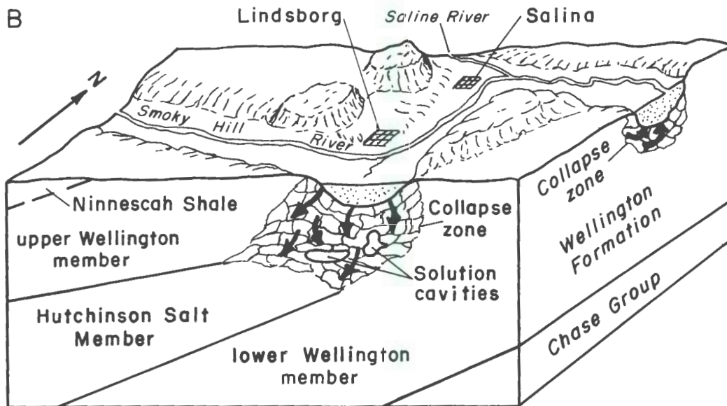
Figure 4.--Conceptual block diagrams near Lindsborg showing geologic development, mechanism of dissolution of the Hutchinson Salt Member, and development of Wellington aquifer between Cretaceous time (A) and present (B).
