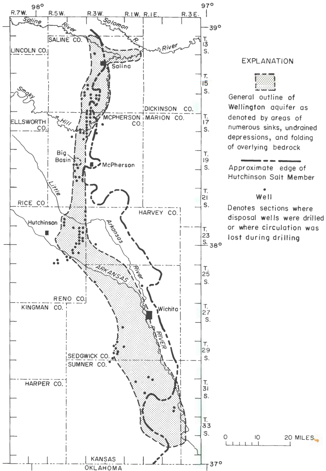
Figure 5.--General outline of Wellington aquifer as denoted by areas of sinks and undrained depressions, locations of disposal wells, and areas where lost circulation was reported.
