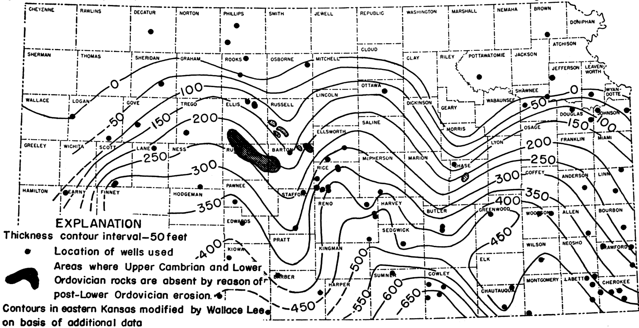
Fig. 9--Thickness of the Jefferson City-Cotter sequence in Kansas.
