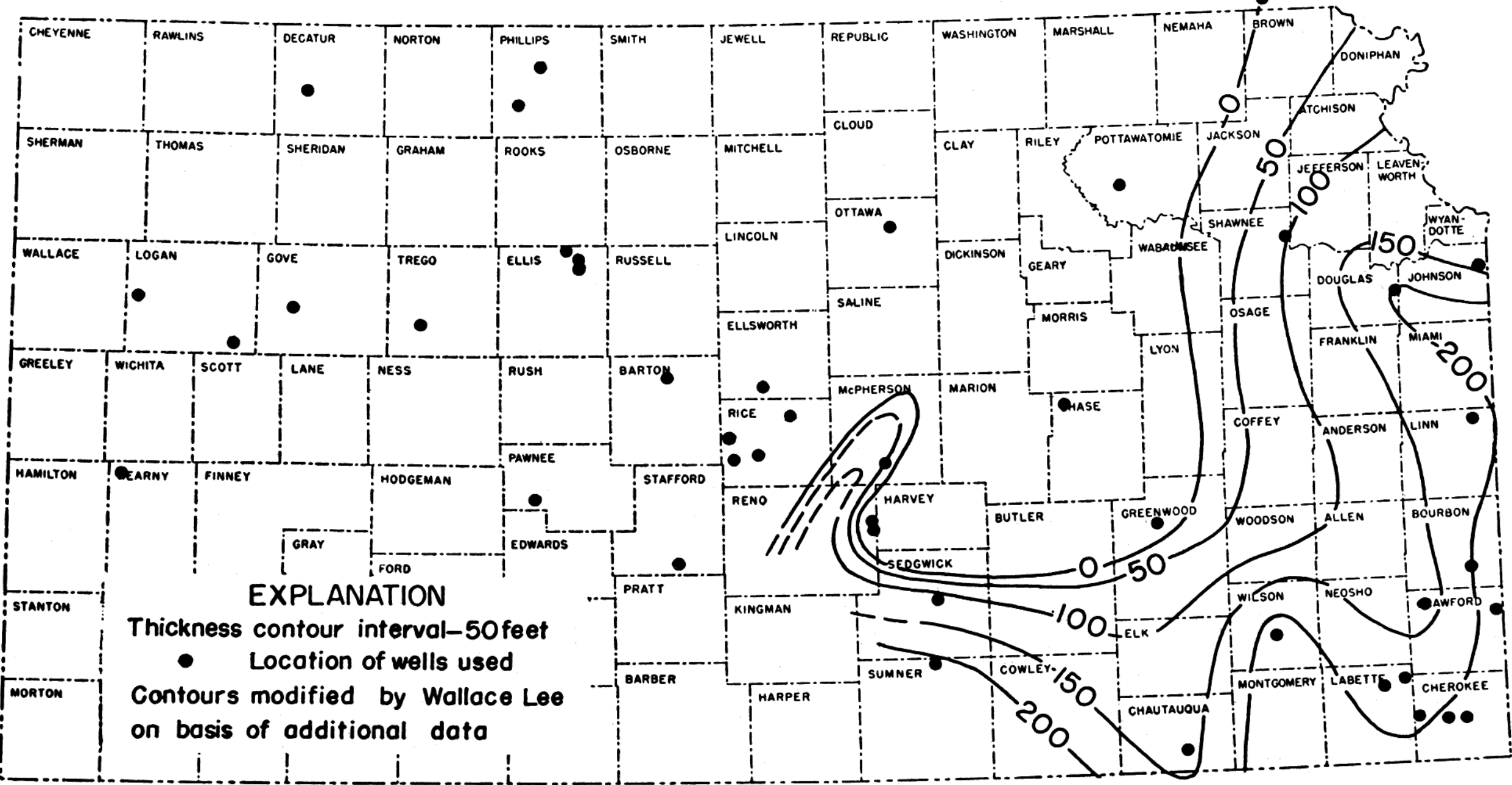
Fig. 6--Thickness of the Van Buren-Gasconade sequence in Kansas.
