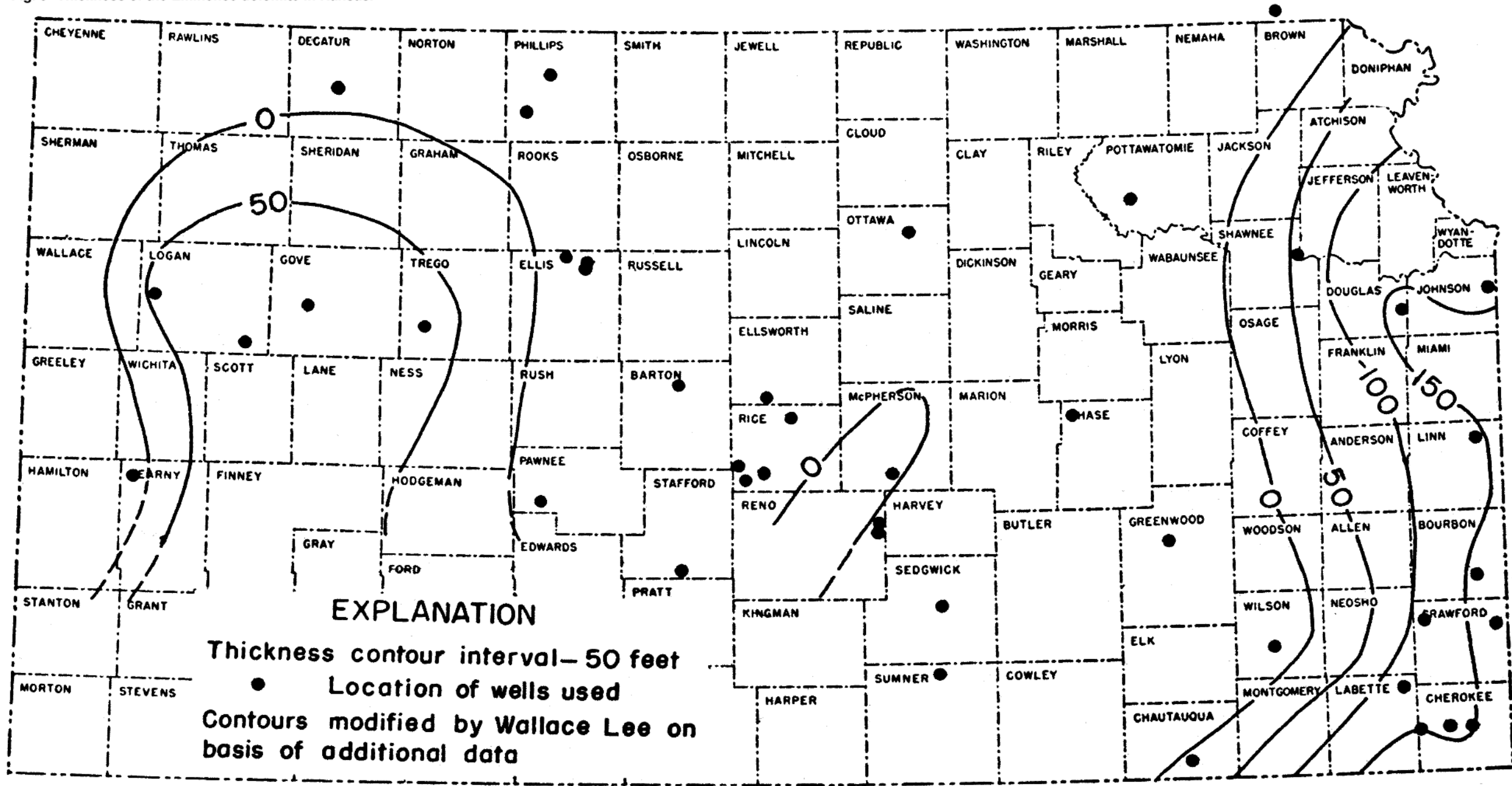
Fig. 5--Thickness of the Eminence dolomite in Kansas.
