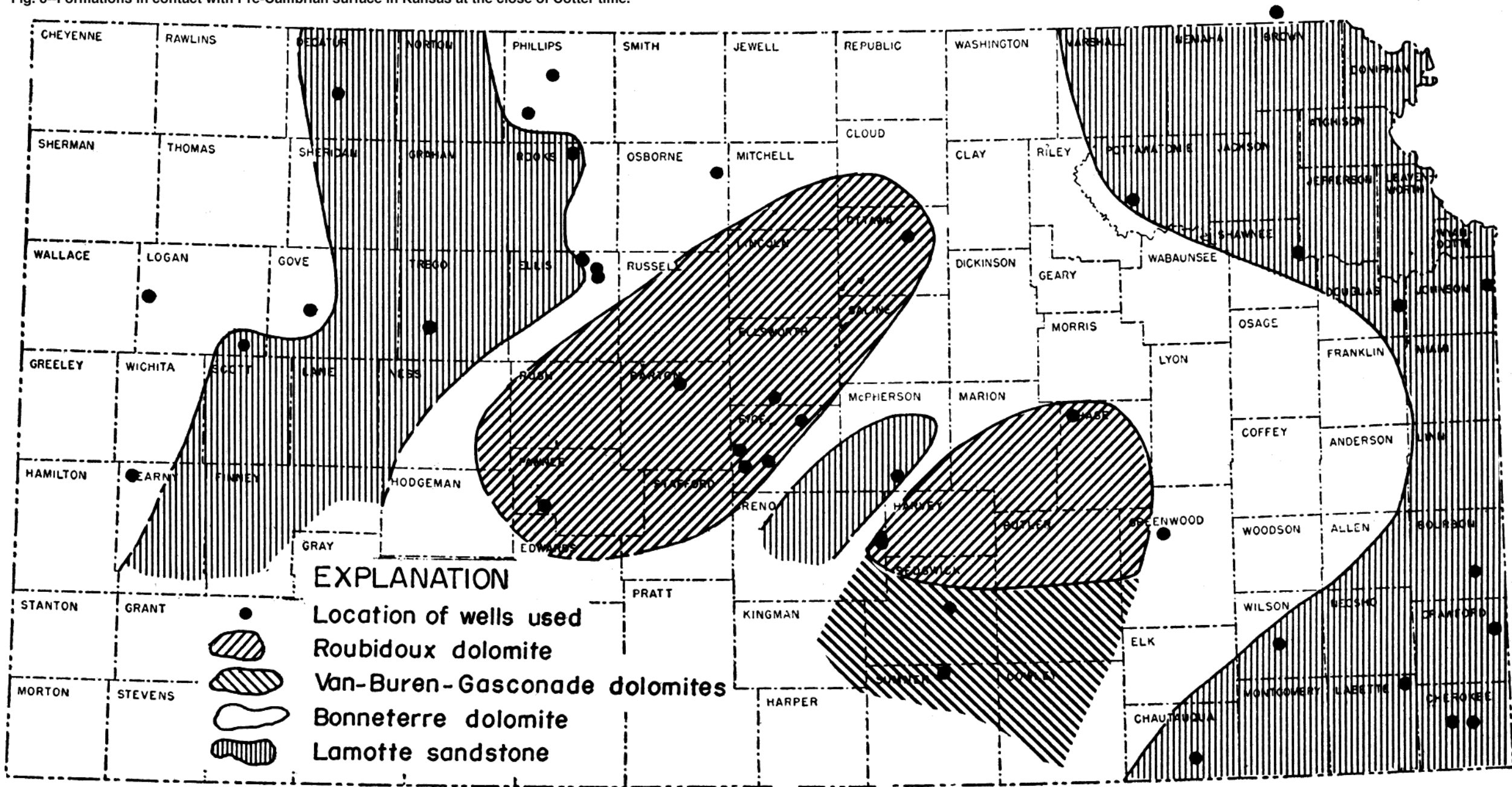
Fig. 3--Formations in contact with Pre-Cambrian surface in Kansas at the close of Cotter time.
