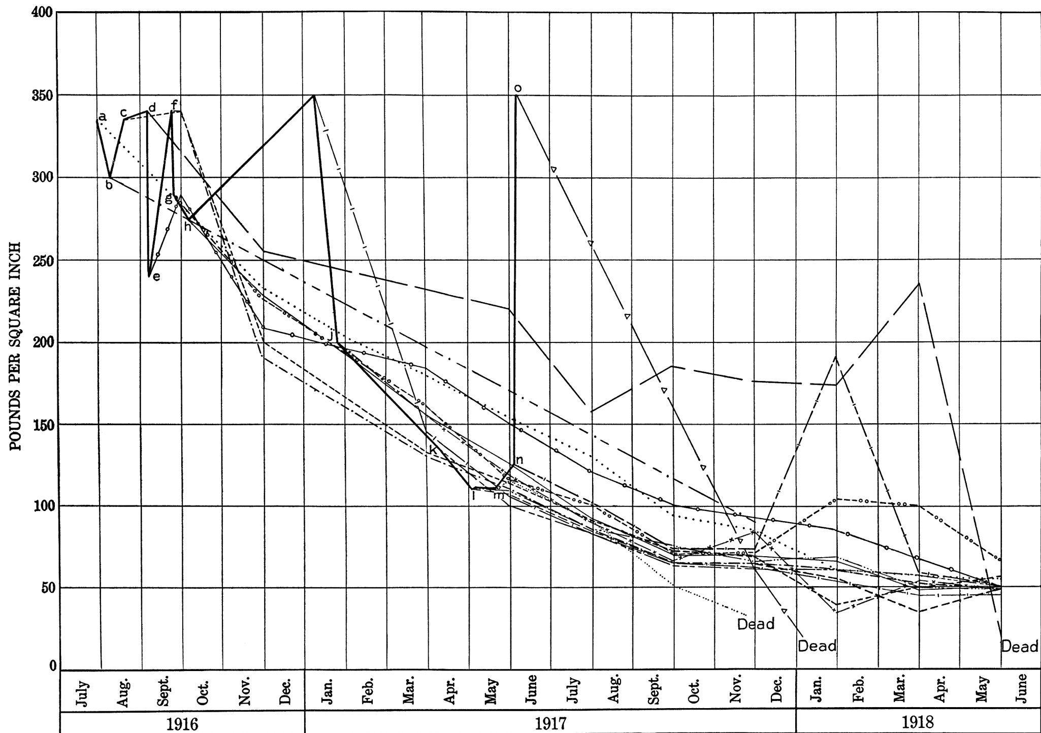
PLATE XVI.—Graphs showing declines in closed rock pressure of sixteen 900-foot "sand" gas wells on the Boyer dome.
