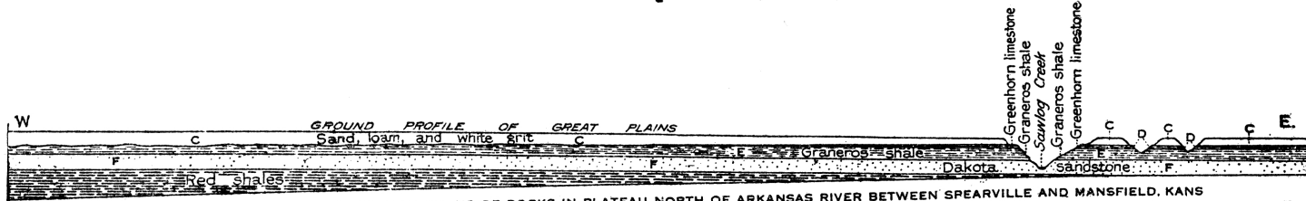
SECTION SHOWING UNDERGROUND RELATIONS OF ROCKS IN PLATEAU NORTH OF ARKANSAS RIVER BETWEEN SPEARVILLE AND MANSFIELD, KANS [U.S.G.S BULL. 613] VERTICAL SCALE GREATLY EXAGGERATED. THIS HAS EFFECT OF INCREASING APPARENT TILT OF BEDS
