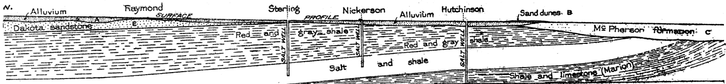
SECTION SHOWING UNDERGROUND RELATIONS OF ROCKS ALONG SANTA FE RAILWAY BETWEEN PAXTON AND ELLINWOOD, KANS. [U.S.G.S. BULL. 613] VERTICAL SCALE GREATLY EXAGGERATED THIS HAS EFFECT OF INCREASING APPARENT TILT OF BEDS
