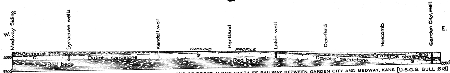
SECTION SHOWING UNDERGROUND RELATIONS OF ROCKS ALONG SANTA FE RAILWAY BETWEEN GARDEN CITY AND MEDWAY, KANS [U.S.G.S. BULL. 613]
