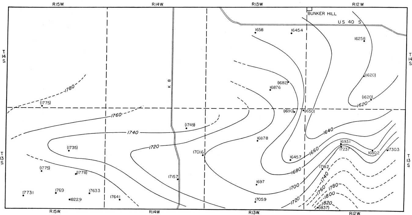
FIG. 7. Contour map of southern Russell county showing the configuration of the pressure-indicating surface of water in the uppermost sandstone beds of the Dakota formation. Dots represent locations of wells, and figures are altitudes of the water level, in feet. Figures enclosed in parentheses are based on altitudes determined from topographic maps of the U. S. Geological Survey; others are based on instrumental levels. Contour interval 20 feet.
