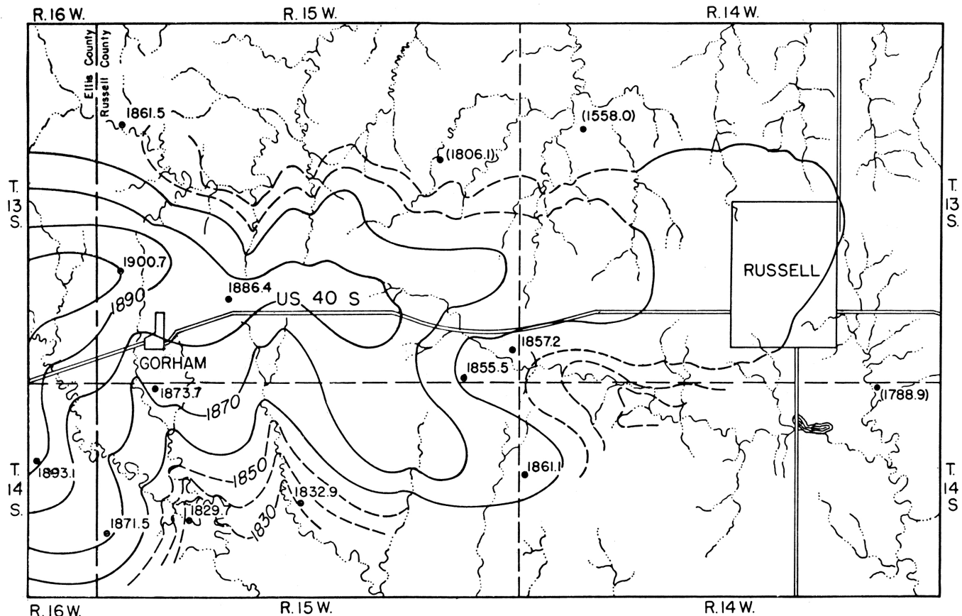
FIG. 4. Contour map showing configuration of the water table in Tertiary deposits west of Russell. Dots represent locations of wells; figures are altitudes of the water levels, in feet. Figures enclosed in parentheses indicate wells that end in alluvium. Contour interval 10 feet.
