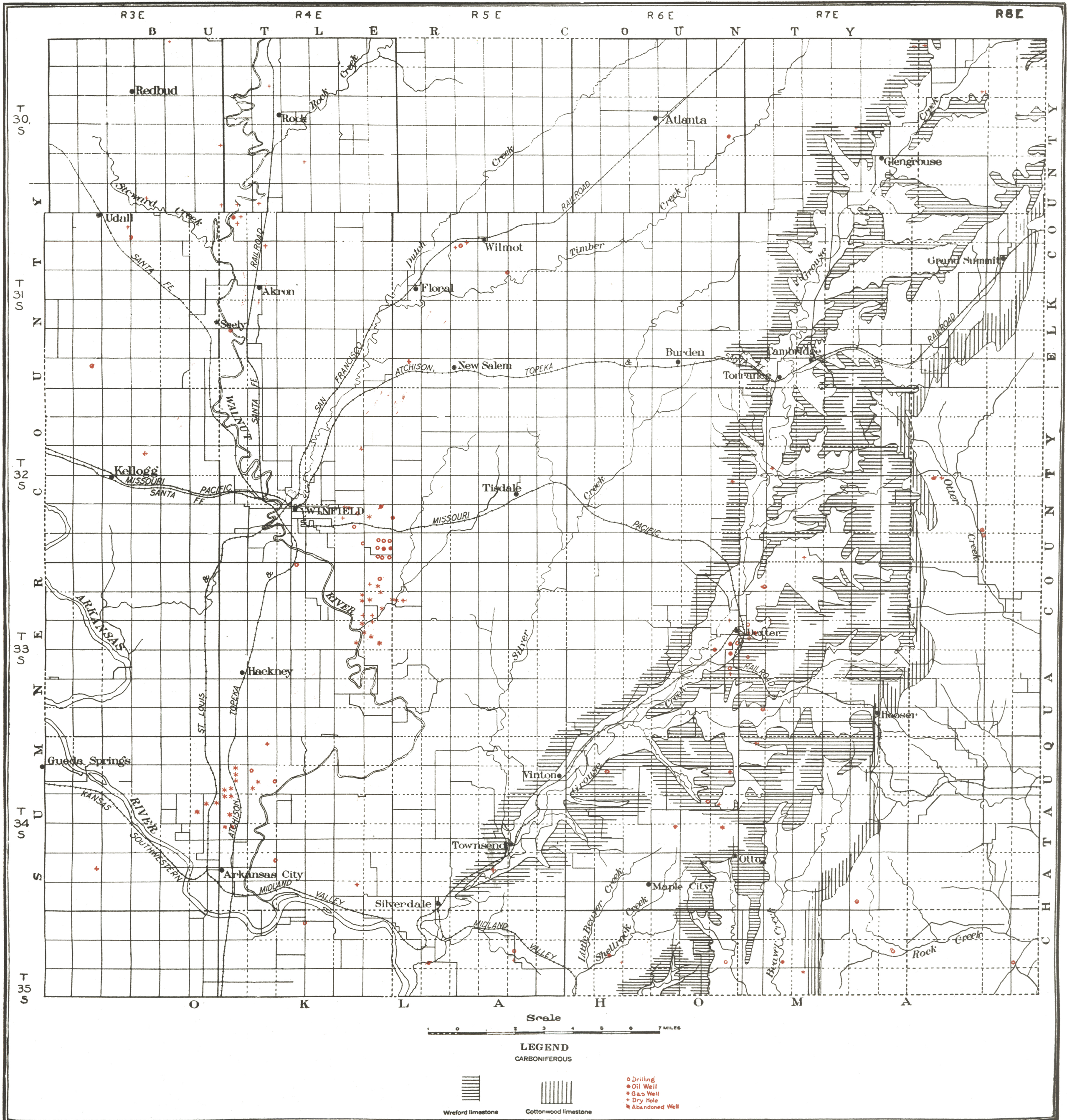
Map of Cowley county, showing outcrop of Cottonwood and Wreford limestones and location of oil and gas wells. (Geology after Haworth and Bennett.)
