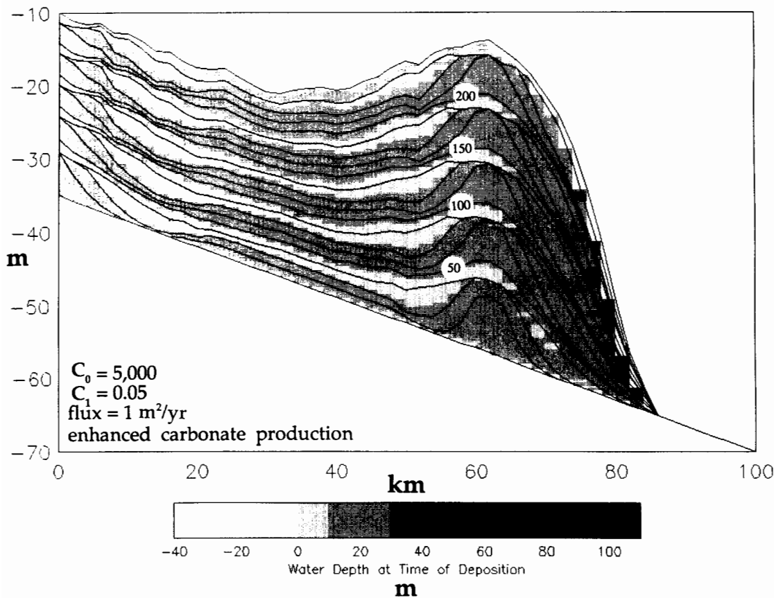
Figure 13. Mixed siliciclastic-carbonate shelf illustrating the combined effects of three zones of sediment production and lateral dispersal. There is a sediment flux from the left-hand side simulating siliciclastic input, flux from below between 20 km and 50 km to simulate lagoonal production, and enhanced flux between 60 km and 64 km to simulate reef growth. A 10-m-amplitude sea-level curve is used. See text for discussion.
