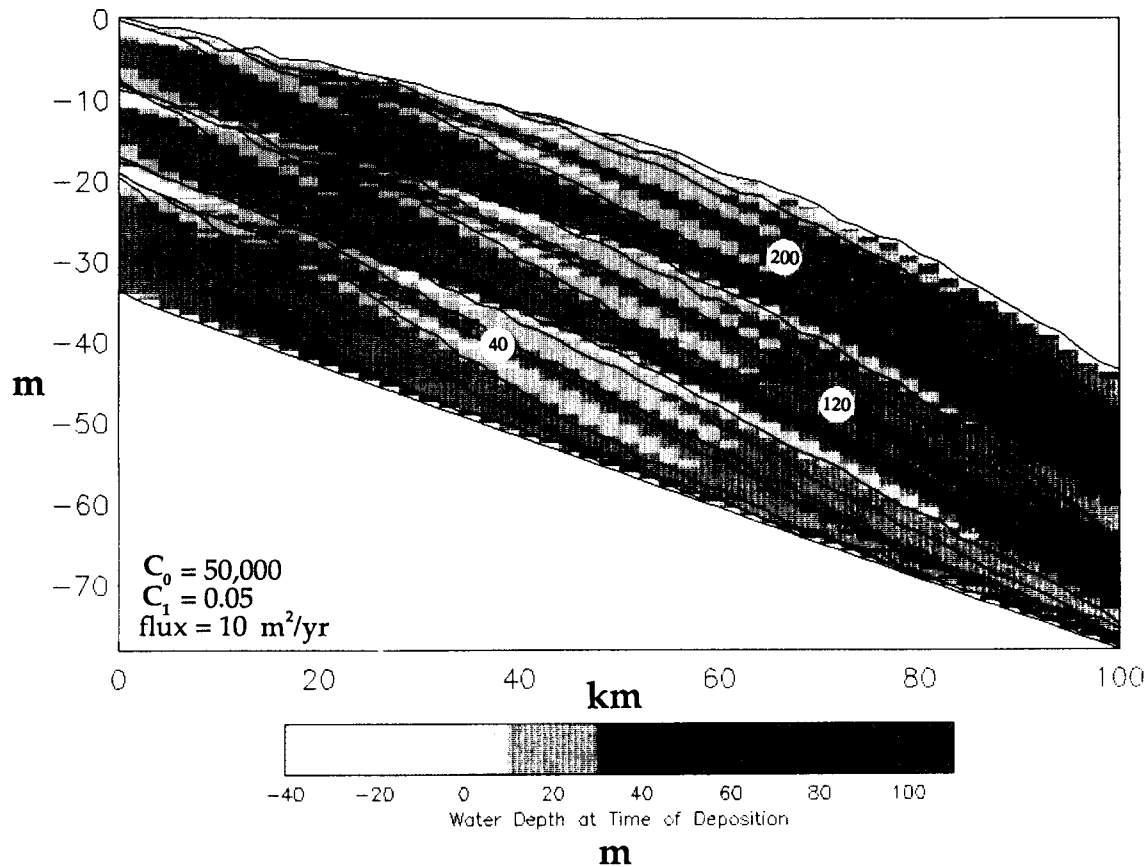
Figure 14. Sediment bypassing associated with complex sea-level oscillation history. Times lines are drawn every 10 k.y. Note development of discrete lenses and complex wedges of shallow-water sediments enclosed in deeper-water sediments. Also, bypassing is maximized during times of sea-level lowstand and not at times of maximum rate of fall.
