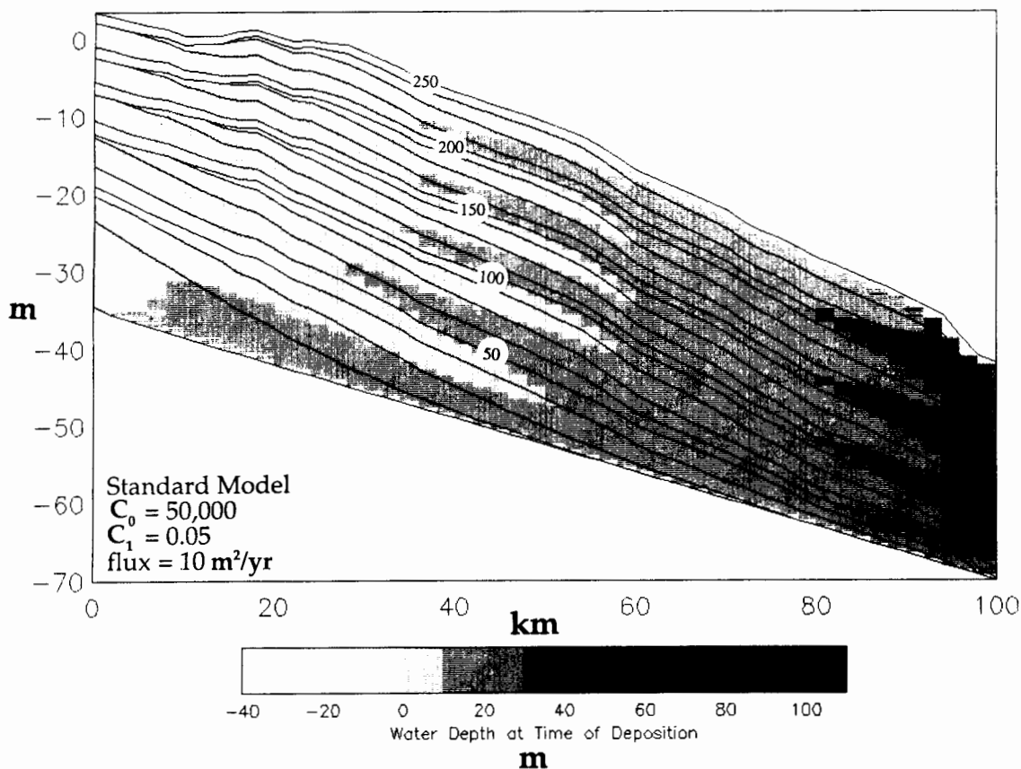
Figure 2. Standard run showing effects of depth dependency on sediment transport. All parameters of the standard model are shown in table 1. Lines within the plots are time lines spaced at intervals of 12.5 k.y. Time lines in all subsequent plots except fig. 14 are spaced at identical intervals. Numbers along time lines within plots indicate the age in kiloyears since beginning of model run. The time line to which the date belongs corresponds to the time line that forms the diameter of the white circle. Note truncation of time lines on the landward end of the profile, indicating erosion during lowstands when D is highest. An example of a surface of maximum truncation occurs along the 87.5-k.y. time line at the lowstand in the sea-level curve, not at the inflection point (time of maximum rate of fall), which occurs at 75 k.y.
