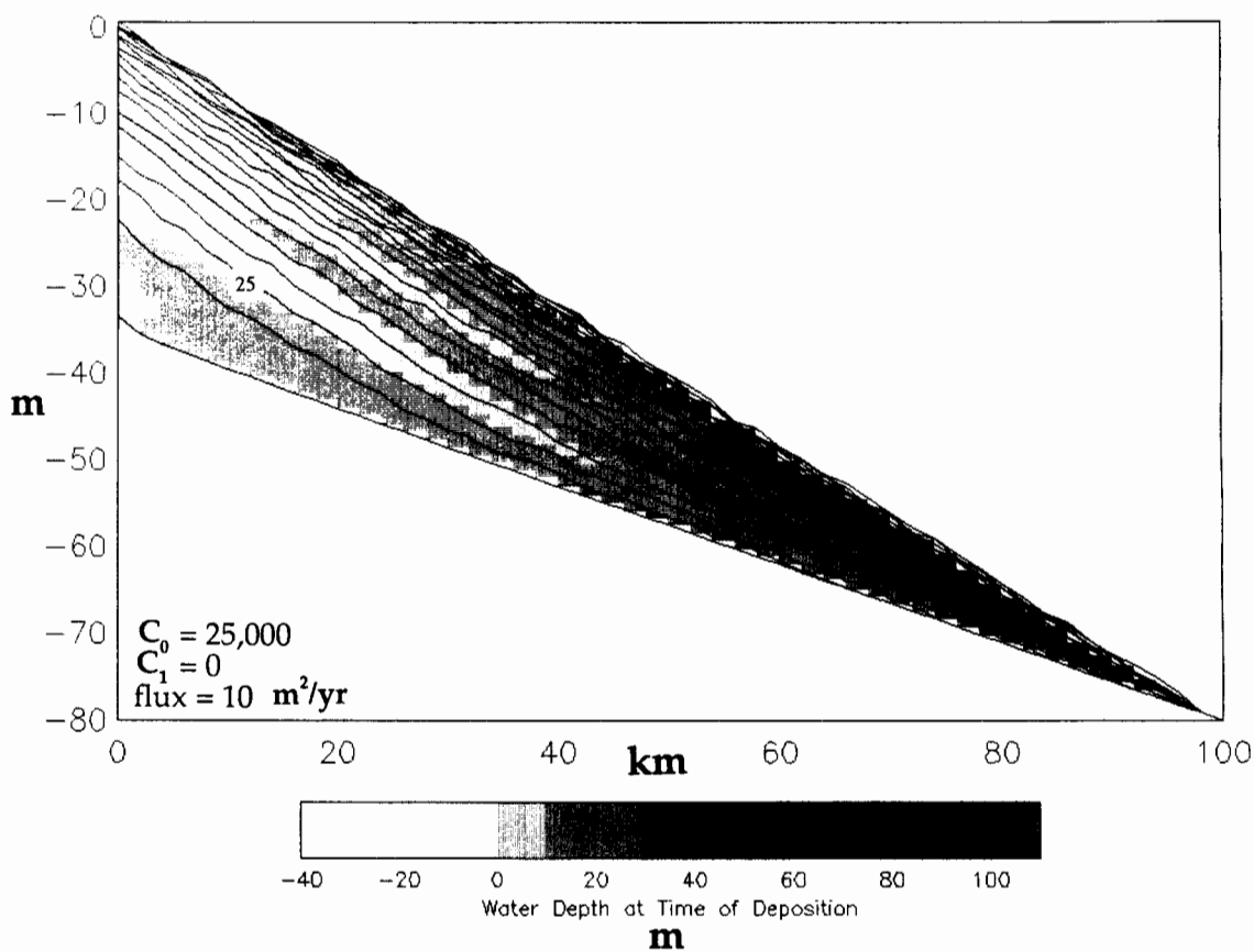
Figure 4. The effect on sediment dispersal patterns when C_1 = 0 and C_0 = 25,000 . In this case D has no dependence on water depth. Sedimentary facies belt migrates in phase with sea-level variations. Compare with fig. 2, where all other parameters are the same except for C_1 and a 10-m-amplitude sea-level curve.
