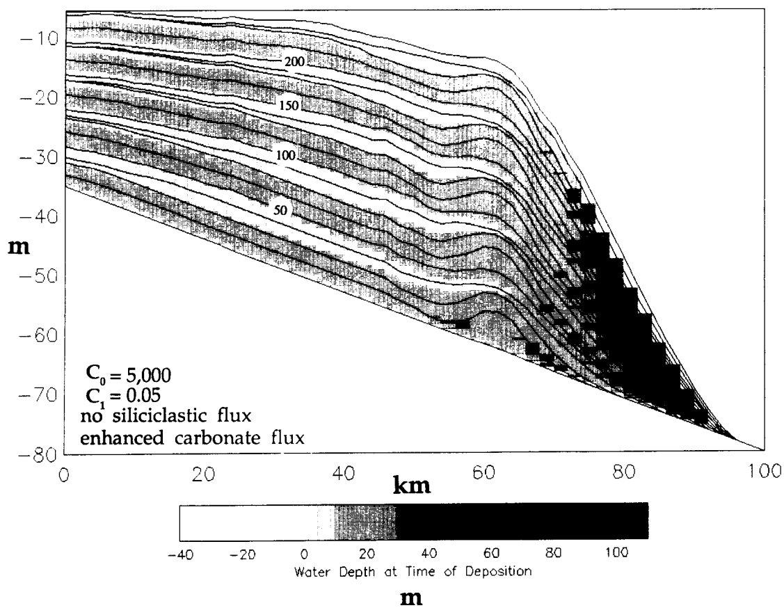
Figure 12. Rimmed carbonate shelf highlighting enhanced carbonate production at the shelf edge between 60 km and 64 km. A 10-m-amplitude sea-level curve is used. See text for discussion.
