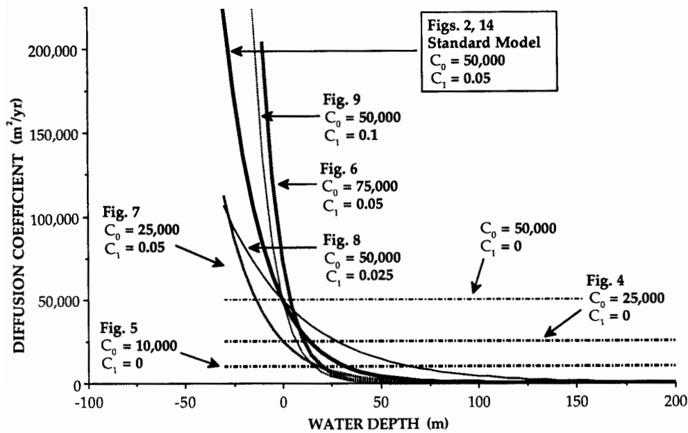
Figure 1. Relationship between water depth and diffusion coefficient D for D = C_0 e^{-C_1 W} , as discussed in text. These curves apply to the siliciclastic model runs. Because of the exponential form of the curves, D is sensitive to small changes in water depth in shallow regions, tapering off sharply at deeper water depth. Increasing C_0 effectively increases the efficiency of the diffusion process and, by implication, lateral transport of sediment. Increasing C_1 causes D to decay more sharply with water depth; this decreases the efficiency of the diffusion process at greater depths. As C_1 is decreased, the disparity between sediment transport efficiency at different depths is significantly decreased. When C_1 = 0 , D is a constant and independent of water depth.
