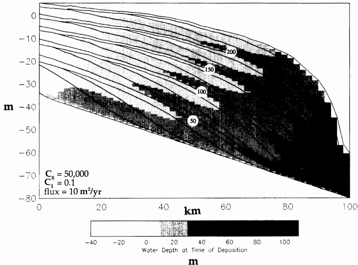
Figure 9. Model run with C_1 increased to 0.1. Note the pronounced increase of shelf gradients into deeper water resulting from the dependence of D on water depth. Compare with fig. 8. See text for further discussion.
