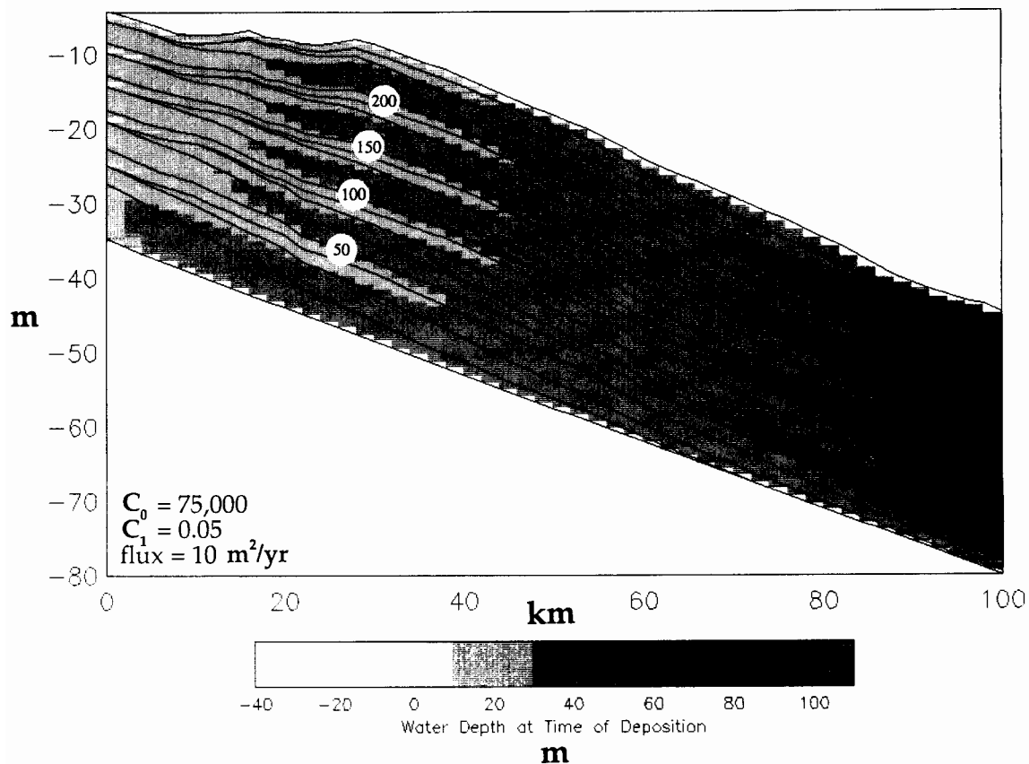
Figure 6. Model run in which C_0 is increased to 75,000 and all other parameters are as in the standard model, including a value of 0.05 for C_1 . Because C_1 is now greater than 0, D depends on water depth. Note how the high value of C_0 results in highly aggradational, tabular deposits.
