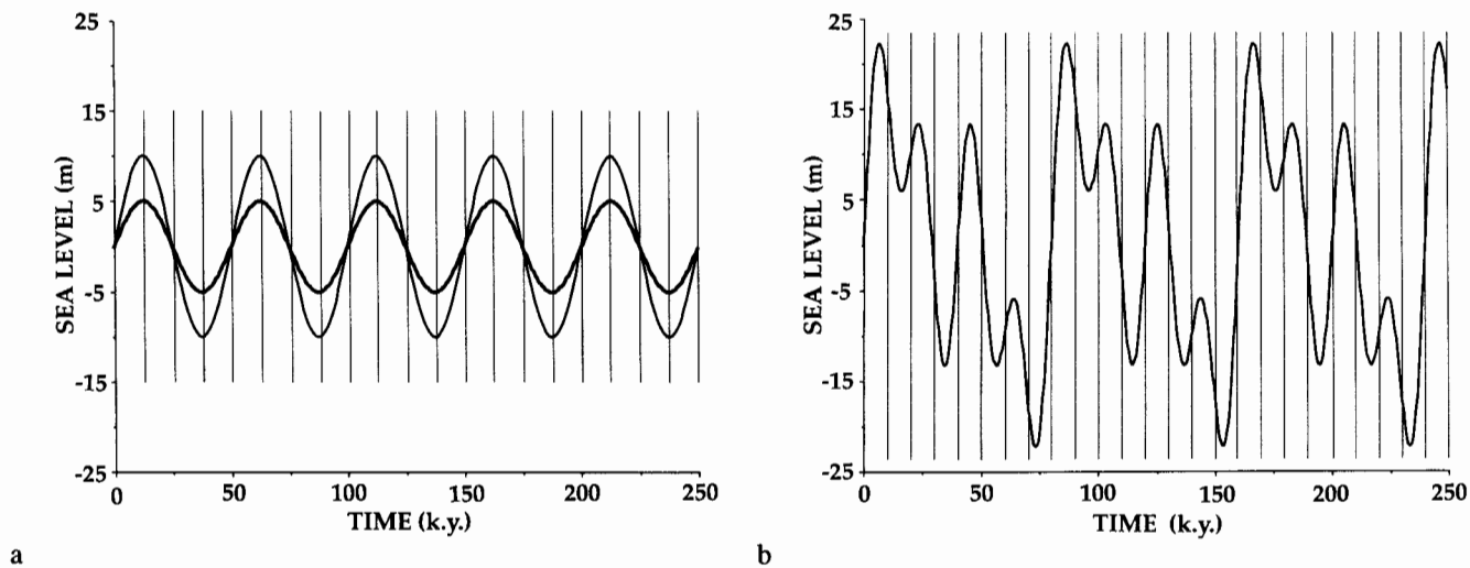
Figure 3. (a) Model sinusoidal sea-level curves with 5 m and 10 m amplitude and constant periods of 50 k.y. Vertical lines correspond to the time lines on the model plots at intervals of 12.5 k.y. (b) A compound sea-level curve, used exclusively for fig. 14, that consists of 3 sinusoids, each with an amplitude of 10 m and periods of 20 k.y., 40 k.y., and 80 k.y. Vertical lines correspond to the time lines in fig. 14 at intervals of 10 k.y.
