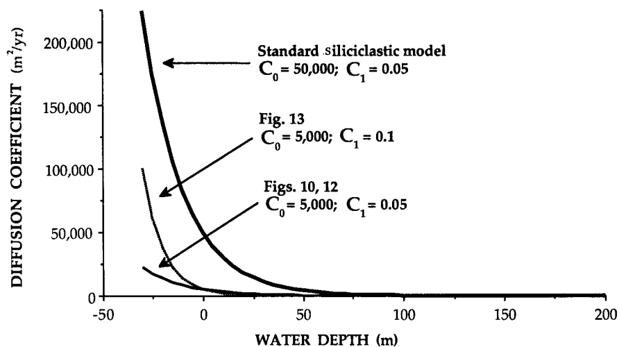
Figure 11. Comparison of diffusion coefficient with water depth used in the carbonate model runs. The standard siliciclastic model curve is plotted for comparison (cf. fig. 1). Lower values of C_0 result in a much lower diffusion coefficient at a given depth and thus in much slower sediment dispersal. This condition is used to mimic early cementation of carbonate materials.
