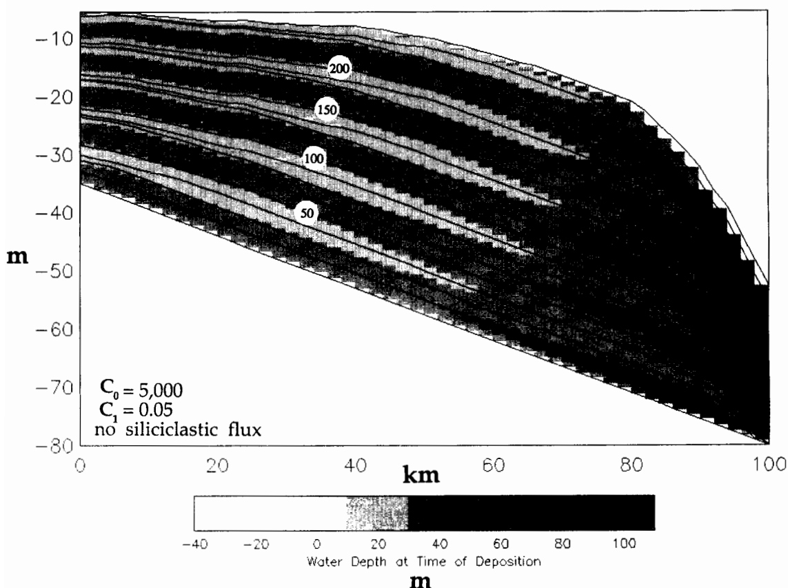
Figure 10. Distally steepened carbonate ramp formed by in situ depth-dependent sediment production and simultaneous restricted lateral sediment transport. A 10-m-amplitude sea-level curve is used. See text for discussion.
