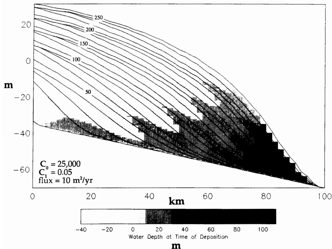
Figure 7. Model run with conditions the same as in fig. 6, except that C_0 is decreased to 25,000. Note the enhanced wedge shape of the deposits, concave-down slopes, and progradational facies patterns.
