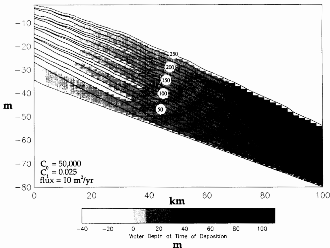
Figure 8. Model run showing effect of decreasing C_1 to 0.025. See text for discussion.
