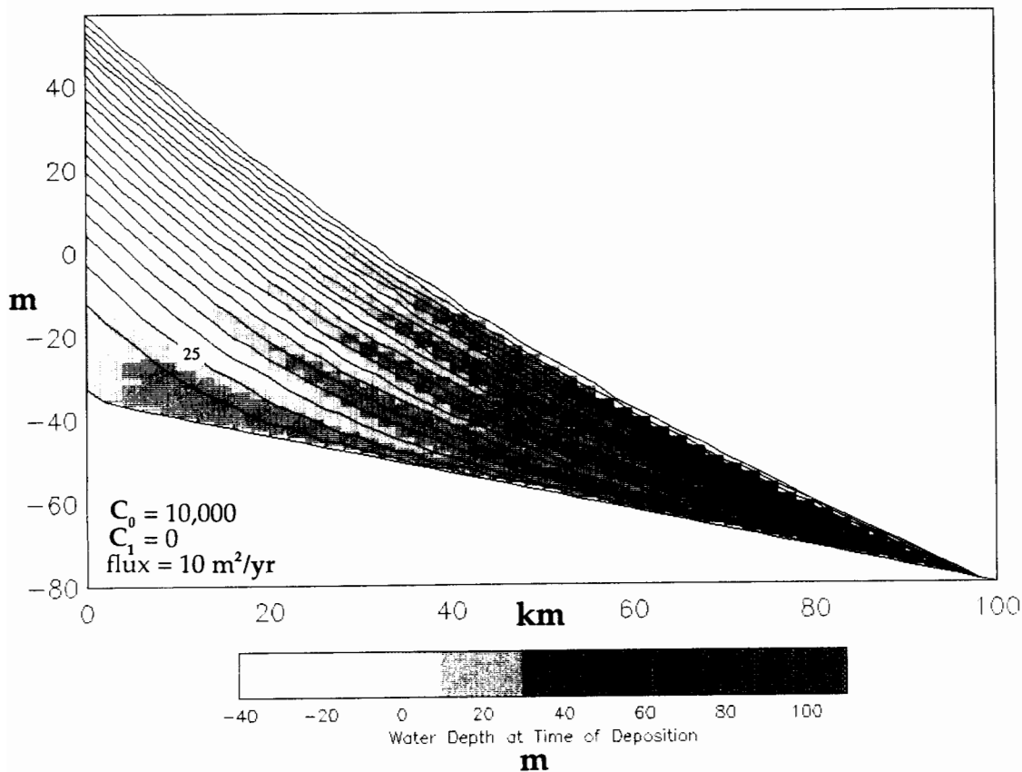
Figure 5. Model run with C_1 = 0 and C_0 decreased to 10,000. This results in less efficient dispersal of sediment and an increase in depositional slope and shallowing to persistent alluvial sedimentation. Compare with fig. 4, where slopes are less steep and sediments are deposited in deeper water on average. A 10-m-amplitude sea-level curve is used.
