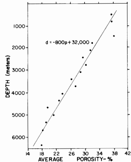
Figure 4. Porosity versus depth of late Tertiary sandstones from Louisiana, US Gulf Coast. The 17,367 analyses have been averaged in thousand-foot intervals for calculation of the least-squares fit. Unfortunately, no error estimates or petrology are available. Unpublished data of G. I. Atwater and E. E. Miller (1965); from Blatt (1979, p. 146).
