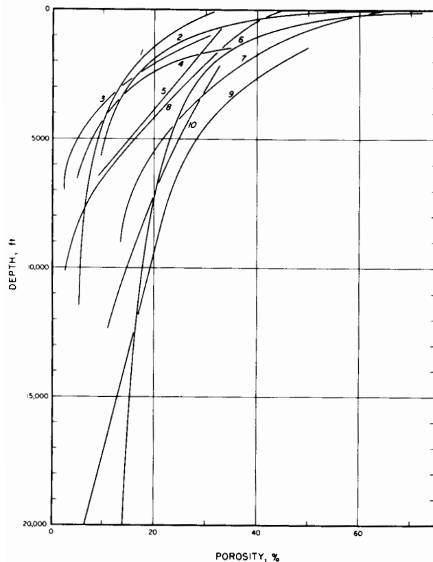
Figure 3. Representative fitted curves of porosity versus depth in mudrock. Locations: (1) Ciscaucasus, USSR. (2) Compilation, Tertiary and Quaternary. (3) Oklahoma, USA, Pennsylvanian and Permian. (4) Japan, Tertiary. (5) Venezuela, Tertiary. (6) Gulf Coast, USA, Tertiary. (7) Japan. (8) Compilation, mainly of locations 3 and 5. (9) Gulf Coast, USA, Tertiary. (10) Gulf Coast, USA, Tertiary. From Rieke and Chilingarian (1974, p. 42); references are given therein.
