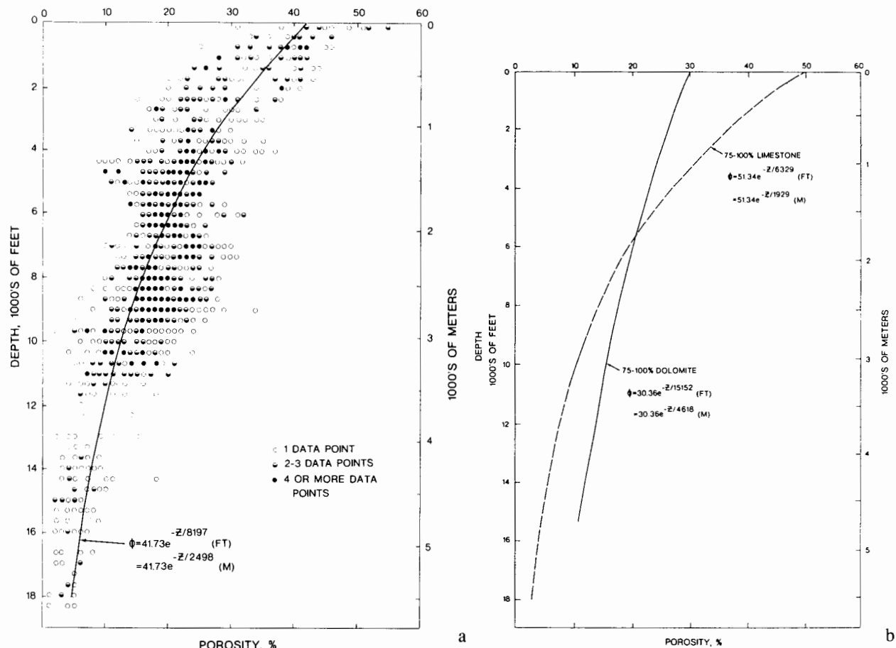
Figure 6. (a) Porosity versus depth from shallow-water carbonates, Pleistocene to Early Cretaceous in age, from south Florida. N = 1,302 ; 167 data points are gravity data from boreholes at shallow depths; the remainder are data points from porosity logs. From Schmoker and Halley (1982, p. 2,566). (b) Data from part a separated into dolomites (75–100% dolomite; N = 336 ) and limestones (75–100% CaCO 3 ; N = 489 ). From Schmoker and Halley (1982, p. 2,569).
