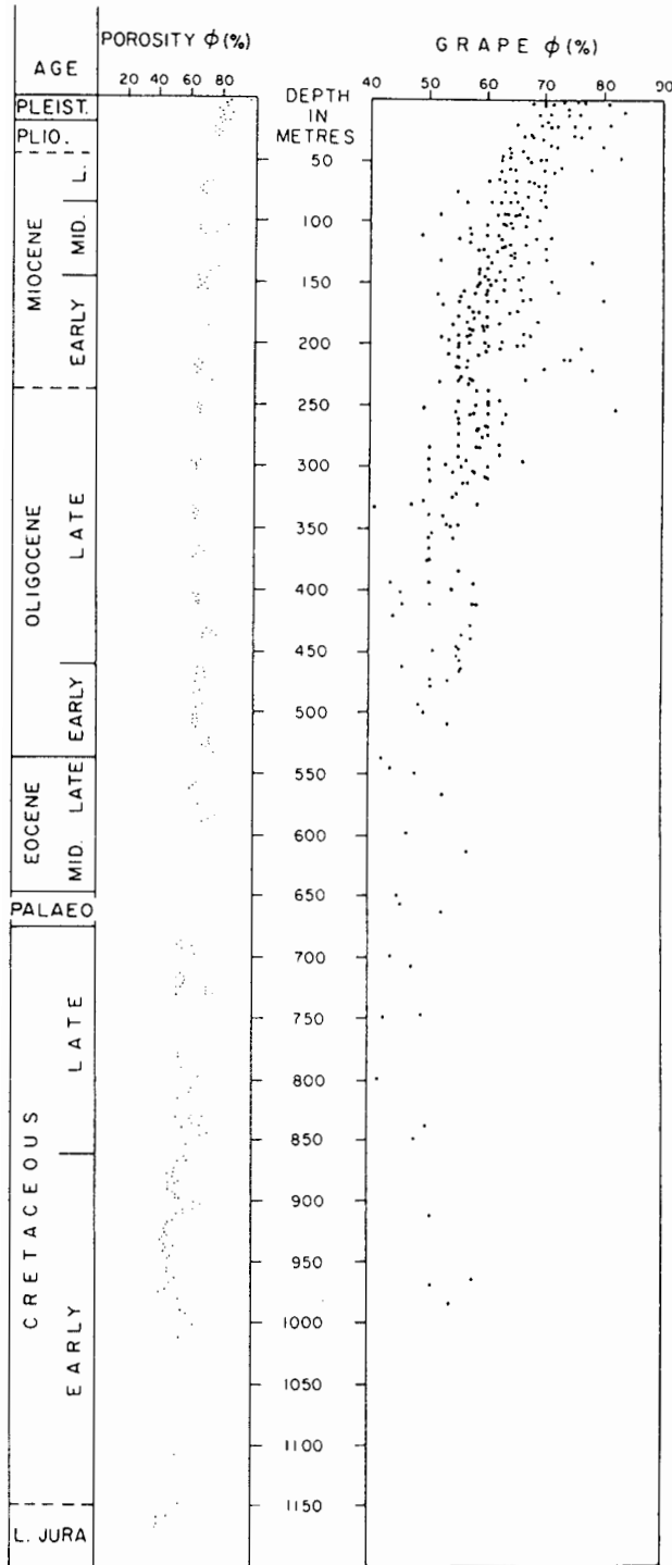
Figure 5. Porosity and depth in pelagic carbonates from the Pacific and Indian oceans. The left column is from Deep Sea Drilling Project (DSDP) site 167, Magellan Rise, central North Pacific. The right column has samples with 80% or more calcium carbonate from 11 other DSDP sites. Note that the ages apply only to site 167 (left-hand column). From Schlanger and Douglas (1974, p. 119).
