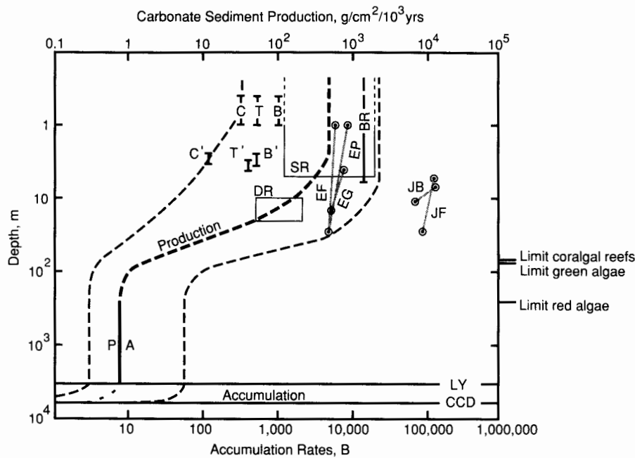
Figure 2. Carbonate sediment production as a function of depth. This curve is a hybrid, as were the original attempts to illustrate depth-related variations (Garrison and Fischer, 1969, fig. 22; Wilson, 1975, fig. I-2); those curves have nevertheless proved fertile. This attempt to quantify the curve encountered a paucity of data on in situ production, especially at intermediate depths. These are needed to document the thresholds related to algal productivity, stressed by R. N. Ginsburg [cf. Wilson (1975) and Schlager (1981)], and the lower limit of coral-algal reef growth ( \approx 70 m; James, 1977). In contrast, data on sedimentation rates, as opposed to production rates, in shallow-water and abyssal settings are abundant (table 1). Data used in constraining the curve are: BR, productivity of a Barbados reef in a sheltered setting (Stearns et al., 1977). SR, compilation of accretion rates ( \text{mm}/10^3 \text{ yr} ) of reefs at less than 5 m (15 ft) depths (Schlager, 1981). DR, compilation of accretion rates of reefs at 10–20 m (30–65 ft) depth (Schlager, 1981). EF, EG, and EP, regressions of growth rate versus depth for three species of corals in Enewetak Atoll (Highsmith, 1979). JF and JB, regressions of growth rate versus depth of Acropora cervicornis on the fore reef and back reef, respectively, in Jamaica (Tunnicliffe, 1983); these are linear growth rates of a branching coral, so they do not constrain accretion rates, but they should help define the variation with depth. C, T, and B, total productivity of carbonate mudbanks with varying degrees of restriction in south Florida [Upper Cross Bank, Tavernier Key, and Buchanan Banks, respectively (Bosence, 1988, 1989)], paired with productivity from adjacent interbank areas ( C' , T' , B' ). PA, accumulation rates of pelagic carbonates from the equatorial Pacific; average for last million years and range for past 45 m.y. (van Andel et al., 1975). LY, the lysocline, a threshold of accelerated carbonate dissolution with depth, currently about 3,500–4,800 m (11,000–16,000 ft) (Scholte et al., 1983). CCD, the carbonate compensation depth, which ranges from <4,000 m ( <13,000 ft) to >5,000 m ( >16,000 ft) in the present oceans (Berger and Winterer, 1974). Benthic production is assumed to approach 0 with the disappearance of red algae at depths of approximately 250 m (800 ft). Pelagic production is a function of surface conditions, so it is shown constant with depth. Pelagic accumulation rates are affected primarily by dissolution on the seafloor. They decrease sharply below the lysocline and drop to 0 at the carbonate compensation depth. The conversion from production rates in grams per square centimeter per 1,000 years to sedimentation rates in Bubnoffs ( \text{mm}/10^3 \text{ yr} ) varies with the porosity and mineralogy of the sediment; for example, 1 \text{ g}/\text{cm}^2/10^3 \text{ yr} would equate to a sedimentation rate of 14.7 B for calcitic sediment with 75% porosity (mud), but only 8.5 B of aragonitic sediment with 40% porosity (sand). The conversion used, 10 \text{ B} = 1 \text{ g}/\text{cm}^2/10^3 \text{ yr} , would apply to aragonitic sediment with about 65% porosity.
