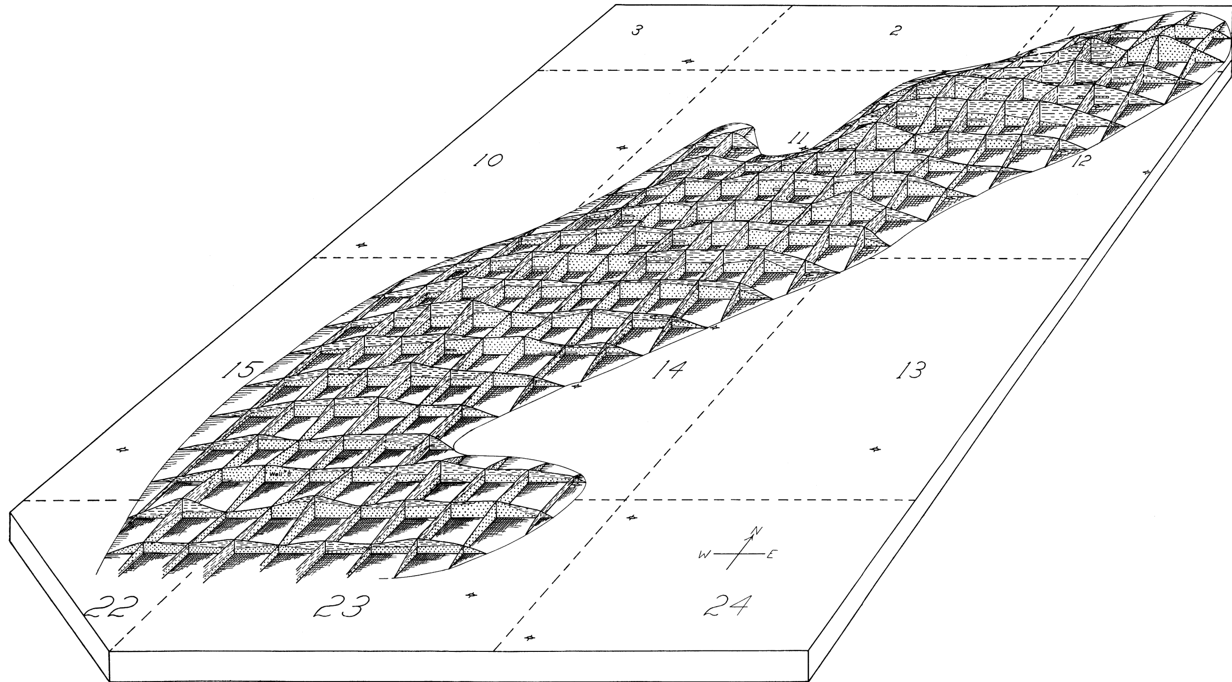
PLATE 11.—Block diagram of the producing sand in the Madison oil field, T. 22 S., R. 11 E., Greenwood county.
