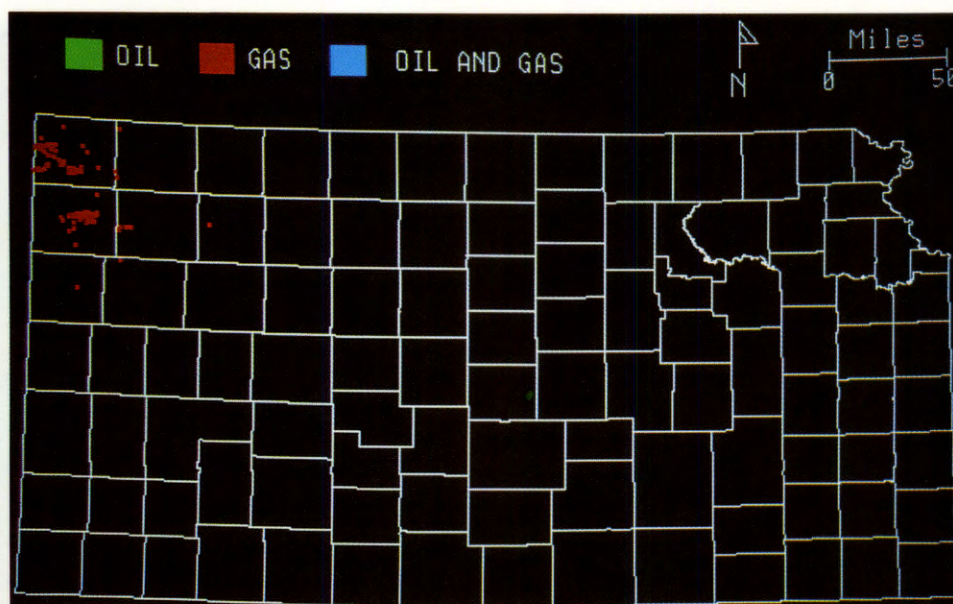
FIGURE 16—MESOZOIC. Mesozoic gas comes from porous chalks of the Cretaceous Niobrara Formation. The chalks produce from small low-relief structures in the northwestern part of the state (Pollastro and Scholle, 1984). Significant commercial exploration of the Niobrara gas in northwestern Kansas has been active only since the early 1970's. It is expected that the production limit of the Mesozoic gas fields in Kansas could be considerably extended over the next few years.
