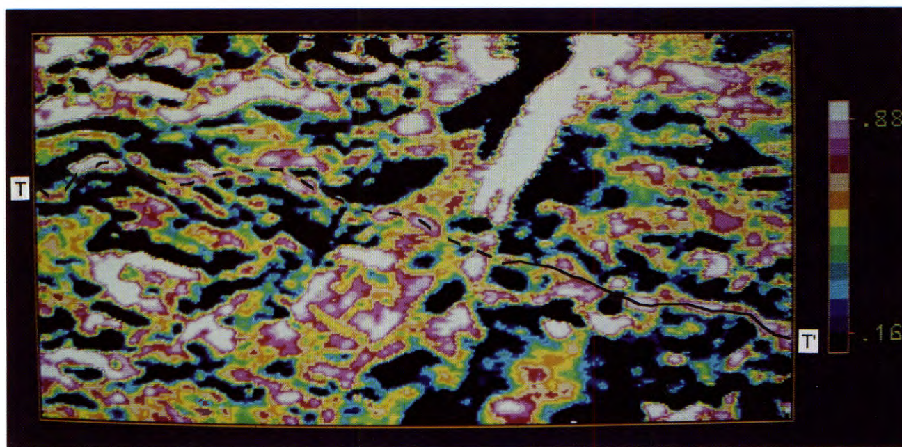
FIGURE 12—OBLIQUE ILLUMINATION OF GRAVITY WITH THE SUN AT 30^\circ ABOVE THE HORIZON AND AN AZIMUTH OF 180^\circ . Gravity-to-distance factor is 0.75 mgal/km.
