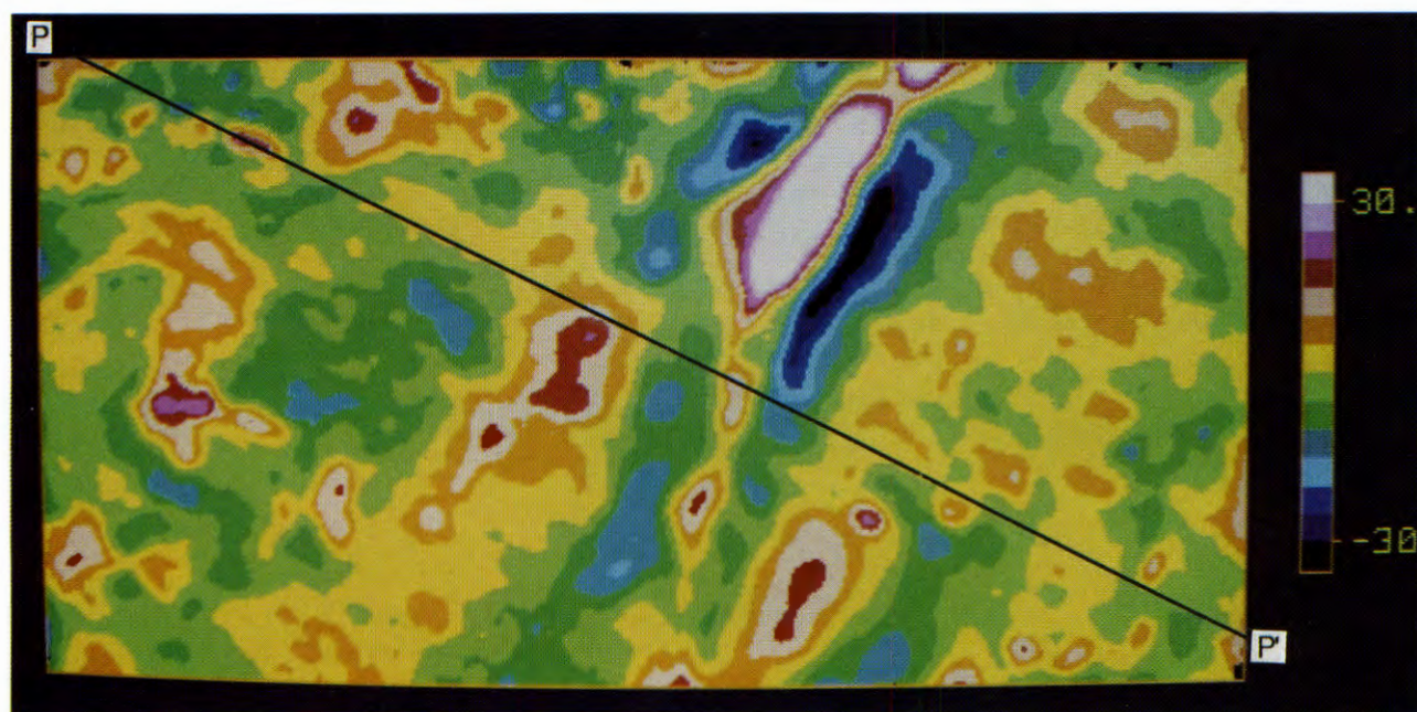
FIGURE 10—GRAVITY MAP OF KANSAS, SEVENTH-ORDER TREND REMOVED.
