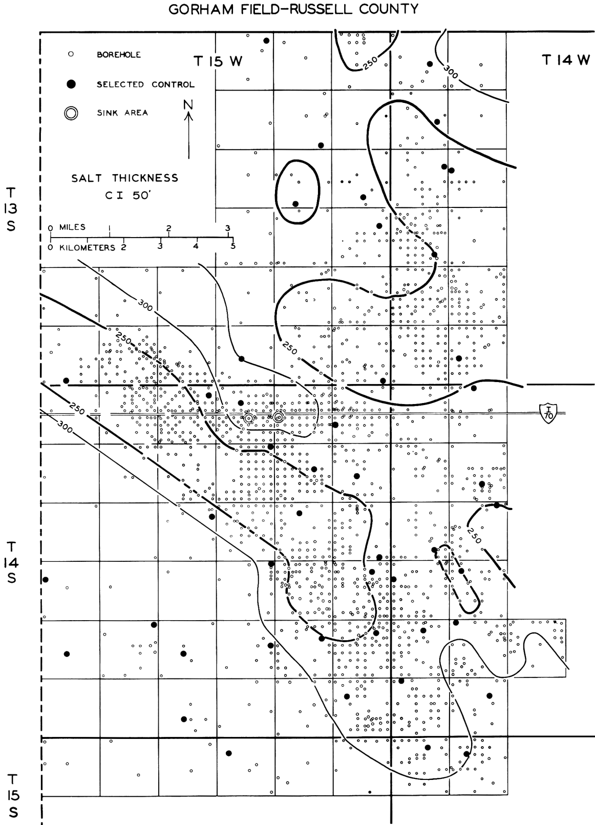
Figure 32--Gorham Oil Field, showing thickness of Hutchinson Salt. Contour interval 50 feet.
